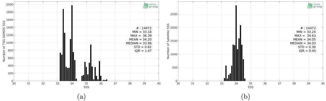
Figure 2: Histograms of SSS from TSG-SAMOS (a) and SMAP-L3-JPL-V4.2-8DAY-RUNNING-60KM (b) considering all match-up pairs per bins of 0.1 over the SPURS 2 Pi-MEP region and for the full satellite product period.
