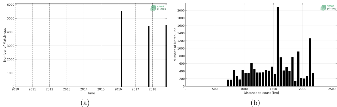
Figure 1: Number of match-ups between TSG-SAMOS and SMAP-L3-JPL-V4.2-8DAY-RUNNING-60KM SSS as a function of time (a) and as function of the distance to coast (b) over the SPURS 2 Pi-MEP region and for the full satellite product period.
