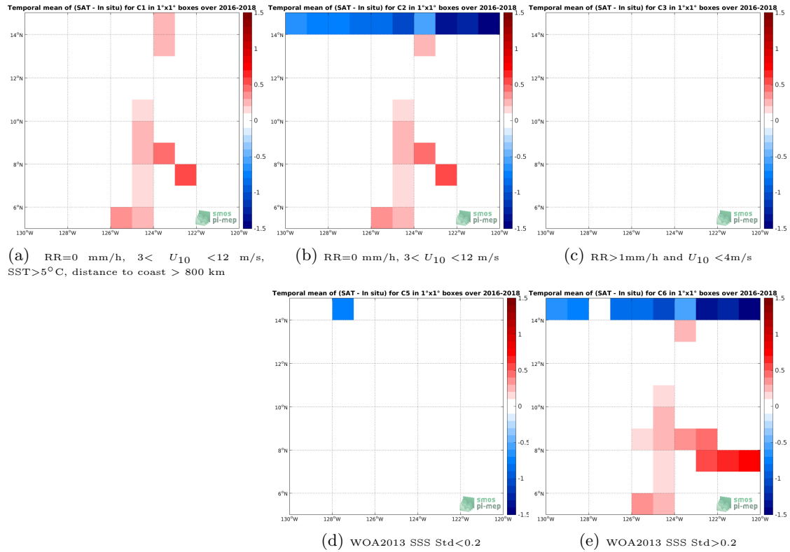
Figure 12: Temporal mean gridded over spatial boxes of size 1^\circ \times 1^\circ of \Delta SSS (SMAP-L3-JPL-V4.2-8DAY-RUNNING-60KM - TSG-SAMOS) for 5 different subdatasets corresponding to:RR=0 mm/h, 3 < U_{10} < 12 m/s, SST >5^\circ C, distance to coast > 800 km (a), RR=0 mm/h, 3 < U_{10} < 12 m/s (b), RR >1 mm/h and U_{10} < 4 m/s (c), WOA2013 SSS Std <0.2 (d), WOA2013 SSS Std >0.2 (e).
