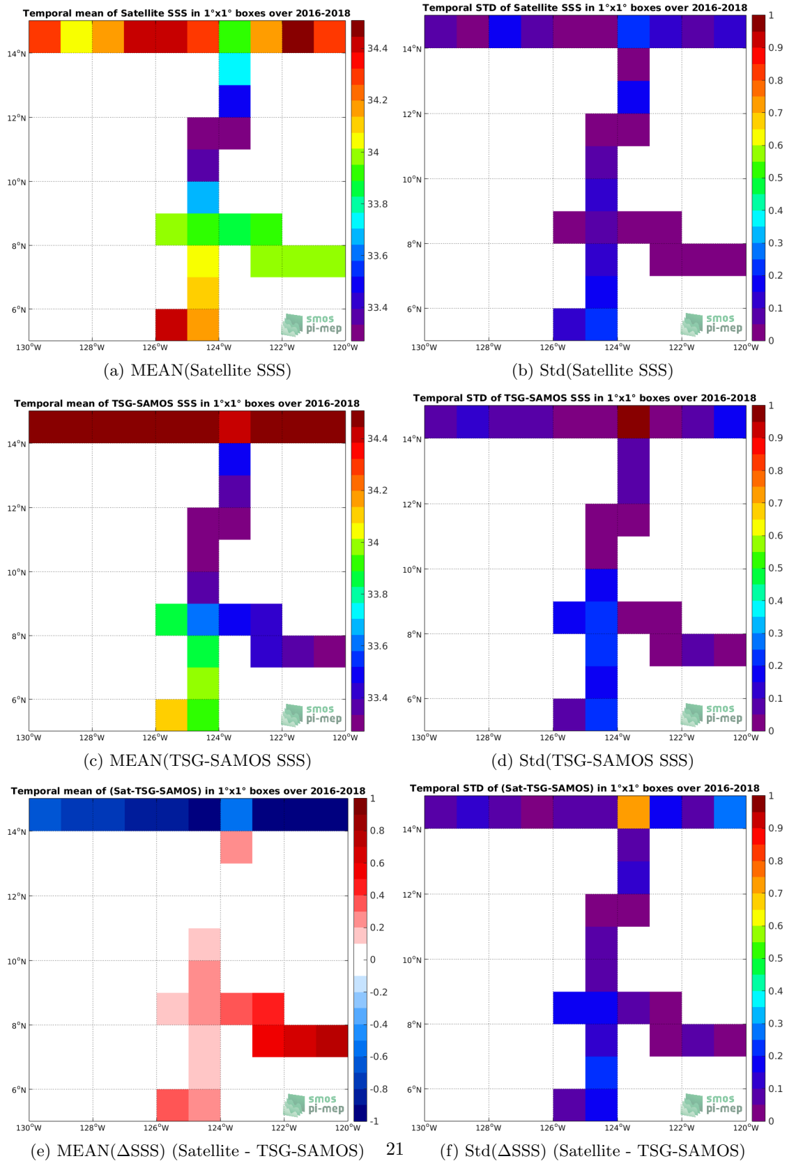
Figure 6: Temporal mean (left) and Std (right) of SSS from SMAP-L3-JPL-V4.2-8DAY-RUNNING-60KM (top), TSG-SAMOS (middle), and of \Delta SSS (Satellite - TSG-SAMOS). Only match-up pairs are used to generate these maps.
