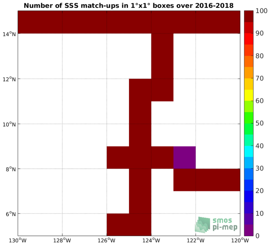
Figure 4: Number of SSS match-ups between TSG-SAMOS SSS and the SMAP-L3-JPL-V4.2-8DAY-RUNNING-60KM SSS product for the SPURS 2 Pi-MEP region over 1°x1° boxes and for the full satellite product period.
