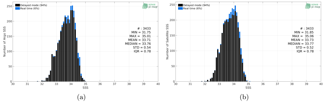
Figure 2: Histograms of SSS from Argo (a) and SMAP SSS L2-AVERAGED v5 (RSS) (b) considering all match-up pairs per bins of 0.1 over the SPURS 2 Pi-MEP region and for the full satellite product period.
