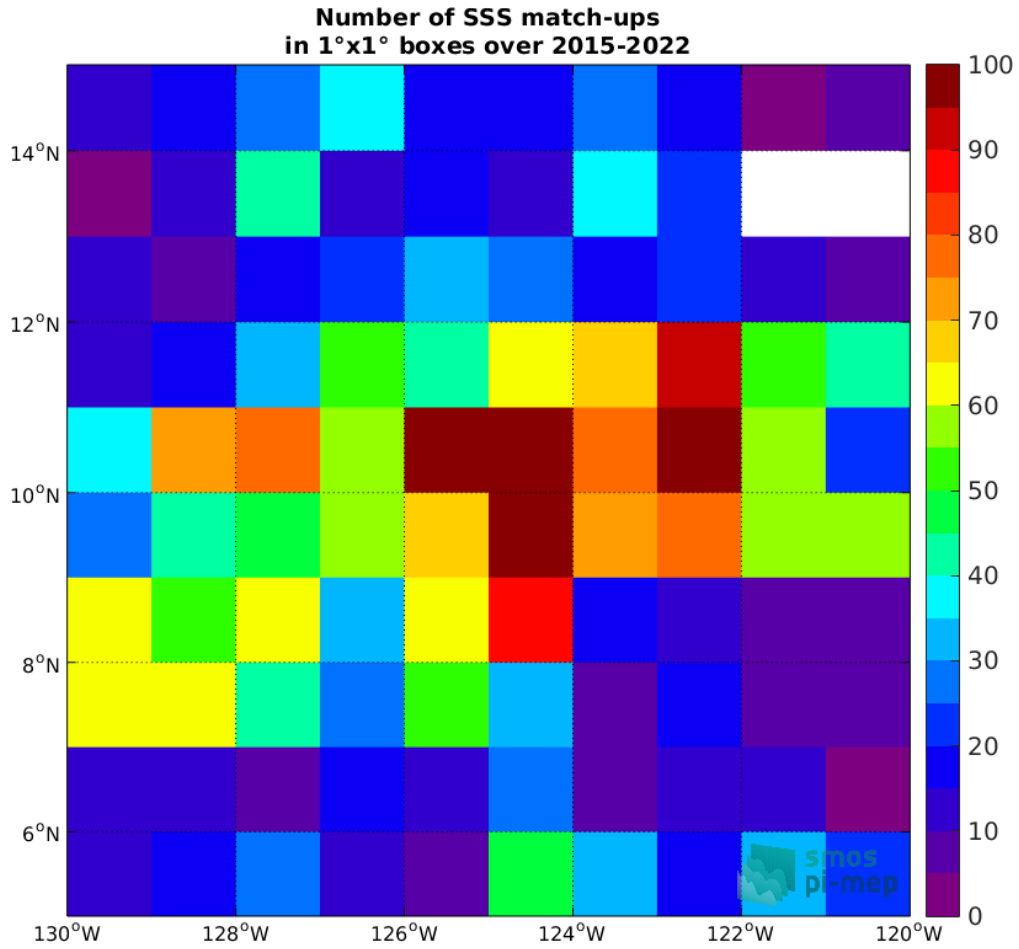
Figure 4: Number of SSS match-ups between Argo SSS and the SMAP SSS L2-AVERAGED v5 (RSS) SSS product for the SPURS 2 Pi-MEP region over 1°x1° boxes and for the full satellite product period.
