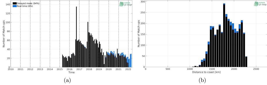
Figure 1: Number of match-ups between Argo and SMAP SSS L2-AVERAGED v5 (RSS) SSS as a function of time (a) and as function of the distance to coast (b) over the SPURS 2 Pi-MEP region and for the full satellite product period.
