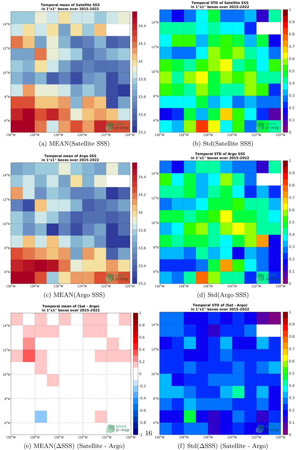
Figure 6: Temporal mean (left) and Std (right) of SSS from SMAP SSS L2-AVERAGED v5.0 (JPL) (top), Argo (middle), and of \Delta SSS (Satellite - Argo). Only match-up pairs are used to generate these maps.
