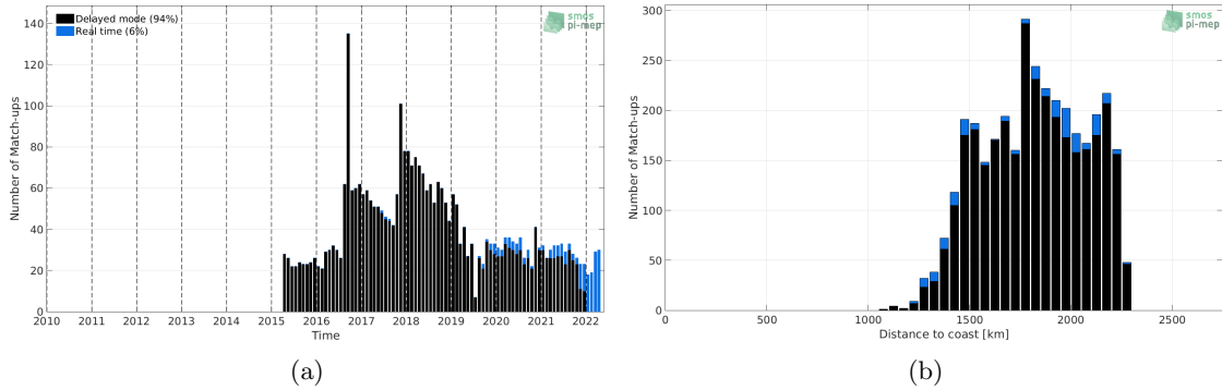
Figure 1: Number of match-ups between Argo and SMAP SSS L2-AVERAGED v5.0 (JPL) SSS as a function of time (a) and as function of the distance to coast (b) over the SPURS 2 Pi-MEP region and for the full satellite product period.
