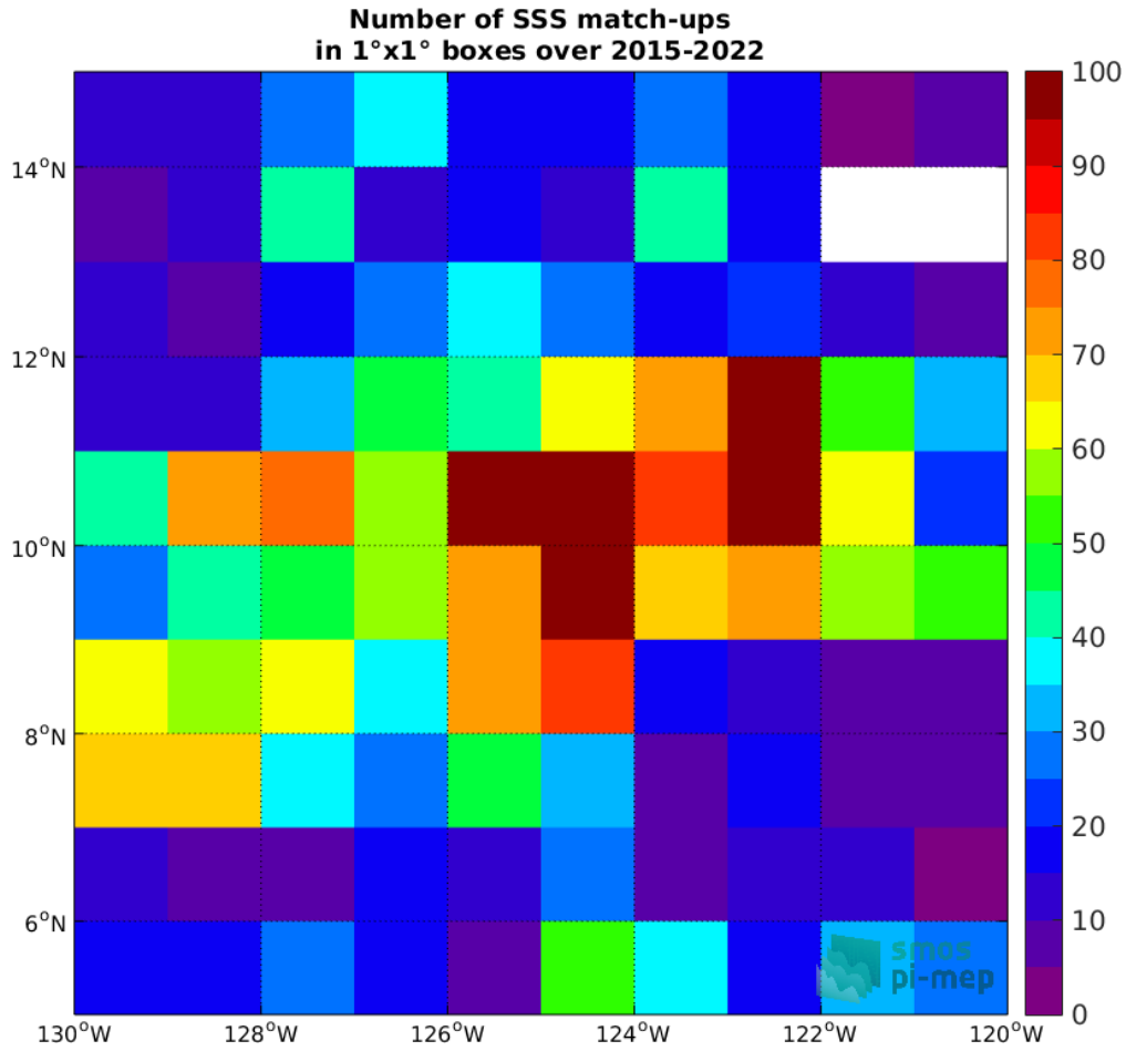
Figure 4: Number of SSS match-ups between Argo SSS and the SMAP SSS L2-AVERAGED v5.0 (JPL) SSS product for the SPURS 2 Pi-MEP region over 1°x1° boxes and for the full satellite product period.
