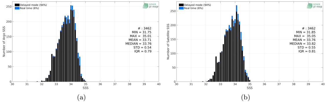
Figure 2: Histograms of SSS from Argo (a) and SMAP SSS L2-AVERAGED v5.0 (JPL) (b) considering all match-up pairs per bins of 0.1 over the SPURS 2 Pi-MEP region and for the full satellite product period.
