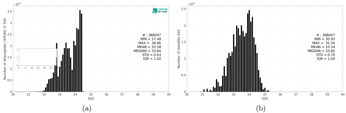
Figure 3: Histograms of SSS from Waveglider (SPURS 2) (a) and SMAP SSS L2 v6 (RSS) (b) considering all match-up pairs per bins of 0.1 over the SPURS 2 Pi-MEP region and for the full satellite product period.
