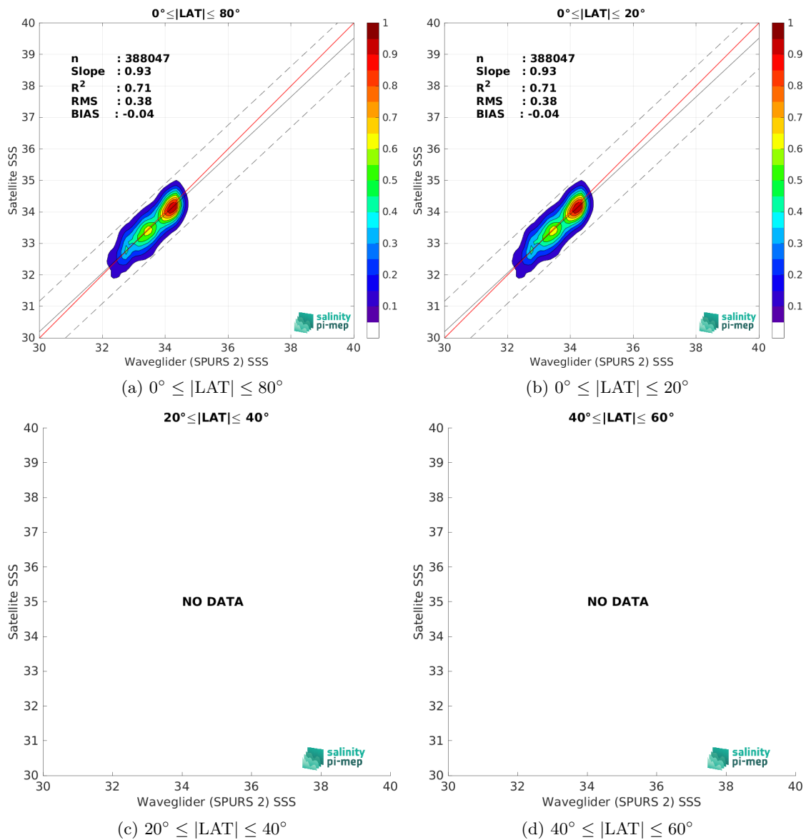
Figure 10: Contour maps of the concentration of SMAP SSS L2 v6 (RSS) SSS (y-axis) versus Waveglider (SPURS 2) SSS (x-axis) at match-up pairs for different latitude bands. For each plot, the red line shows x=y . The black thin and dashed lines indicate a linear fit through the data cloud and the \pm 95\% confidence levels, respectively. The number match-up pairs n , the slope and R^2 coefficient of the linear fit, the root mean square (RMS) and the mean bias between satellite and in situ data are indicated for each latitude band in each plots.
