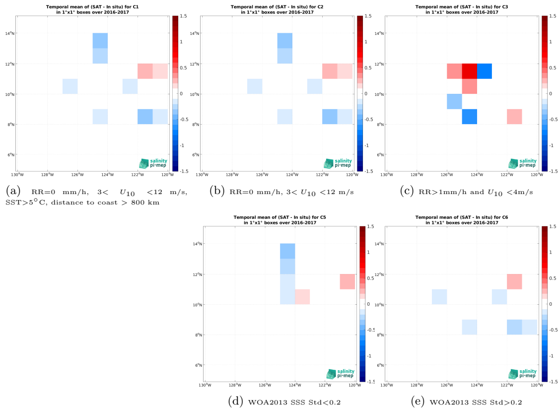
Figure 14: Temporal mean gridded over spatial boxes of size 1^\circ \times 1^\circ of \Delta SSS (SMAP SSS L2 v6 (RSS) - Waveglider (SPURS 2)) for 5 different subdatasets corresponding to:RR=0 mm/h, 3 < U_{10} < 12 m/s, SST>5°C, distance to coast > 800 km (a), RR=0 mm/h, 3 < U_{10} < 12 m/s (b), RR>1mm/h and U_{10} < 4 m/s (c), WOA2013 SSS Std<0.2 (d), WOA2013 SSS Std>0.2 (e).
