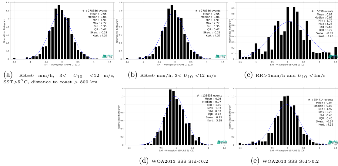
Figure 15: Normalized histogram of \Delta SSS (SMAP SSS L2 v6 (RSS) - Waveglider (SPURS 2)) for 5 different subdatasets corresponding to: RR=0 mm/h, 3 < U_{10} < 12 m/s, SST > 5°C, distance to coast > 800 km (a), RR=0 mm/h, 3 < U_{10} < 12 m/s (b), RR > 1mm/h and U_{10} < 4 m/s (c), WOA2013 SSS Std < 0.2 (d), WOA2013 SSS Std > 0.2 (e).
