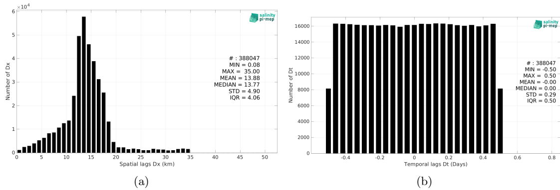
Figure 6: Histograms of the spatial (a) and temporal (b) lags between the location/time of the Waveglider (SPURS 2) measurement and the date of the corresponding SMAP SSS L2 v6 (RSS) SSS pixel.
