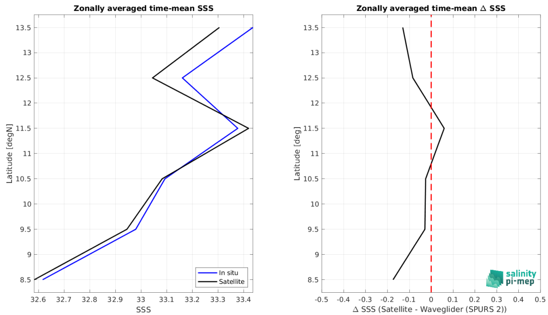
Figure 9: Left panel: Zonal mean SSS from SMAP SSS L2 v6 (RSS) satellite product (black) and from Waveglider (SPURS 2) (blue). Right panel: Zonal mean of \Delta SSS (Satellite - Waveglider (SPURS 2)) for all the collected Pi-MEP match-up pairs estimated over the full satellite product period.
