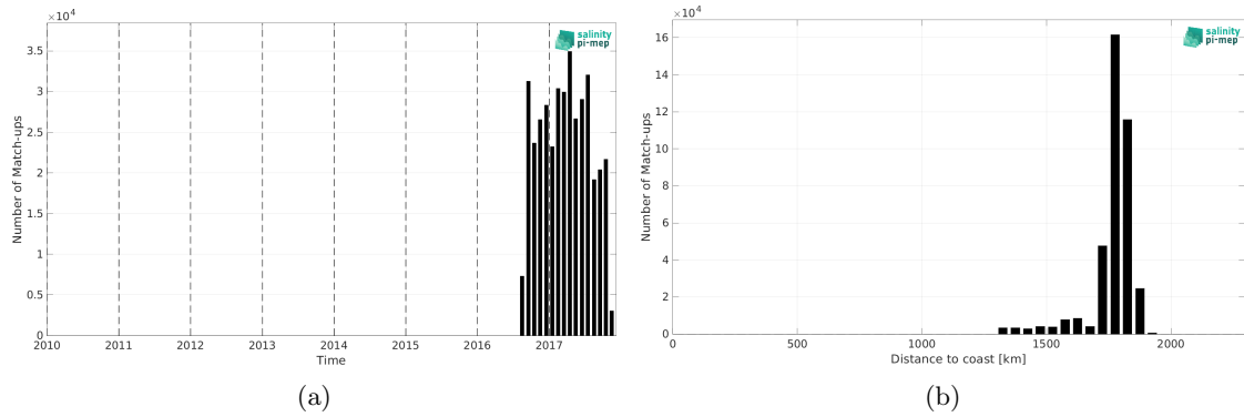
Figure 2: Number of match-ups between Waveglider (SPURS 2) and SMAP SSS L2 v6 (RSS) SSS as a function of time (a) and as function of the distance to coast (b) over the SPURS 2 Pi-MEP region and for the full satellite product period.
