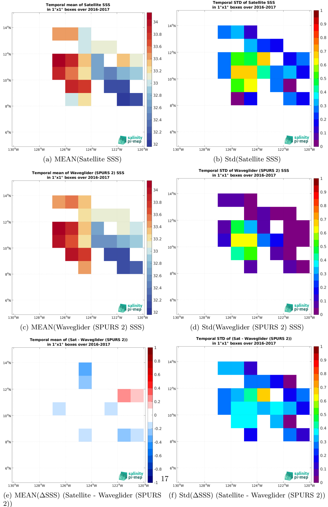
Figure 7: Temporal mean (left) and Std (right) of SSS from SMAP SSS L2 v6 (RSS) (top), Waveglider (SPURS 2) (middle), and of \Delta SSS (Satellite - Waveglider (SPURS 2)). Only match-up pairs are used to generate these maps.
