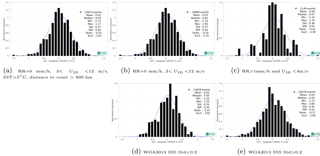
Figure 15: Normalized histogram of \Delta SSS (SMAP SSS L2 v6 (RSS) - Seaglider (SPURS 2)) for 5 different subdatasets corresponding to: RR=0 mm/h, 3 < U_{10} < 12 m/s, SST > 5°C, distance to coast > 800 km (a), RR=0 mm/h, 3 < U_{10} < 12 m/s (b), RR > 1mm/h and U_{10} < 4 m/s (c), WOA2013 SSS Std < 0.2 (d), WOA2013 SSS Std > 0.2 (e).
