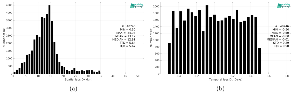
Figure 6: Histograms of the spatial (a) and temporal (b) lags between the location/time of the Seaglider (SPURS 2) measurement and the date of the corresponding SMAP SSS L2 v6 (RSS) SSS pixel.
