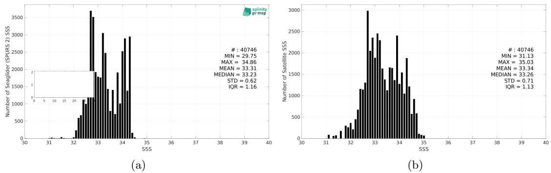
Figure 3: Histograms of SSS from Seaglider (SPURS 2) (a) and SMAP SSS L2 v6 (RSS) (b) considering all match-up pairs per bins of 0.1 over the SPURS 2 Pi-MEP region and for the full satellite product period.
