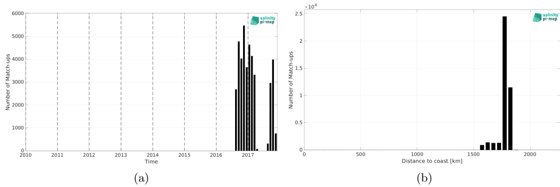
Figure 2: Number of match-ups between Seaglider (SPURS 2) and SMAP SSS L2 v6 (RSS) SSS as a function of time (a) and as function of the distance to coast (b) over the SPURS 2 Pi-MEP region and for the full satellite product period.
