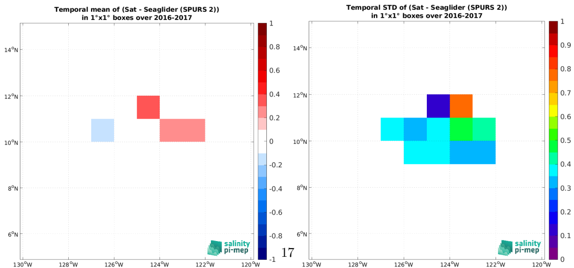
(e) MEAN( \Delta SSS) (Satellite - Seaglider (SPURS 2))
