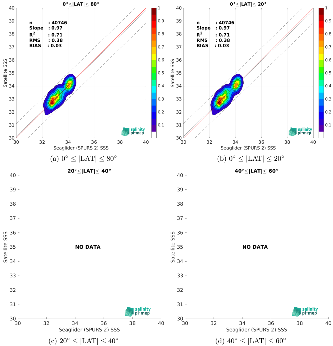
Figure 10: Contour maps of the concentration of SMAP SSS L2 v6 (RSS) SSS (y-axis) versus Seaglider (SPURS 2) SSS (x-axis) at match-up pairs for different latitude bands. For each plot, the red line shows x=y . The black thin and dashed lines indicate a linear fit through the data cloud and the \pm 95\% confidence levels, respectively. The number match-up pairs n , the slope and R^2 coefficient of the linear fit, the root mean square (RMS) and the mean bias between satellite and in situ data are indicated for each latitude band in each plots.
