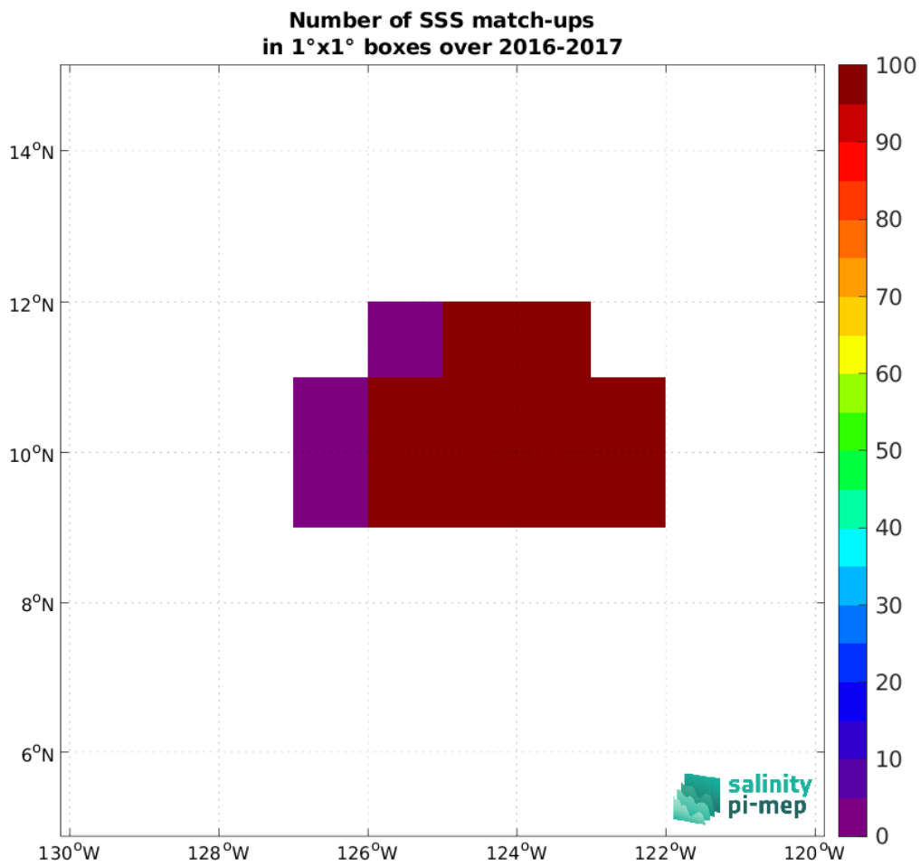
Figure 5: Number of SSS match-ups between Seagliders (SPURS 2) SSS and the SMAP SSS L2 v6 (RSS) SSS product for the SPURS 2 Pi-MEP region over 1^\circ \times 1^\circ boxes and for the full satellite product period.
