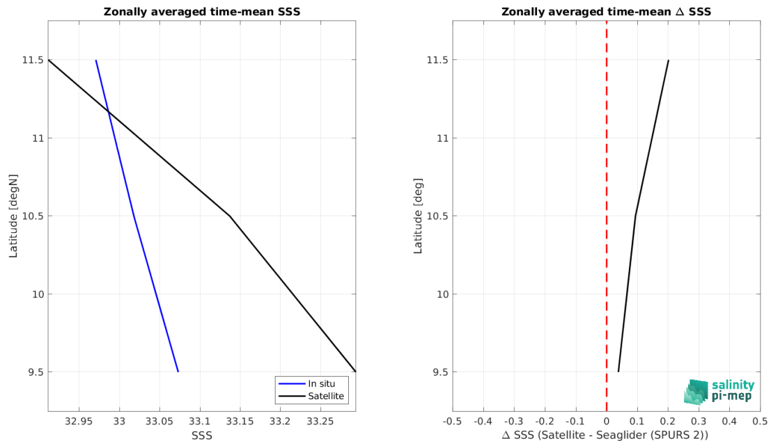
Figure 9: Left panel: Zonal mean SSS from SMAP SSS L2 v6 (RSS) satellite product (black) and from Seaglider (SPURS 2) (blue). Right panel: Zonal mean of \Delta SSS (Satellite - Seaglider (SPURS 2)) for all the collected Pi-MEP match-up pairs estimated over the full satellite product period.
