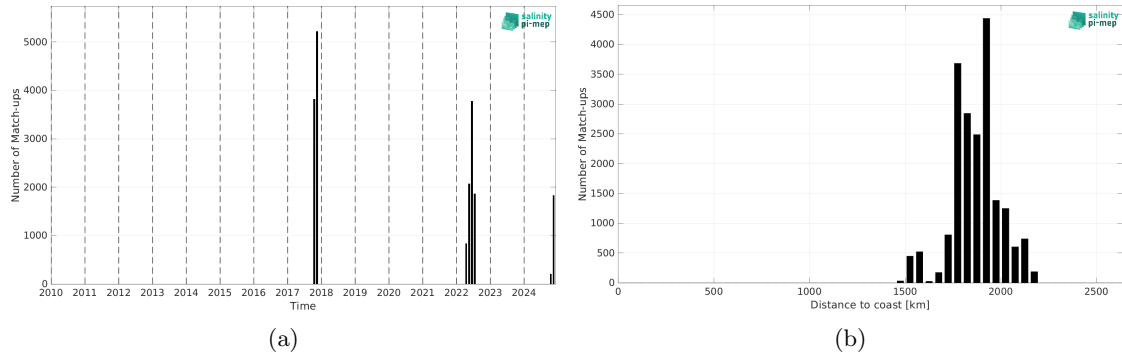
Figure 2: Number of match-ups between Saildrone and SMAP SSS L2 v6 (RSS) SSS as a function of time (a) and as function of the distance to coast (b) over the SPURS 2 Pi-MEP region and for the full satellite product period.
