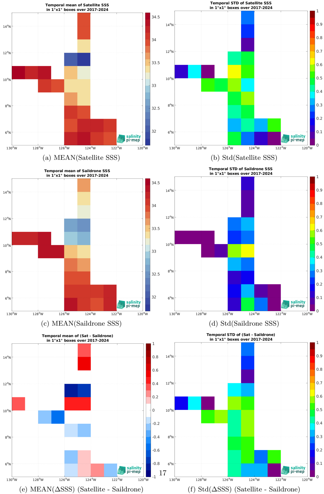
Figure 7: Temporal mean (left) and Std (right) of SSS from SMAP SSS L2 v6 (RSS) (top), Saildrone (middle), and of \Delta SSS (Satellite - Saildrone). Only match-up pairs are used to generate these maps.
