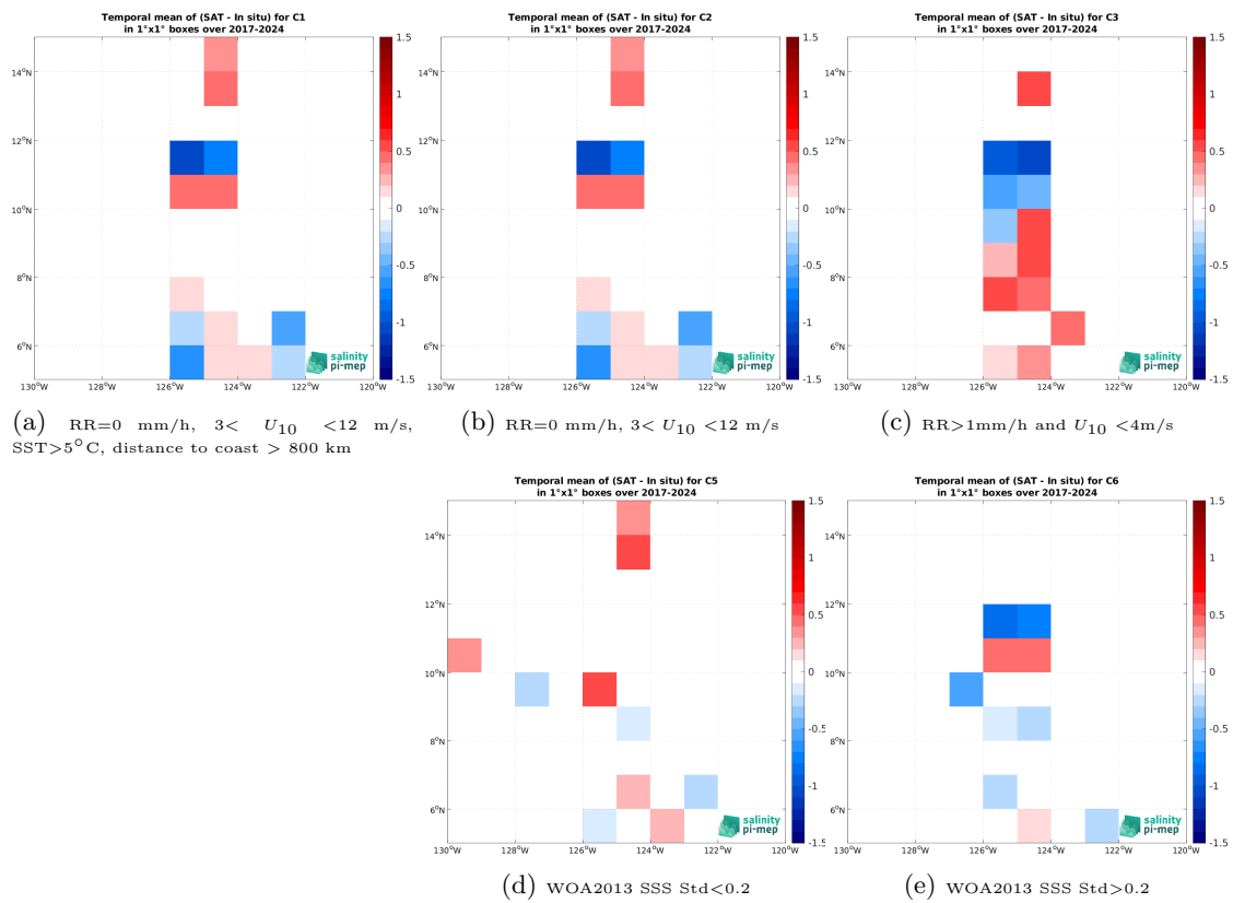
Figure 14: Temporal mean gridded over spatial boxes of size 1^\circ \times 1^\circ of \Delta SSS (SMAP SSS L2 v6 (RSS) - Saildrone) for 5 different subdatasets corresponding to:RR=0 mm/h, 3 < U_{10} < 12 m/s, SST>5°C, distance to coast > 800 km (a), RR=0 mm/h, 3 < U_{10} < 12 m/s (b), RR>1mm/h and U_{10} < 4 m/s (c), WOA2013 SSS Std<0.2 (d), WOA2013 SSS Std>0.2 (e).
