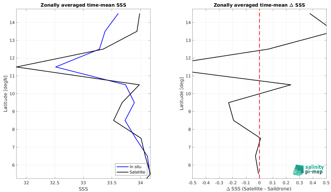
Figure 9: Left panel: Zonal mean SSS from SMAP SSS L2 v6 (RSS) satellite product (black) and from Sairdron (blue). Right panel: Zonal mean of \Delta SSS (Satellite - Sairdron) for all the collected Pi-MEP match-up pairs estimated over the full satellite product period.
