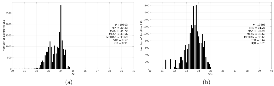
Figure 3: Histograms of SSS from Saildrone (a) and SMAP SSS L2 v6 (RSS) (b) considering all match-up pairs per bins of 0.1 over the SPURS 2 Pi-MEP region and for the full satellite product period.
