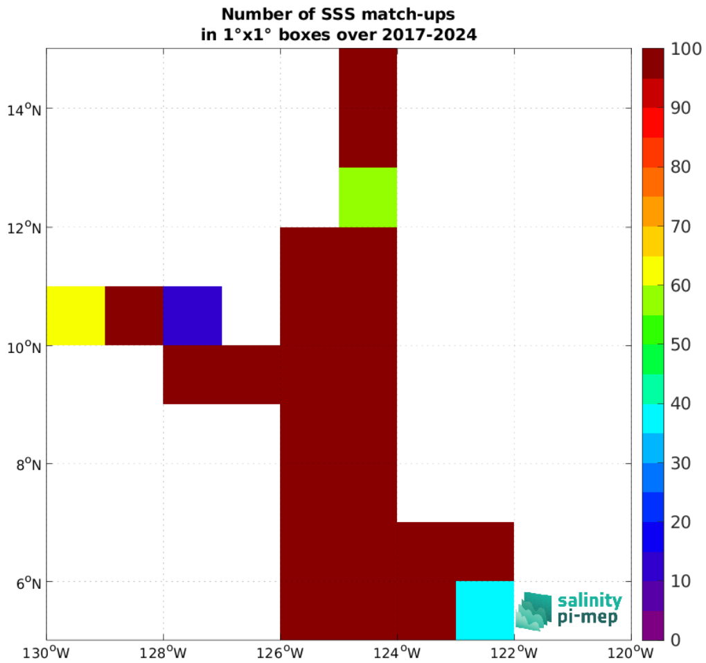
Figure 5: Number of SSS match-ups between Saildrone SSS and the SMAP SSS L2 v6 (RSS) SSS product for the SPURS 2 Pi-MEP region over 1°x1° boxes and for the full satellite product period.
