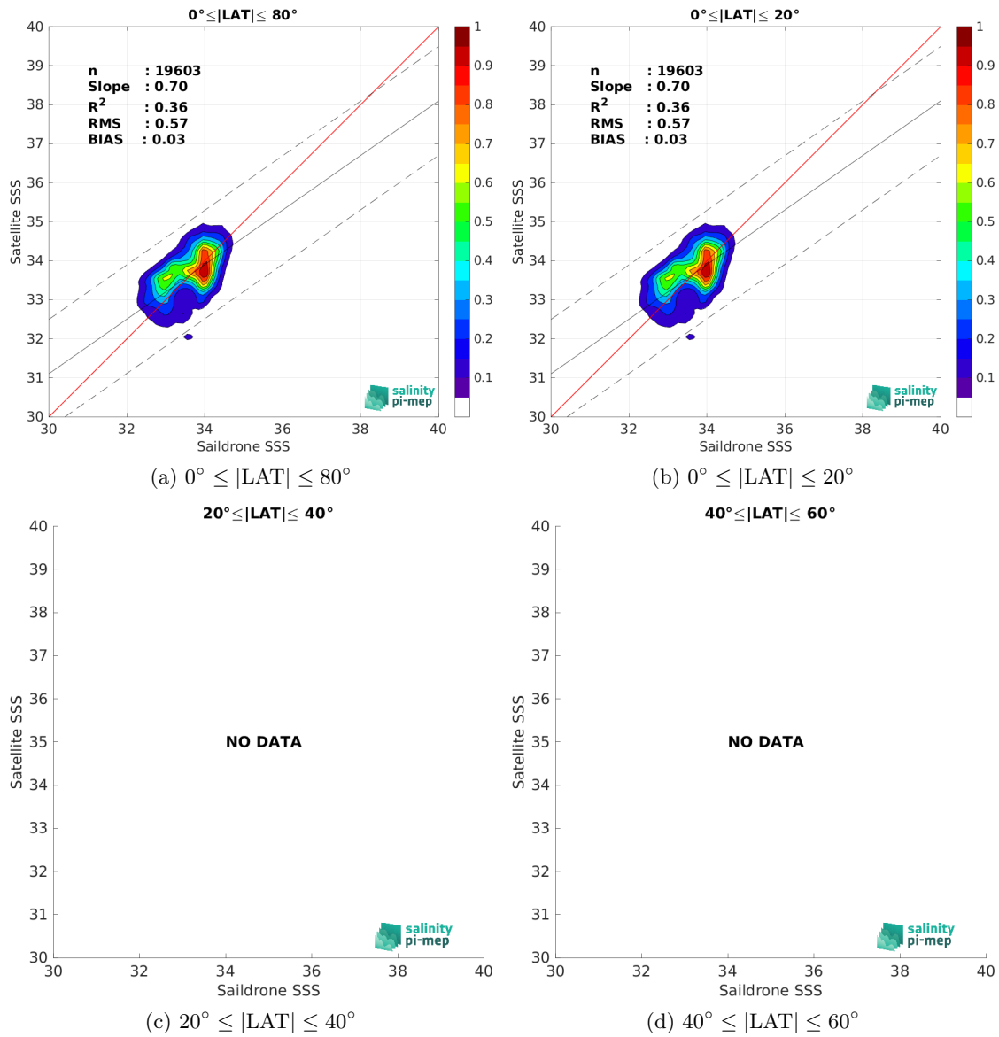
Figure 10: Contour maps of the concentration of SMAP SSS L2 v6 (RSS) SSS (y-axis) versus Sailldrone SSS (x-axis) at match-up pairs for different latitude bands. For each plot, the red line shows x=y . The black thin and dashed lines indicate a linear fit through the data cloud and the \pm 95\% confidence levels, respectively. The number match-up pairs n , the slope and R^2 coefficient of the linear fit, the root mean square (RMS) and the mean bias between satellite and in situ data are indicated for each latitude band in each plots.
