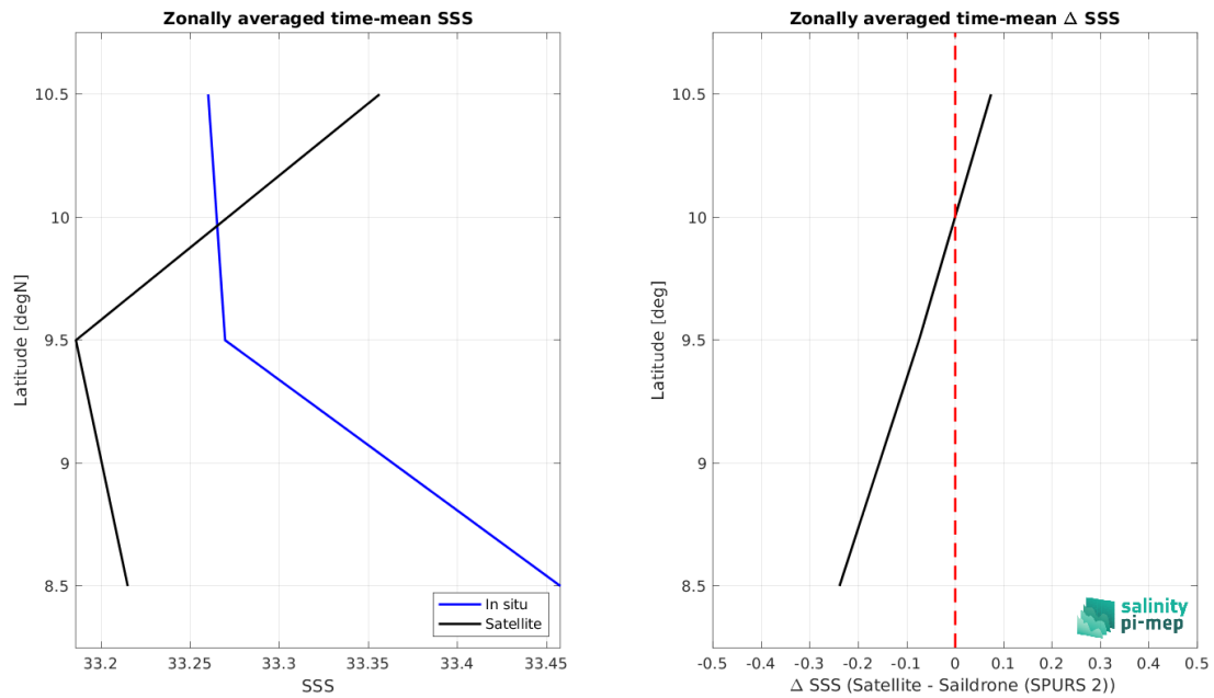
Figure 9: Left panel: Zonal mean SSS from SMAP SSS L2 v6 (RSS) satellite product (black) and from Saildrone (SPURS 2) (blue). Right panel: Zonal mean of \Delta SSS (Satellite - Saildrone (SPURS 2)) for all the collected Pi-MEP match-up pairs estimated over the full satellite product period.
