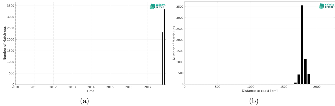
Figure 2: Number of match-ups between Saildrone (SPURS 2) and SMAP SSS L2 v6 (RSS) SSS as a function of time (a) and as function of the distance to coast (b) over the SPURS 2 Pi-MEP region and for the full satellite product period.
