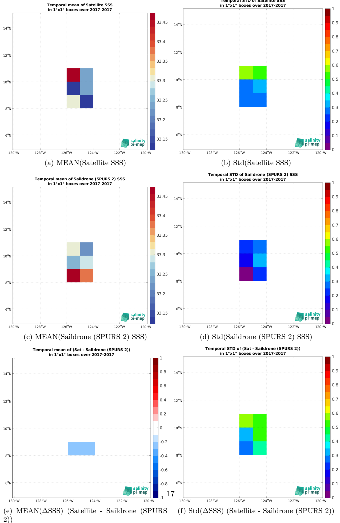
Figure 7: Temporal mean (left) and Std (right) of SSS from SMAP SSS L2 v6 (RSS) (top), Saildrone (SPURS 2) (middle), and of \Delta SSS (Satellite - Saildrone (SPURS 2)). Only match-up pairs are used to generate these maps.
