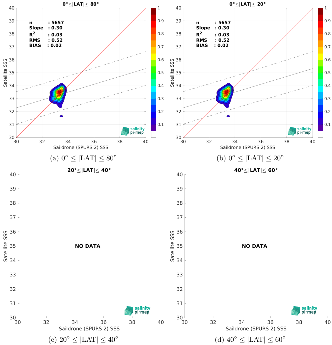
Figure 10: Contour maps of the concentration of SMAP SSS L2 v6 (RSS) SSS (y-axis) versus Saildrone (SPURS 2) SSS (x-axis) at match-up pairs for different latitude bands. For each plot, the red line shows x=y . The black thin and dashed lines indicate a linear fit through the data cloud and the \pm 95\% confidence levels, respectively. The number match-up pairs n , the slope and R^2 coefficient of the linear fit, the root mean square (RMS) and the mean bias between satellite and in situ data are indicated for each latitude band in each plots.
