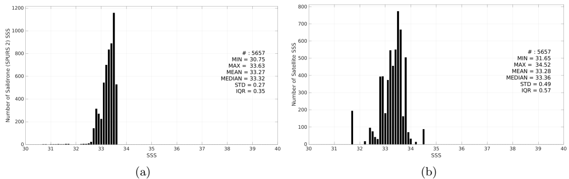
Figure 3: Histograms of SSS from Saildrone (SPURS 2) (a) and SMAP SSS L2 v6 (RSS) (b) considering all match-up pairs per bins of 0.1 over the SPURS 2 Pi-MEP region and for the full satellite product period.
