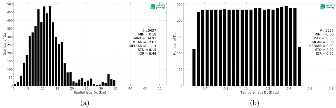
Figure 6: Histograms of the spatial (a) and temporal (b) lags between the location/time of the Saildrone (SPURS 2) measurement and the date of the corresponding SMAP SSS L2 v6 (RSS) SSS pixel.
