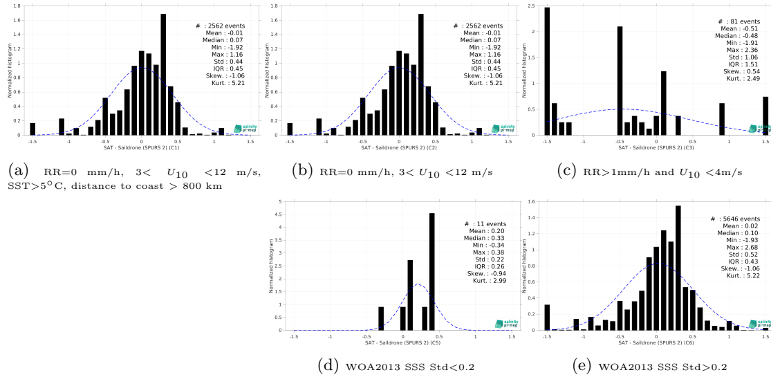
Figure 15: Normalized histogram of \Delta SSS (SMAP SSS L2 v6 (RSS) - Saildrone (SPURS 2)) for 5 different subdatasets corresponding to: RR=0 mm/h, 3 < U_{10} < 12 m/s, SST > 5°C, distance to coast > 800 km (a), RR=0 mm/h, 3 < U_{10} < 12 m/s (b), RR > 1mm/h and U_{10} < 4 m/s (c), WOA2013 SSS Std < 0.2 (d), WOA2013 SSS Std > 0.2 (e).
