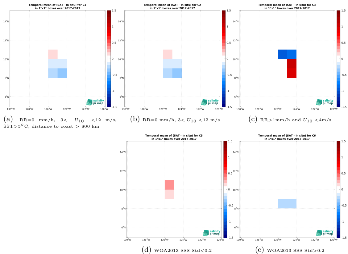
Figure 14: Temporal mean gridded over spatial boxes of size 1^\circ \times 1^\circ of \Delta SSS (SMAP SSS L2 v6 (RSS) - Saildrone (SPURS 2)) for 5 different subdatasets corresponding to:RR=0 mm/h, 3 < U_{10} < 12 m/s, SST >5^\circ C, distance to coast > 800 km (a), RR=0 mm/h, 3 < U_{10} < 12 m/s (b), RR >1 mm/h and U_{10} < 4 m/s (c), WOA2013 SSS Std <0.2 (d), WOA2013 SSS Std >0.2 (e).
