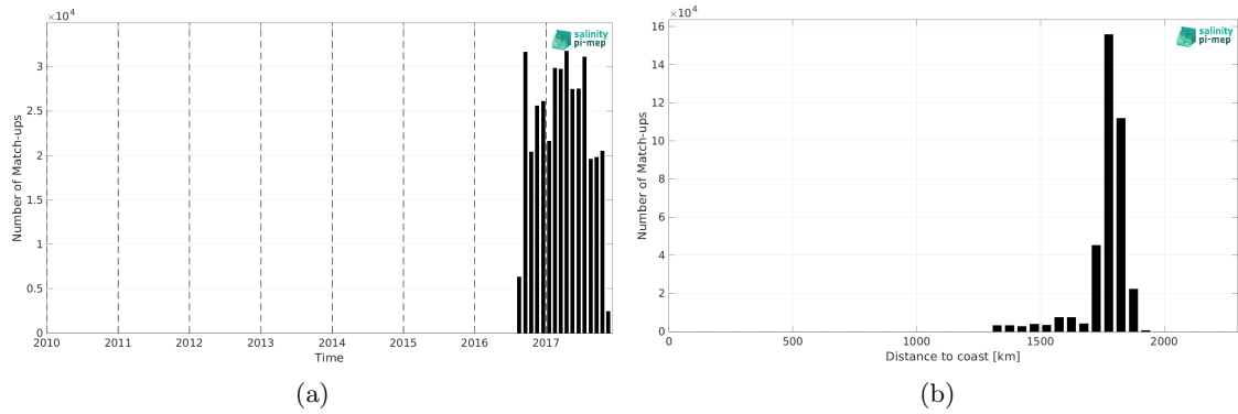
Figure 2: Number of match-ups between Waveglider (SPURS 2) and SMAP SSS L2 v6 - 40 km (RSS) SSS as a function of time (a) and as function of the distance to coast (b) over the SPURS 2 Pi-MEP region and for the full satellite product period.
