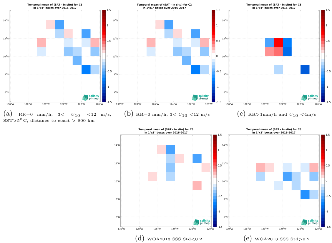
Figure 14: Temporal mean gridded over spatial boxes of size 1^\circ \times 1^\circ of \Delta SSS (SMAP SSS L2 v6 - 40 km (RSS) - Waveglider (SPURS 2)) for 5 different subdatasets corresponding to: RR=0 mm/h, 3 < U_{10} < 12 m/s, SST > 5°C, distance to coast > 800 km (a), RR=0 mm/h, 3 < U_{10} < 12 m/s (b), RR > 1mm/h and U_{10} < 4 m/s (c), WOA2013 SSS Std < 0.2 (d), WOA2013 SSS Std > 0.2 (e).
