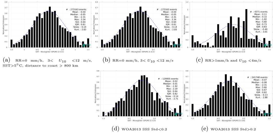
Figure 15: Normalized histogram of \Delta SSS (SMAP SSS L2 v6 - 40 km (RSS) - Waveglider (SPURS 2)) for 5 different subdatasets corresponding to: RR=0 mm/h, 3 < U_{10} < 12 m/s, SST > 5°C, distance to coast > 800 km (a), RR=0 mm/h, 3 < U_{10} < 12 m/s (b), RR > 1mm/h and U_{10} < 4 m/s (c), WOA2013 SSS Std < 0.2 (d), WOA2013 SSS Std > 0.2 (e).
