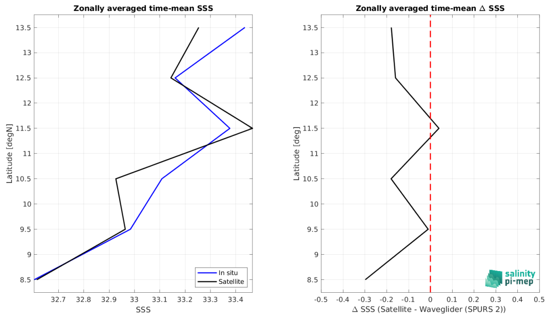
Figure 9: Left panel: Zonal mean SSS from SMAP SSS L2 v6 - 40 km (RSS) satellite product (black) and from Waveglider (SPURS 2) (blue). Right panel: Zonal mean of \Delta SSS (Satellite - Waveglider (SPURS 2)) for all the collected Pi-MEP match-up pairs estimated over the full satellite product period.
