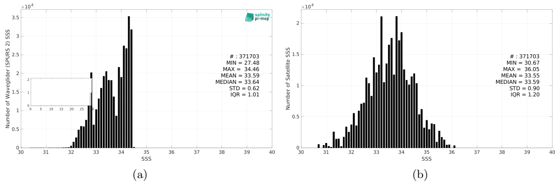
Figure 3: Histograms of SSS from Waveglider (SPURS 2) (a) and SMAP SSS L2 v6 - 40 km (RSS) (b) considering all match-up pairs per bins of 0.1 over the SPURS 2 Pi-MEP region and for the full satellite product period.
