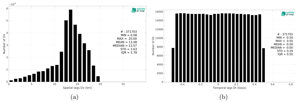
Figure 6: Histograms of the spatial (a) and temporal (b) lags between the location/time of the Waveglider (SPURS 2) measurement and the date of the corresponding SMAP SSS L2 v6 - 40 km (RSS) SSS pixel.
