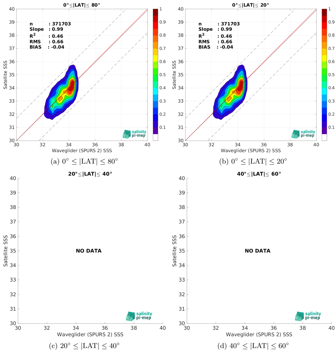
Figure 10: Contour maps of the concentration of SMAP SSS L2 v6 - 40 km (RSS) SSS (y-axis) versus Waveglider (SPURS 2) SSS (x-axis) at match-up pairs for different latitude bands. For each plot, the red line shows x=y . The black thin and dashed lines indicate a linear fit through the data cloud and the \pm 95\% confidence levels, respectively. The number match-up pairs n , the slope and R^2 coefficient of the linear fit, the root mean square (RMS) and the mean bias between satellite and in situ data are indicated for each latitude band in each plots.
