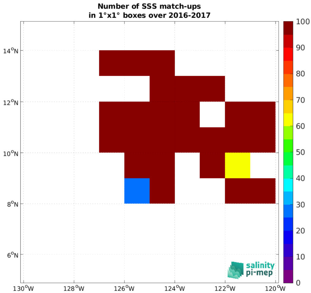
Figure 5: Number of SSS match-ups between Waveglider (SPURS 2) SSS and the SMAP SSS L2 v6 - 40 km (RSS) SSS product for the SPURS 2 Pi-MEP region over 1°x1° boxes and for the full satellite product period.
