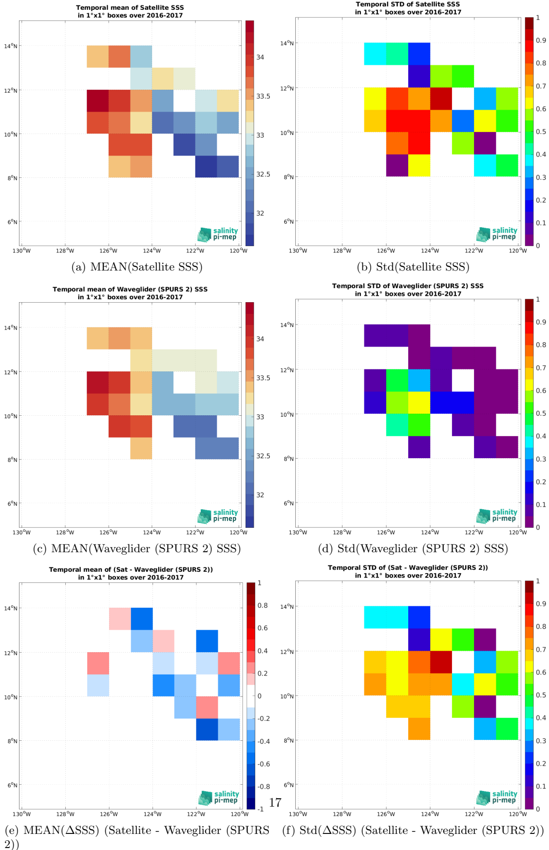
Figure 7: Temporal mean (left) and Std (right) of SSS from SMAP SSS L2 v6 - 40 km (RSS) (top), Waveglider (SPURS 2) (middle), and of \Delta SSS (Satellite - Waveglider (SPURS 2)). Only match-up pairs are used to generate these maps.
