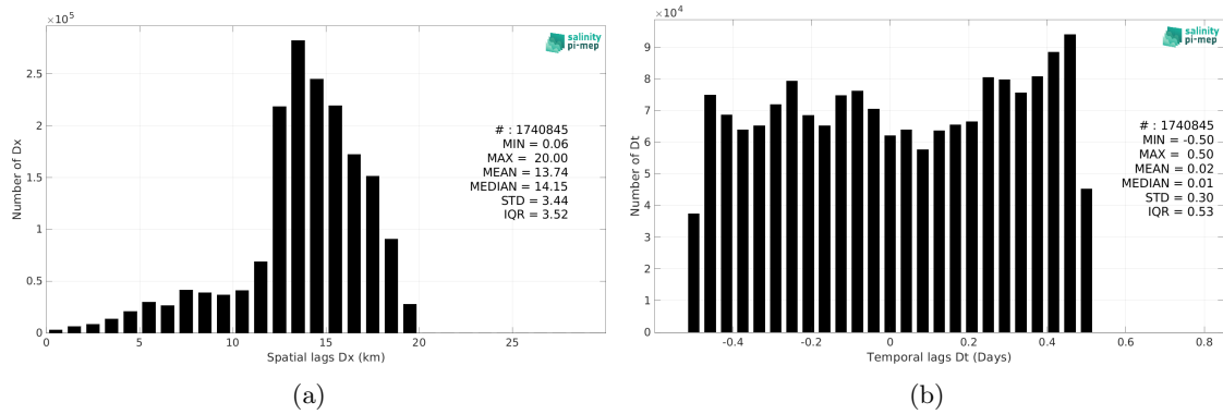
Figure 6: Histograms of the spatial (a) and temporal (b) lags between the location/time of the Salinity Snake (SPURS 2) measurement and the date of the corresponding SMAP SSS L2 v6 - 40 km (RSS) SSS pixel.
