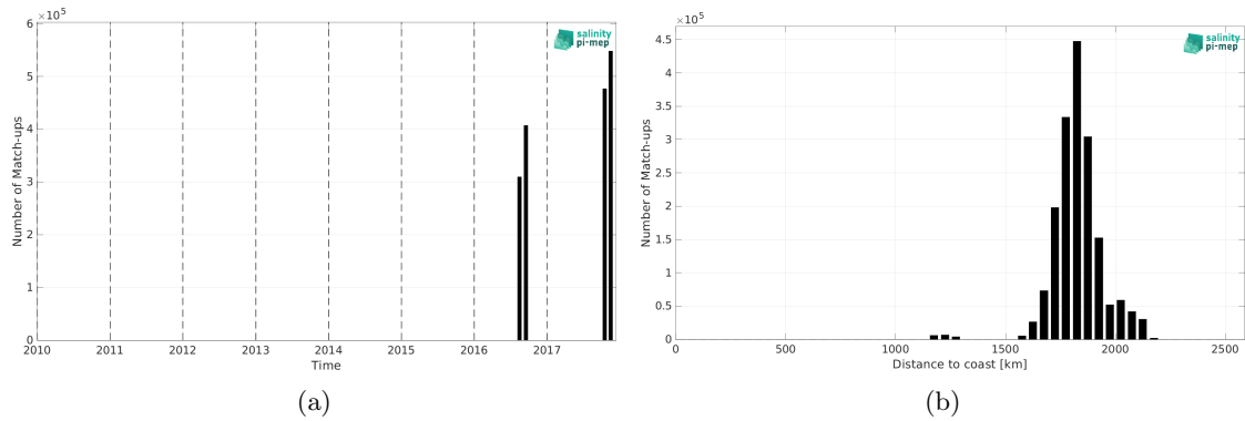
Figure 2: Number of match-ups between Salinity Snake (SPURS 2) and SMAP SSS L2 v6 - 40 km (RSS) SSS as a function of time (a) and as function of the distance to coast (b) over the SPURS 2 Pi-MEP region and for the full satellite product period.
