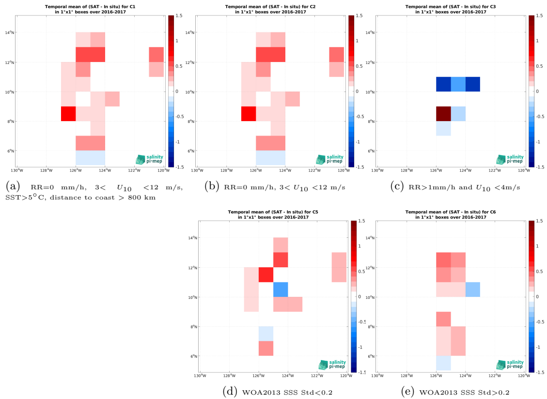
Figure 14: Temporal mean gridded over spatial boxes of size 1^\circ \times 1^\circ of \Delta\text{SSS} (SMAP SSS L2 v6 - 40 km (RSS) - Salinity Snake (SPURS 2)) for 5 different subdatasets corresponding to:RR=0 mm/h, 3 < U_{10} < 12 m/s, SST >5^\circ\text{C} , distance to coast > 800 km (a), RR=0 mm/h, 3 < U_{10} < 12 m/s (b), RR >1 mm/h and U_{10} < 4 m/s (c), WOA2013 SSS Std <0.2 (d), WOA2013 SSS Std >0.2 (e).
