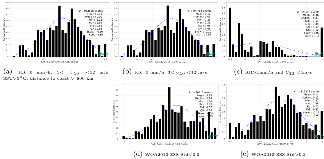
Figure 15: Normalized histogram of \Delta SSS (SMAP SSS L2 v6 - 40 km (RSS) - Salinity Snake (SPURS 2)) for 5 different subdatasets corresponding to: RR=0 mm/h, 3 < U_{10} < 12 m/s, SST > 5°C, distance to coast > 800 km (a), RR=0 mm/h, 3 < U_{10} < 12 m/s (b), RR > 1mm/h and U_{10} < 4 m/s (c), WOA2013 SSS Std < 0.2 (d), WOA2013 SSS Std > 0.2 (e).
