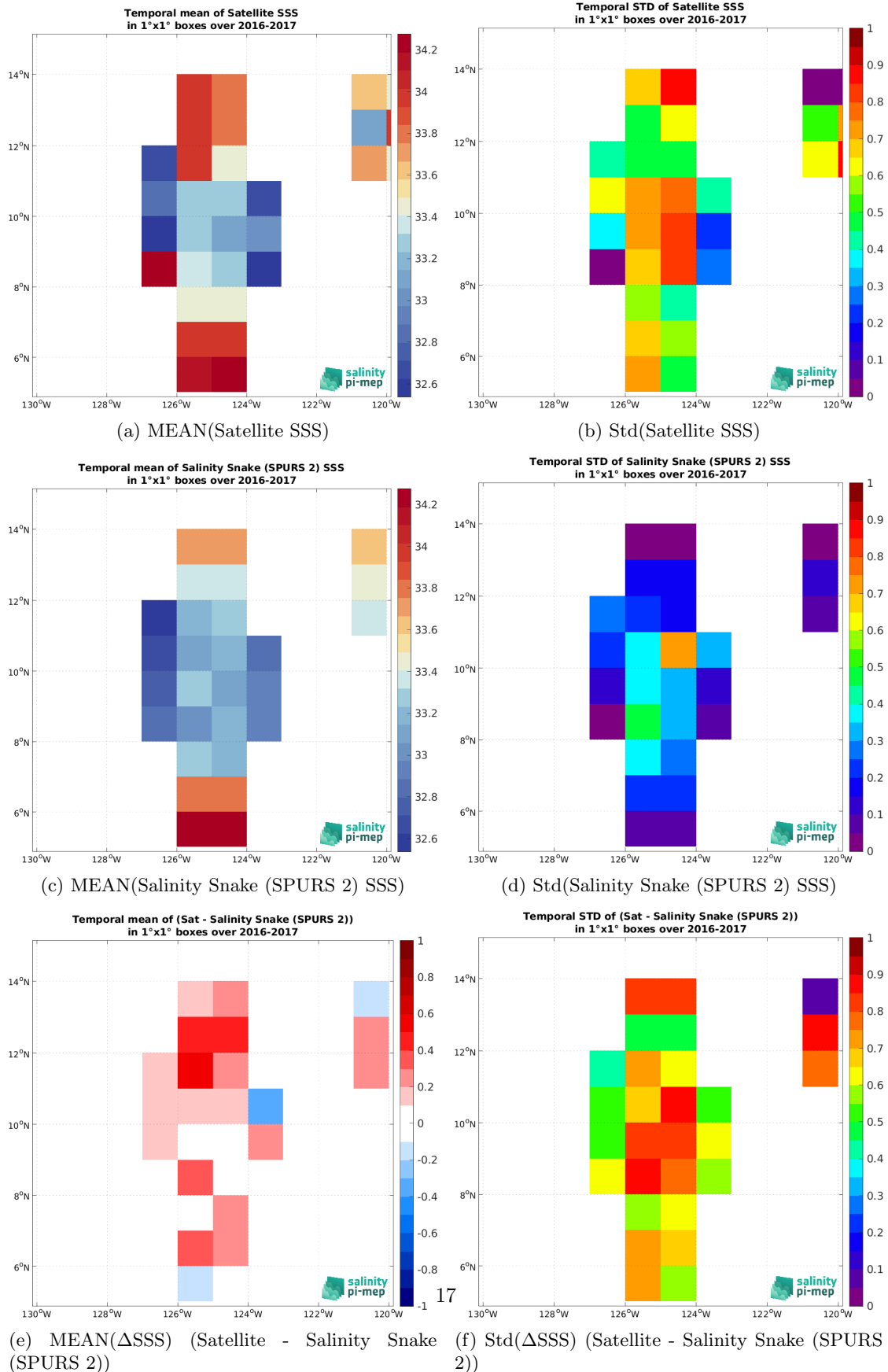
Figure 7: Temporal mean (left) and Std (right) of SSS from SMAP SSS L2 v6 - 40 km (RSS) (top), Salinity Snake (SPURS 2) (middle), and of \Delta SSS (Satellite - Salinity Snake (SPURS 2)). Only match-up pairs are used to generate these maps.
