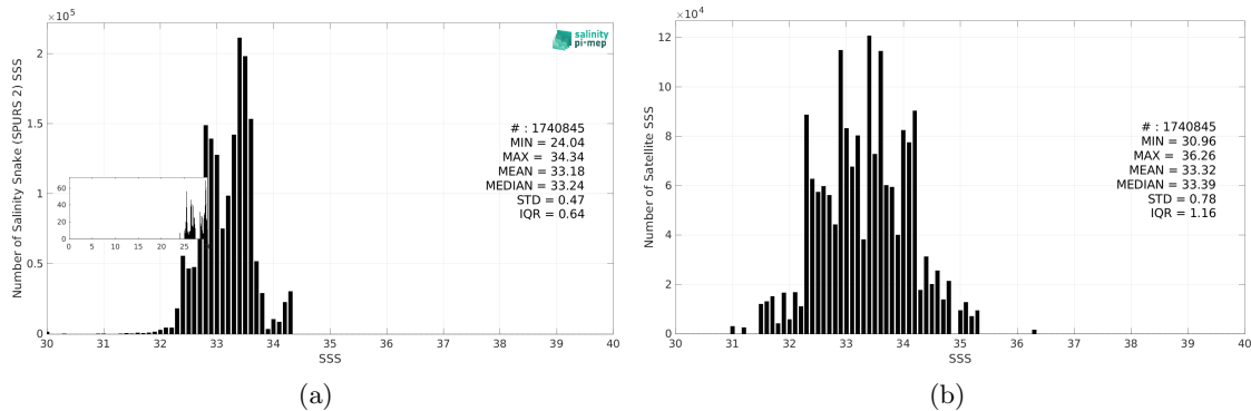
Figure 3: Histograms of SSS from Salinity Snake (SPURS 2) (a) and SMAP SSS L2 v6 - 40 km (RSS) (b) considering all match-up pairs per bins of 0.1 over the SPURS 2 Pi-MEP region and for the full satellite product period.
