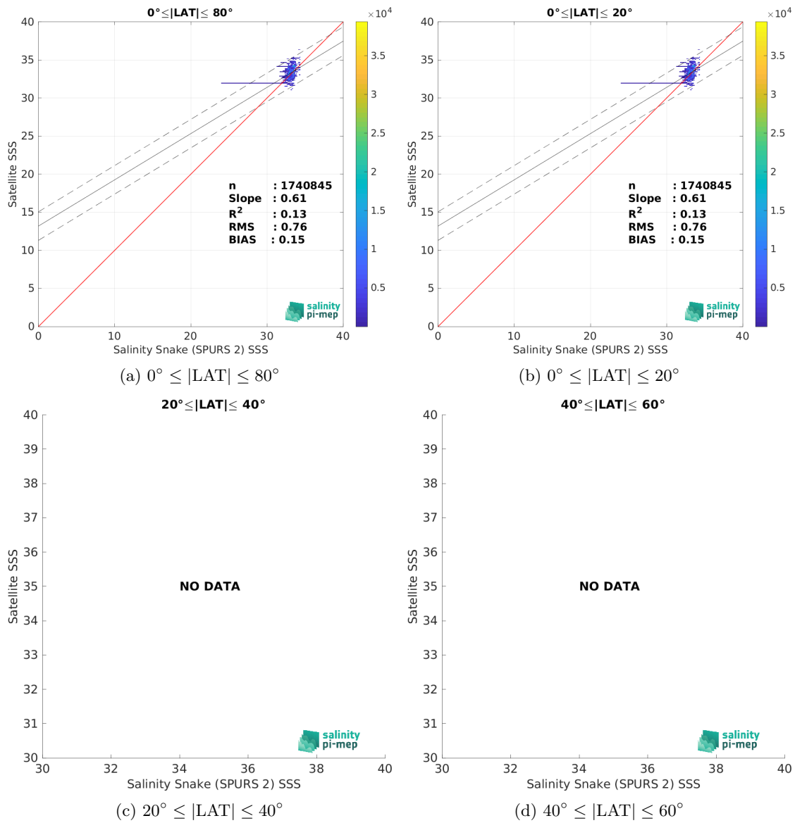
Figure 10: Contour maps of the concentration of SMAP SSS L2 v6 - 40 km (RSS) SSS (y-axis) versus Salinity Snake (SPURS 2) SSS (x-axis) at match-up pairs for different latitude bands. For each plot, the red line shows x=y . The black thin and dashed lines indicate a linear fit through the data cloud and the \pm 95\% confidence levels, respectively. The number match-up pairs n , the slope and R^2 coefficient of the linear fit, the root mean square (RMS) and the mean bias between satellite and in situ data are indicated for each latitude band in each plots.
