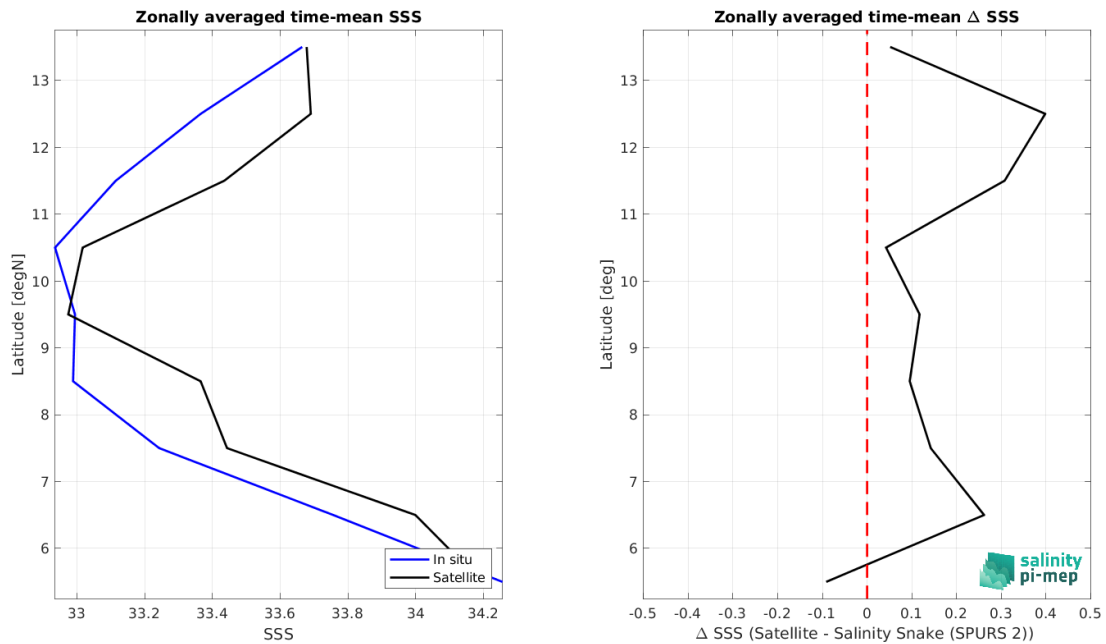
Figure 9: Left panel: Zonal mean SSS from SMAP SSS L2 v6 - 40 km (RSS) satellite product (black) and from Salinity Snake (SPURS 2) (blue). Right panel: Zonal mean of \Delta SSS (Satellite - Salinity Snake (SPURS 2)) for all the collected Pi-MEP match-up pairs estimated over the full satellite product period.
