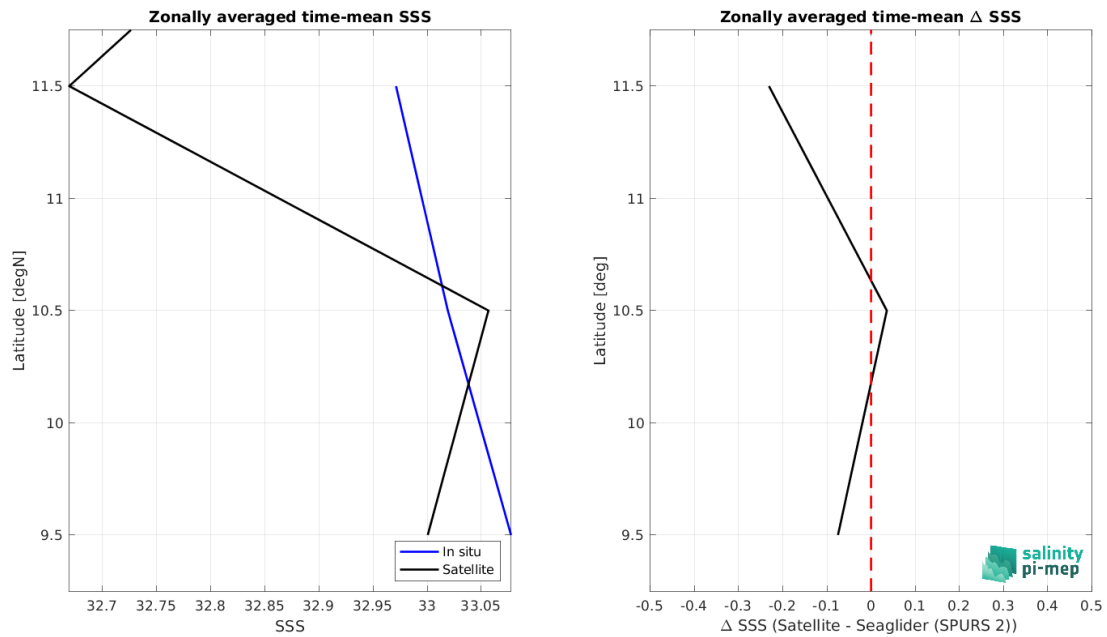
Figure 9: Left panel: Zonal mean SSS from SMAP SSS L2 v6 - 40 km (RSS) satellite product (black) and from Seaglider (SPURS 2) (blue). Right panel: Zonal mean of \Delta SSS (Satellite - Seaglider (SPURS 2)) for all the collected Pi-MEP match-up pairs estimated over the full satellite product period.
