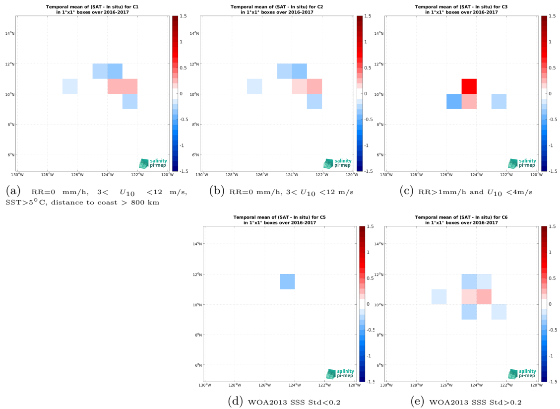
Figure 14: Temporal mean gridded over spatial boxes of size 1^\circ \times 1^\circ of \Delta\text{SSS} (SMAP SSS L2 v6 - 40 km (RSS) - Seaglider (SPURS 2)) for 5 different subdatasets corresponding to:RR=0 mm/h, 3 < U_{10} < 12 m/s, SST>5°C, distance to coast > 800 km (a), RR=0 mm/h, 3 < U_{10} < 12 m/s (b), RR>1mm/h and U_{10} < 4 m/s (c), WOA2013 SSS Std<0.2 (d), WOA2013 SSS Std>0.2 (e).
