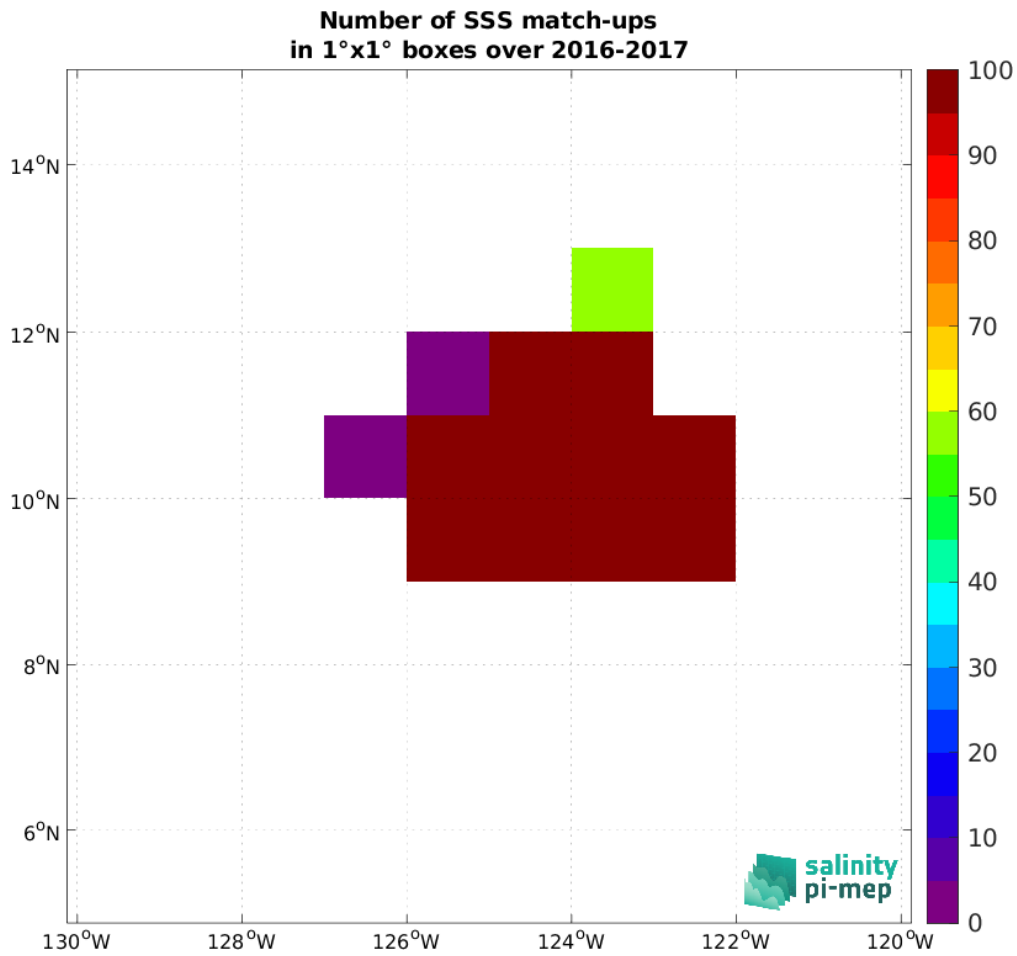
Figure 5: Number of SSS match-ups between Seagliders (SPURS 2) SSS and the SMAP SSS L2 v6 - 40 km (RSS) SSS product for the SPURS 2 Pi-MEP region over 1°x1° boxes and for the full satellite product period.
