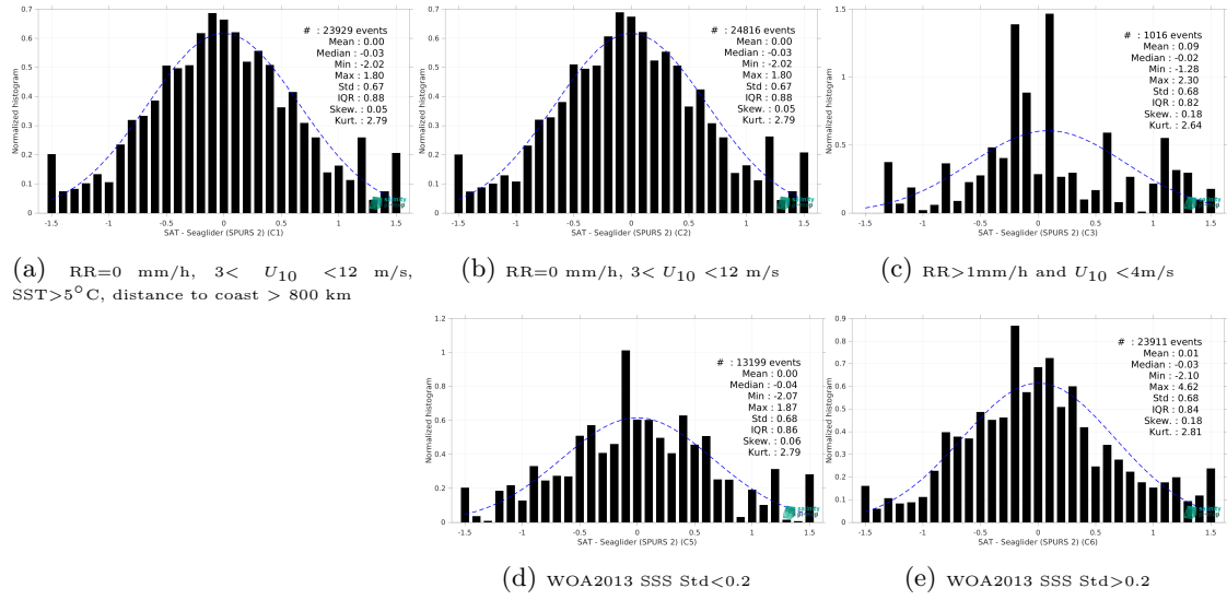
Figure 15: Normalized histogram of \Delta SSS (SMAP SSS L2 v6 - 40 km (RSS) - Seaglider (SPURS 2)) for 5 different subdatasets corresponding to: RR=0 mm/h, 3 < U_{10} < 12 m/s, SST>5°C, distance to coast > 800 km (a), RR=0 mm/h, 3 < U_{10} < 12 m/s (b), RR>1mm/h and U_{10} < 4 m/s (c), WOA2013 SSS Std<0.2 (d), WOA2013 SSS Std>0.2 (e).
