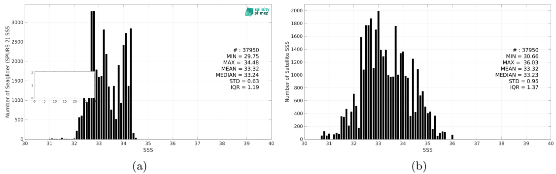
Figure 3: Histograms of SSS from Seaglider (SPURS 2) (a) and SMAP SSS L2 v6 - 40 km (RSS) (b) considering all match-up pairs per bins of 0.1 over the SPURS 2 Pi-MEP region and for the full satellite product period.
