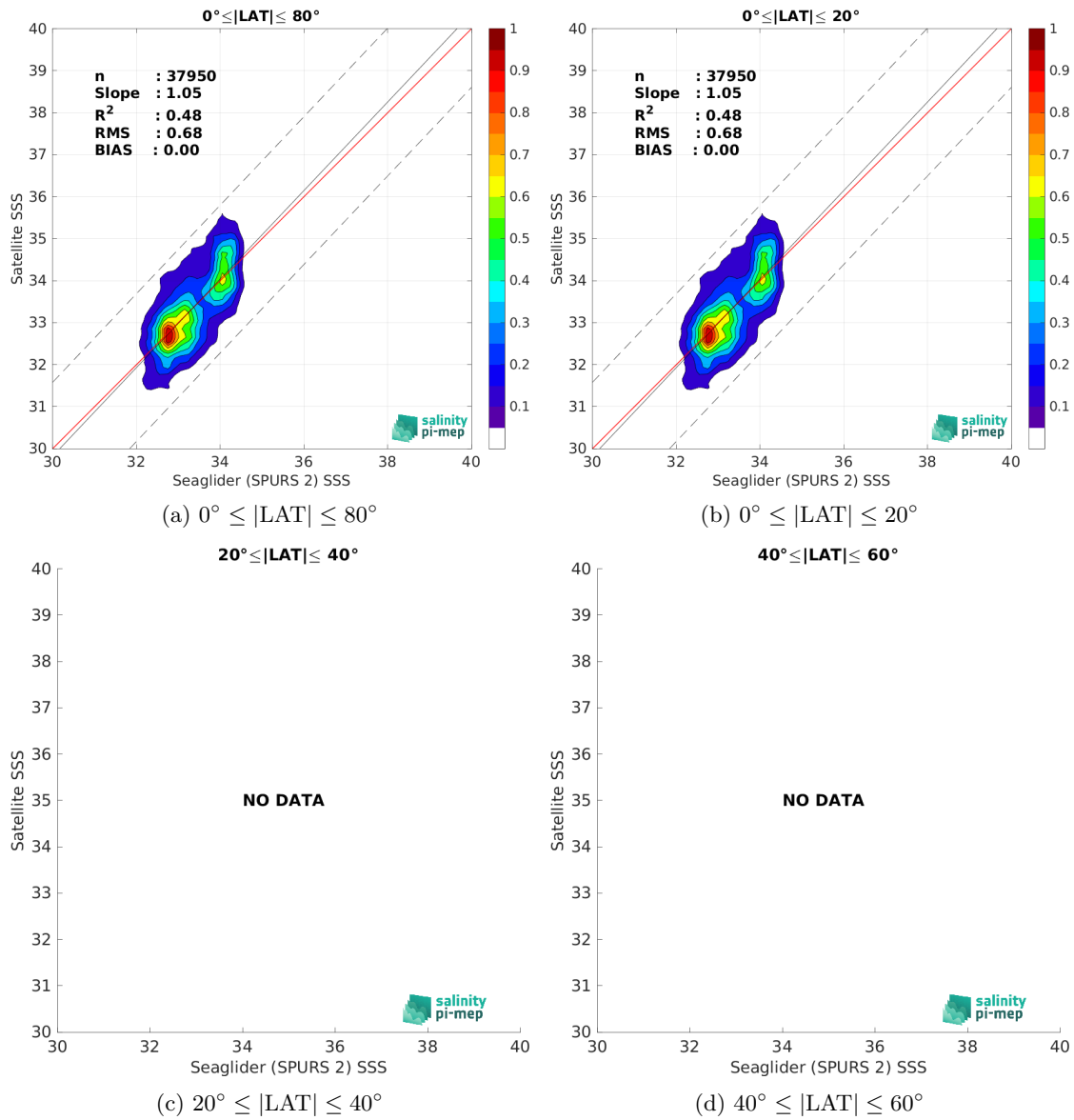
Figure 10: Contour maps of the concentration of SMAP SSS L2 v6 - 40 km (RSS) SSS (y-axis) versus Seaglider (SPURS 2) SSS (x-axis) at match-up pairs for different latitude bands. For each plot, the red line shows x=y . The black thin and dashed lines indicate a linear fit through the data cloud and the \pm 95\% confidence levels, respectively. The number match-up pairs n , the slope and R^2 coefficient of the linear fit, the root mean square (RMS) and the mean bias between satellite and in situ data are indicated for each latitude band in each plots.
