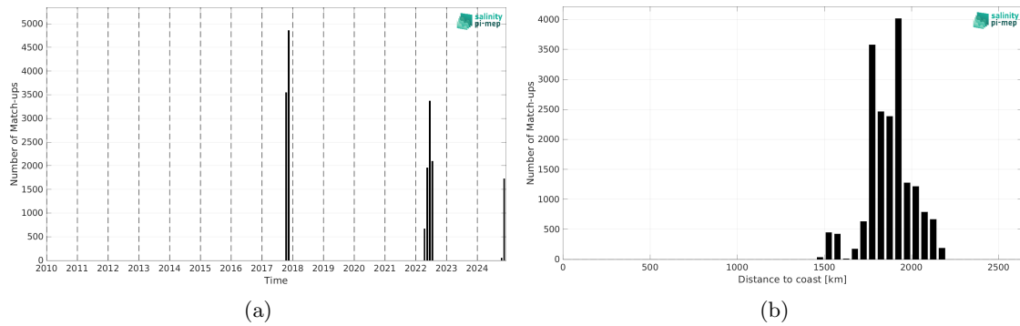
Figure 2: Number of match-ups between Sairdrone and SMAP SSS L2 v6 - 40 km (RSS) SSS as a function of time (a) and as function of the distance to coast (b) over the SPURS 2 Pi-MEP region and for the full satellite product period.
