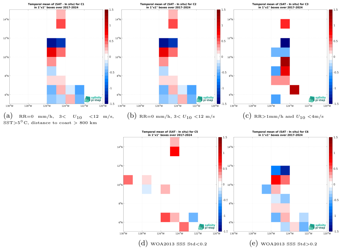
Figure 14: Temporal mean gridded over spatial boxes of size 1^\circ \times 1^\circ of \Delta SSS (SMAP SSS L2 v6 - 40 km (RSS) - Saldrone) for 5 different subdatasets corresponding to:RR=0 mm/h, 3 < U_{10} < 12 m/s, SST>5°C, distance to coast > 800 km (a), RR=0 mm/h, 3 < U_{10} < 12 m/s (b), RR>1mm/h and U_{10} < 4 m/s (c), WOA2013 SSS Std<0.2 (d), WOA2013 SSS Std>0.2 (e).
