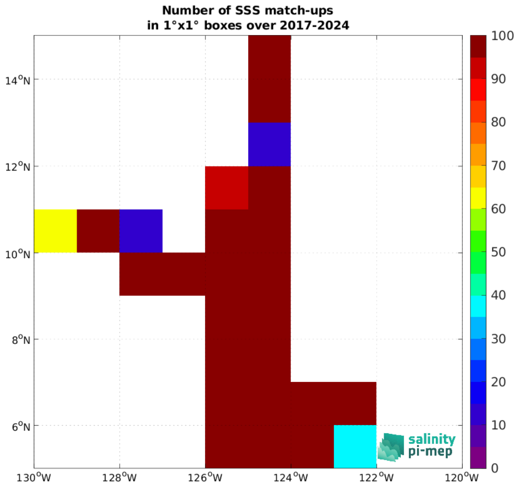
Figure 5: Number of SSS match-ups between Saildrone SSS and the SMAP SSS L2 v6 - 40 km (RSS) SSS product for the SPURS 2 Pi-MEP region over 1^\circ \times 1^\circ boxes and for the full satellite product period.
