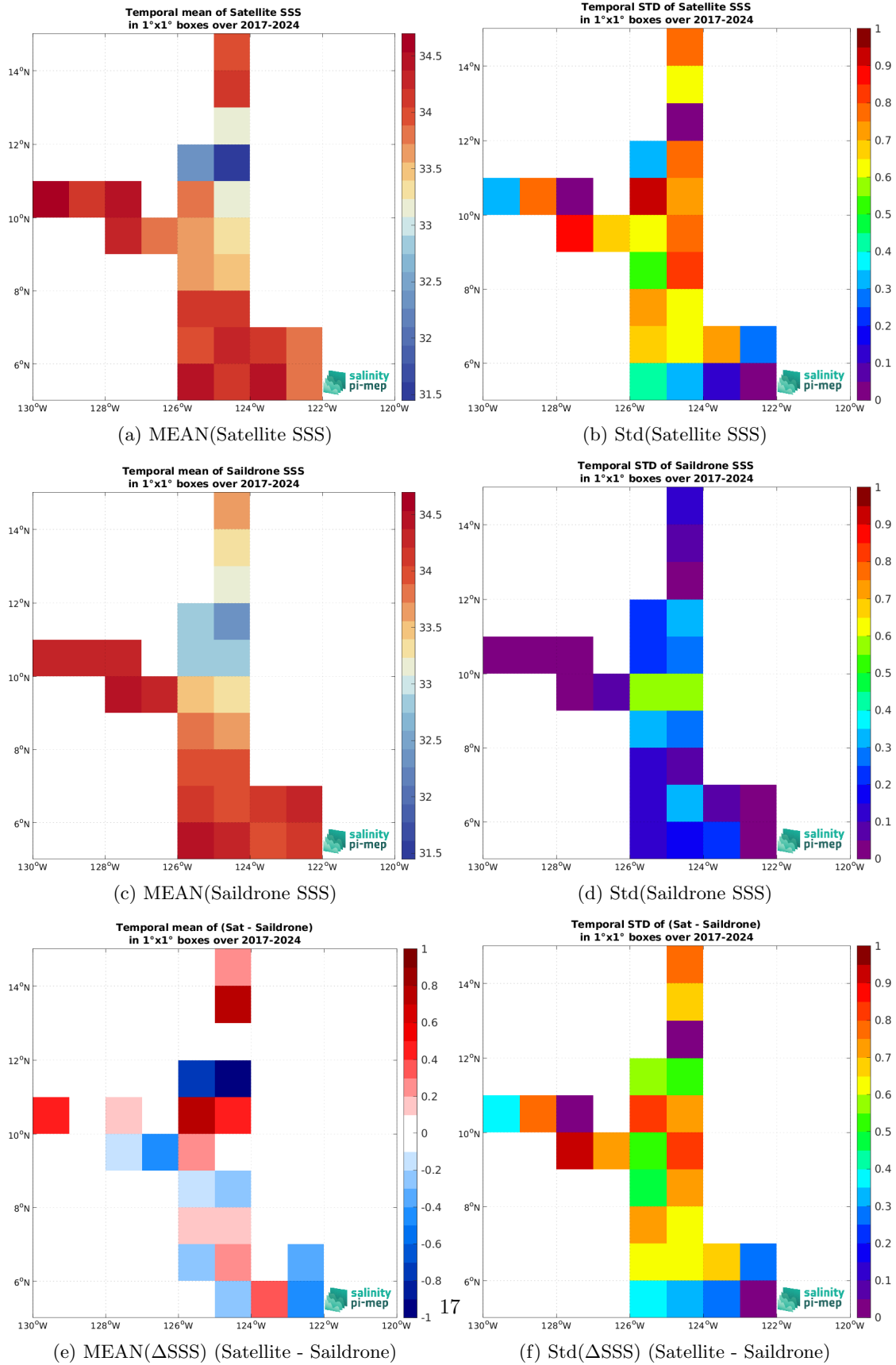
Figure 7: Temporal mean (left) and Std (right) of SSS from SMAP SSS L2 v6 - 40 km (RSS) (top), Saildrone (middle), and of \Delta SSS (Satellite - Saildrone). Only match-up pairs are used to generate these maps.
