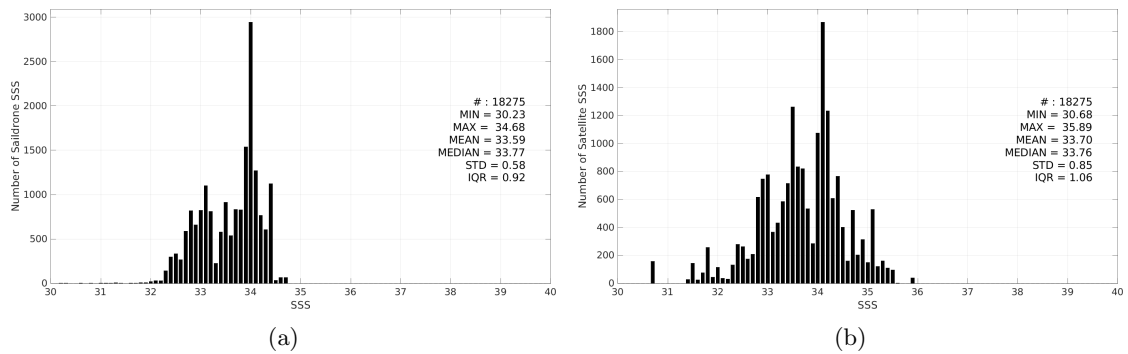
Figure 3: Histograms of SSS from Sairdrone (a) and SMAP SSS L2 v6 - 40 km (RSS) (b) considering all match-up pairs per bins of 0.1 over the SPURS 2 Pi-MEP region and for the full satellite product period.
