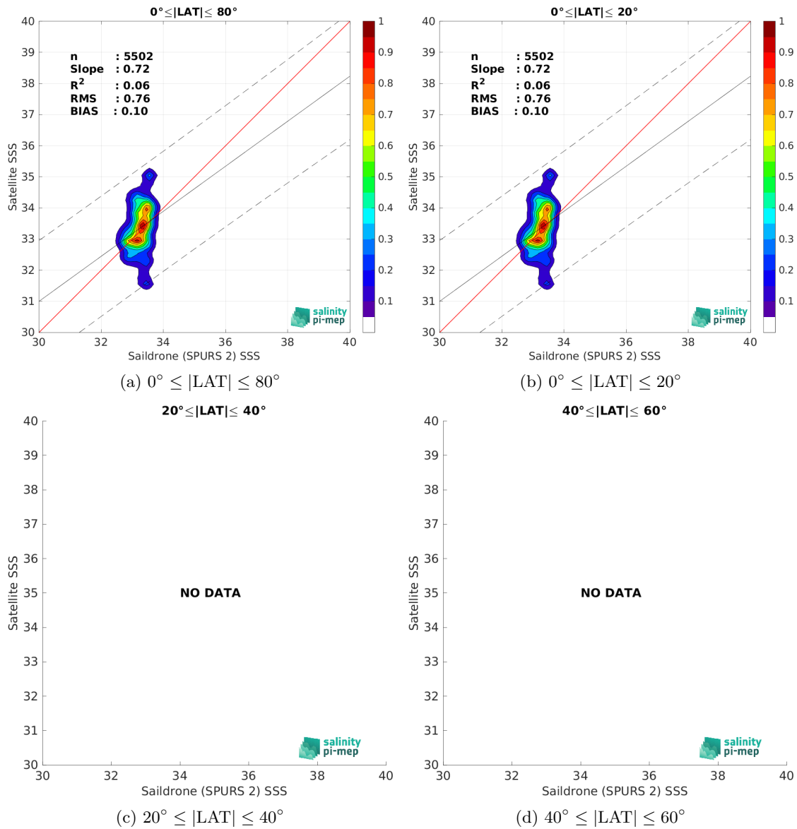
Figure 10: Contour maps of the concentration of SMAP SSS L2 v6 - 40 km (RSS) SSS (y-axis) versus Saildrone (SPURS 2) SSS (x-axis) at match-up pairs for different latitude bands. For each plot, the red line shows x=y . The black thin and dashed lines indicate a linear fit through the data cloud and the \pm 95\% confidence levels, respectively. The number match-up pairs n , the slope and R^2 coefficient of the linear fit, the root mean square (RMS) and the mean bias between satellite and in situ data are indicated for each latitude band in each plots.
