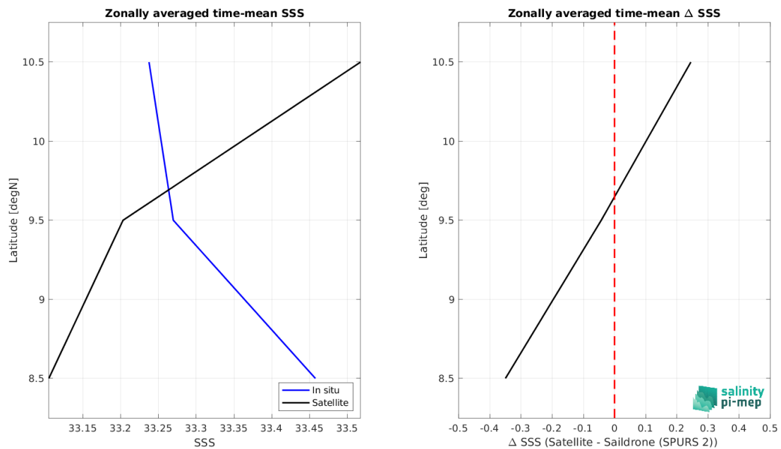
Figure 9: Left panel: Zonal mean SSS from SMAP SSS L2 v6 - 40 km (RSS) satellite product (black) and from Sairdrone (SPURS 2) (blue). Right panel: Zonal mean of \Delta SSS (Satellite - Sairdrone (SPURS 2)) for all the collected Pi-MEP match-up pairs estimated over the full satellite product period.
