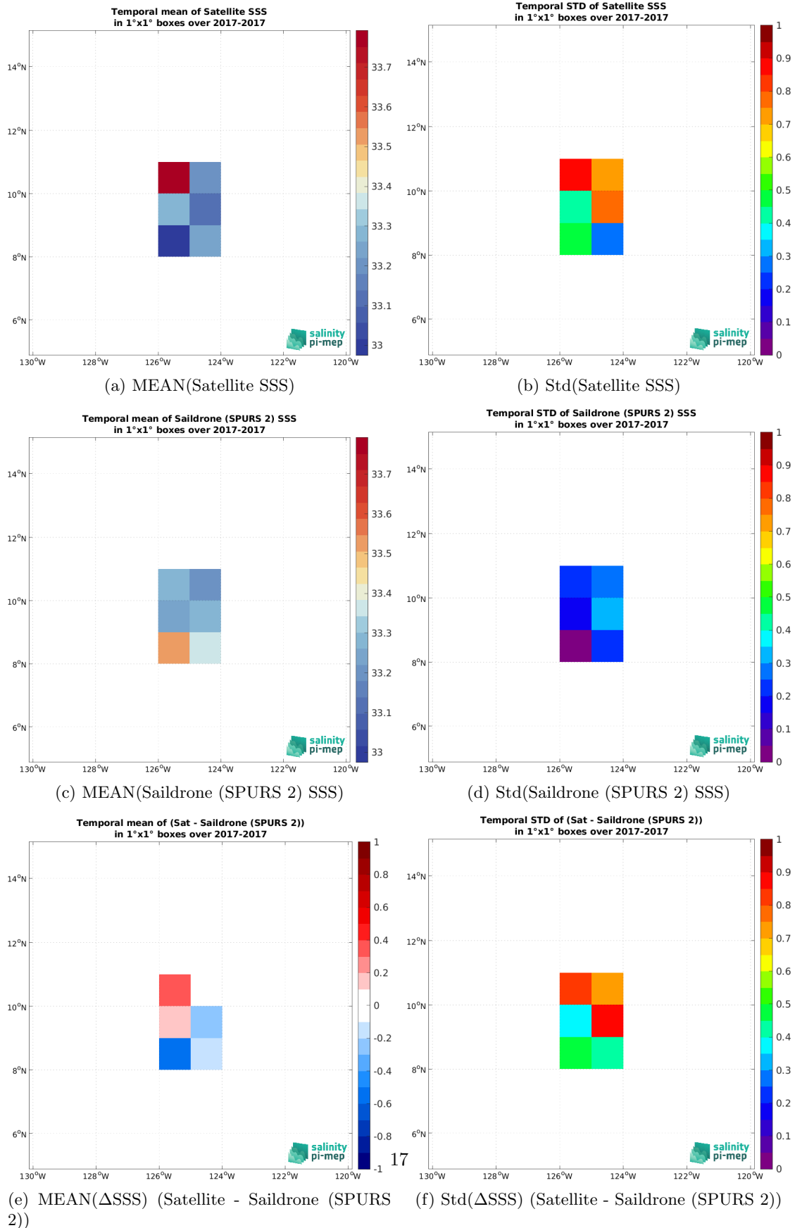
Figure 7: Temporal mean (left) and Std (right) of SSS from SMAP SSS L2 v6 - 40 km (RSS) (top), Saildrone (SPURS 2) (middle), and of \Delta SSS (Satellite - Saildrone (SPURS 2)). Only match-up pairs are used to generate these maps.
