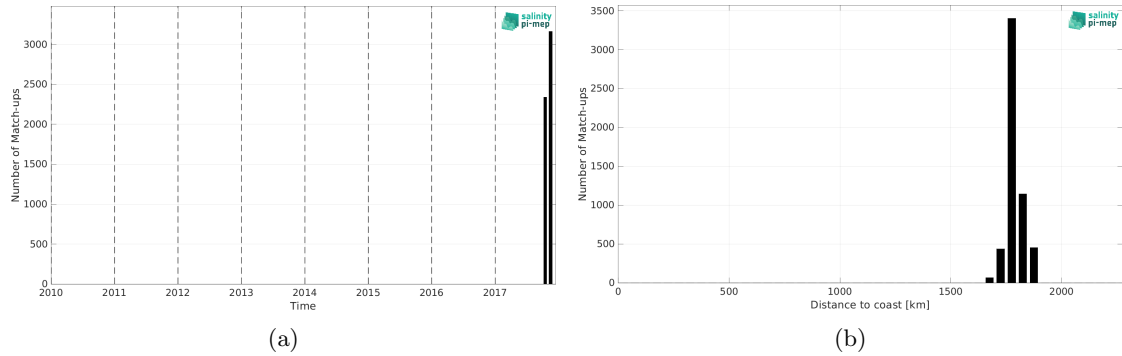
Figure 2: Number of match-ups between Saildrone (SPURS 2) and SMAP SSS L2 v6 - 40 km (RSS) SSS as a function of time (a) and as function of the distance to coast (b) over the SPURS 2 Pi-MEP region and for the full satellite product period.
