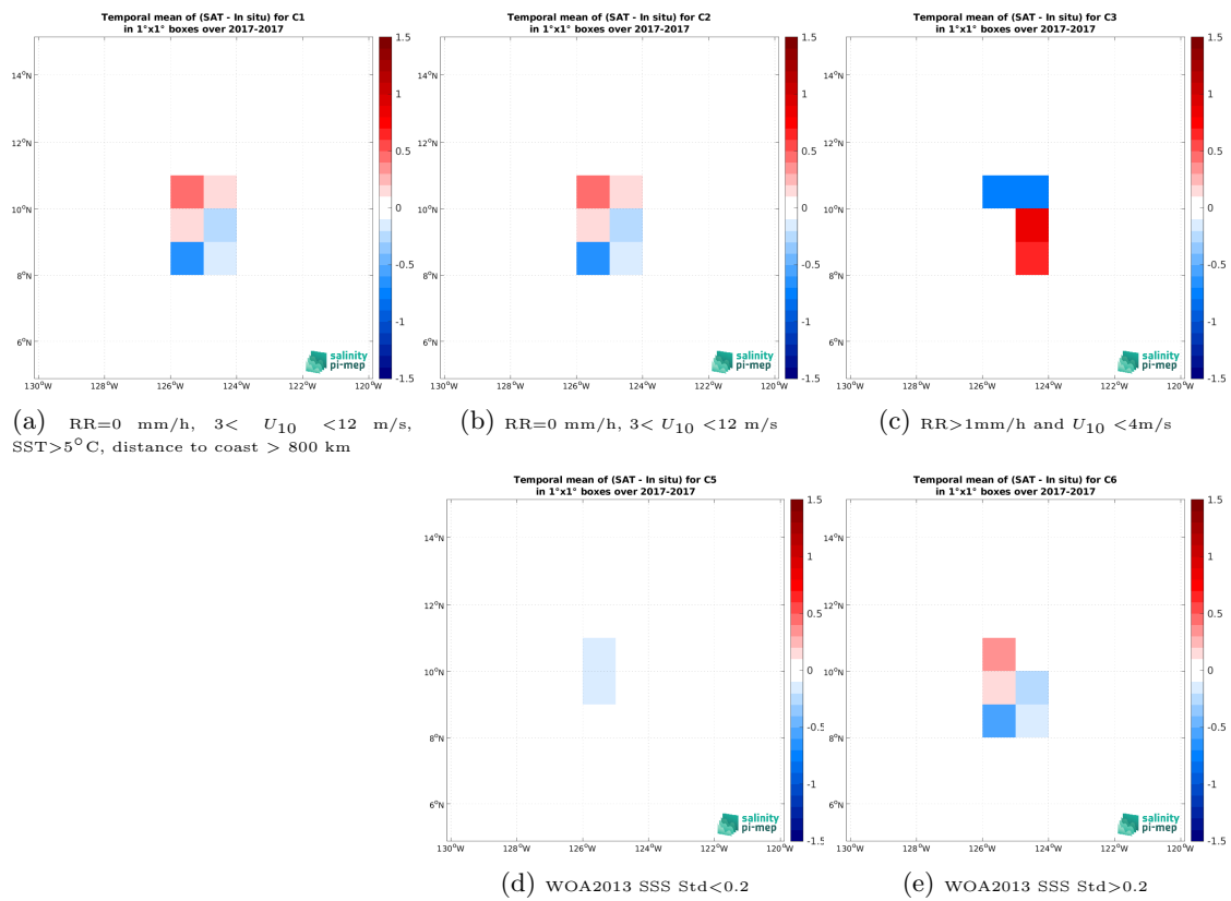
Figure 14: Temporal mean gridded over spatial boxes of size 1^\circ \times 1^\circ of \Delta SSS (SMAP SSS L2 v6 - 40 km (RSS) - Saildrone (SPURS 2)) for 5 different subdatasets corresponding to:RR=0 mm/h, 3 < U_{10} < 12 m/s, SST >5^\circ\text{C} , distance to coast > 800 km (a), RR=0 mm/h, 3 < U_{10} < 12 m/s (b), RR >1 mm/h and U_{10} < 4 m/s (c), WOA2013 SSS Std <0.2 (d), WOA2013 SSS Std >0.2 (e).
