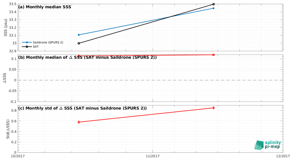
Figure 8: Time series of the monthly median SSS (top), median of \Delta SSS (Satellite - Sairdron (SPURS 2)) and Std of \Delta SSS (Satellite - Sairdron (SPURS 2)) over the SPURS 2 Pi-MEP region considering all match-ups collected by the Pi-MEP.
