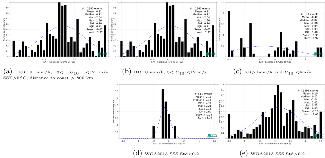
Figure 15: Normalized histogram of \Delta SSS (SMAP SSS L2 v6 - 40 km (RSS) - Saildrone (SPURS 2)) for 5 different subdatasets corresponding to: RR=0 mm/h, 3 < U_{10} < 12 m/s, SST > 5°C, distance to coast > 800 km (a), RR=0 mm/h, 3 < U_{10} < 12 m/s (b), RR > 1mm/h and U_{10} < 4 m/s (c), WOA2013 SSS Std < 0.2 (d), WOA2013 SSS Std > 0.2 (e).
