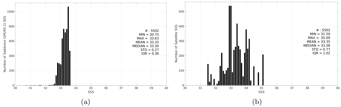
Figure 3: Histograms of SSS from Saildrone (SPURS 2) (a) and SMAP SSS L2 v6 - 40 km (RSS) (b) considering all match-up pairs per bins of 0.1 over the SPURS 2 Pi-MEP region and for the full satellite product period.
