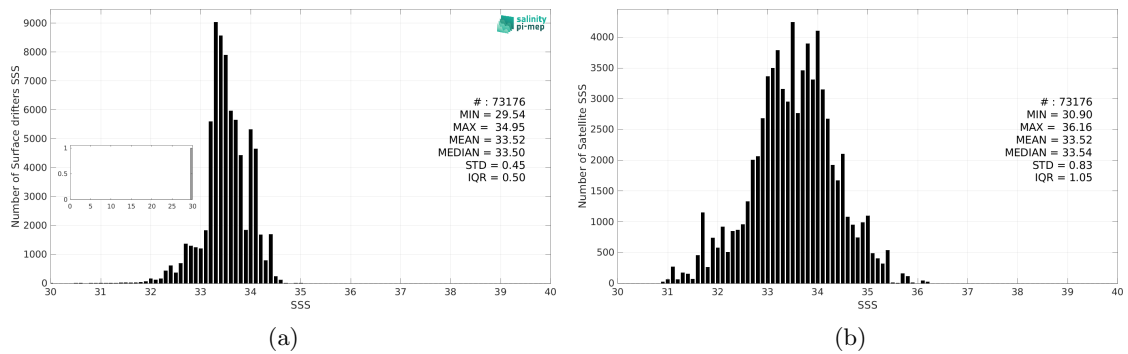
Figure 3: Histograms of SSS from Surface drifters (a) and SMAP SSS L2 v6 - 40 km (RSS) (b) considering all match-up pairs per bins of 0.1 over the SPURS 2 Pi-MEP region and for the full satellite product period.
