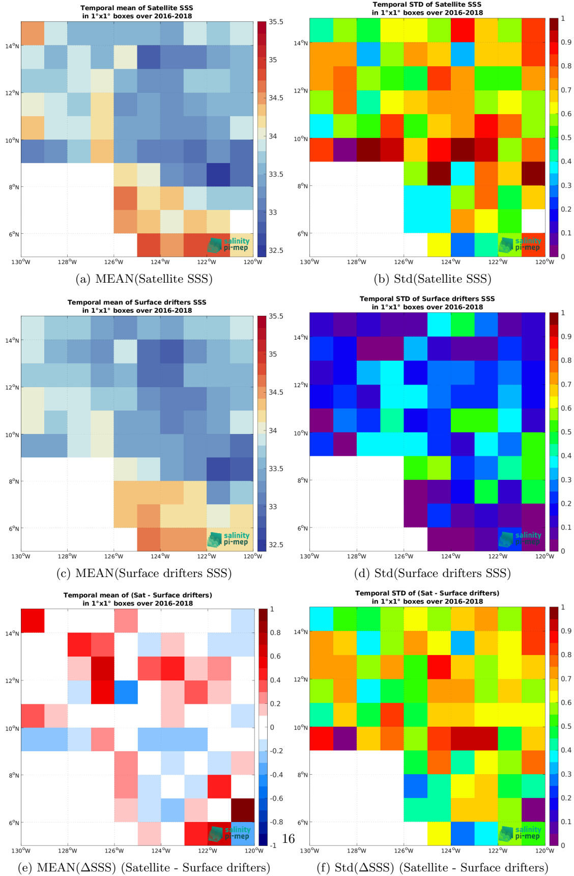
Figure 6: Temporal mean (left) and Std (right) of SSS from SMAP SSS L2 v6 - 40 km (RSS) (top), Surface drifters (middle), and of \Delta SSS (Satellite - Surface drifters). Only match-up pairs are used to generate these maps.
