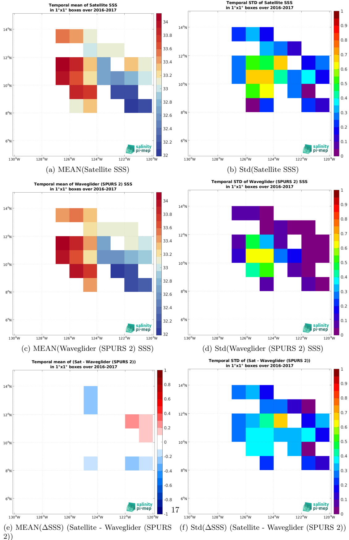
Figure 6: Temporal mean (left) and Std (right) of SSS from SMAP SSS L2 v5 (RSS) (top), Waveglider (SPURS 2) (middle), and of \Delta SSS (Satellite - Waveglider (SPURS 2)). Only match-up pairs are used to generate these maps.
