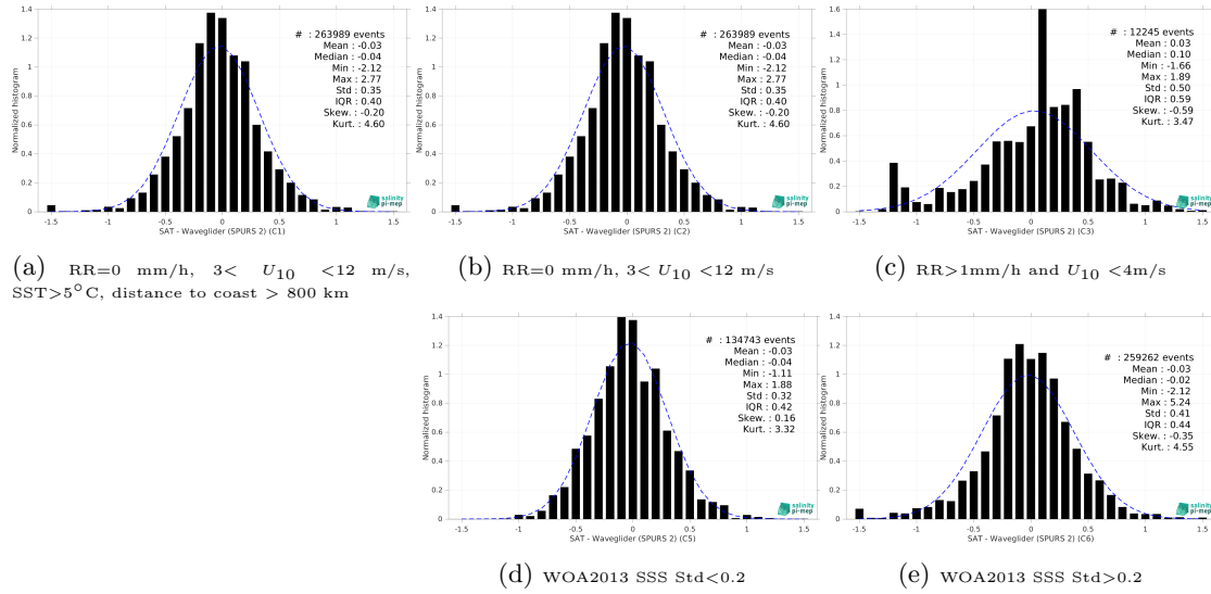
Figure 13: Normalized histogram of \Delta SSS (SMAP SSS L2 v5 (RSS) - Waveglider (SPURS 2)) for 5 different subdatasets corresponding to: RR=0 mm/h, 3 < U_{10} < 12 m/s, SST > 5°C, distance to coast > 800 km (a), RR=0 mm/h, 3 < U_{10} < 12 m/s (b), RR > 1mm/h and U_{10} < 4 m/s (c), WOA2013 SSS Std < 0.2 (d), WOA2013 SSS Std > 0.2 (e).
