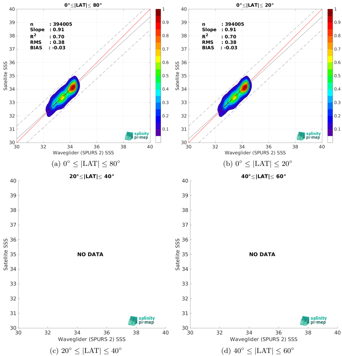
Figure 9: Contour maps of the concentration of SMAP SSS L2 v5 (RSS) SSS (y-axis) versus Waveglider (SPURS 2) SSS (x-axis) at match-up pairs for different latitude bands. For each plot, the red line shows x=y . The black thin and dashed lines indicate a linear fit through the data cloud and the \pm 95\% confidence levels, respectively. The number match-up pairs n , the slope and R^2 coefficient of the linear fit, the root mean square (RMS) and the mean bias between satellite and in situ data are indicated for each latitude band in each plots.
