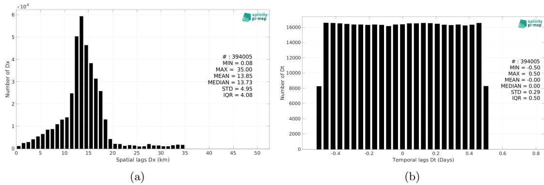
Figure 5: Histograms of the spatial (a) and temporal (b) lags between the location/time of the Waveglider (SPURS 2) measurement and the date of the corresponding SMAP SSS L2 v5 (RSS) SSS pixel.
