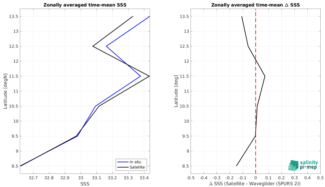
Figure 8: Left panel: Zonal mean SSS from SMAP SSS L2 v5 (RSS) satellite product (black) and from Waveglider (SPURS 2) (blue). Right panel: Zonal mean of \Delta SSS (Satellite - Waveglider (SPURS 2)) for all the collected Pi-MEP match-up pairs estimated over the full satellite product period.
