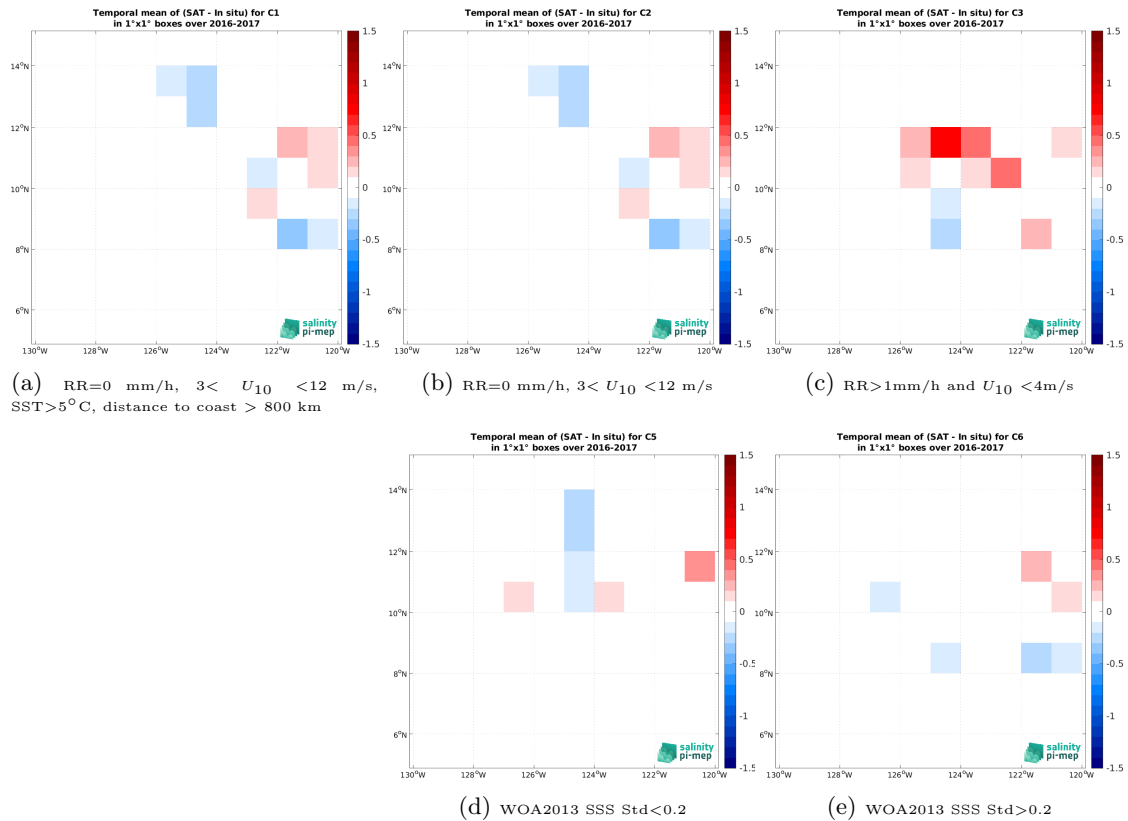
Figure 12: Temporal mean gridded over spatial boxes of size 1^\circ \times 1^\circ of \Delta SSS (SMAP SSS L2 v5 (RSS) - Waveglider (SPURS 2)) for 5 different subdatasets corresponding to:RR=0 mm/h, 3 < U_{10} < 12 m/s, SST > 5^\circ C , distance to coast > 800 km (a), RR=0 mm/h, 3 < U_{10} < 12 m/s (b), RR >1 mm/h and U_{10} < 4 m/s (c), WOA2013 SSS Std <0.2 (d), WOA2013 SSS Std >0.2 (e).
