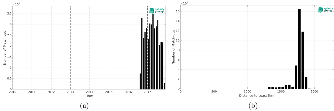
Figure 1: Number of match-ups between Waveglider (SPURS 2) and SMAP SSS L2 v5 (RSS) SSS as a function of time (a) and as function of the distance to coast (b) over the SPURS 2 Pi-MEP region and for the full satellite product period.
