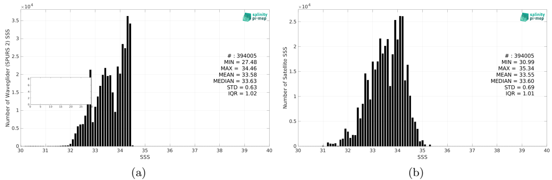
Figure 2: Histograms of SSS from Waveglider (SPURS 2) (a) and SMAP SSS L2 v5 (RSS) (b) considering all match-up pairs per bins of 0.1 over the SPURS 2 Pi-MEP region and for the full satellite product period.
