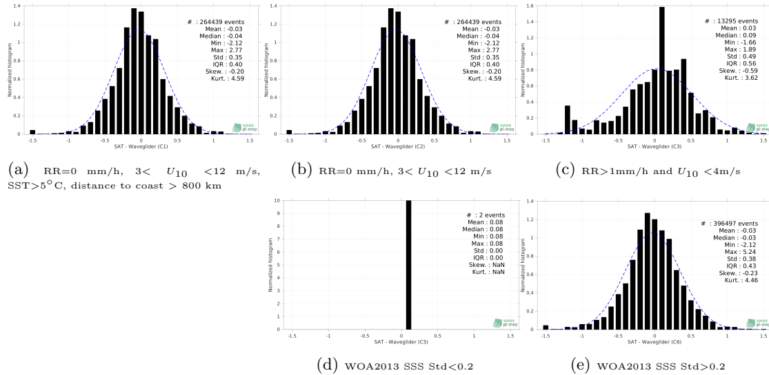
Figure 12: Normalized histogram of \Delta SSS (SMAP SSS L2 v5 (RSS) - Waveglider) for 5 different subdatasets corresponding to: RR=0 mm/h, 3 < U_{10} < 12 m/s, SST > 5°C, distance to coast > 800 km (a), RR=0 mm/h, 3 < U_{10} < 12 m/s (b), RR > 1mm/h and U_{10} < 4 m/s (c), WOA2013 SSS Std < 0.2 (d), WOA2013 SSS Std > 0.2 (e).
