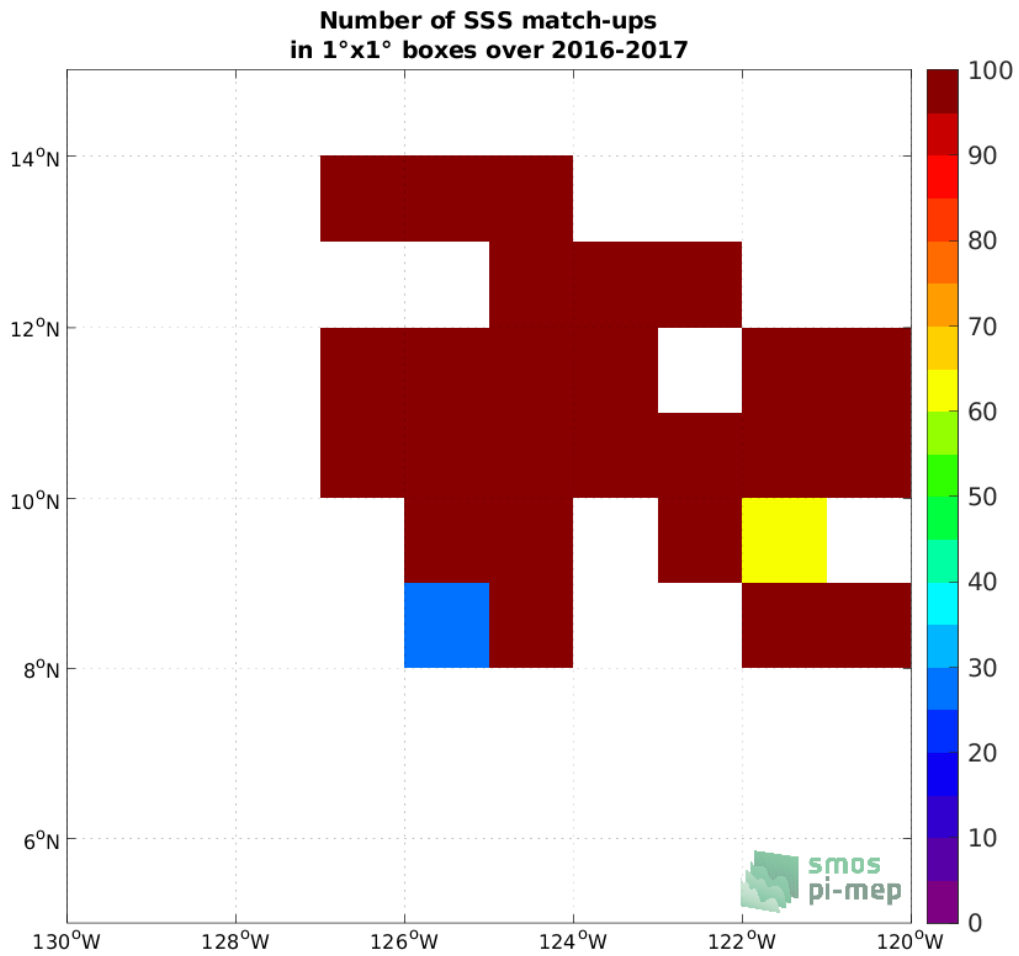
Figure 3: Number of SSS match-ups between Waveglider SSS and the SMAP SSS L2 v5 (RSS) SSS product for the SPURS 2 Pi-MEP region over 1°x1° boxes and for the full satellite product period.
