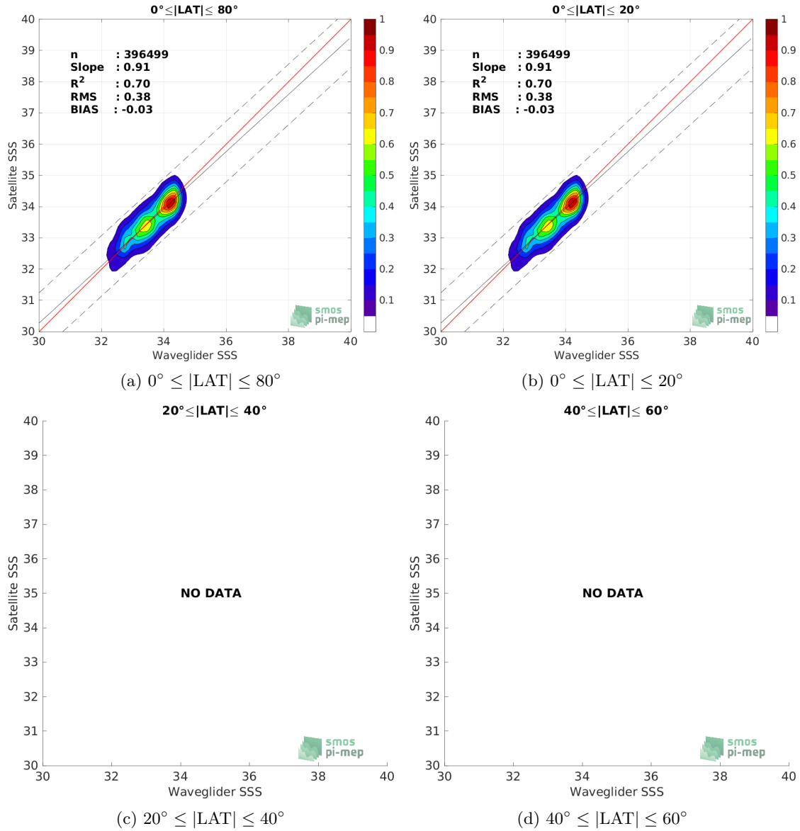
Figure 8: Contour maps of the concentration of SMAP SSS L2 v5 (RSS) SSS (y-axis) versus Waveglider SSS (x-axis) at match-up pairs for different latitude bands. For each plot, the red line shows x=y . The black thin and dashed lines indicate a linear fit through the data cloud and the \pm 95\% confidence levels, respectively. The number match-up pairs n , the slope and R^2 coefficient of the linear fit, the root mean square (RMS) and the mean bias between satellite and in situ data are indicated for each latitude band in each plots.
