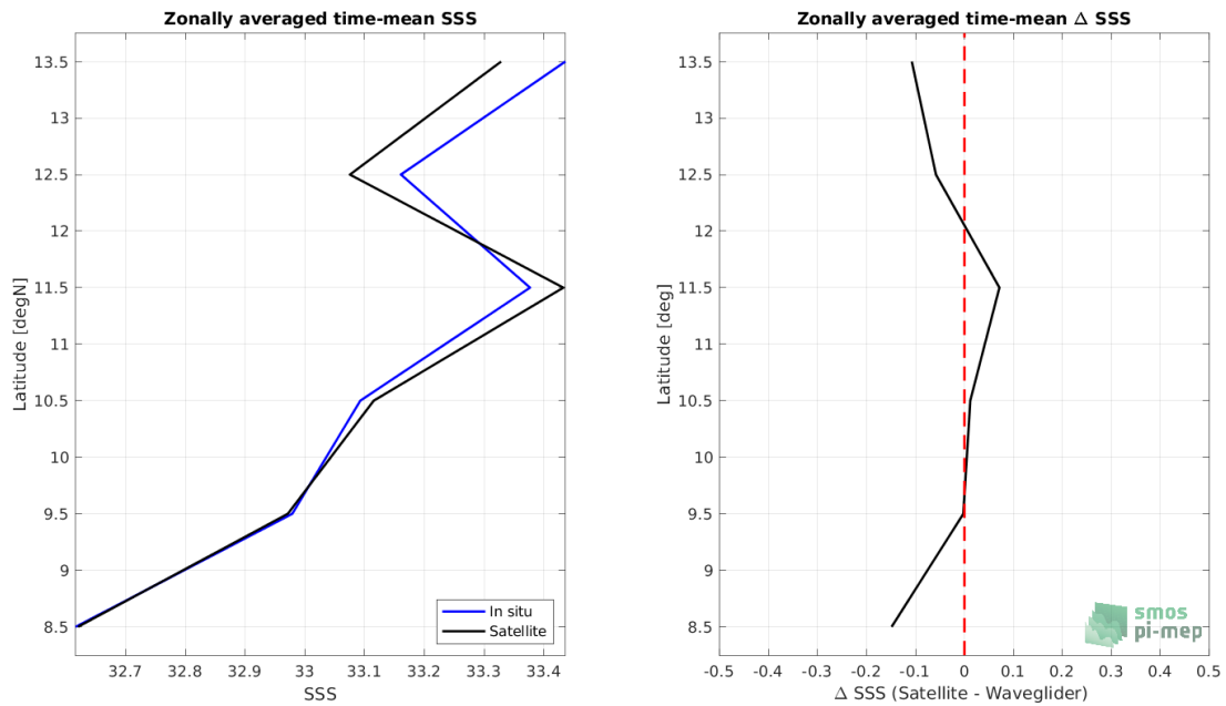
Figure 7: Left panel: Zonal mean SSS from SMAP SSS L2 v5 (RSS) satellite product (black) and from Waveglider (blue). Right panel: Zonal mean of \Delta SSS (Satellite - Waveglider) for all the collected Pi-MEP match-up pairs estimated over the full satellite product period.
