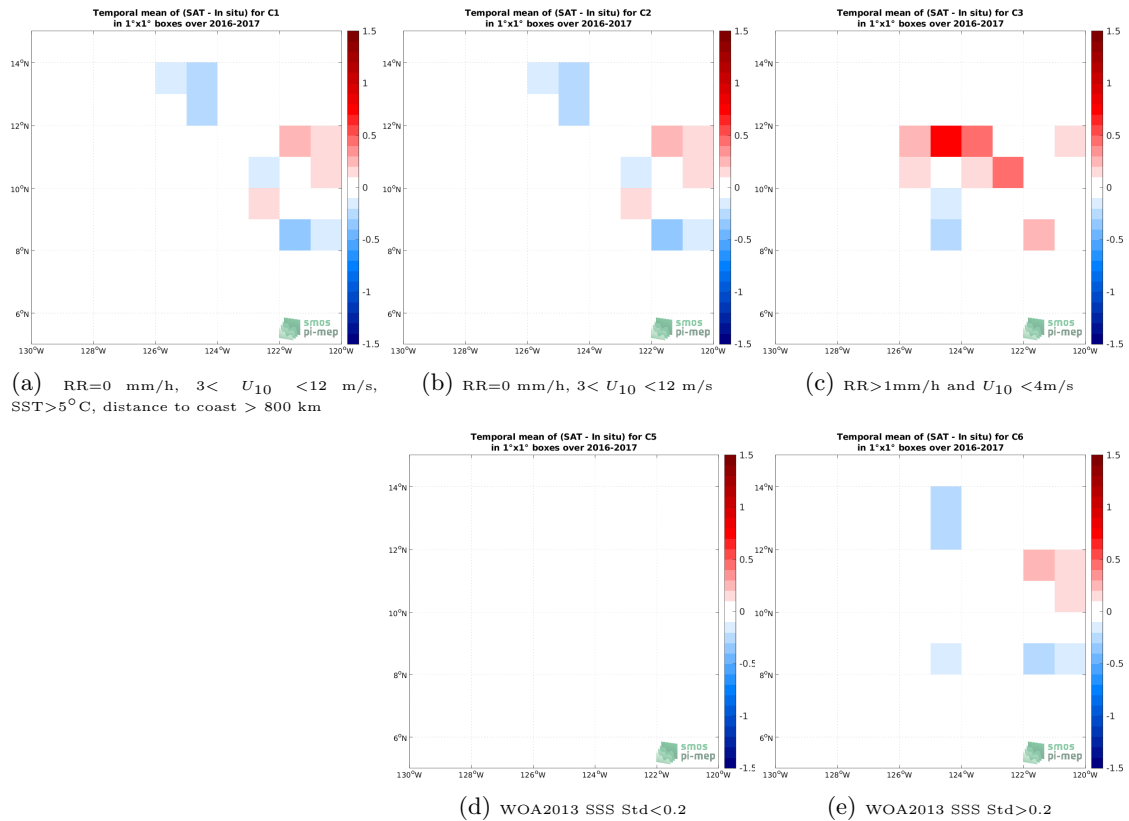
Figure 11: Temporal mean gridded over spatial boxes of size 1^\circ \times 1^\circ of \Delta SSS (SMAP SSS L2 v5 (RSS) - Waveglider) for 5 different subdatasets corresponding to:RR=0 mm/h, 3 < U_{10} < 12 m/s, SST >5^\circ C, distance to coast > 800 km (a), RR=0 mm/h, 3 < U_{10} < 12 m/s (b), RR >1 mm/h and U_{10} < 4 m/s (c), WOA2013 SSS Std <0.2 (d), WOA2013 SSS Std >0.2 (e).
