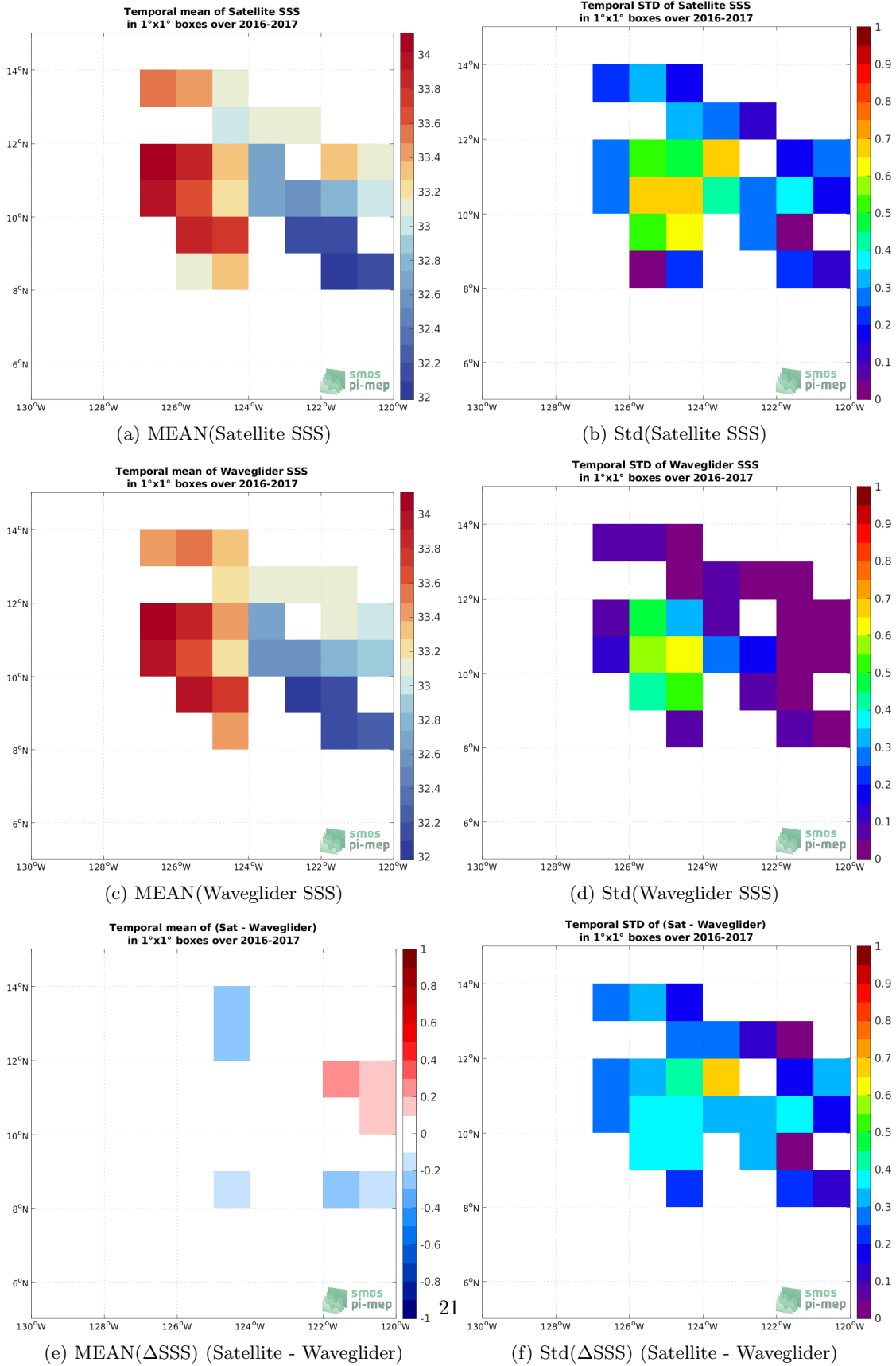
Figure 5: Temporal mean (left) and Std (right) of SSS from SMAP SSS L2 v5 (RSS) (top), Waveglider (middle), and of \Delta SSS (Satellite - Waveglider). Only match-up pairs are used to generate these maps.
