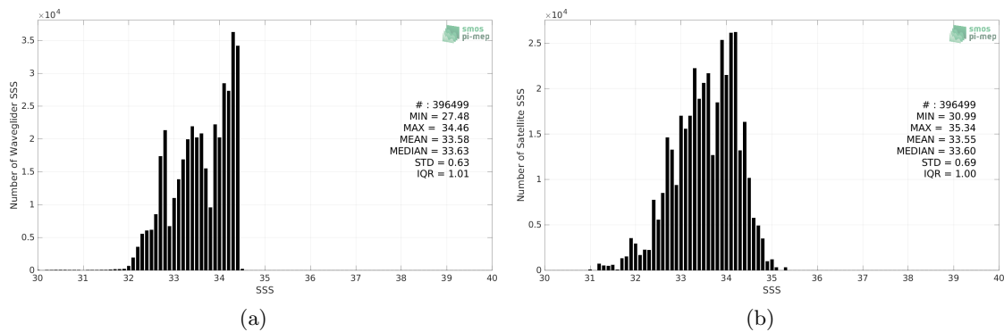
Figure 2: Histograms of SSS from Waveglider (a) and SMAP SSS L2 v5 (RSS) (b) considering all match-up pairs per bins of 0.1 over the SPURS 2 Pi-MEP region and for the full satellite product period.
