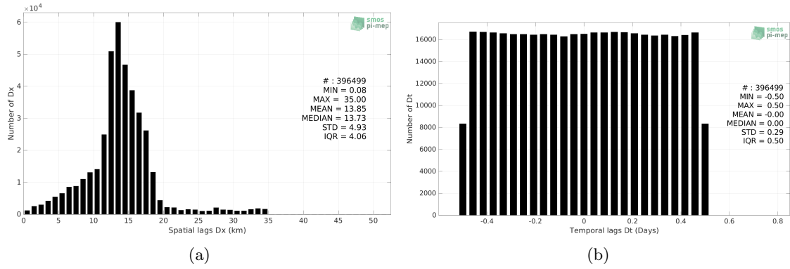
Figure 4: Histograms of the spatial (a) and temporal (b) lags between the location/time of the Waveglider measurement and the date of the corresponding SMAP SSS L2 v5 (RSS) SSS pixel.
