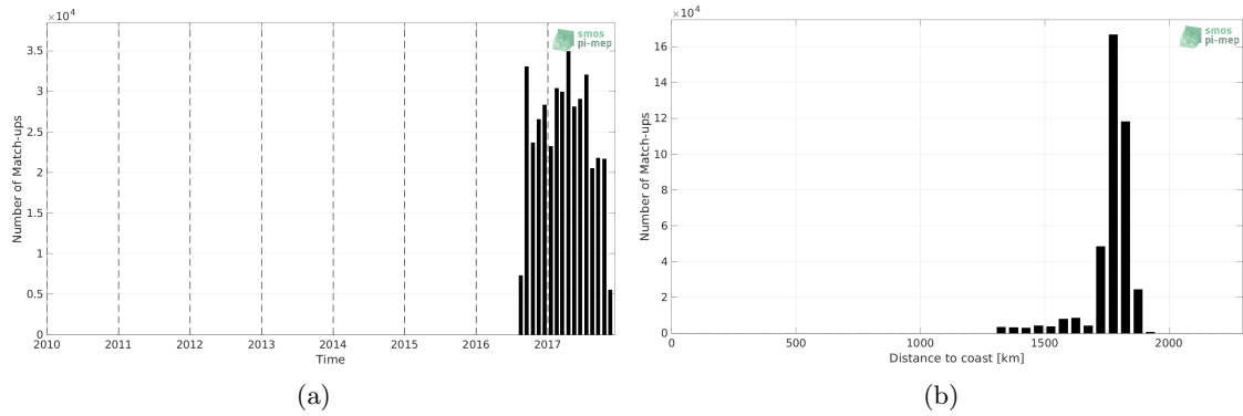
Figure 1: Number of match-ups between Waveglider and SMAP SSS L2 v5 (RSS) SSS as a function of time (a) and as function of the distance to coast (b) over the SPURS 2 Pi-MEP region and for the full satellite product period.
