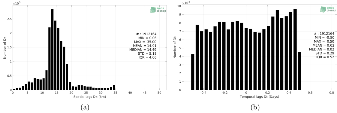
Figure 5: Histograms of the spatial (a) and temporal (b) lags between the location/time of the Salinity Snake measurement and the date of the corresponding SMAP SSS L2 v5 (RSS) SSS pixel.
