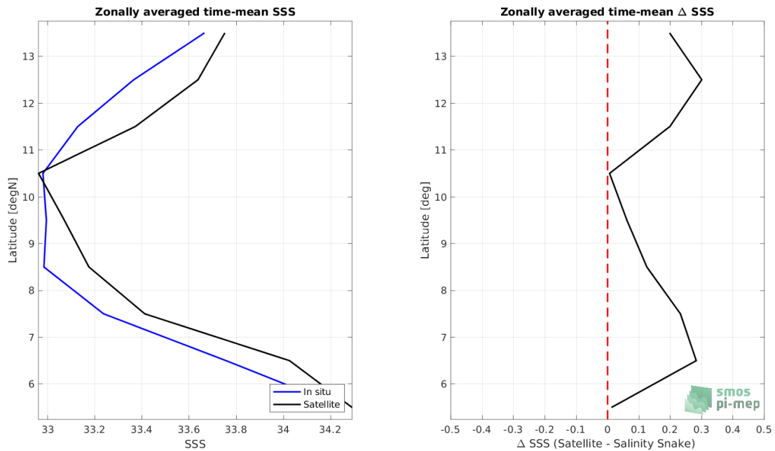
Figure 8: Left panel: Zonal mean SSS from SMAP SSS L2 v5 (RSS) satellite product (black) and from Salinity Snake (blue). Right panel: Zonal mean of \Delta SSS (Satellite - Salinity Snake) for all the collected Pi-MEP match-up pairs estimated over the full satellite product period.
