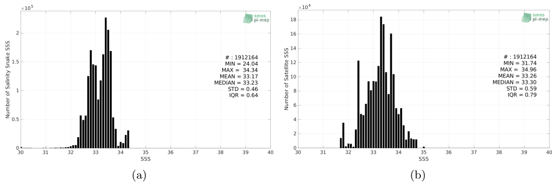
Figure 2: Histograms of SSS from Salinity Snake (a) and SMAP SSS L2 v5 (RSS) (b) considering all match-up pairs per bins of 0.1 over the SPURS 2 Pi-MEP region and for the full satellite product period.
