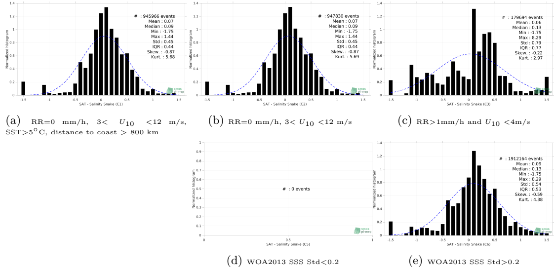
Figure 13: Normalized histogram of \Delta SSS (SMAP SSS L2 v5 (RSS) - Salinity Snake) for 5 different subdatasets corresponding to: RR=0 mm/h, 3 < U_{10} < 12 m/s, SST > 5°C, distance to coast > 800 km (a), RR=0 mm/h, 3 < U_{10} < 12 m/s (b), RR > 1mm/h and U_{10} < 4 m/s (c), WOA2013 SSS Std < 0.2 (d), WOA2013 SSS Std > 0.2 (e).
