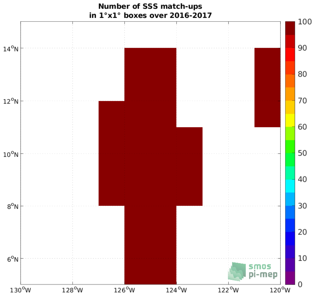
Figure 4: Number of SSS match-ups between Salinity Snake SSS and the SMAP SSS L2 v5 (RSS) SSS product for the SPURS 2 Pi-MEP region over 1°x1° boxes and for the full satellite product period.
