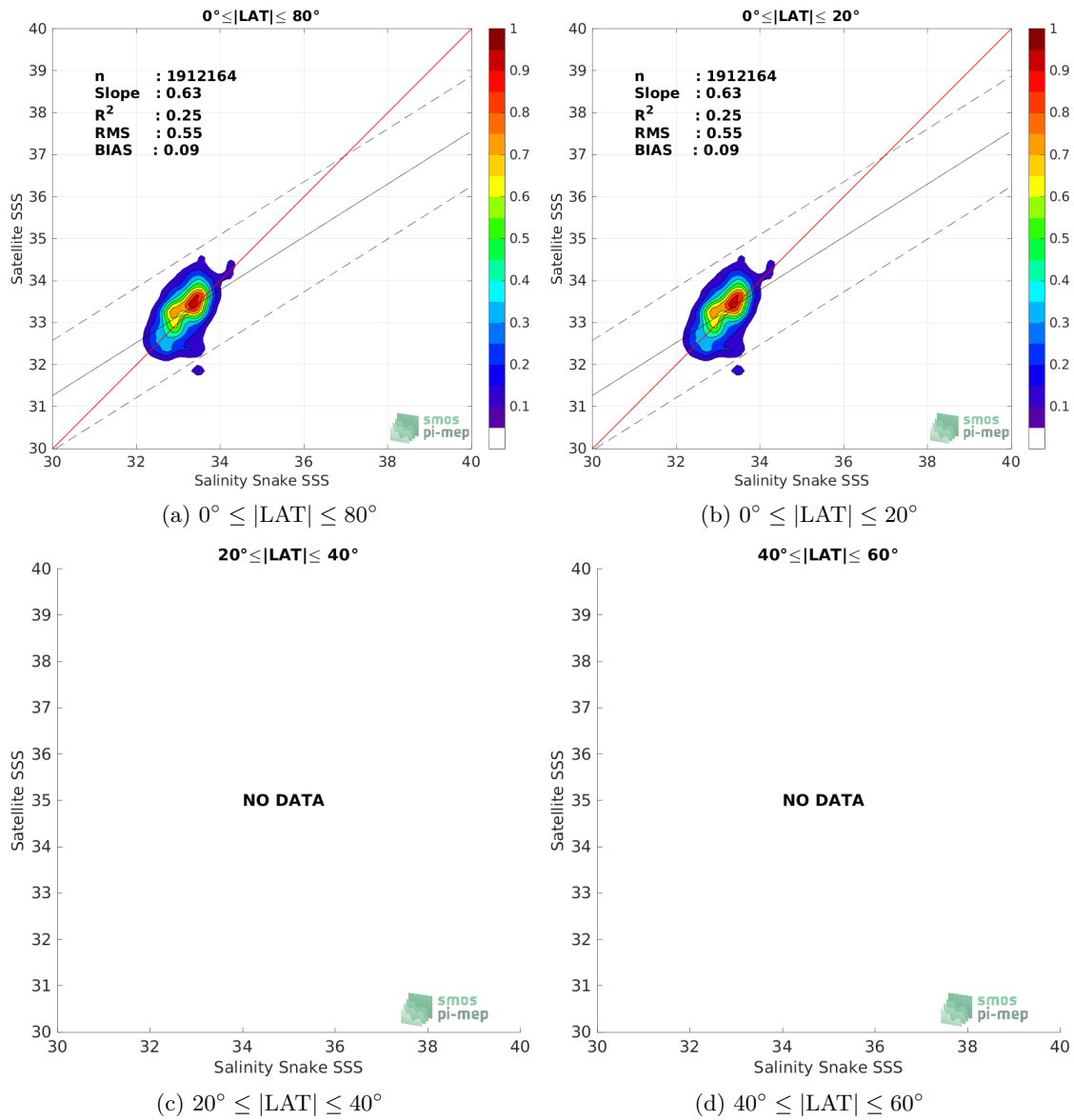
Figure 9: Contour maps of the concentration of SMAP SSS L2 v5 (RSS) SSS (y-axis) versus Salinity Snake SSS (x-axis) at match-up pairs for different latitude bands. For each plot, the red line shows x=y . The black thin and dashed lines indicate a linear fit through the data cloud and the \pm 95\% confidence levels, respectively. The number match-up pairs n , the slope and R^2 coefficient of the linear fit, the root mean square (RMS) and the mean bias between satellite and in situ data are indicated for each latitude band in each plots.
