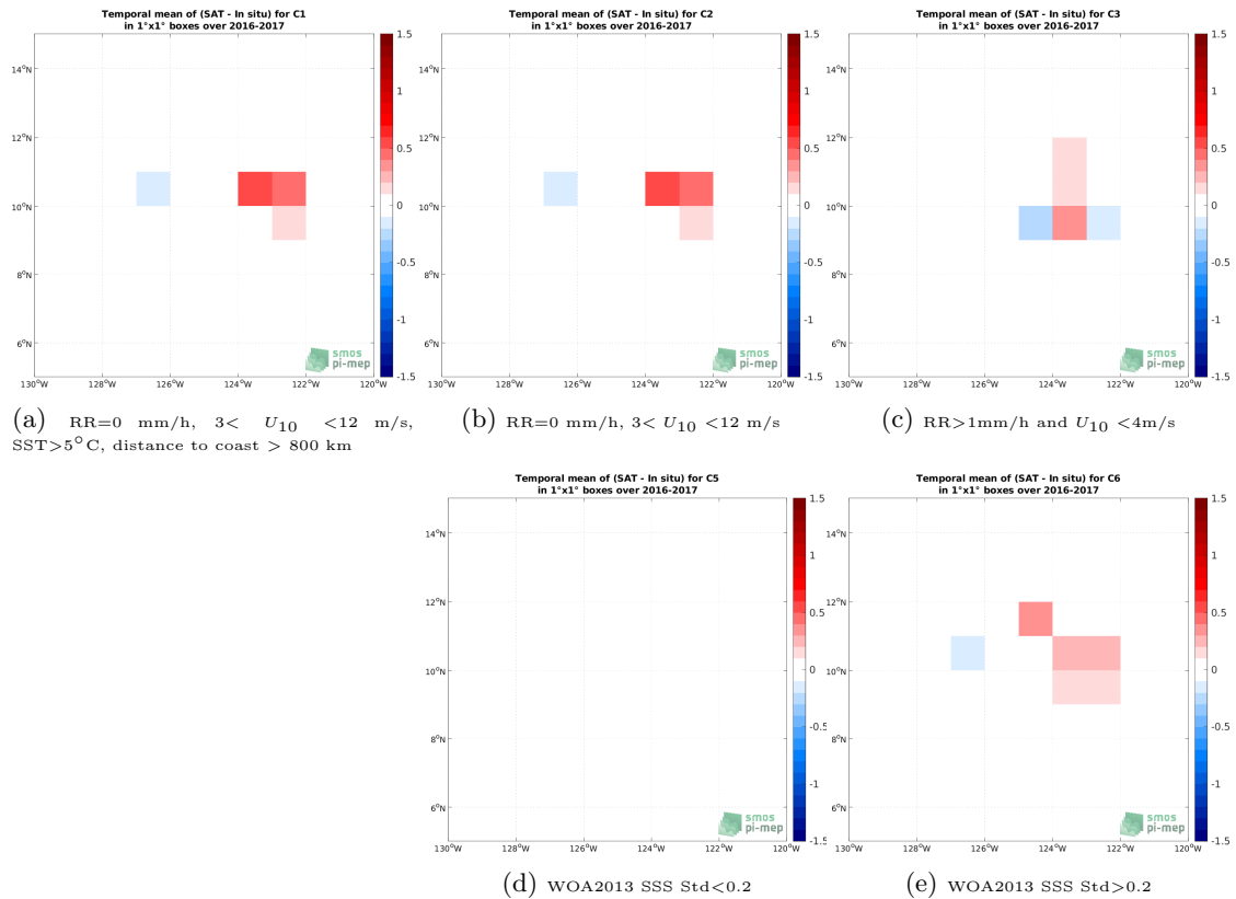
Figure 12: Temporal mean gridded over spatial boxes of size 1^\circ \times 1^\circ of \Delta SSS (SMAP SSS L2 v5 (RSS) - Seaglider) for 5 different subdatasets corresponding to:RR=0 mm/h, 3 < U_{10} < 12 m/s, SST > 5^\circ\text{C} , distance to coast > 800 km (a), RR=0 mm/h, 3 < U_{10} < 12 m/s (b), RR > 1 mm/h and U_{10} < 4 m/s (c), WOA2013 SSS Std < 0.2 (d), WOA2013 SSS Std > 0.2 (e).
