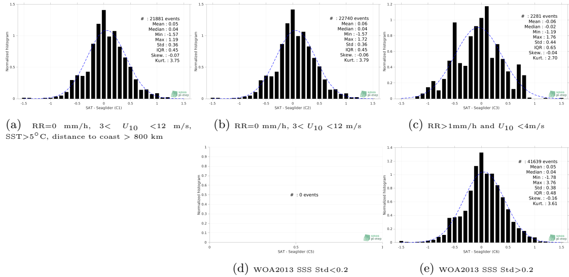
Figure 13: Normalized histogram of \Delta SSS (SMAP SSS L2 v5 (RSS) - Seaglider) for 5 different subdatasets corresponding to: RR=0 mm/h, 3 < U_{10} < 12 m/s, SST > 5°C, distance to coast > 800 km (a), RR=0 mm/h, 3 < U_{10} < 12 m/s (b), RR > 1mm/h and U_{10} < 4 m/s (c), WOA2013 SSS Std < 0.2 (d), WOA2013 SSS Std > 0.2 (e).
