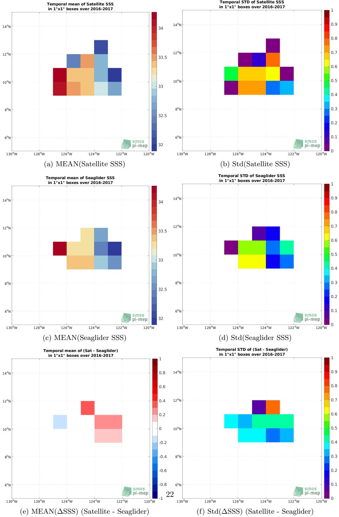
Figure 6: Temporal mean (left) and Std (right) of SSS from SMAP SSS L2 v5 (RSS) (top), Seaglider (middle), and of \Delta SSS (Satellite - Seaglider). Only match-up pairs are used to generate these maps.
