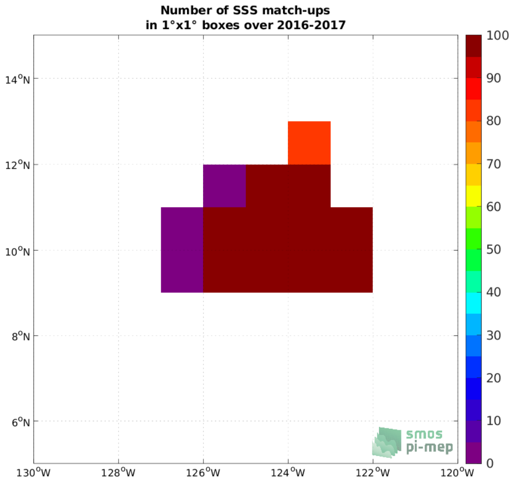
Figure 4: Number of SSS match-ups between Seaglider SSS and the SMAP SSS L2 v5 (RSS) SSS product for the SPURS 2 Pi-MEP region over 1°x1° boxes and for the full satellite product period.
