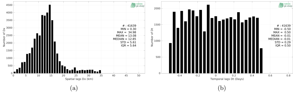
Figure 5: Histograms of the spatial (a) and temporal (b) lags between the location/time of the Seaglider measurement and the date of the corresponding SMAP SSS L2 v5 (RSS) SSS pixel.
