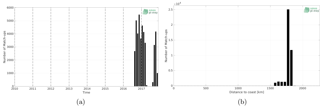
Figure 1: Number of match-ups between Seaglider and SMAP SSS L2 v5 (RSS) SSS as a function of time (a) and as function of the distance to coast (b) over the SPURS 2 Pi-MEP region and for the full satellite product period.
