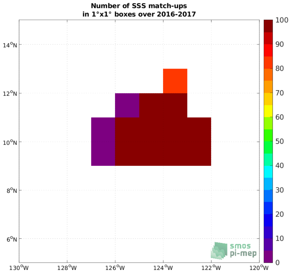
Figure 3: Number of SSS match-ups between Seaglider SSS and the SMAP SSS L2 v5 (RSS) SSS product for the SPURS 2 Pi-MEP region over 1°x1° boxes and for the full satellite product period.
