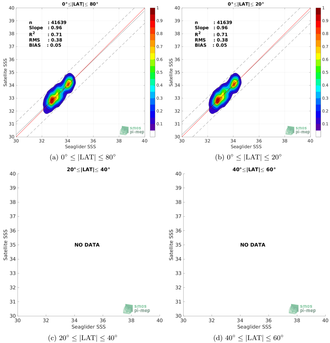
Figure 8: Contour maps of the concentration of SMAP SSS L2 v5 (RSS) SSS (y-axis) versus Seaglider SSS (x-axis) at match-up pairs for different latitude bands. For each plot, the red line shows x=y . The black thin and dashed lines indicate a linear fit through the data cloud and the \pm 95\% confidence levels, respectively. The number match-up pairs n , the slope and R^2 coefficient of the linear fit, the root mean square (RMS) and the mean bias between satellite and in situ data are indicated for each latitude band in each plots.
