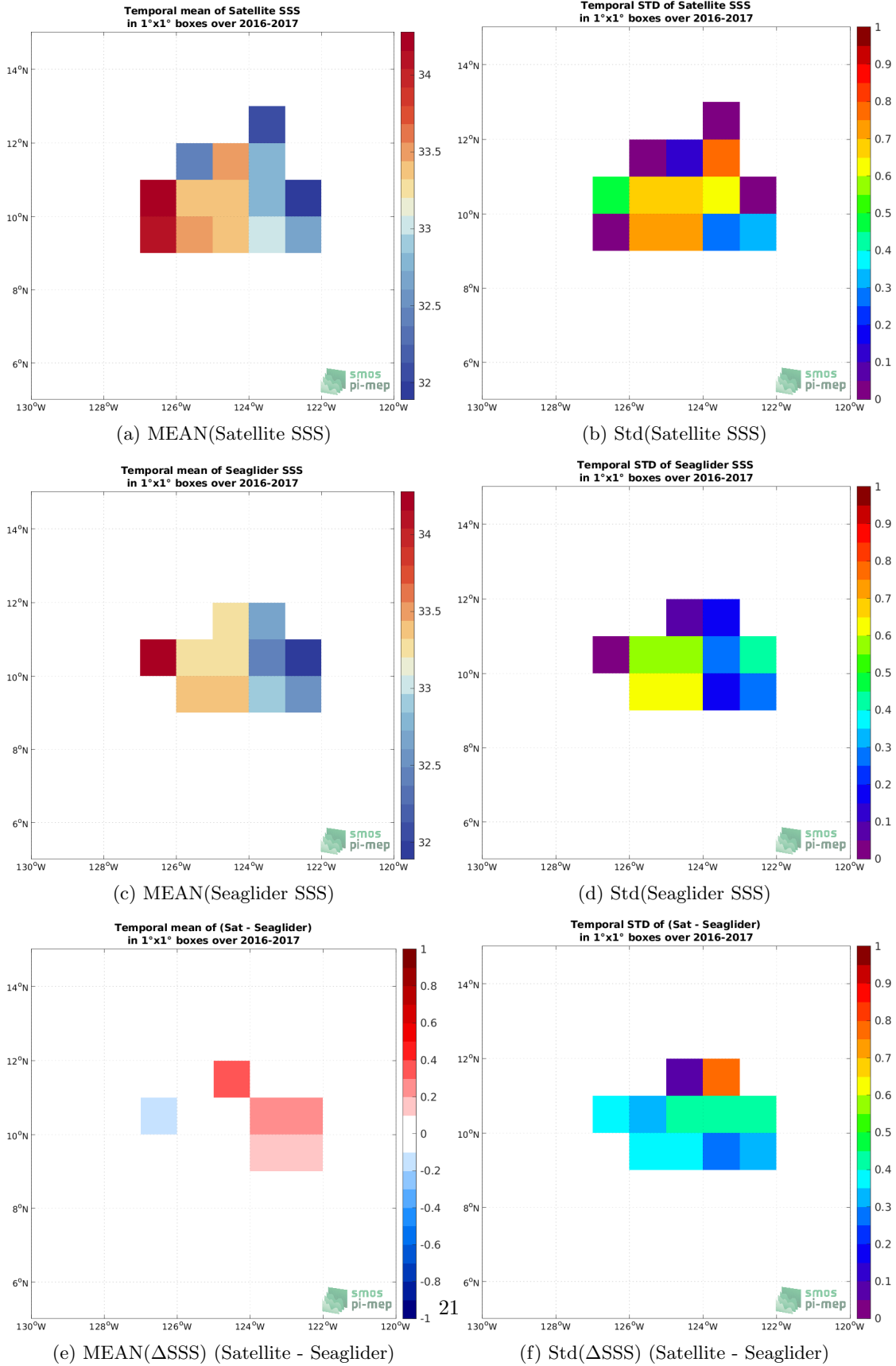
Figure 5: Temporal mean (left) and Std (right) of SSS from SMAP SSS L2 v5 (RSS) (top), Seaglider (middle), and of \Delta SSS (Satellite - Seaglider). Only match-up pairs are used to generate these maps.
