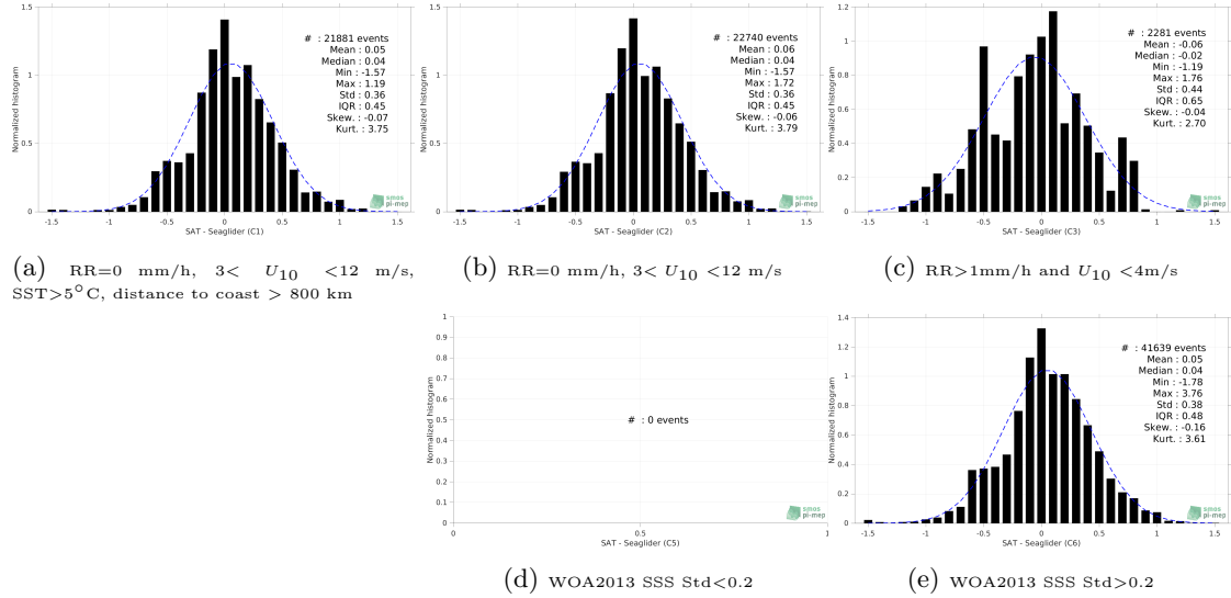
Figure 12: Normalized histogram of \Delta SSS (SMAP SSS L2 v5 (RSS) - Seaglider) for 5 different subdatasets corresponding to: RR=0 mm/h, 3 < U_{10} < 12 m/s, SST>5°C, distance to coast > 800 km (a), RR=0 mm/h, 3 < U_{10} < 12 m/s (b), RR>1mm/h and U_{10} < 4 m/s (c), WOA2013 SSS Std<0.2 (d), WOA2013 SSS Std>0.2 (e).
