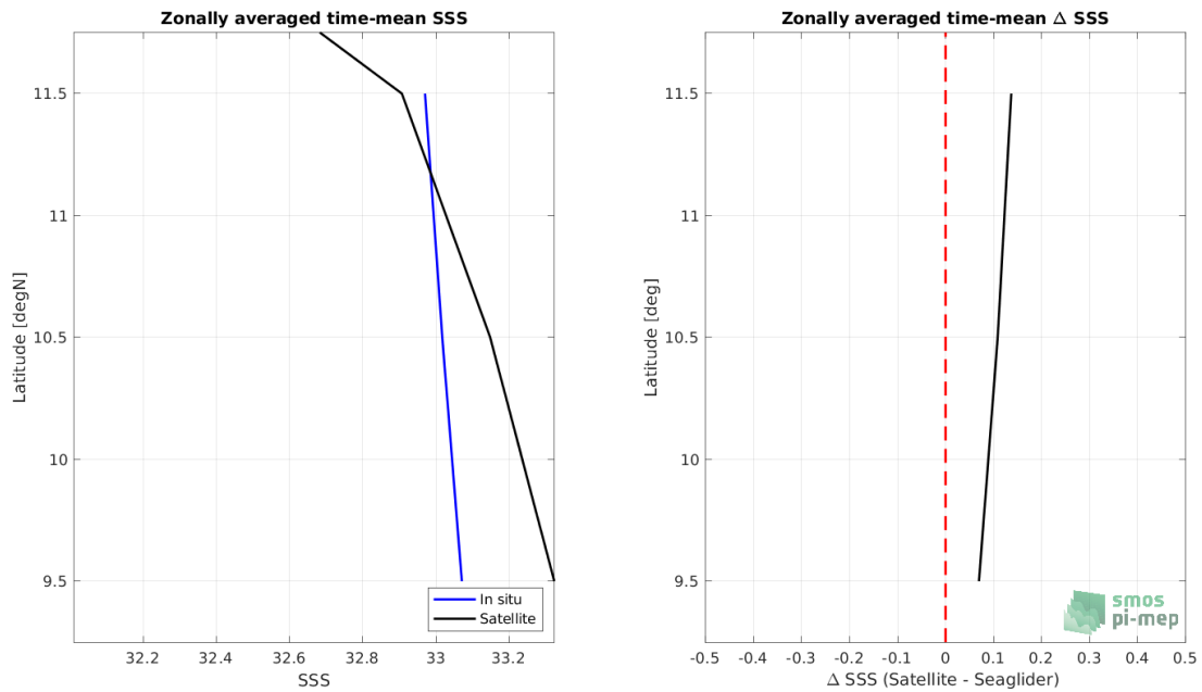
Figure 7: Left panel: Zonal mean SSS from SMAP SSS L2 v5 (RSS) satellite product (black) and from Seaglider (blue). Right panel: Zonal mean of \Delta SSS (Satellite - Seaglider) for all the collected Pi-MEP match-up pairs estimated over the full satellite product period.
