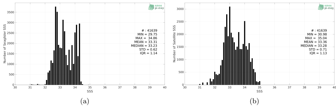
Figure 2: Histograms of SSS from Seaglider (a) and SMAP SSS L2 v5 (RSS) (b) considering all match-up pairs per bins of 0.1 over the SPURS 2 Pi-MEP region and for the full satellite product period.
