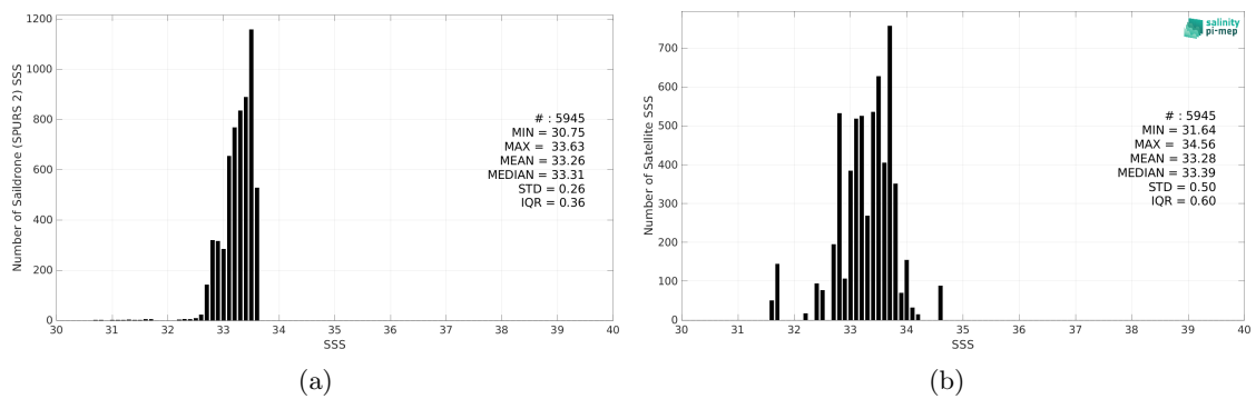
Figure 2: Histograms of SSS from Saildrone (SPURS 2) (a) and SMAP SSS L2 v5 (RSS) (b) considering all match-up pairs per bins of 0.1 over the SPURS 2 Pi-MEP region and for the full satellite product period.
