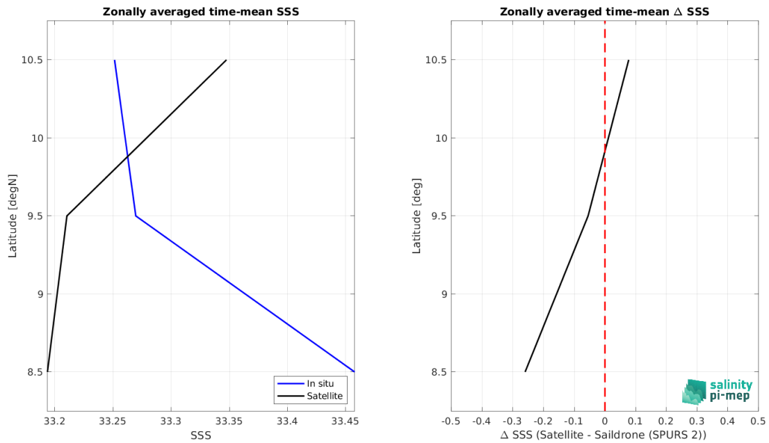
Figure 8: Left panel: Zonal mean SSS from SMAP SSS L2 v5 (RSS) satellite product (black) and from Sairdrone (SPURS 2) (blue). Right panel: Zonal mean of \Delta SSS (Satellite - Sairdrone (SPURS 2)) for all the collected Pi-MEP match-up pairs estimated over the full satellite product period.
