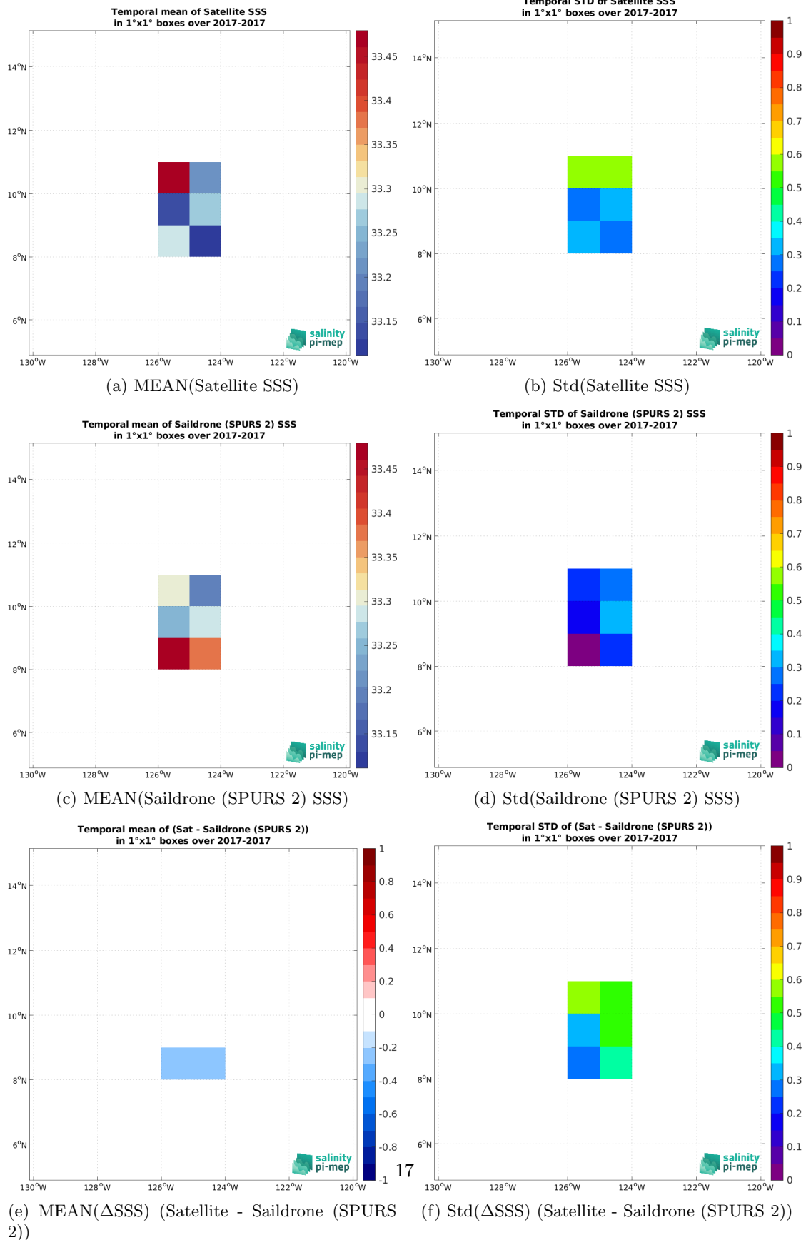
Figure 6: Temporal mean (left) and Std (right) of SSS from SMAP SSS L2 v5 (RSS) (top), Saildrone (SPURS 2) (middle), and of \Delta SSS (Satellite - Saildrone (SPURS 2)). Only match-up pairs are used to generate these maps.
