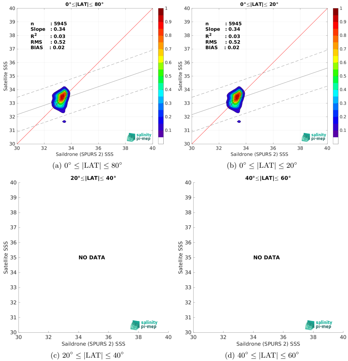
Figure 9: Contour maps of the concentration of SMAP SSS L2 v5 (RSS) SSS (y-axis) versus Saildrone (SPURS 2) SSS (x-axis) at match-up pairs for different latitude bands. For each plot, the red line shows x=y . The black thin and dashed lines indicate a linear fit through the data cloud and the \pm 95\% confidence levels, respectively. The number match-up pairs n , the slope and R^2 coefficient of the linear fit, the root mean square (RMS) and the mean bias between satellite and in situ data are indicated for each latitude band in each plots.
