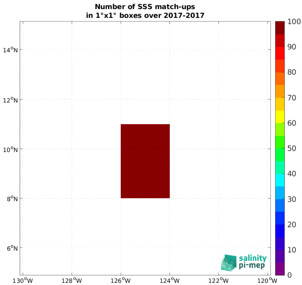
Figure 4: Number of SSS match-ups between Saildrone (SPURS 2) SSS and the SMAP SSS L2 v5 (RSS) SSS product for the SPURS 2 Pi-MEP region over 1^\circ \times 1^\circ boxes and for the full satellite product period.
