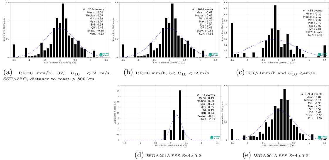
Figure 13: Normalized histogram of \Delta SSS (SMAP SSS L2 v5 (RSS) - Saildrone (SPURS 2)) for 5 different subdatasets corresponding to: RR=0 mm/h, 3 < U_{10} < 12 m/s, SST > 5°C, distance to coast > 800 km (a), RR=0 mm/h, 3 < U_{10} < 12 m/s (b), RR > 1mm/h and U_{10} < 4 m/s (c), WOA2013 SSS Std < 0.2 (d), WOA2013 SSS Std > 0.2 (e).
