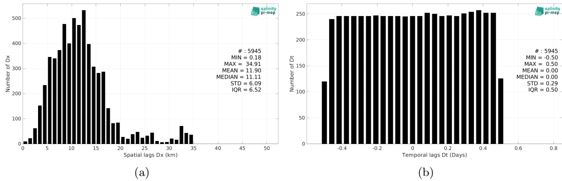
Figure 5: Histograms of the spatial (a) and temporal (b) lags between the location/time of the Saildrone (SPURS 2) measurement and the date of the corresponding SMAP SSS L2 v5 (RSS) SSS pixel.
