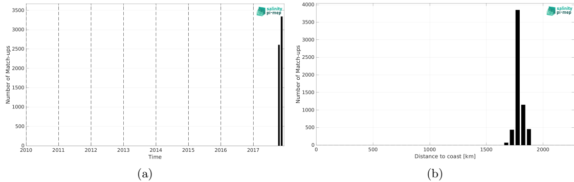
Figure 1: Number of match-ups between Saildrone (SPURS 2) and SMAP SSS L2 v5 (RSS) SSS as a function of time (a) and as function of the distance to coast (b) over the SPURS 2 Pi-MEP region and for the full satellite product period.
