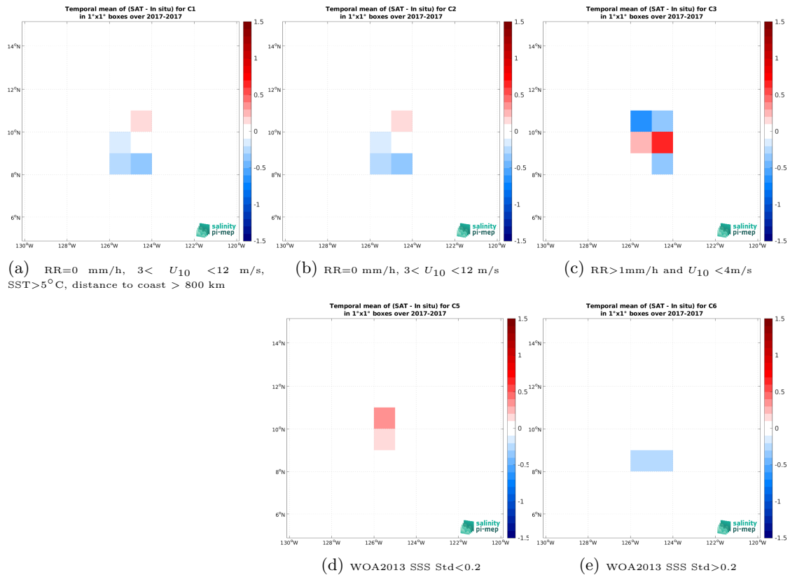
Figure 12: Temporal mean gridded over spatial boxes of size 1^\circ \times 1^\circ of \Delta SSS (SMAP SSS L2 v5 (RSS) - Saildrone (SPURS 2)) for 5 different subdatasets corresponding to:RR=0 mm/h, 3 < U_{10} < 12 m/s, SST >5^\circ\text{C} , distance to coast > 800 km (a), RR=0 mm/h, 3 < U_{10} < 12 m/s (b), RR >1 mm/h and U_{10} < 4 m/s (c), WOA2013 SSS Std <0.2 (d), WOA2013 SSS Std >0.2 (e).
