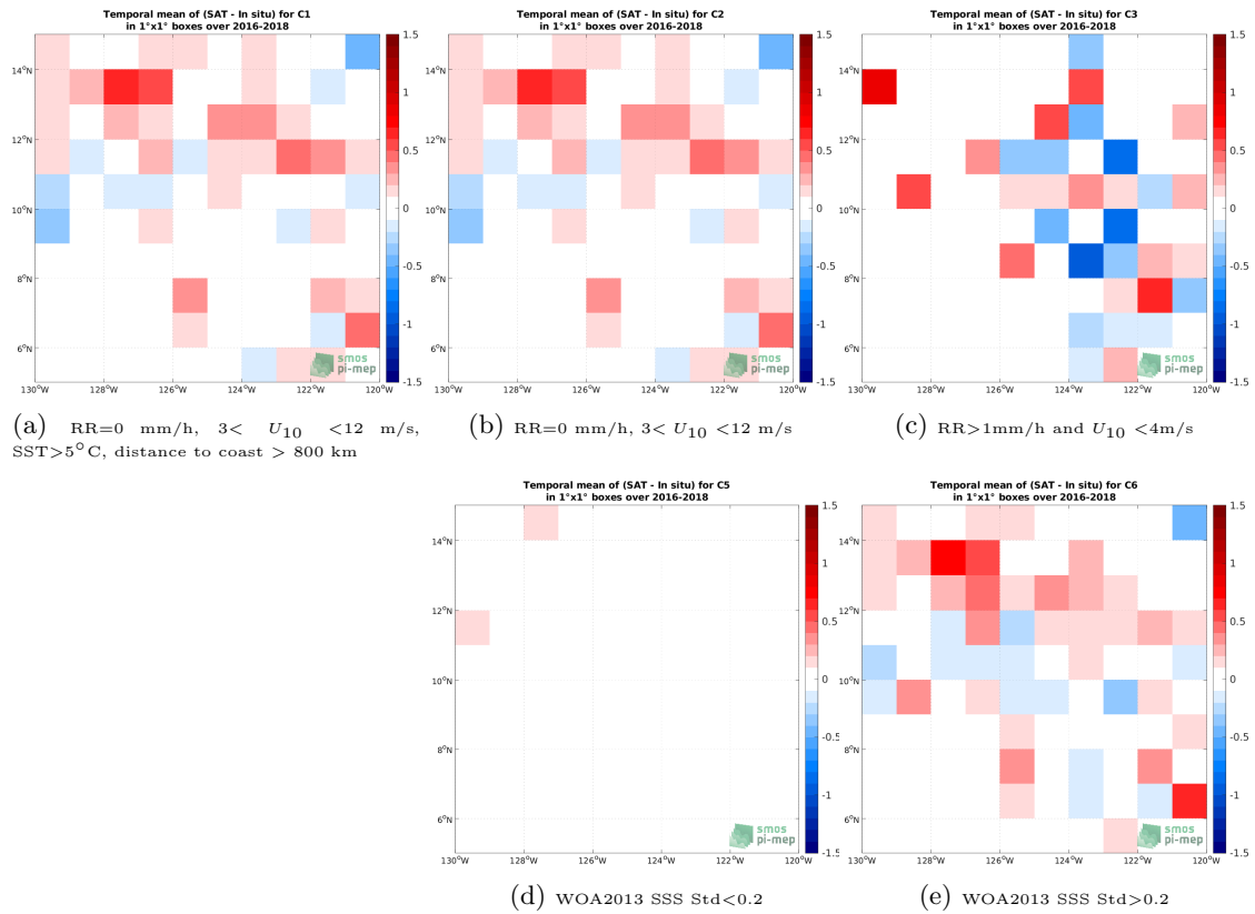
Figure 11: Temporal mean gridded over spatial boxes of size 1^\circ \times 1^\circ of \Delta SSS (SMAP SSS L2 v5 (RSS) - Surface drifters) for 5 different subdatasets corresponding to: RR=0 mm/h, 3 < U_{10} < 12 m/s, SST > 5^\circ C , distance to coast > 800 km (a), RR=0 mm/h, 3 < U_{10} < 12 m/s (b), RR > 1 mm/h and U_{10} < 4 m/s (c), WOA2013 SSS Std < 0.2 (d), WOA2013 SSS Std > 0.2 (e).
