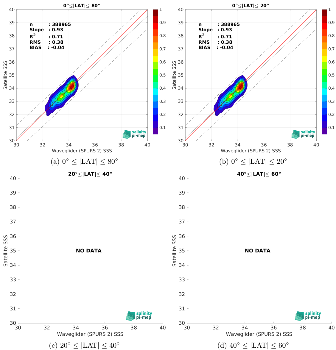
Figure 10: Contour maps of the concentration of SMAP SSS L2 v5.3 (RSS) SSS (y-axis) versus Waveglider (SPURS 2) SSS (x-axis) at match-up pairs for different latitude bands. For each plot, the red line shows x=y . The black thin and dashed lines indicate a linear fit through the data cloud and the \pm 95\% confidence levels, respectively. The number match-up pairs n , the slope and R^2 coefficient of the linear fit, the root mean square (RMS) and the mean bias between satellite and in situ data are indicated for each latitude band in each plots.
