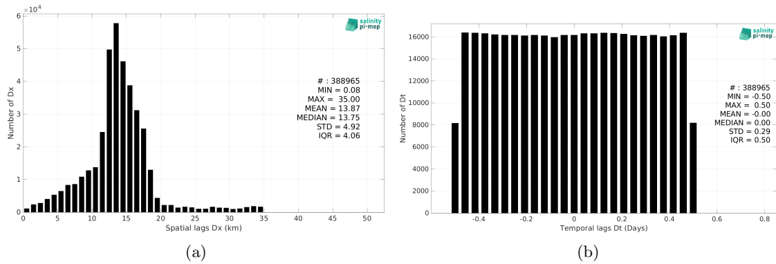
Figure 6: Histograms of the spatial (a) and temporal (b) lags between the location/time of the Waveglider (SPURS 2) measurement and the date of the corresponding SMAP SSS L2 v5.3 (RSS) SSS pixel.
