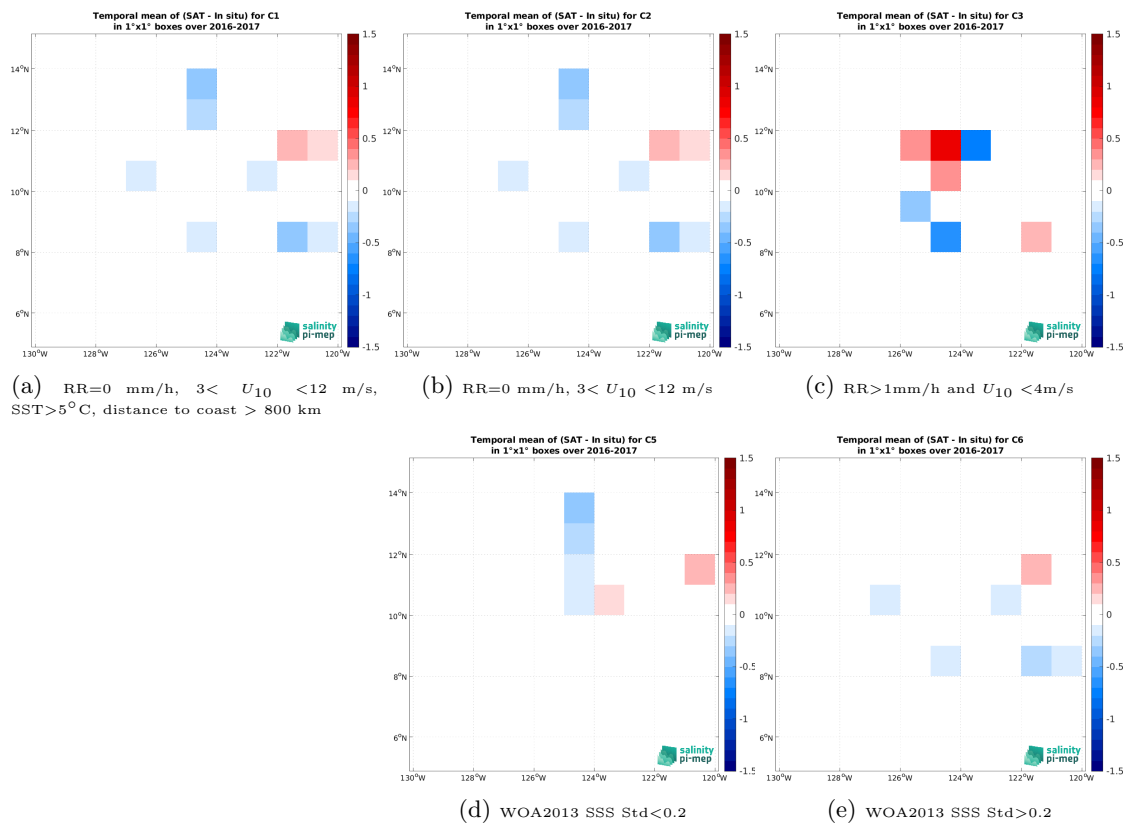
Figure 14: Temporal mean gridded over spatial boxes of size 1^\circ \times 1^\circ of \Delta SSS (SMAP SSS L2 v5.3 (RSS) - Waveglider (SPURS 2)) for 5 different subdatasets corresponding to:RR=0 mm/h, 3 < U_{10} < 12 m/s, SST >5^\circ\text{C} , distance to coast > 800 km (a), RR=0 mm/h, 3 < U_{10} < 12 m/s (b), RR >1 mm/h and U_{10} < 4 m/s (c), WOA2013 SSS Std <0.2 (d), WOA2013 SSS Std >0.2 (e).
