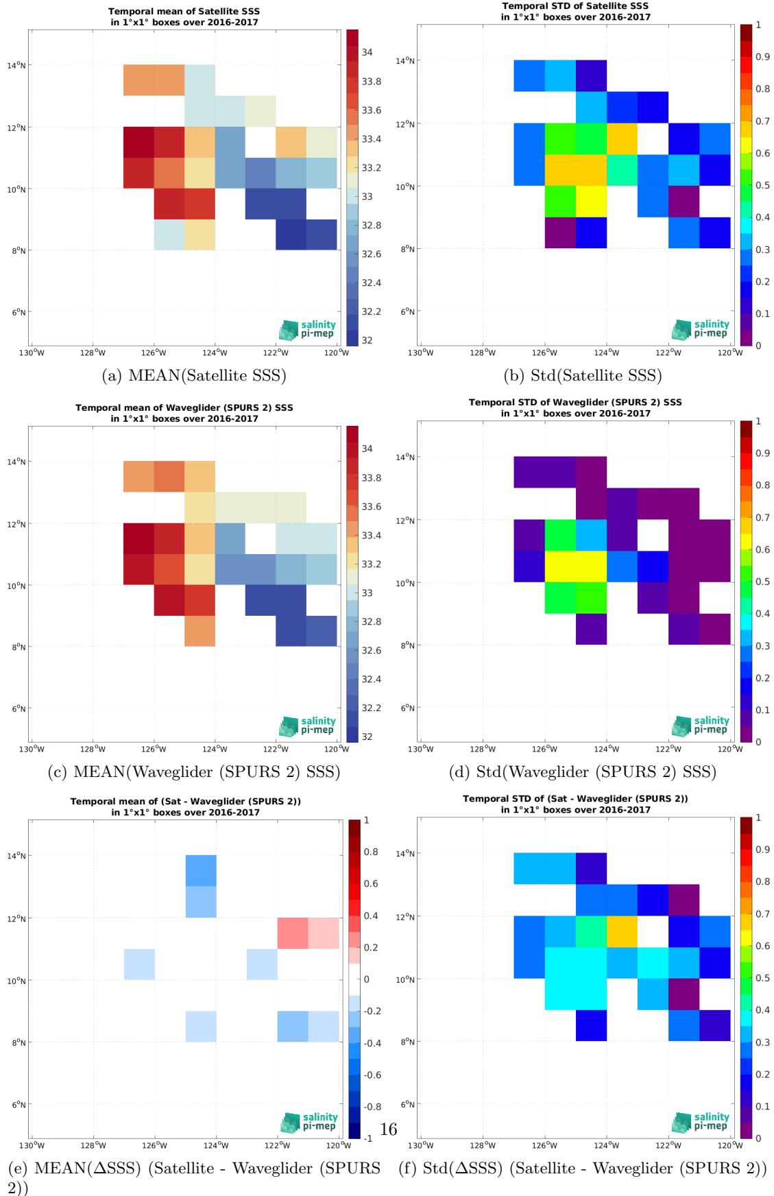
Figure 7: Temporal mean (left) and Std (right) of SSS from SMAP SSS L2 v5.3 (RSS) (top), Waveglider (SPURS 2) (middle), and of \Delta SSS (Satellite - Waveglider (SPURS 2)). Only match-up pairs are used to generate these maps.
