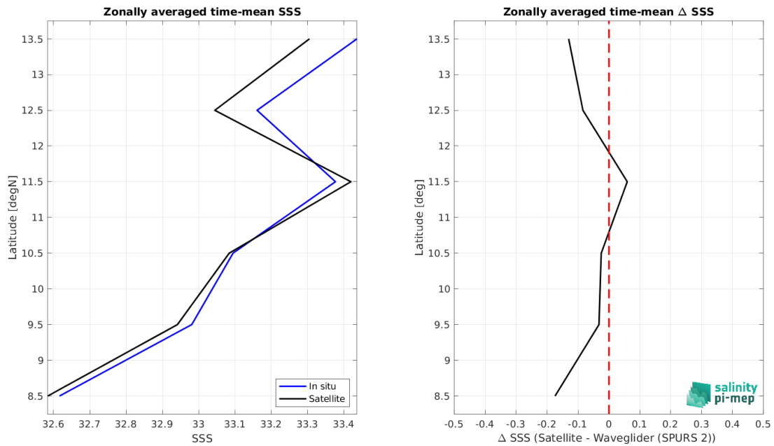
Figure 9: Left panel: Zonal mean SSS from SMAP SSS L2 v5.3 (RSS) satellite product (black) and from Waveglider (SPURS 2) (blue). Right panel: Zonal mean of \Delta SSS (Satellite - Waveglider (SPURS 2)) for all the collected Pi-MEP match-up pairs estimated over the full satellite product period.
