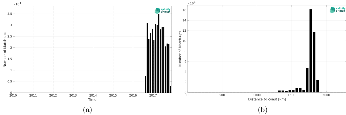
Figure 2: Number of match-ups between Waveglider (SPURS 2) and SMAP SSS L2 v5.3 (RSS) SSS as a function of time (a) and as function of the distance to coast (b) over the SPURS 2 Pi-MEP region and for the full satellite product period.
