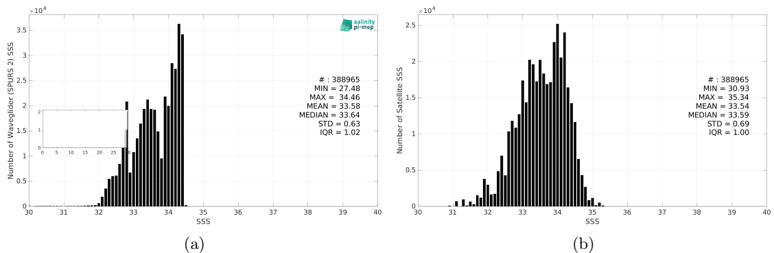
Figure 3: Histograms of SSS from Waveglider (SPURS 2) (a) and SMAP SSS L2 v5.3 (RSS) (b) considering all match-up pairs per bins of 0.1 over the SPURS 2 Pi-MEP region and for the full satellite product period.
