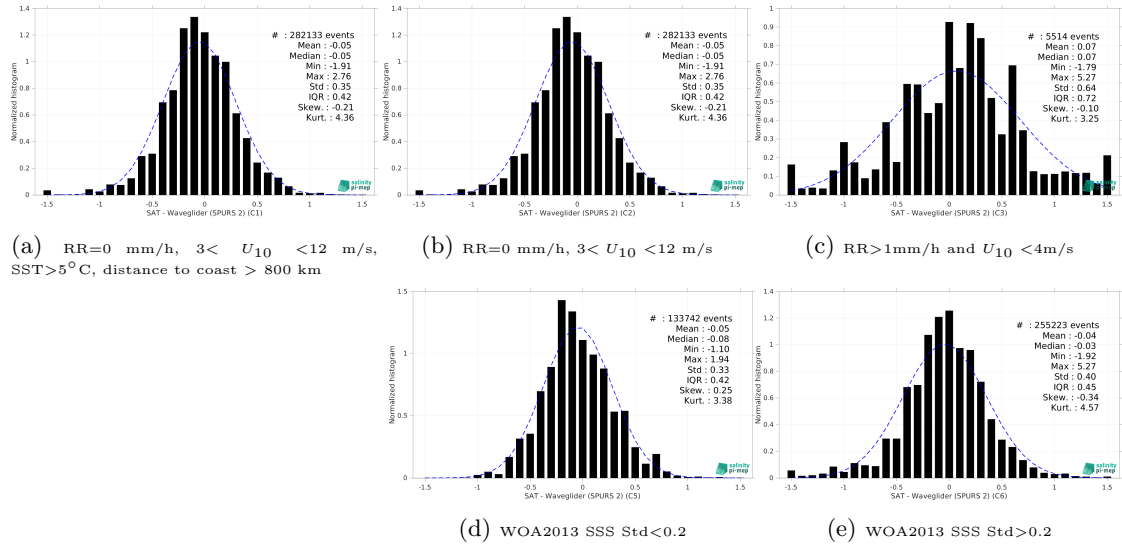
Figure 15: Normalized histogram of \Delta SSS (SMAP SSS L2 v5.3 (RSS) - Waveglider (SPURS 2)) for 5 different subdatasets corresponding to: RR=0 mm/h, 3 < U_{10} < 12 m/s, SST>5°C, distance to coast > 800 km (a), RR=0 mm/h, 3 < U_{10} < 12 m/s (b), RR>1mm/h and U_{10} < 4 m/s (c), WOA2013 SSS Std<0.2 (d), WOA2013 SSS Std>0.2 (e).
