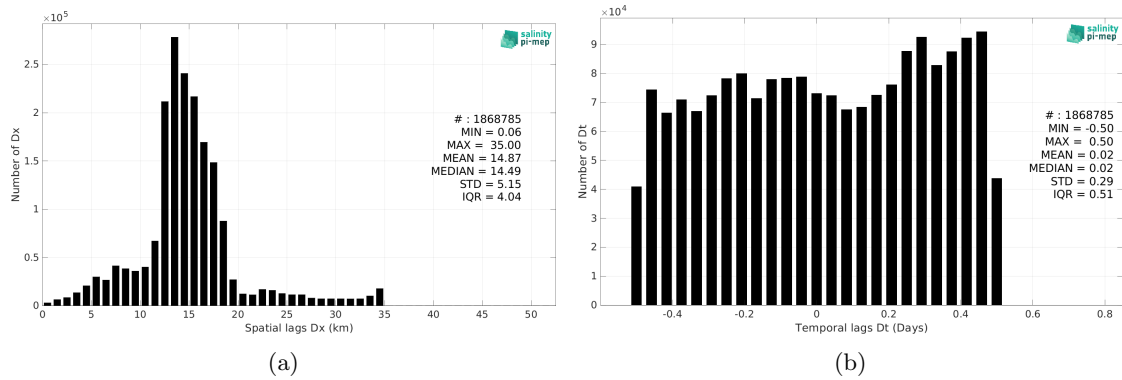
Figure 6: Histograms of the spatial (a) and temporal (b) lags between the location/time of the Salinity Snake (SPURS 2) measurement and the date of the corresponding SMAP SSS L2 v5.3 (RSS) SSS pixel.
