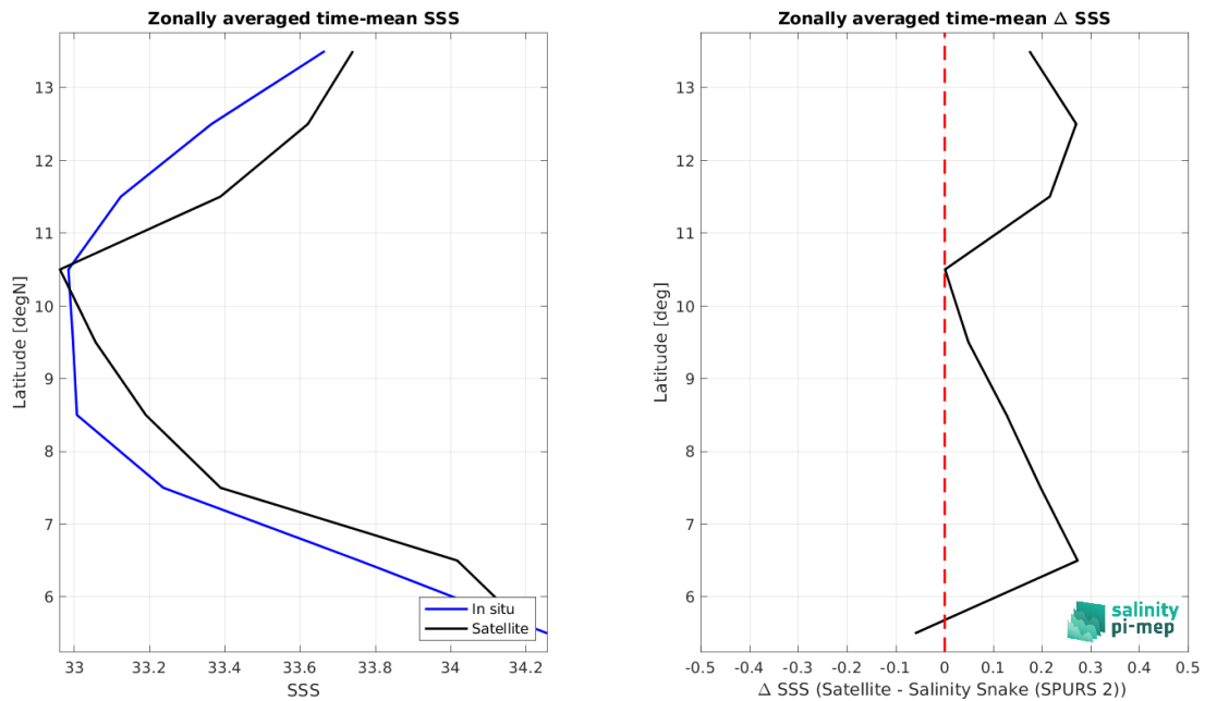
Figure 9: Left panel: Zonal mean SSS from SMAP SSS L2 v5.3 (RSS) satellite product (black) and from Salinity Snake (SPURS 2) (blue). Right panel: Zonal mean of \Delta SSS (Satellite - Salinity Snake (SPURS 2)) for all the collected Pi-MEP match-up pairs estimated over the full satellite product period.
