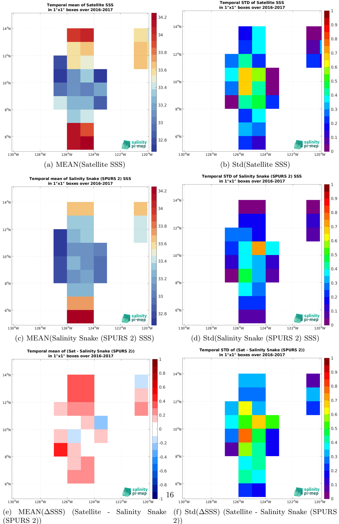
Figure 7: Temporal mean (left) and Std (right) of SSS from SMAP SSS L2 v5.3 (RSS) (top), Salinity Snake (SPURS 2) (middle), and of \Delta SSS (Satellite - Salinity Snake (SPURS 2)). Only match-up pairs are used to generate these maps.
