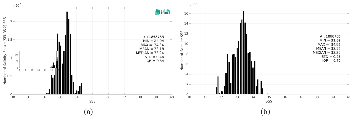
Figure 3: Histograms of SSS from Salinity Snake (SPURS 2) (a) and SMAP SSS L2 v5.3 (RSS) (b) considering all match-up pairs per bins of 0.1 over the SPURS 2 Pi-MEP region and for the full satellite product period.
