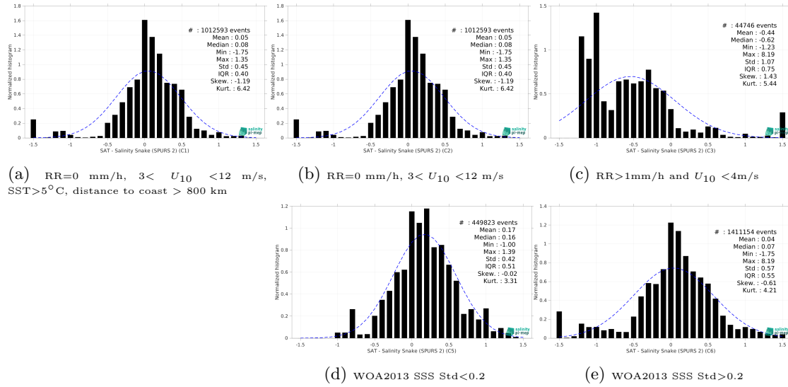
Figure 15: Normalized histogram of \Delta SSS (SMAP SSS L2 v5.3 (RSS) - Salinity Snake (SPURS 2)) for 5 different subdatasets corresponding to: RR=0 mm/h, 3 < U_{10} < 12 m/s, SST > 5°C, distance to coast > 800 km (a), RR=0 mm/h, 3 < U_{10} < 12 m/s (b), RR > 1mm/h and U_{10} < 4 m/s (c), WOA2013 SSS Std < 0.2 (d), WOA2013 SSS Std > 0.2 (e).
