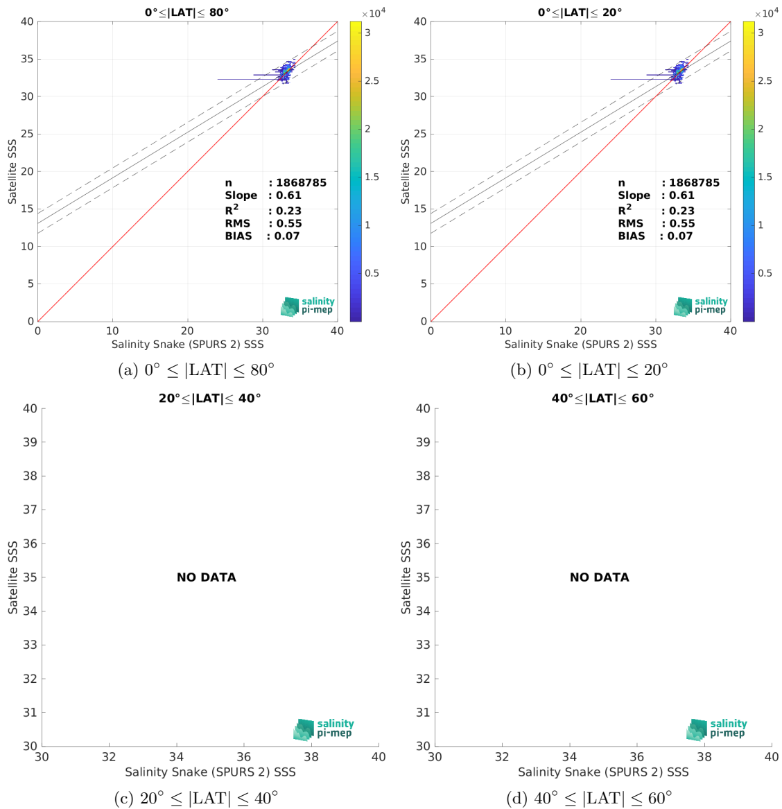
Figure 10: Contour maps of the concentration of SMAP SSS L2 v5.3 (RSS) SSS (y-axis) versus Salinity Snake (SPURS 2) SSS (x-axis) at match-up pairs for different latitude bands. For each plot, the red line shows x=y . The black thin and dashed lines indicate a linear fit through the data cloud and the \pm 95\% confidence levels, respectively. The number match-up pairs n , the slope and R^2 coefficient of the linear fit, the root mean square (RMS) and the mean bias between satellite and in situ data are indicated for each latitude band in each plots.
