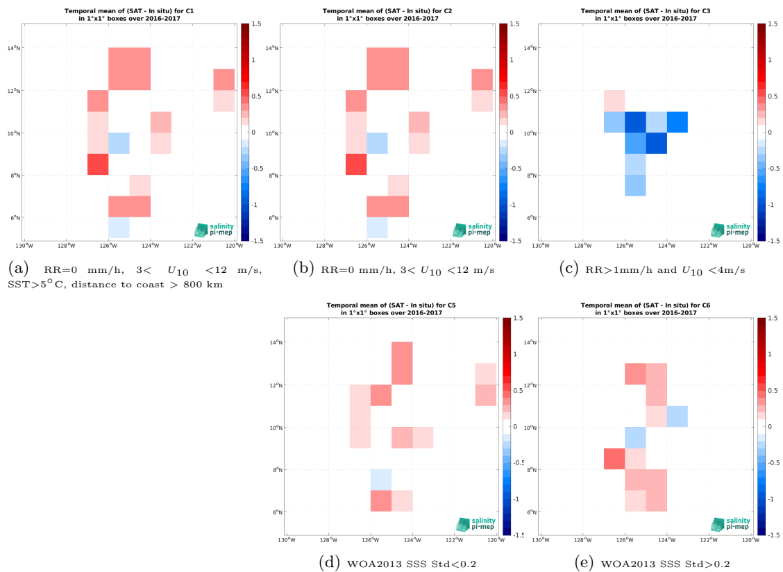
Figure 14: Temporal mean gridded over spatial boxes of size 1^\circ \times 1^\circ of \Delta\text{SSS} (SMAP SSS L2 v5.3 (RSS) - Salinity Snake (SPURS 2)) for 5 different subdatasets corresponding to: RR=0 mm/h, 3 < U_{10} < 12 m/s, SST > 5^\circ\text{C} , distance to coast > 800 km (a), RR=0 mm/h, 3 < U_{10} < 12 m/s (b), RR > 1 mm/h and U_{10} < 4 m/s (c), WOA2013 SSS Std < 0.2 (d), WOA2013 SSS Std > 0.2 (e).
