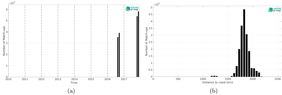
Figure 2: Number of match-ups between Salinity Snake (SPURS 2) and SMAP SSS L2 v5.3 (RSS) SSS as a function of time (a) and as function of the distance to coast (b) over the SPURS 2 Pi-MEP region and for the full satellite product period.
