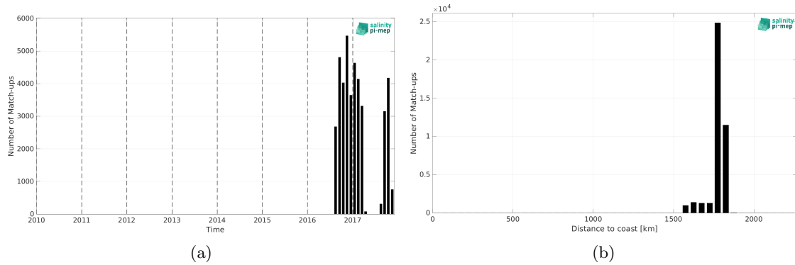
Figure 2: Number of match-ups between Seaglider (SPURS 2) and SMAP SSS L2 v5.3 (RSS) SSS as a function of time (a) and as function of the distance to coast (b) over the SPURS 2 Pi-MEP region and for the full satellite product period.
