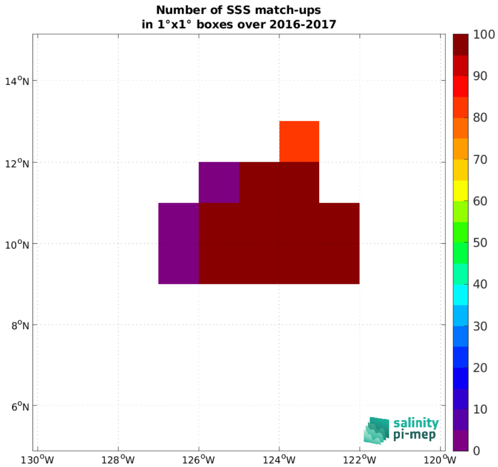
Figure 5: Number of SSS match-ups between Seaglider (SPURS 2) SSS and the SMAP SSS L2 v5.3 (RSS) SSS product for the SPURS 2 Pi-MEP region over 1°x1° boxes and for the full satellite product period.
