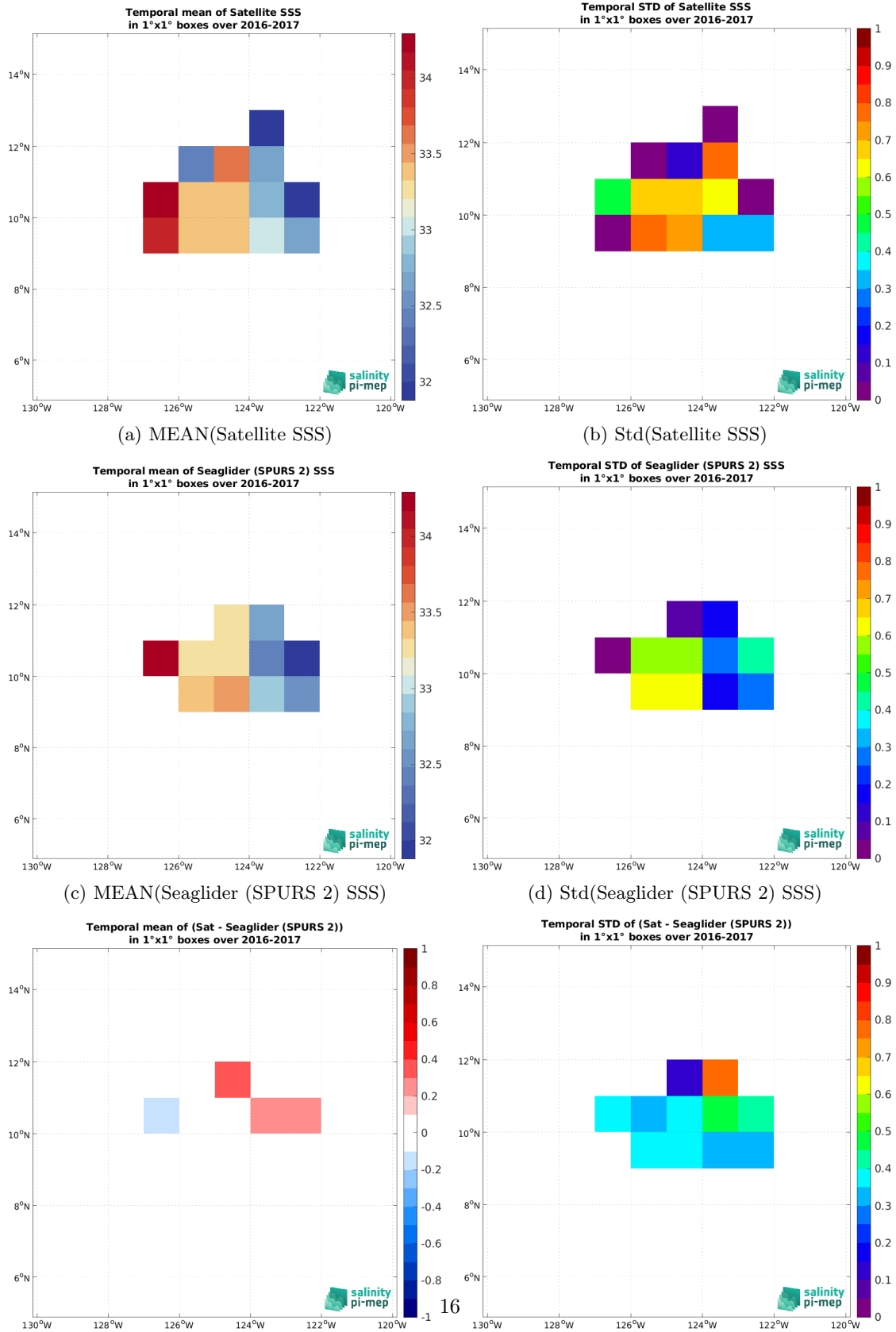
Figure 7: Temporal mean (left) and Std (right) of SSS from SMAP SSS L2 v5.3 (RSS) (top), Seaglider (SPURS 2) (middle), and of \Delta SSS (Satellite - Seaglider (SPURS 2)). Only match-up pairs are used to generate these maps.
