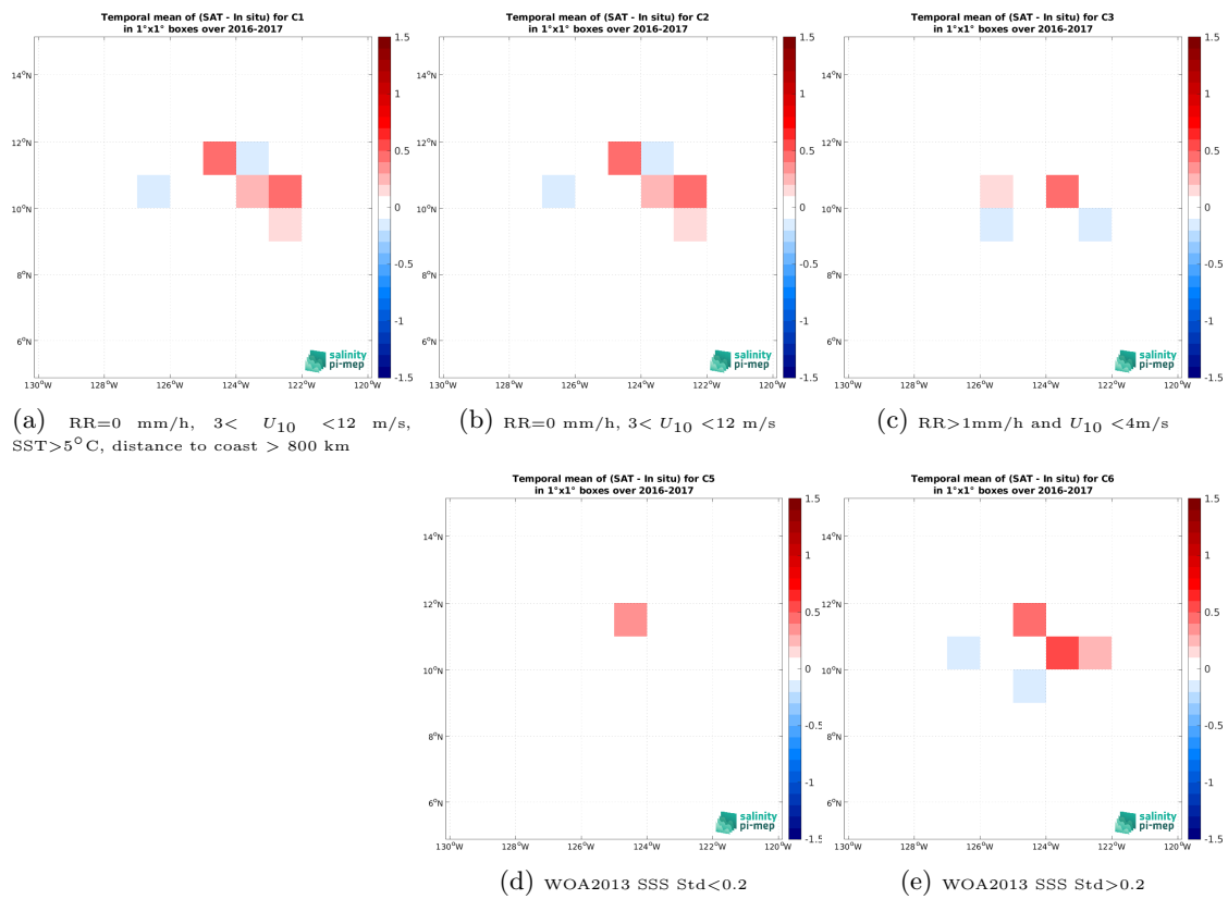
Figure 14: Temporal mean gridded over spatial boxes of size 1^\circ \times 1^\circ of \Delta SSS (SMAP SSS L2 v5.3 (RSS) - Seaglider (SPURS 2)) for 5 different subdatasets corresponding to:RR=0 mm/h, 3 < U_{10} < 12 m/s, SST >5^\circ\text{C} , distance to coast > 800 km (a), RR=0 mm/h, 3 < U_{10} < 12 m/s (b), RR >1 mm/h and U_{10} < 4 m/s (c), WOA2013 SSS Std <0.2 (d), WOA2013 SSS Std >0.2 (e).
