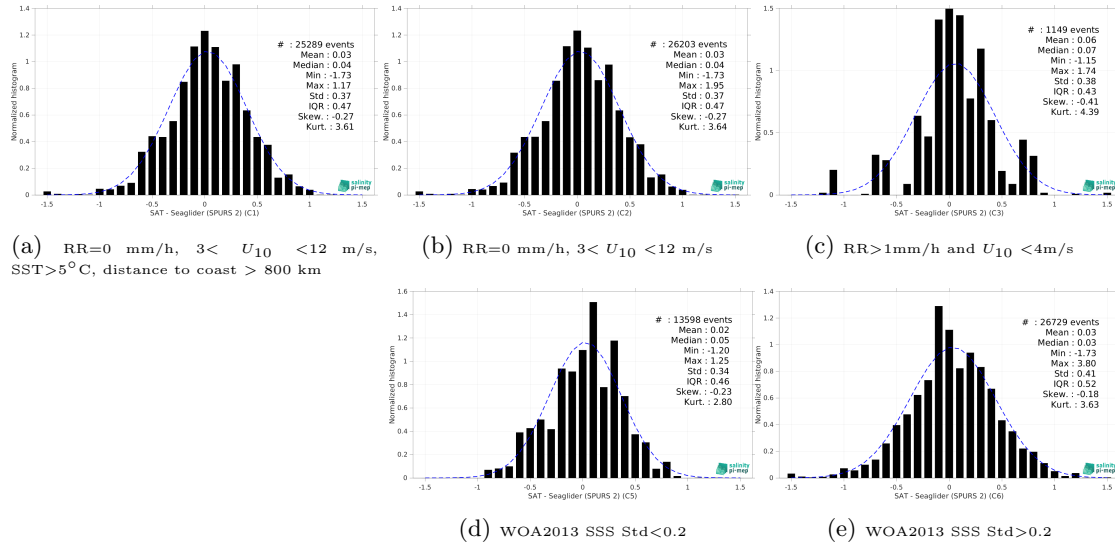
Figure 15: Normalized histogram of \Delta\text{SSS} (SMAP SSS L2 v5.3 (RSS) - Seaglider (SPURS 2)) for 5 different subdatasets corresponding to: RR=0 mm/h, 3 < U_{10} < 12 m/s, SST > 5^\circ\text{C} , distance to coast > 800 km (a), RR=0 mm/h, 3 < U_{10} < 12 m/s (b), RR > 1 mm/h and U_{10} < 4 m/s (c), WOA2013 SSS Std < 0.2 (d), WOA2013 SSS Std > 0.2 (e).
