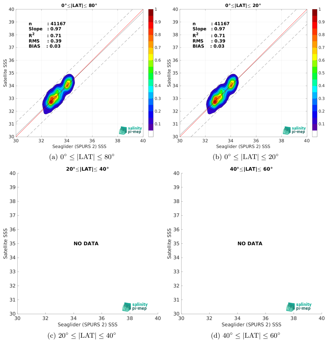
Figure 10: Contour maps of the concentration of SMAP SSS L2 v5.3 (RSS) SSS (y-axis) versus Seaglider (SPURS 2) SSS (x-axis) at match-up pairs for different latitude bands. For each plot, the red line shows x=y . The black thin and dashed lines indicate a linear fit through the data cloud and the \pm 95\% confidence levels, respectively. The number match-up pairs n , the slope and R^2 coefficient of the linear fit, the root mean square (RMS) and the mean bias between satellite and in situ data are indicated for each latitude band in each plots.
