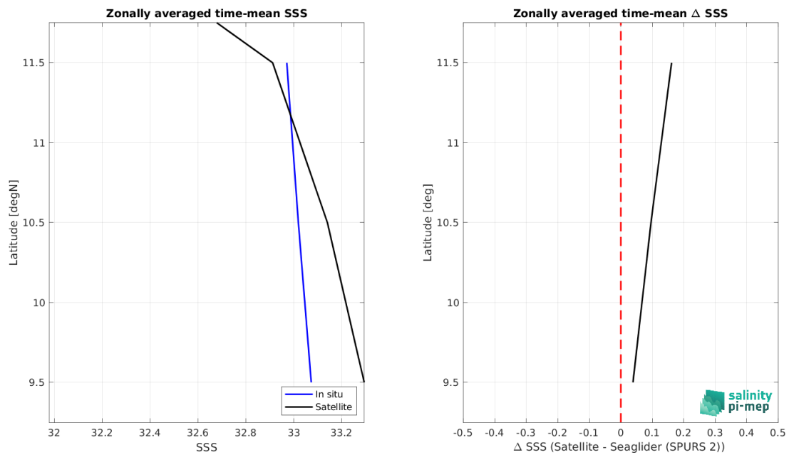
Figure 9: Left panel: Zonal mean SSS from SMAP SSS L2 v5.3 (RSS) satellite product (black) and from Seaglider (SPURS 2) (blue). Right panel: Zonal mean of \Delta SSS (Satellite - Seaglider (SPURS 2)) for all the collected Pi-MEP match-up pairs estimated over the full satellite product period.
