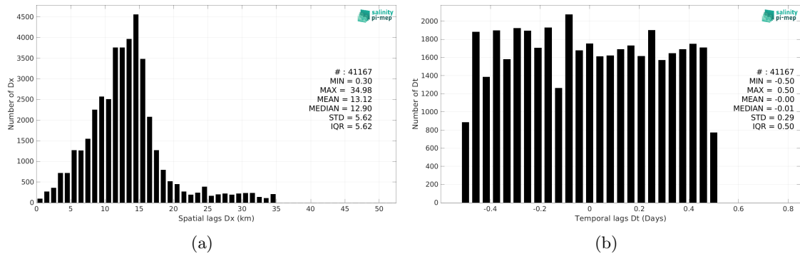
Figure 6: Histograms of the spatial (a) and temporal (b) lags between the location/time of the Seaglider (SPURS 2) measurement and the date of the corresponding SMAP SSS L2 v5.3 (RSS) SSS pixel.
