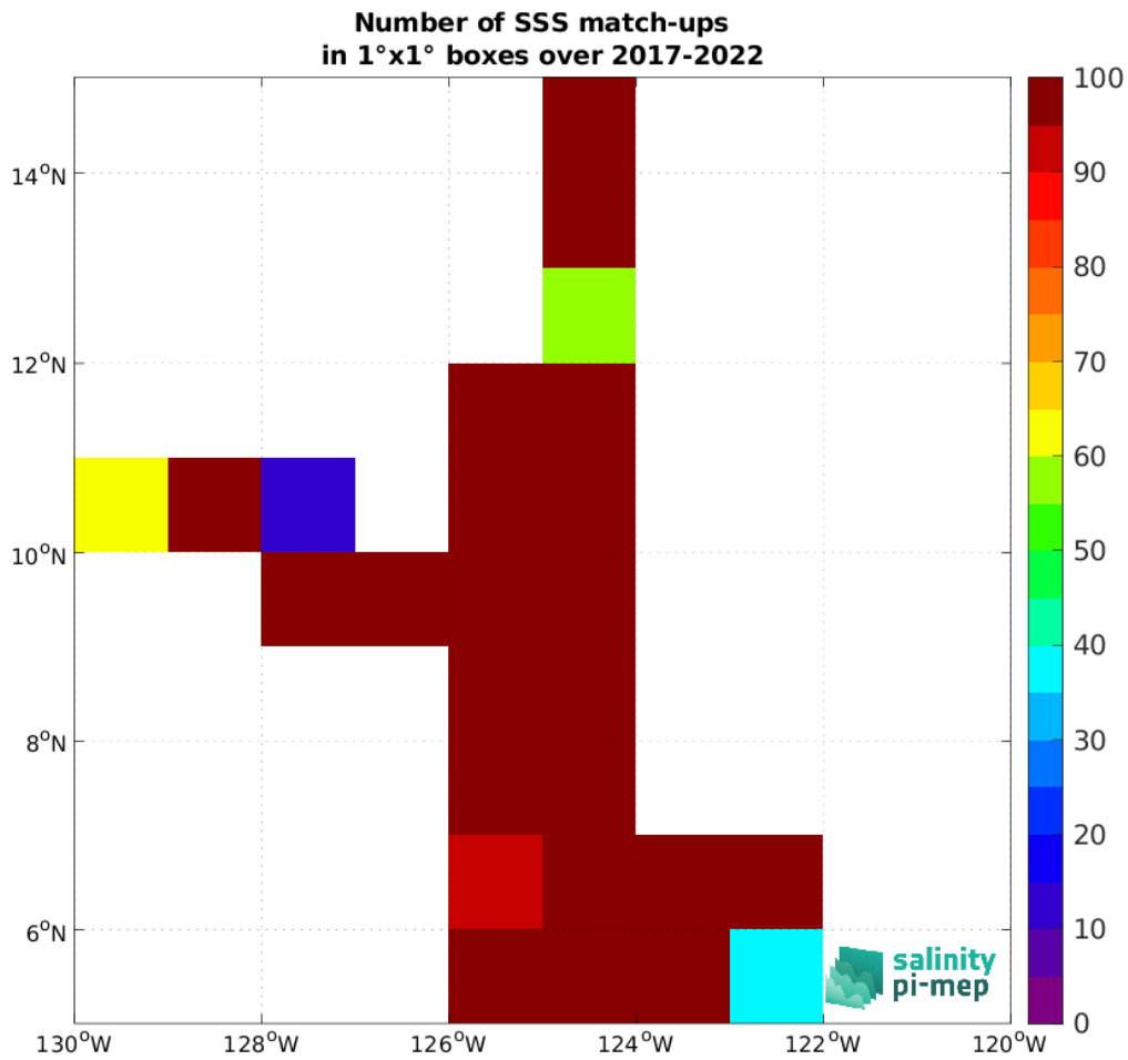
Figure 5: Number of SSS match-ups between Saildrone SSS and the SMAP SSS L2 v5.3 (RSS) SSS product for the SPURS 2 Pi-MEP region over 1^\circ \times 1^\circ boxes and for the full satellite product period.
