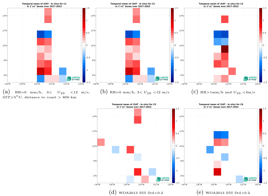
Figure 14: Temporal mean gridded over spatial boxes of size 1^\circ \times 1^\circ of \Delta\text{SSS} (SMAP SSS L2 v5.3 (RSS) - Saildrone) for 5 different subdatasets corresponding to:RR=0 mm/h, 3 < U_{10} < 12 m/s, SST > 5°C, distance to coast > 800 km (a), RR=0 mm/h, 3 < U_{10} < 12 m/s (b), RR > 1mm/h and U_{10} < 4 m/s (c), WOA2013 SSS Std < 0.2 (d), WOA2013 SSS Std > 0.2 (e).
