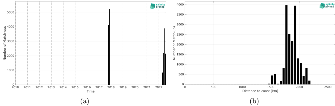
Figure 2: Number of match-ups between Saildrone and SMAP SSS L2 v5.3 (RSS) SSS as a function of time (a) and as function of the distance to coast (b) over the SPURS 2 Pi-MEP region and for the full satellite product period.
