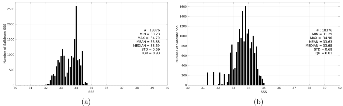
Figure 3: Histograms of SSS from Saildrone (a) and SMAP SSS L2 v5.3 (RSS) (b) considering all match-up pairs per bins of 0.1 over the SPURS 2 Pi-MEP region and for the full satellite product period.
