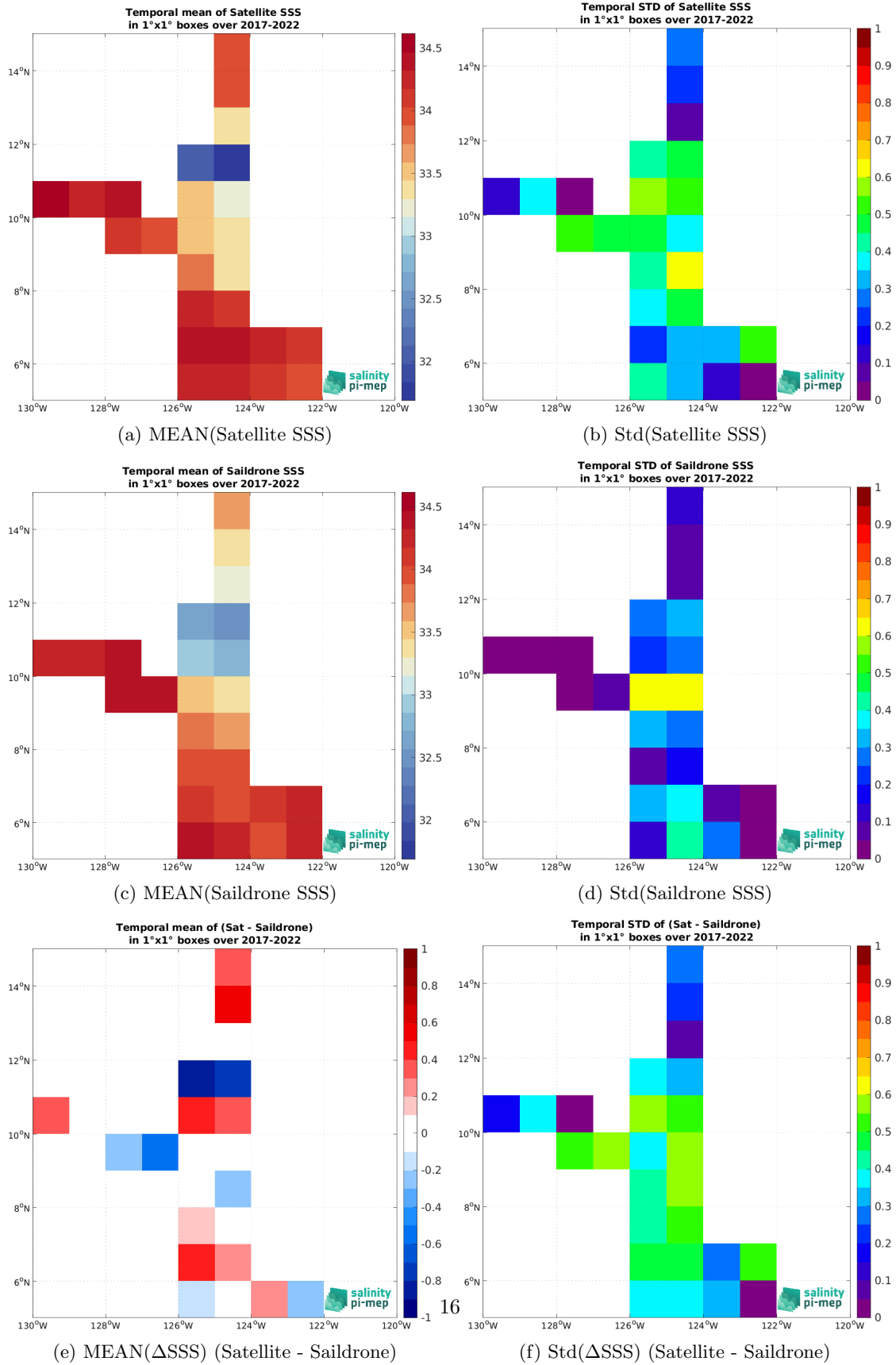
Figure 7: Temporal mean (left) and Std (right) of SSS from SMAP SSS L2 v5.3 (RSS) (top), Saildrone (middle), and of \Delta SSS (Satellite - Saildrone). Only match-up pairs are used to generate these maps.
