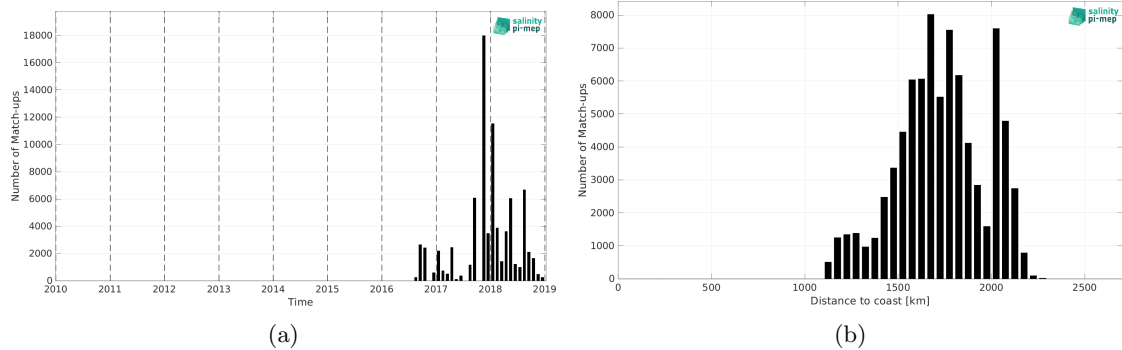
Figure 2: Number of match-ups between Surface drifters and SMAP SSS L2 v5.3 (RSS) SSS as a function of time (a) and as function of the distance to coast (b) over the SPURS 2 Pi-MEP region and for the full satellite product period.
