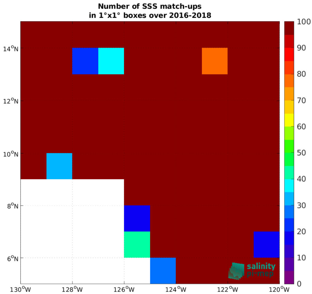
Figure 4: Number of SSS match-ups between Surface drifters SSS and the SMAP SSS L2 v5.3 (RSS) SSS product for the SPURS 2 Pi-MEP region over 1^\circ \times 1^\circ boxes and for the full satellite product period.
