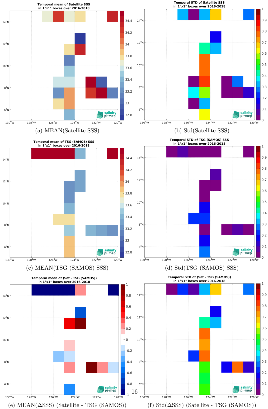
Figure 7: Temporal mean (left) and Std (right) of SSS from SMAP SSS L2 v5.3 - 40 km (RSS) (top), TSG (SAMOS) (middle), and of \Delta SSS (Satellite - TSG (SAMOS)). Only match-up pairs are used to generate these maps.
