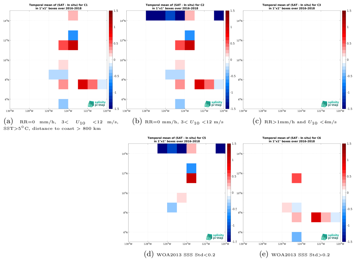
Figure 14: Temporal mean gridded over spatial boxes of size 1^\circ \times 1^\circ of \Delta SSS (SMAP SSS L2 v5.3 - 40 km (RSS) - TSG (SAMOS)) for 5 different subdatasets corresponding to: RR=0 mm/h, 3 < U_{10} < 12 m/s, SST > 5^\circ C , distance to coast > 800 km (a), RR=0 mm/h, 3 < U_{10} < 12 m/s (b), RR > 1 mm/h and U_{10} < 4 m/s (c), WOA2013 SSS Std < 0.2 (d), WOA2013 SSS Std > 0.2 (e).
