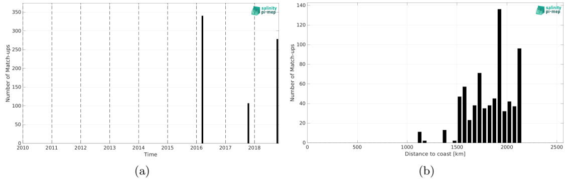
Figure 2: Number of match-ups between TSG (SAMOS) and SMAP SSS L2 v5.3 - 40 km (RSS) SSS as a function of time (a) and as function of the distance to coast (b) over the SPURS 2 Pi-MEP region and for the full satellite product period.
