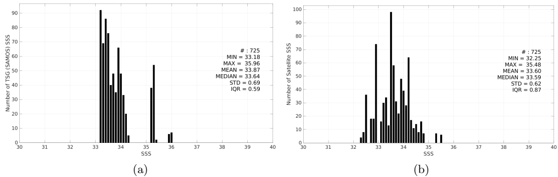
Figure 3: Histograms of SSS from TSG (SAMOS) (a) and SMAP SSS L2 v5.3 - 40 km (RSS) (b) considering all match-up pairs per bins of 0.1 over the SPURS 2 Pi-MEP region and for the full satellite product period.
