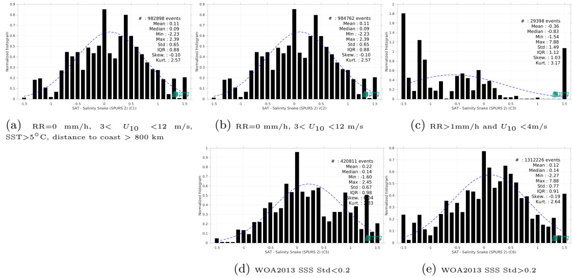
Figure 15: Normalized histogram of \Delta SSS (SMAP SSS L2 v5.3 - 40 km (RSS) - Salinity Snake (SPURS 2)) for 5 different subdatasets corresponding to: RR=0 mm/h, 3 < U_{10} < 12 m/s, SST > 5°C, distance to coast > 800 km (a), RR=0 mm/h, 3 < U_{10} < 12 m/s (b), RR > 1mm/h and U_{10} < 4 m/s (c), WOA2013 SSS Std < 0.2 (d), WOA2013 SSS Std > 0.2 (e).
