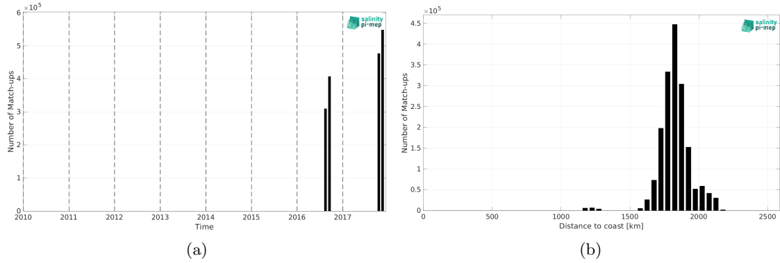
Figure 2: Number of match-ups between Salinity Snake (SPURS 2) and SMAP SSS L2 v5.3 - 40 km (RSS) SSS as a function of time (a) and as function of the distance to coast (b) over the SPURS 2 Pi-MEP region and for the full satellite product period.
