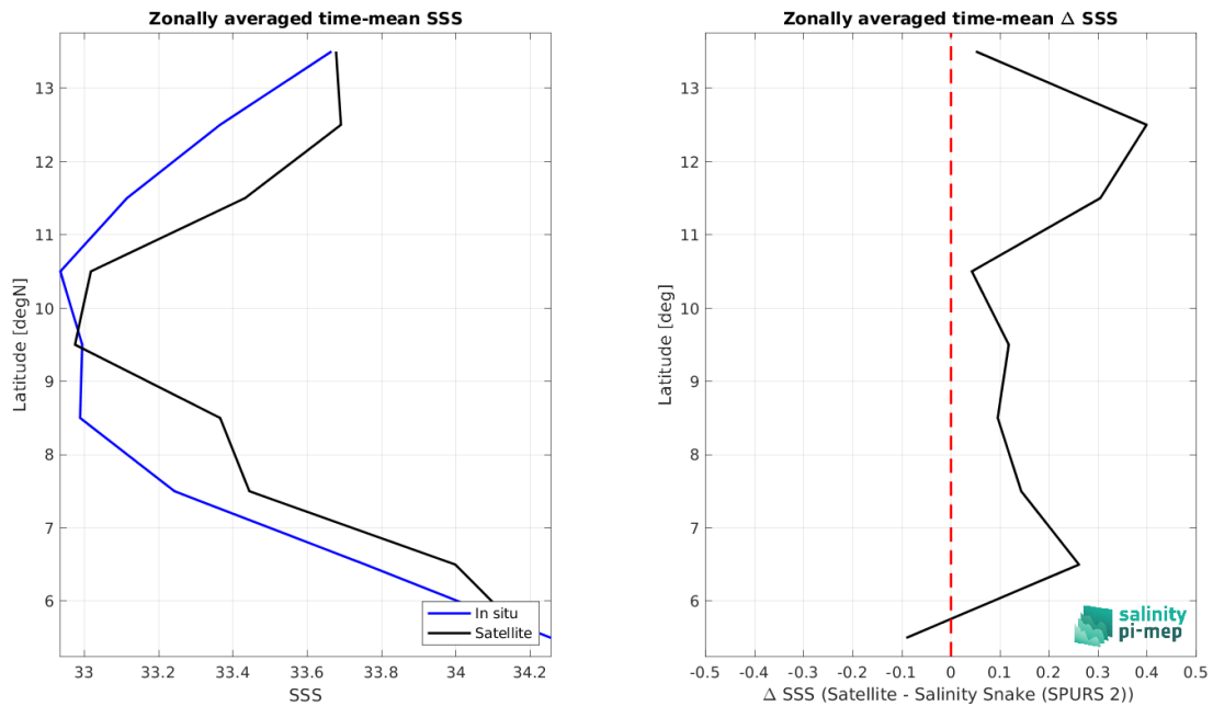
Figure 9: Left panel: Zonal mean SSS from SMAP SSS L2 v5.3 - 40 km (RSS) satellite product (black) and from Salinity Snake (SPURS 2) (blue). Right panel: Zonal mean of \Delta SSS (Satellite - Salinity Snake (SPURS 2)) for all the collected Pi-MEP match-up pairs estimated over the full satellite product period.
