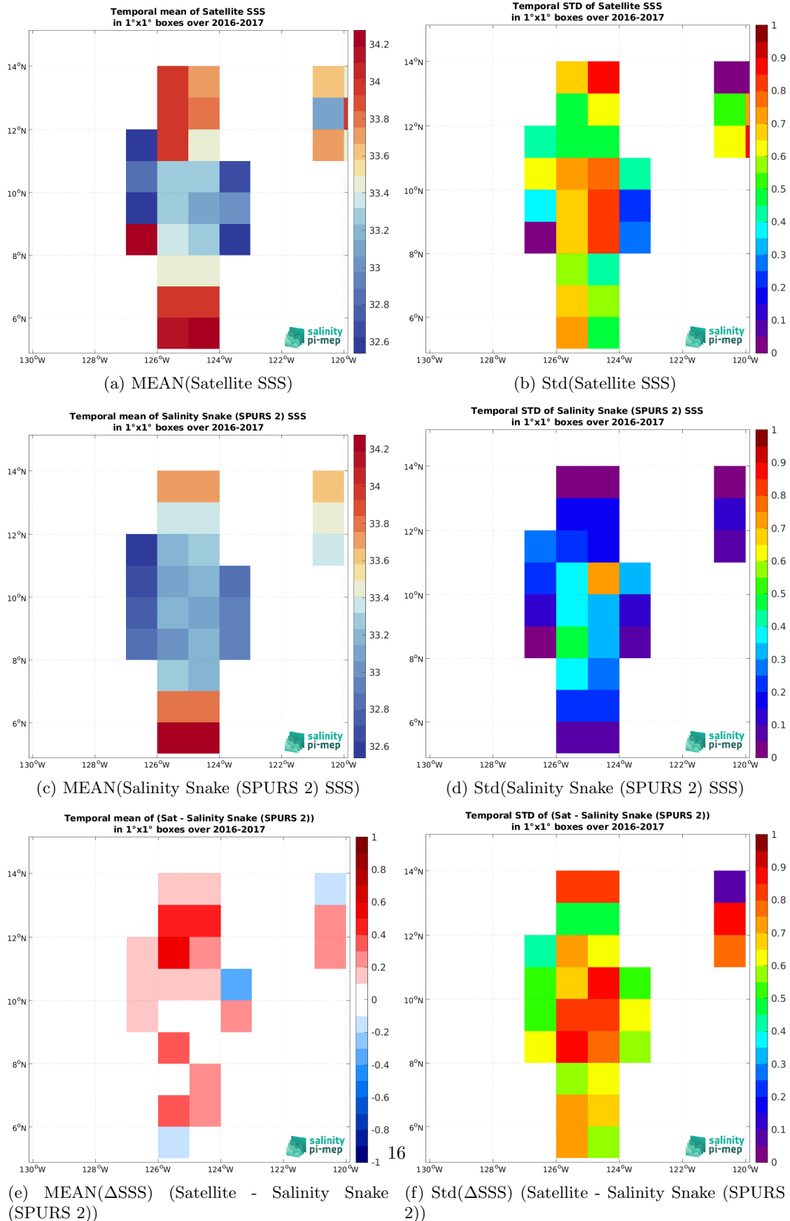
Figure 7: Temporal mean (left) and Std (right) of SSS from SMAP SSS L2 v5.3 - 40 km (RSS) (top), Salinity Snake (SPURS 2) (middle), and of \Delta SSS (Satellite - Salinity Snake (SPURS 2)). Only match-up pairs are used to generate these maps.
