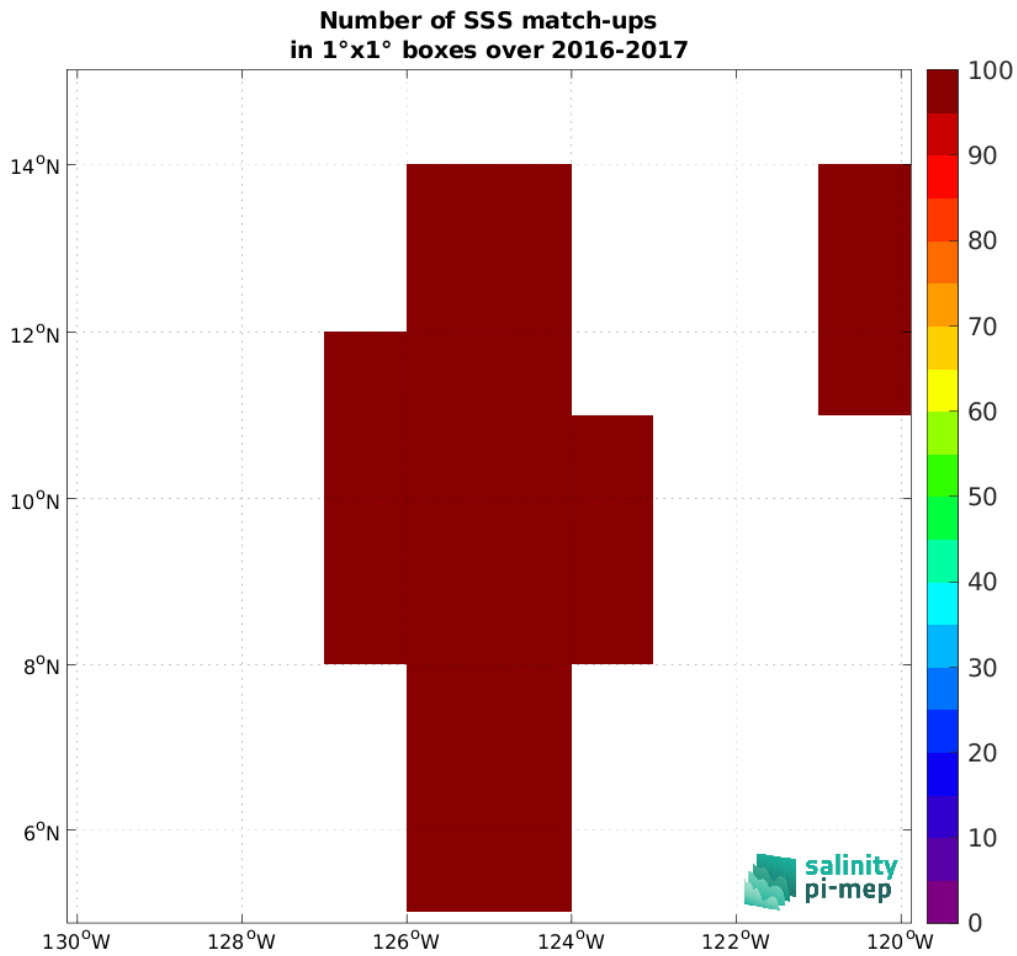
Figure 5: Number of SSS match-ups between Salinity Snake (SPURS 2) SSS and the SMAP SSS L2 v5.3 - 40 km (RSS) SSS product for the SPURS 2 Pi-MEP region over 1^\circ \times 1^\circ boxes and for the full satellite product period.
