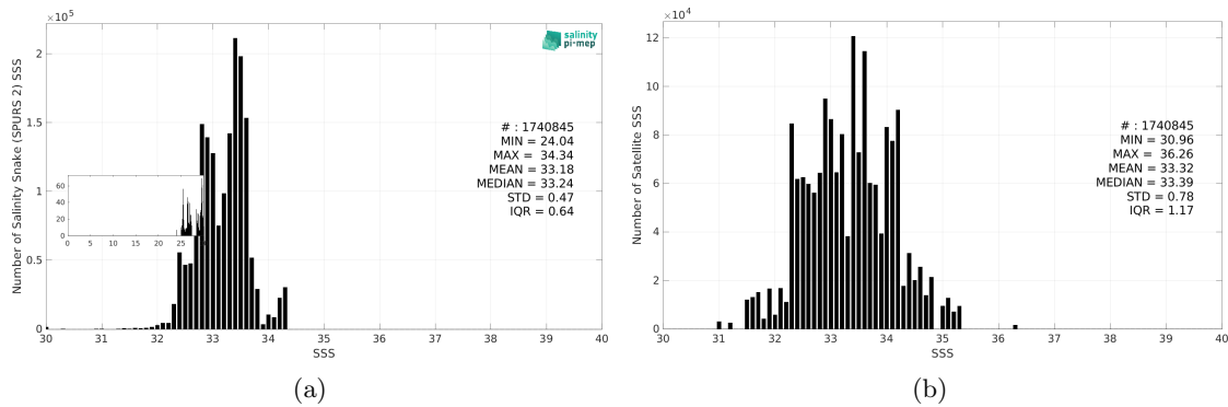
Figure 3: Histograms of SSS from Salinity Snake (SPURS 2) (a) and SMAP SSS L2 v5.3 - 40 km (RSS) (b) considering all match-up pairs per bins of 0.1 over the SPURS 2 Pi-MEP region and for the full satellite product period.
