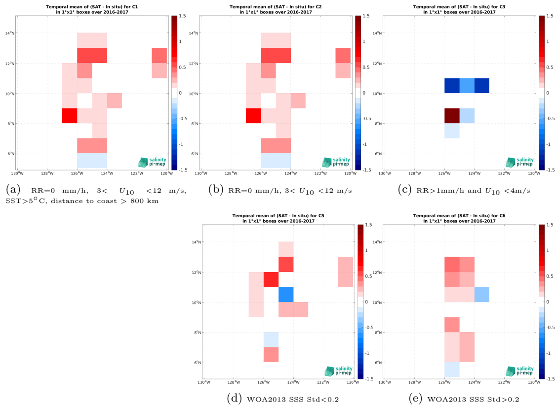
Figure 14: Temporal mean gridded over spatial boxes of size 1^\circ \times 1^\circ of \Delta\text{SSS} (SMAP SSS L2 v5.3 - 40 km (RSS) - Salinity Snake (SPURS 2)) for 5 different subdatasets corresponding to:RR=0 mm/h, 3 < U_{10} < 12 m/s, SST>5°C, distance to coast > 800 km (a), RR=0 mm/h, 3 < U_{10} < 12 m/s (b), RR>1mm/h and U_{10} < 4 m/s (c), WOA2013 SSS Std<0.2 (d), WOA2013 SSS Std>0.2 (e).
