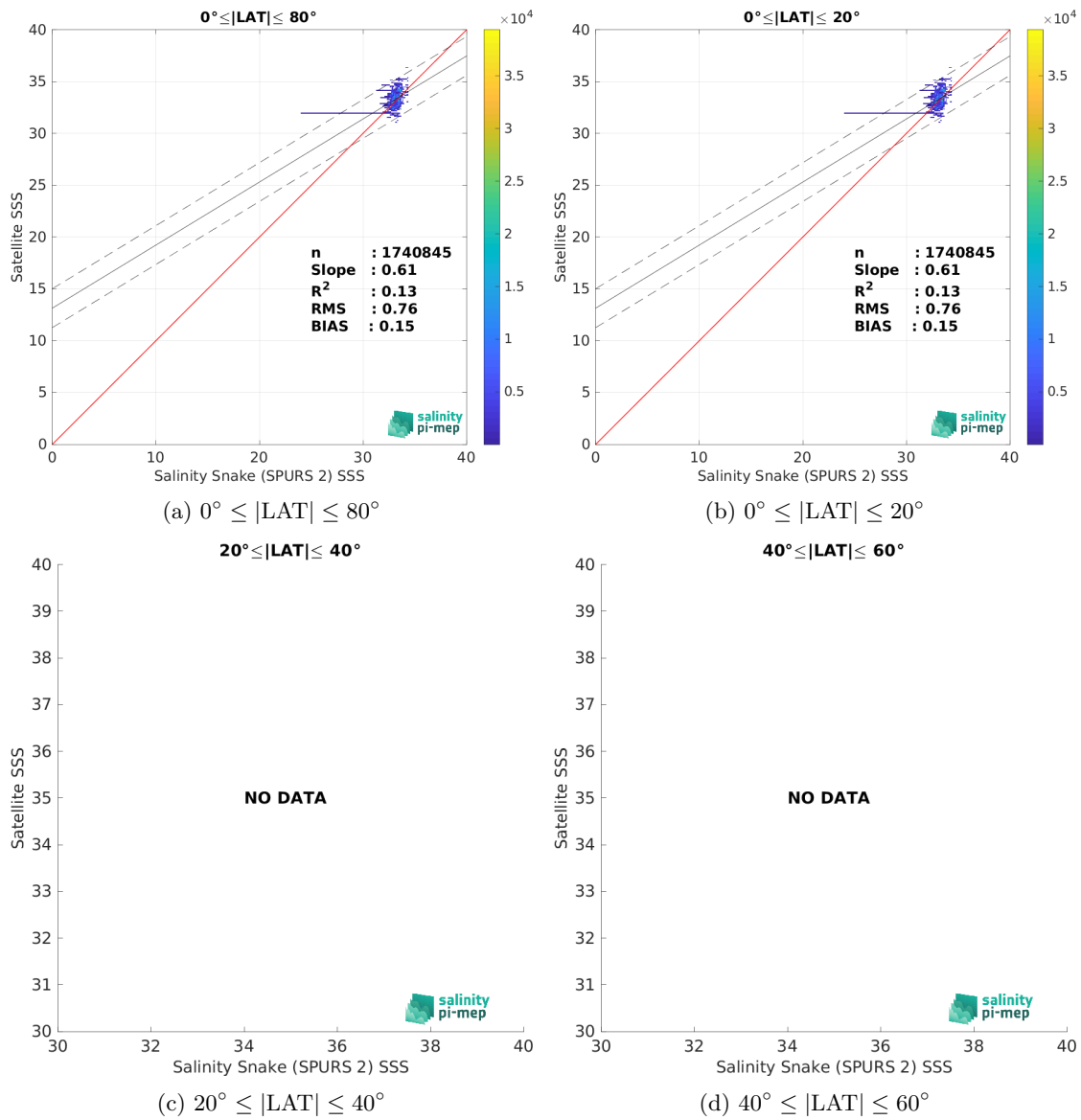
Figure 10: Contour maps of the concentration of SMAP SSS L2 v5.3 - 40 km (RSS) SSS (y-axis) versus Salinity Snake (SPURS 2) SSS (x-axis) at match-up pairs for different latitude bands. For each plot, the red line shows x=y . The black thin and dashed lines indicate a linear fit through the data cloud and the \pm 95\% confidence levels, respectively. The number match-up pairs n , the slope and R^2 coefficient of the linear fit, the root mean square (RMS) and the mean bias between satellite and in situ data are indicated for each latitude band in each plots.
