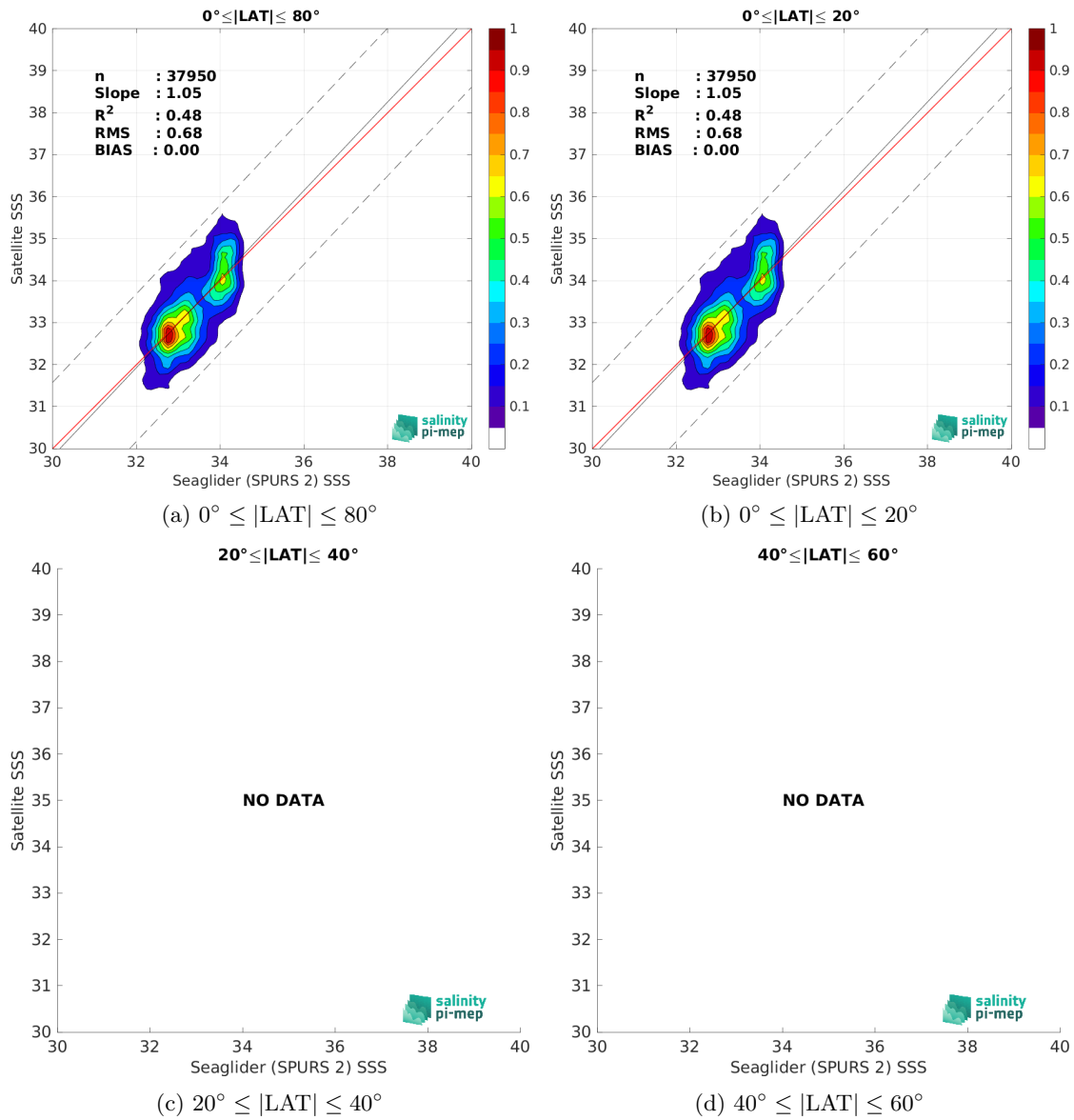
Figure 10: Contour maps of the concentration of SMAP SSS L2 v5.3 - 40 km (RSS) SSS (y-axis) versus Seaglider (SPURS 2) SSS (x-axis) at match-up pairs for different latitude bands. For each plot, the red line shows x=y . The black thin and dashed lines indicate a linear fit through the data cloud and the \pm 95\% confidence levels, respectively. The number match-up pairs n , the slope and R^2 coefficient of the linear fit, the root mean square (RMS) and the mean bias between satellite and in situ data are indicated for each latitude band in each plots.
