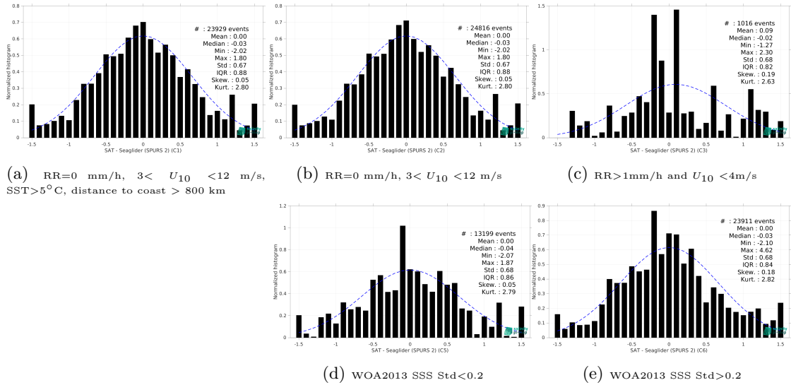
Figure 15: Normalized histogram of \Delta SSS (SMAP SSS L2 v5.3 - 40 km (RSS) - Seaglider (SPURS 2)) for 5 different subdatasets corresponding to: RR=0 mm/h, 3 < U_{10} < 12 m/s, SST > 5°C, distance to coast > 800 km (a), RR=0 mm/h, 3 < U_{10} < 12 m/s (b), RR > 1mm/h and U_{10} < 4 m/s (c), WOA2013 SSS Std < 0.2 (d), WOA2013 SSS Std > 0.2 (e).
