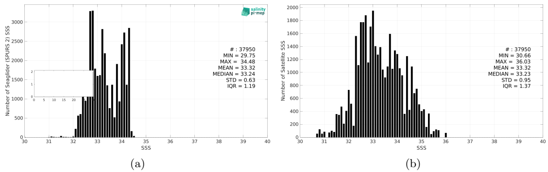
Figure 3: Histograms of SSS from Seaglider (SPURS 2) (a) and SMAP SSS L2 v5.3 - 40 km (RSS) (b) considering all match-up pairs per bins of 0.1 over the SPURS 2 Pi-MEP region and for the full satellite product period.
