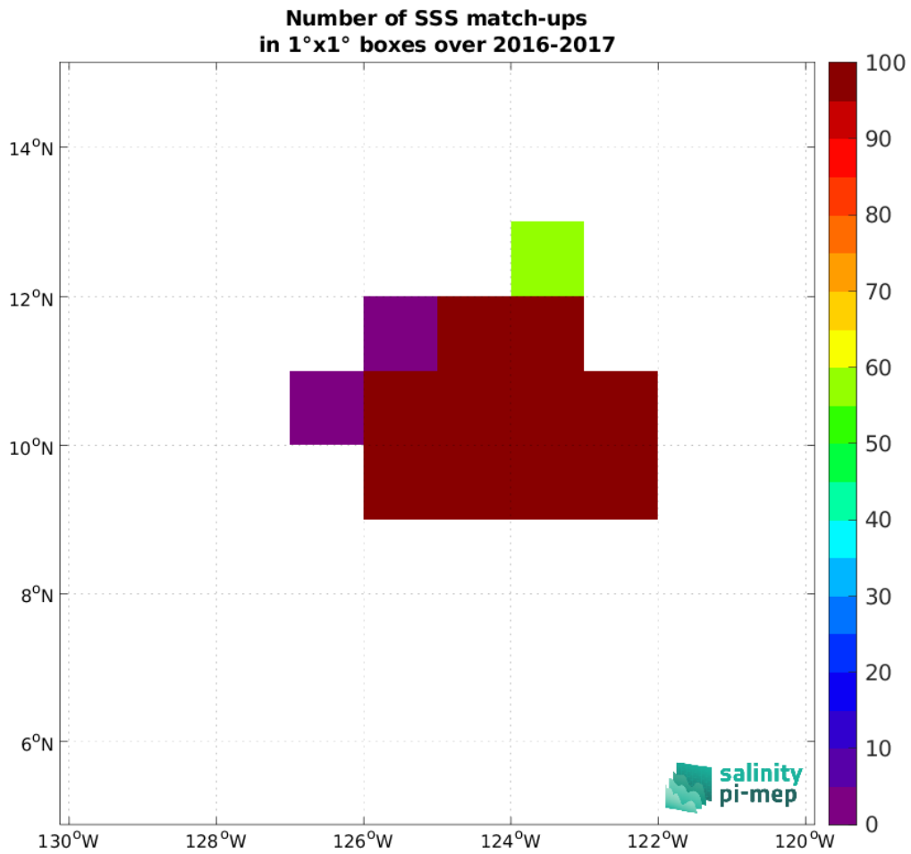
Figure 5: Number of SSS match-ups between Seagliders (SPURS 2) SSS and the SMAP SSS L2 v5.3 - 40 km (RSS) SSS product for the SPURS 2 Pi-MEP region over 1°x1° boxes and for the full satellite product period.
