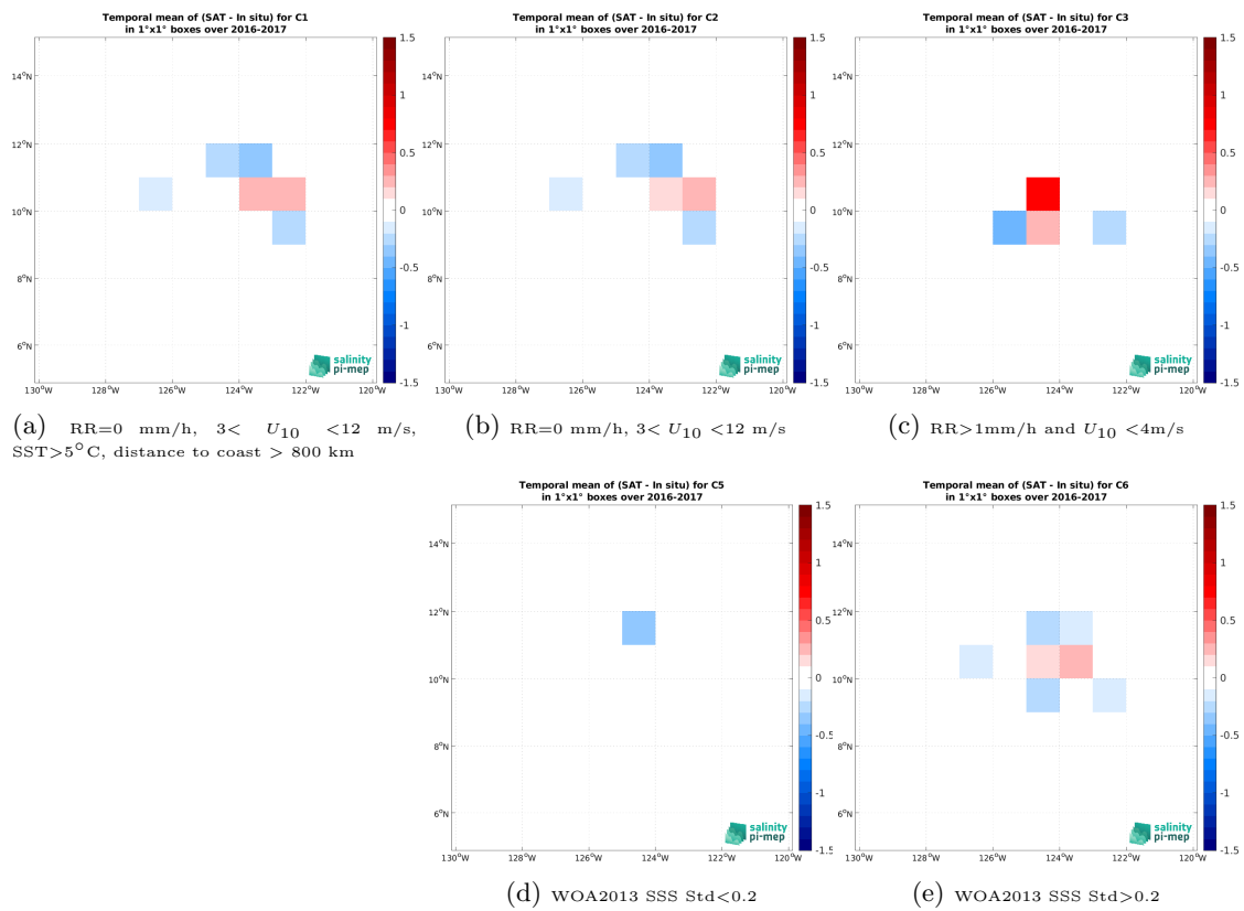
Figure 14: Temporal mean gridded over spatial boxes of size 1^\circ \times 1^\circ of \Delta SSS (SMAP SSS L2 v5.3 - 40 km (RSS) - Seaglider (SPURS 2)) for 5 different subdatasets corresponding to:RR=0 mm/h, 3 < U_{10} < 12 m/s, SST>5°C, distance to coast > 800 km (a), RR=0 mm/h, 3 < U_{10} < 12 m/s (b), RR>1mm/h and U_{10} < 4 m/s (c), WOA2013 SSS Std<0.2 (d), WOA2013 SSS Std>0.2 (e).
