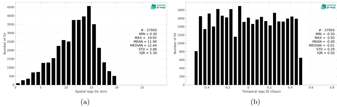
Figure 6: Histograms of the spatial (a) and temporal (b) lags between the location/time of the Seaglider (SPURS 2) measurement and the date of the corresponding SMAP SSS L2 v5.3 - 40 km (RSS) SSS pixel.
