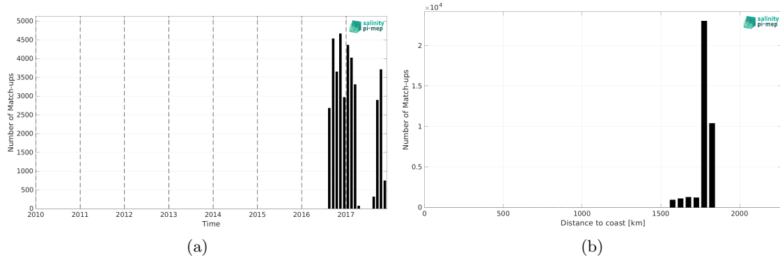
Figure 2: Number of match-ups between Seaglider (SPURS 2) and SMAP SSS L2 v5.3 - 40 km (RSS) SSS as a function of time (a) and as function of the distance to coast (b) over the SPURS 2 Pi-MEP region and for the full satellite product period.
