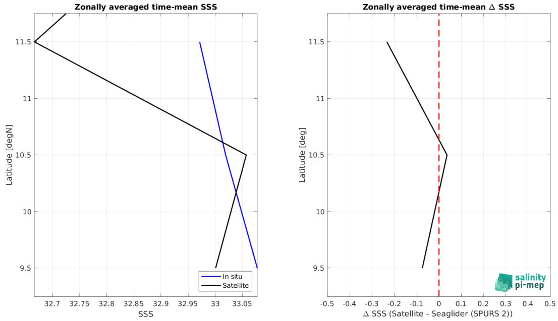
Figure 9: Left panel: Zonal mean SSS from SMAP SSS L2 v5.3 - 40 km (RSS) satellite product (black) and from Seaglider (SPURS 2) (blue). Right panel: Zonal mean of \Delta SSS (Satellite - Seaglider (SPURS 2)) for all the collected Pi-MEP match-up pairs estimated over the full satellite product period.
