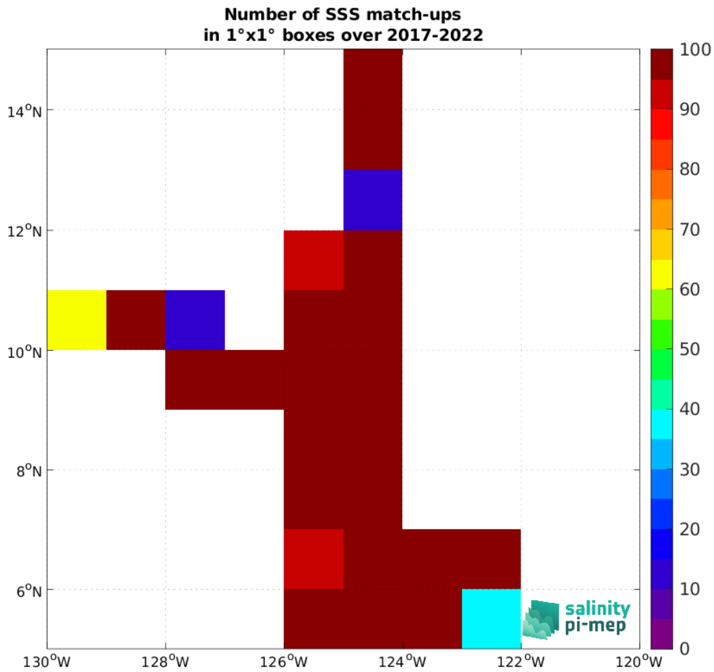
Figure 5: Number of SSS match-ups between Saildrone SSS and the SMAP SSS L2 v5.3 - 40 km (RSS) SSS product for the SPURS 2 Pi-MEP region over 1^\circ \times 1^\circ boxes and for the full satellite product period.
