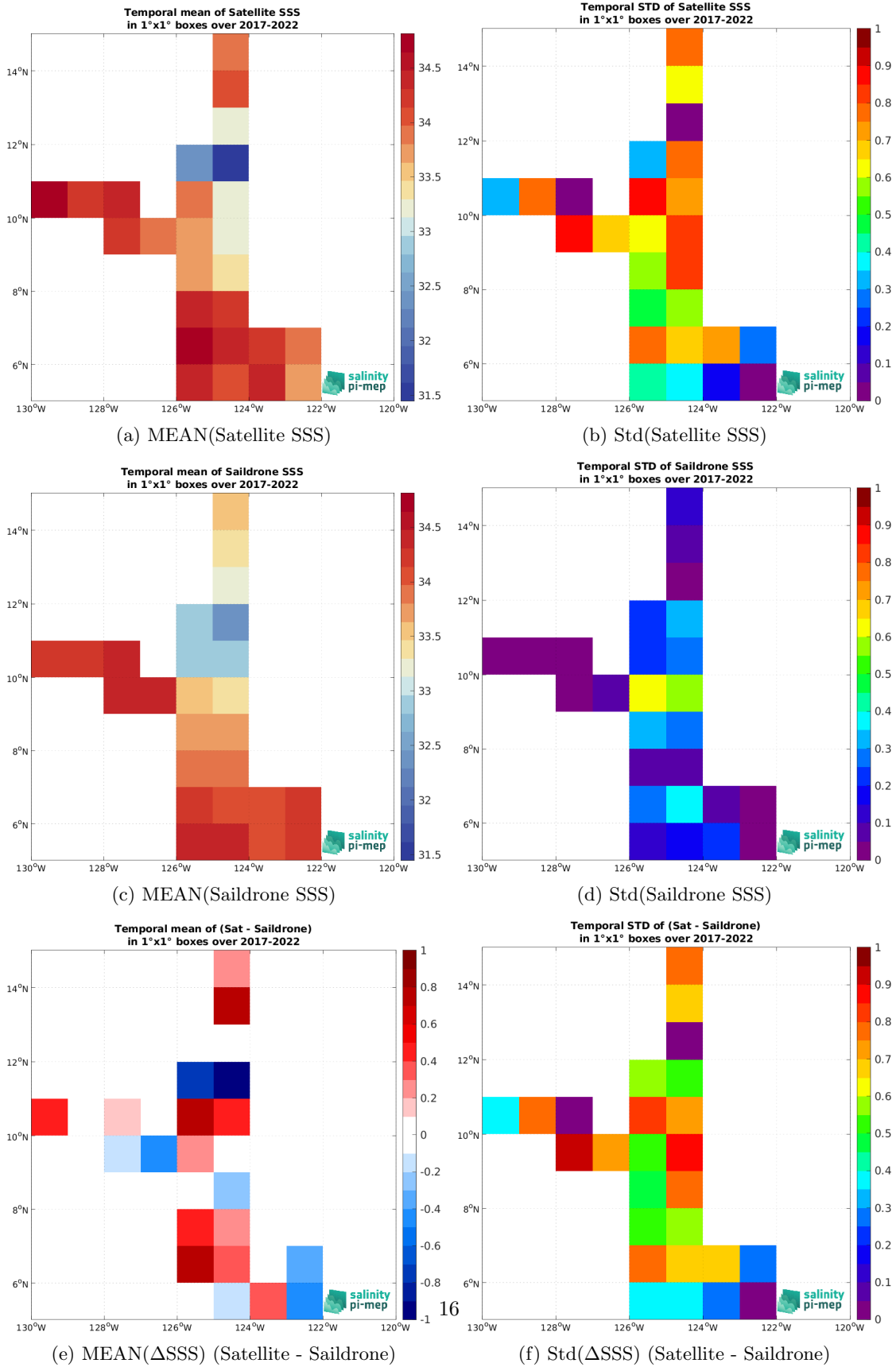
Figure 7: Temporal mean (left) and Std (right) of SSS from SMAP SSS L2 v5.3 - 40 km (RSS) (top), Saildrone (middle), and of \Delta SSS (Satellite - Saildrone). Only match-up pairs are used to generate these maps.
