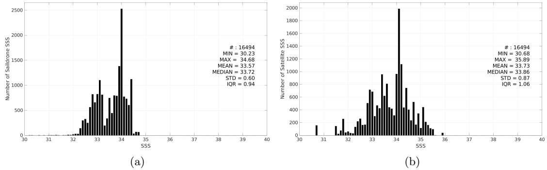
Figure 3: Histograms of SSS from Saildrone (a) and SMAP SSS L2 v5.3 - 40 km (RSS) (b) considering all match-up pairs per bins of 0.1 over the SPURS 2 Pi-MEP region and for the full satellite product period.
