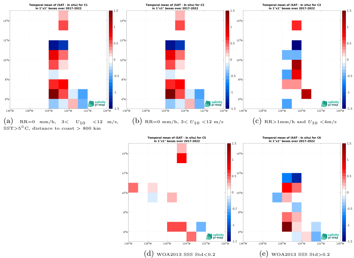
Figure 14: Temporal mean gridded over spatial boxes of size 1^\circ \times 1^\circ of \Delta SSS (SMAP SSS L2 v5.3 - 40 km (RSS) - Sailydrone) for 5 different subdatasets corresponding to:RR=0 mm/h, 3 < U_{10} < 12 m/s, SST > 5°C, distance to coast > 800 km (a), RR=0 mm/h, 3 < U_{10} < 12 m/s (b), RR > 1mm/h and U_{10} < 4 m/s (c), WOA2013 SSS Std < 0.2 (d), WOA2013 SSS Std > 0.2 (e).
