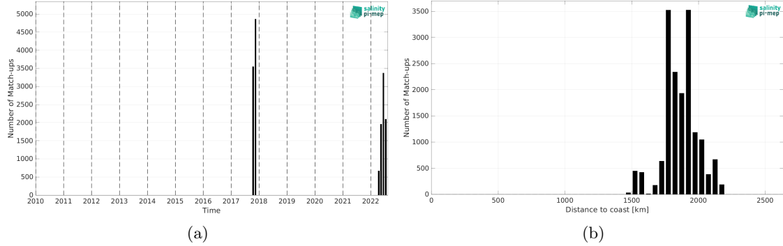
Figure 2: Number of match-ups between Saildrone and SMAP SSS L2 v5.3 - 40 km (RSS) SSS as a function of time (a) and as function of the distance to coast (b) over the SPURS 2 Pi-MEP region and for the full satellite product period.
