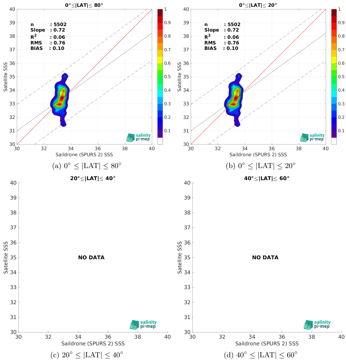
Figure 10: Contour maps of the concentration of SMAP SSS L2 v5.3 - 40 km (RSS) SSS (y-axis) versus Saildrone (SPURS 2) SSS (x-axis) at match-up pairs for different latitude bands. For each plot, the red line shows x=y . The black thin and dashed lines indicate a linear fit through the data cloud and the \pm 95\% confidence levels, respectively. The number match-up pairs n , the slope and R^2 coefficient of the linear fit, the root mean square (RMS) and the mean bias between satellite and in situ data are indicated for each latitude band in each plots.
