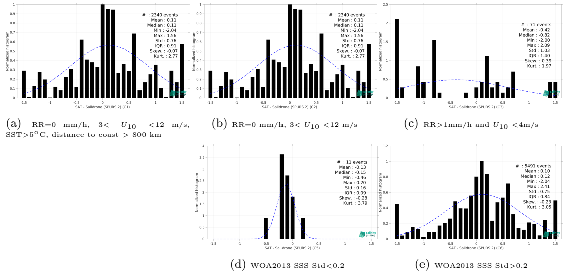
Figure 15: Normalized histogram of \Delta SSS (SMAP SSS L2 v5.3 - 40 km (RSS) - Sailability (SPURS 2)) for 5 different subdatasets corresponding to: RR=0 mm/h, 3 < U_{10} < 12 m/s, SST > 5°C, distance to coast > 800 km (a), RR=0 mm/h, 3 < U_{10} < 12 m/s (b), RR > 1mm/h and U_{10} < 4 m/s (c), WOA2013 SSS Std < 0.2 (d), WOA2013 SSS Std > 0.2 (e).
