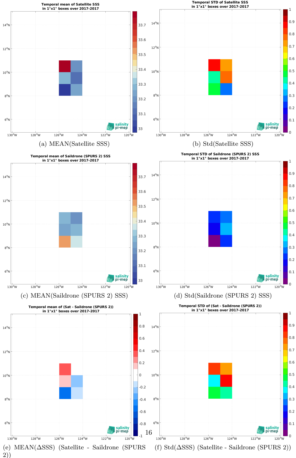
Figure 7: Temporal mean (left) and Std (right) of SSS from SMAP SSS L2 v5.3 - 40 km (RSS) (top), Saildrone (SPURS 2) (middle), and of \Delta SSS (Satellite - Saildrone (SPURS 2)). Only match-up pairs are used to generate these maps.
