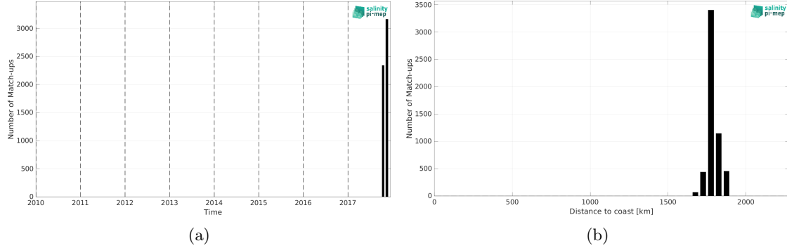
Figure 2: Number of match-ups between Saildrone (SPURS 2) and SMAP SSS L2 v5.3 - 40 km (RSS) SSS as a function of time (a) and as function of the distance to coast (b) over the SPURS 2 Pi-MEP region and for the full satellite product period.
