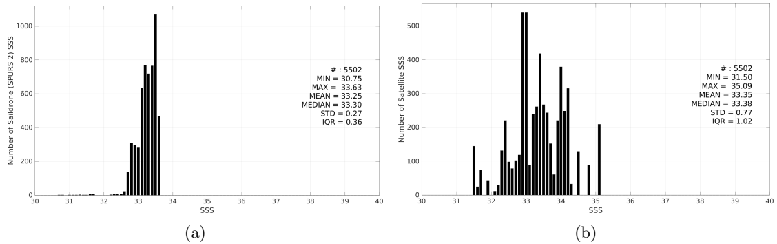
Figure 3: Histograms of SSS from Saildrone (SPURS 2) (a) and SMAP SSS L2 v5.3 - 40 km (RSS) (b) considering all match-up pairs per bins of 0.1 over the SPURS 2 Pi-MEP region and for the full satellite product period.
