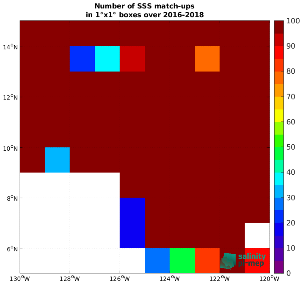
Figure 4: Number of SSS match-ups between Surface drifters SSS and the SMAP SSS L2 v5.3 - 40 km (RSS) SSS product for the SPURS 2 Pi-MEP region over 1°x1° boxes and for the full satellite product period.
