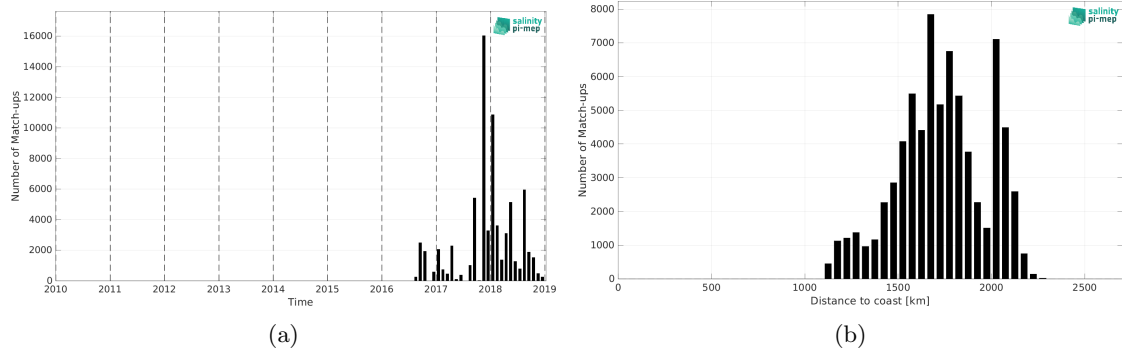
Figure 2: Number of match-ups between Surface drifters and SMAP SSS L2 v5.3 - 40 km (RSS) SSS as a function of time (a) and as function of the distance to coast (b) over the SPURS 2 Pi-MEP region and for the full satellite product period.
