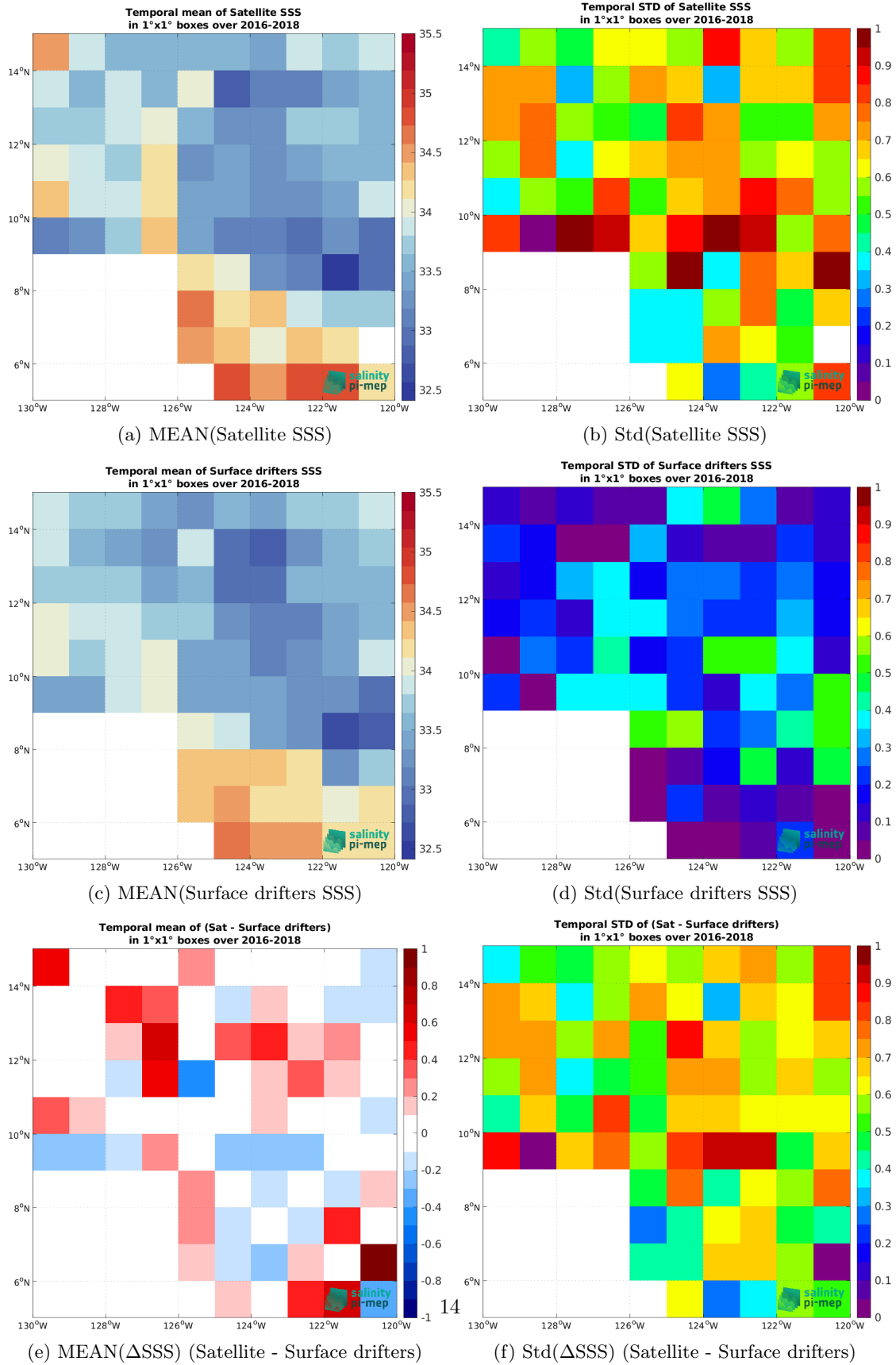
Figure 6: Temporal mean (left) and Std (right) of SSS from SMAP SSS L2 v5.3 - 40 km (RSS) (top), Surface drifters (middle), and of \Delta SSS (Satellite - Surface drifters). Only match-up pairs are used to generate these maps.
