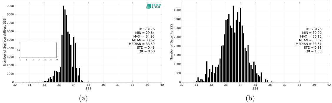
Figure 3: Histograms of SSS from Surface drifters (a) and SMAP SSS L2 v5.3 - 40 km (RSS) (b) considering all match-up pairs per bins of 0.1 over the SPURS 2 Pi-MEP region and for the full satellite product period.
