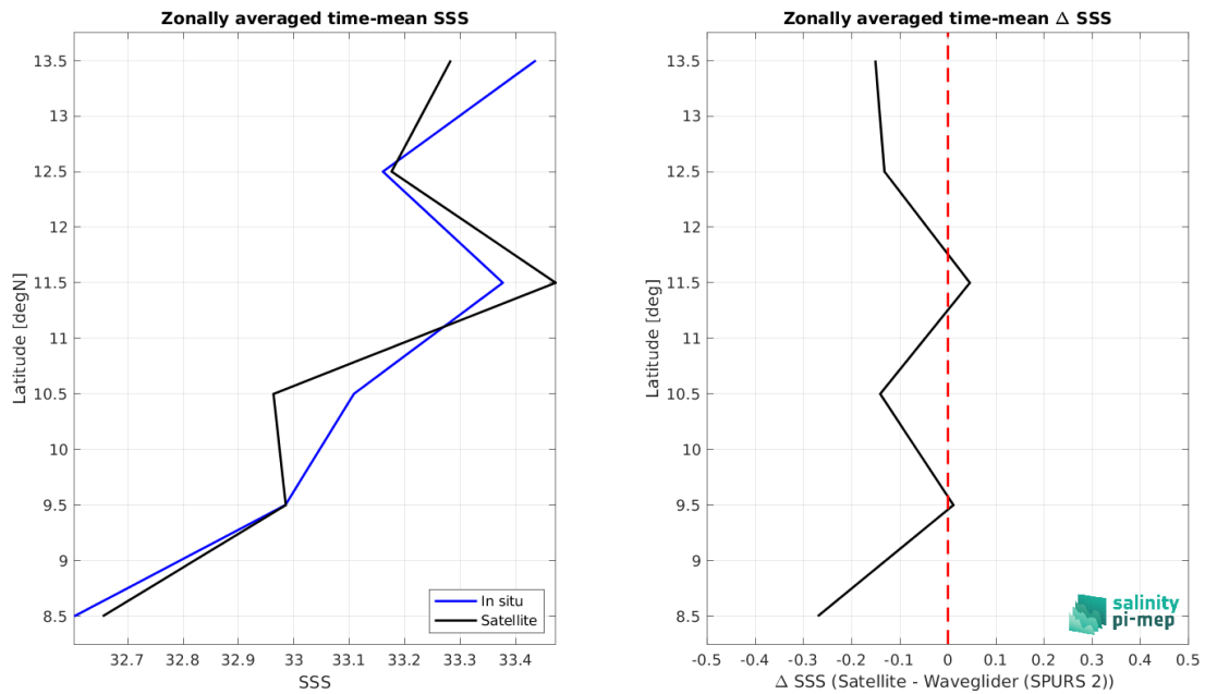
Figure 8: Left panel: Zonal mean SSS from SMAP SSS L2 v5 - 40 km (RSS) satellite product (black) and from Waveglider (SPURS 2) (blue). Right panel: Zonal mean of \Delta SSS (Satellite - Waveglider (SPURS 2)) for all the collected Pi-MEP match-up pairs estimated over the full satellite product period.
