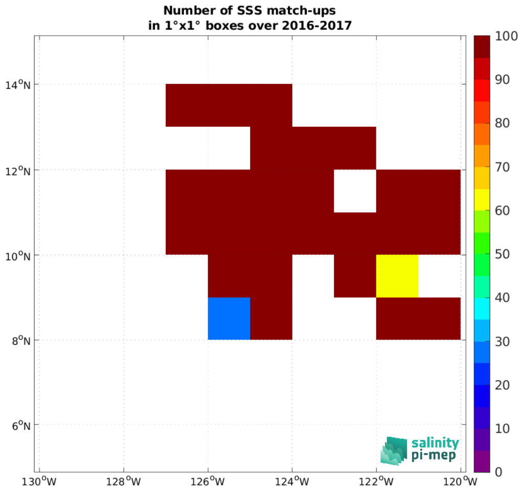
Figure 4: Number of SSS match-ups between Waveglider (SPURS 2) SSS and the SMAP SSS L2 v5 - 40 km (RSS) SSS product for the SPURS 2 Pi-MEP region over 1°x1° boxes and for the full satellite product period.
