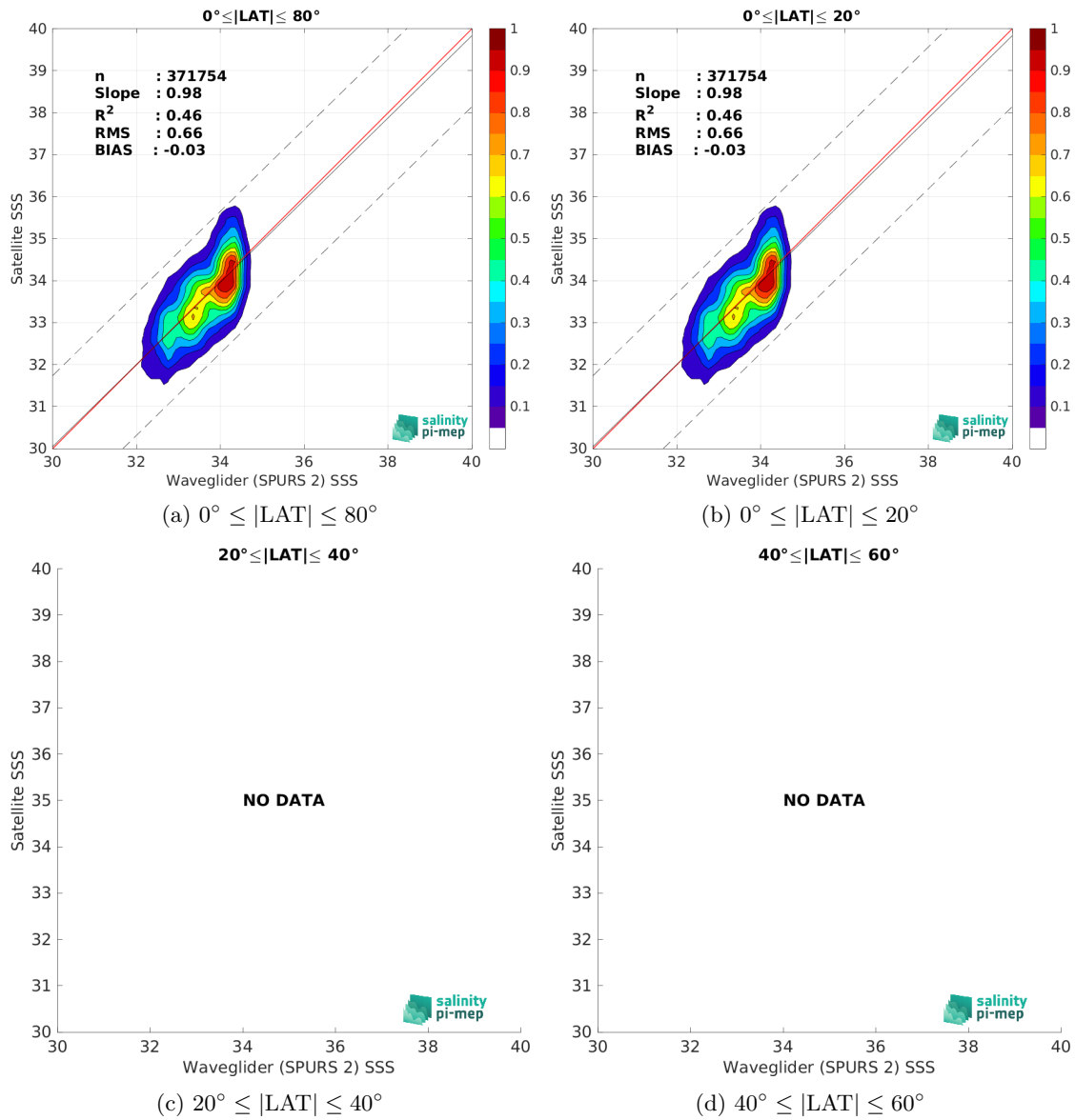
Figure 9: Contour maps of the concentration of SMAP SSS L2 v5 - 40 km (RSS) SSS (y-axis) versus Waveglider (SPURS 2) SSS (x-axis) at match-up pairs for different latitude bands. For each plot, the red line shows x=y . The black thin and dashed lines indicate a linear fit through the data cloud and the \pm 95\% confidence levels, respectively. The number match-up pairs n , the slope and R^2 coefficient of the linear fit, the root mean square (RMS) and the mean bias between satellite and in situ data are indicated for each latitude band in each plots.
