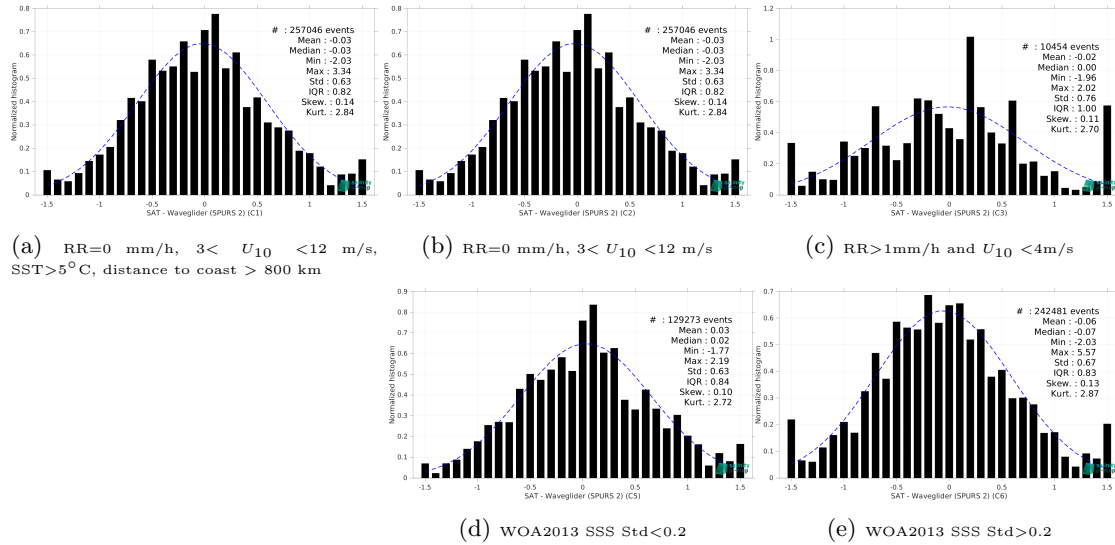
Figure 13: Normalized histogram of \Delta SSS (SMAP SSS L2 v5 - 40 km (RSS) - Waveglider (SPURS 2)) for 5 different subdatasets corresponding to: RR=0 mm/h, 3 < U_{10} < 12 m/s, SST>5°C, distance to coast > 800 km (a), RR=0 mm/h, 3 < U_{10} < 12 m/s (b), RR>1mm/h and U_{10} < 4 m/s (c), WOA2013 SSS Std<0.2 (d), WOA2013 SSS Std>0.2 (e).
