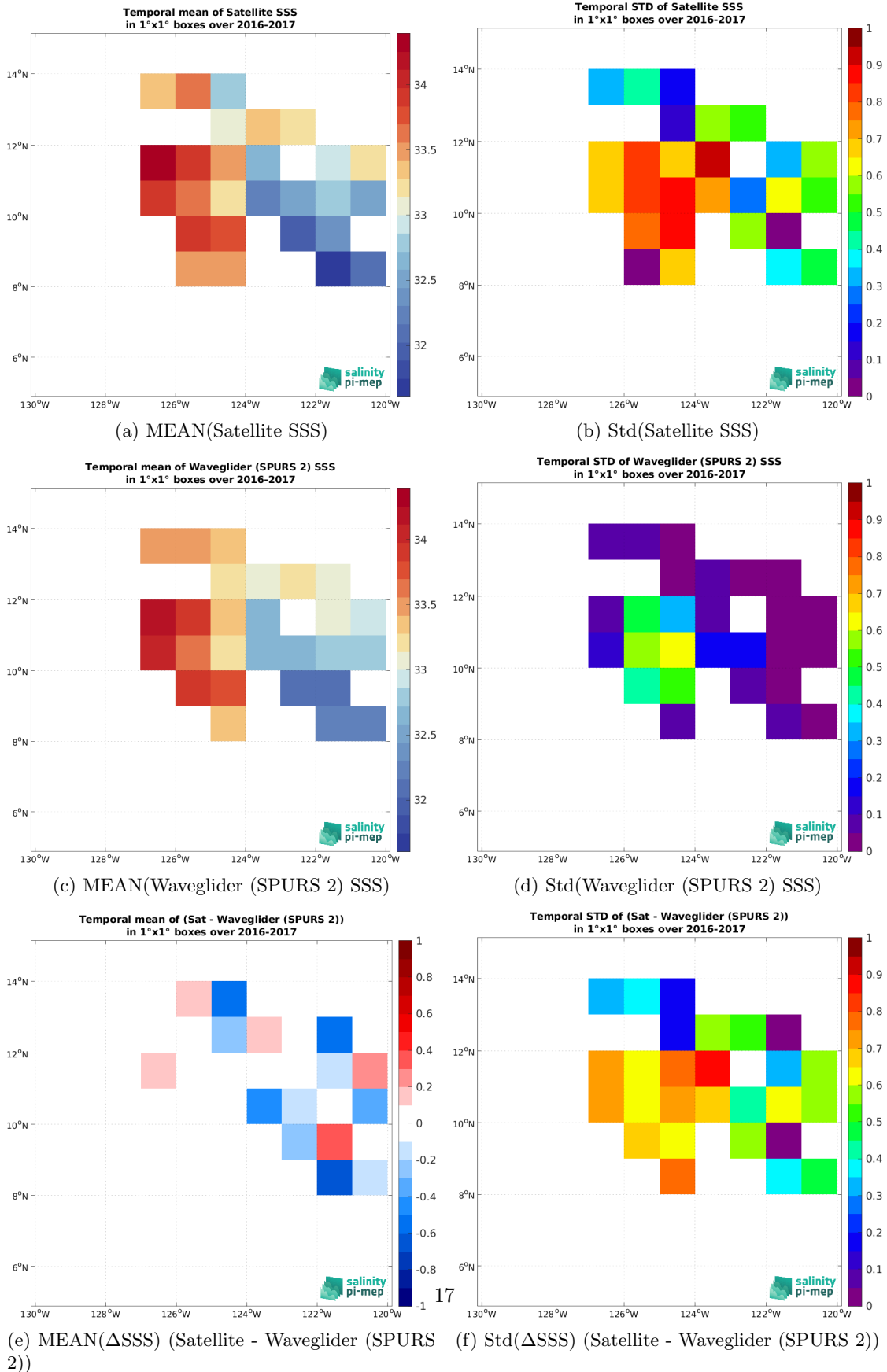
Figure 6: Temporal mean (left) and Std (right) of SSS from SMAP SSS L2 v5 - 40 km (RSS) (top), Waveglider (SPURS 2) (middle), and of \Delta SSS (Satellite - Waveglider (SPURS 2)). Only match-up pairs are used to generate these maps.
