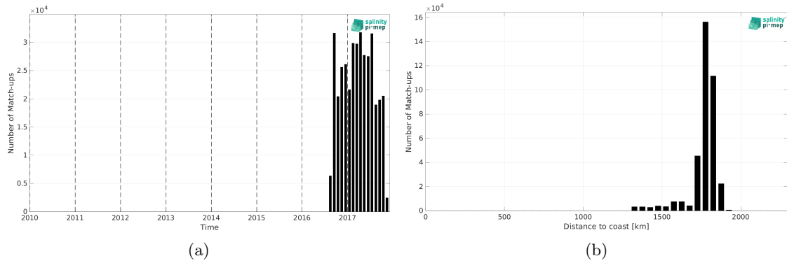
Figure 1: Number of match-ups between Waveglider (SPURS 2) and SMAP SSS L2 v5 - 40 km (RSS) SSS as a function of time (a) and as function of the distance to coast (b) over the SPURS 2 Pi-MEP region and for the full satellite product period.
