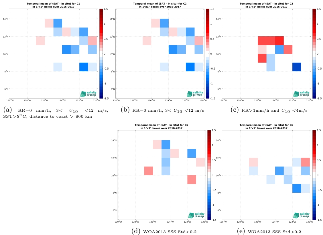
Figure 12: Temporal mean gridded over spatial boxes of size 1^\circ \times 1^\circ of \Delta SSS (SMAP SSS L2 v5 - 40 km (RSS) - Waveglider (SPURS 2)) for 5 different subdatasets corresponding to:RR=0 mm/h, 3 < U_{10} < 12 m/s, SST >5^\circ\text{C} , distance to coast > 800 km (a), RR=0 mm/h, 3 < U_{10} < 12 m/s (b), RR >1 mm/h and U_{10} < 4 m/s (c), WOA2013 SSS Std <0.2 (d), WOA2013 SSS Std >0.2 (e).
