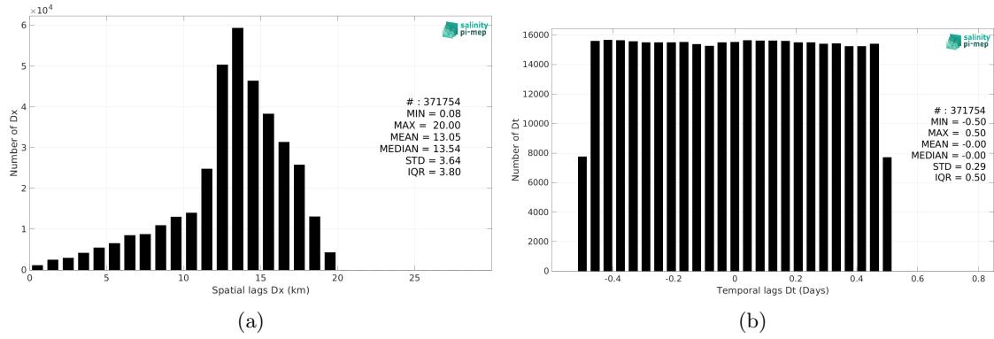
Figure 5: Histograms of the spatial (a) and temporal (b) lags between the location/time of the Waveglider (SPURS 2) measurement and the date of the corresponding SMAP SSS L2 v5 - 40 km (RSS) SSS pixel.
