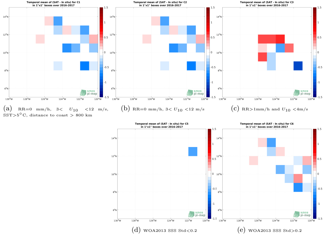
Figure 11: Temporal mean gridded over spatial boxes of size 1^\circ \times 1^\circ of \Delta SSS (SMAP SSS L2 v5 - 40 km (RSS) - Waveglider) for 5 different subdatasets corresponding to: RR=0 mm/h, 3 < U_{10} < 12 m/s, SST >5^\circ\text{C} , distance to coast > 800 km (a), RR=0 mm/h, 3 < U_{10} < 12 m/s (b), RR >1 mm/h and U_{10} < 4 m/s (c), WOA2013 SSS Std <0.2 (d), WOA2013 SSS Std >0.2 (e).
