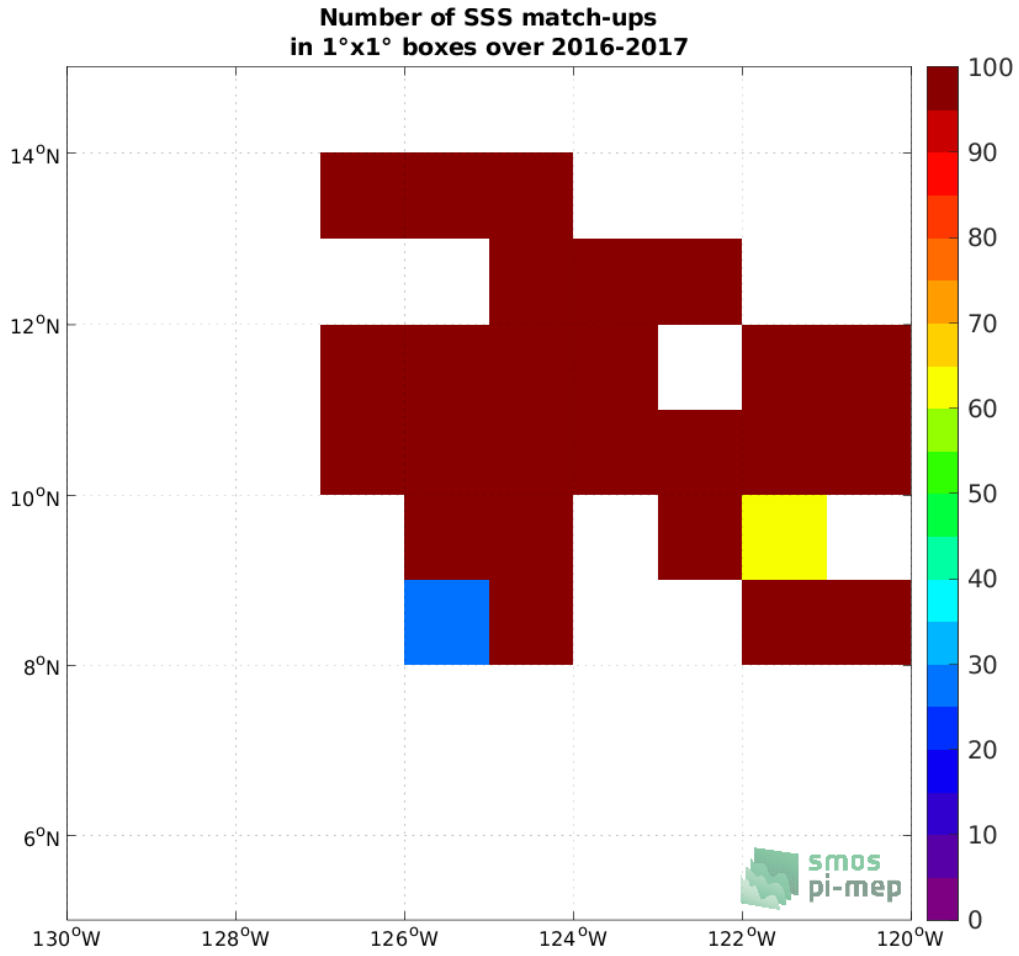
Figure 3: Number of SSS match-ups between Waveglider SSS and the SMAP SSS L2 v5 - 40 km (RSS) SSS product for the SPURS 2 Pi-MEP region over 1°x1° boxes and for the full satellite product period.
