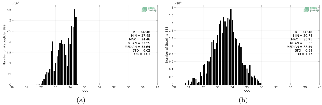
Figure 2: Histograms of SSS from Waveglider (a) and SMAP SSS L2 v5 - 40 km (RSS) (b) considering all match-up pairs per bins of 0.1 over the SPURS 2 Pi-MEP region and for the full satellite product period.
