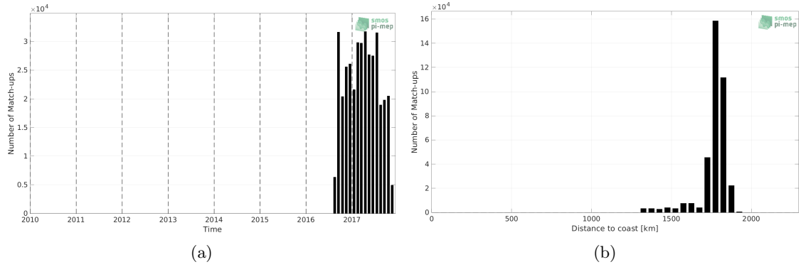
Figure 1: Number of match-ups between Waveglider and SMAP SSS L2 v5 - 40 km (RSS) SSS as a function of time (a) and as function of the distance to coast (b) over the SPURS 2 Pi-MEP region and for the full satellite product period.
