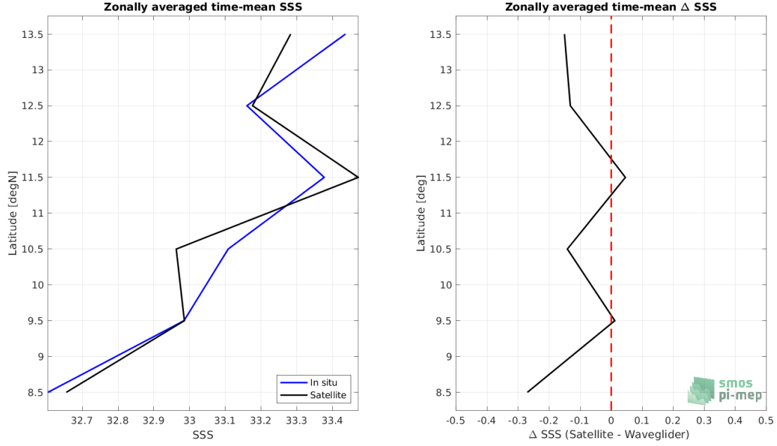
Figure 7: Left panel: Zonal mean SSS from SMAP SSS L2 v5 - 40 km (RSS) satellite product (black) and from Waveglider (blue). Right panel: Zonal mean of \Delta SSS (Satellite - Waveglider) for all the collected Pi-MEP match-up pairs estimated over the full satellite product period.
