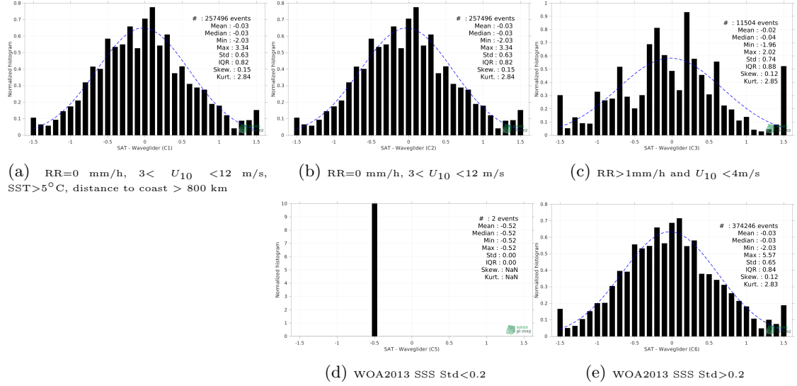
Figure 12: Normalized histogram of \Delta SSS (SMAP SSS L2 v5 - 40 km (RSS) - Waveglider) for 5 different subdatasets corresponding to: RR=0 mm/h, 3 < U_{10} < 12 m/s, SST>5°C, distance to coast > 800 km (a), RR=0 mm/h, 3 < U_{10} < 12 m/s (b), RR>1mm/h and U_{10} < 4 m/s (c), WOA2013 SSS Std<0.2 (d), WOA2013 SSS Std>0.2 (e).
