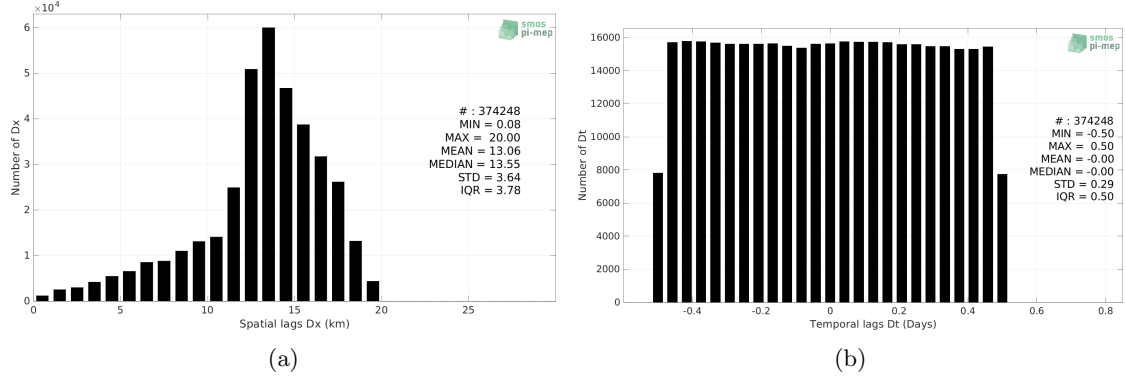
Figure 4: Histograms of the spatial (a) and temporal (b) lags between the location/time of the Waveglider measurement and the date of the corresponding SMAP SSS L2 v5 - 40 km (RSS) SSS pixel.
