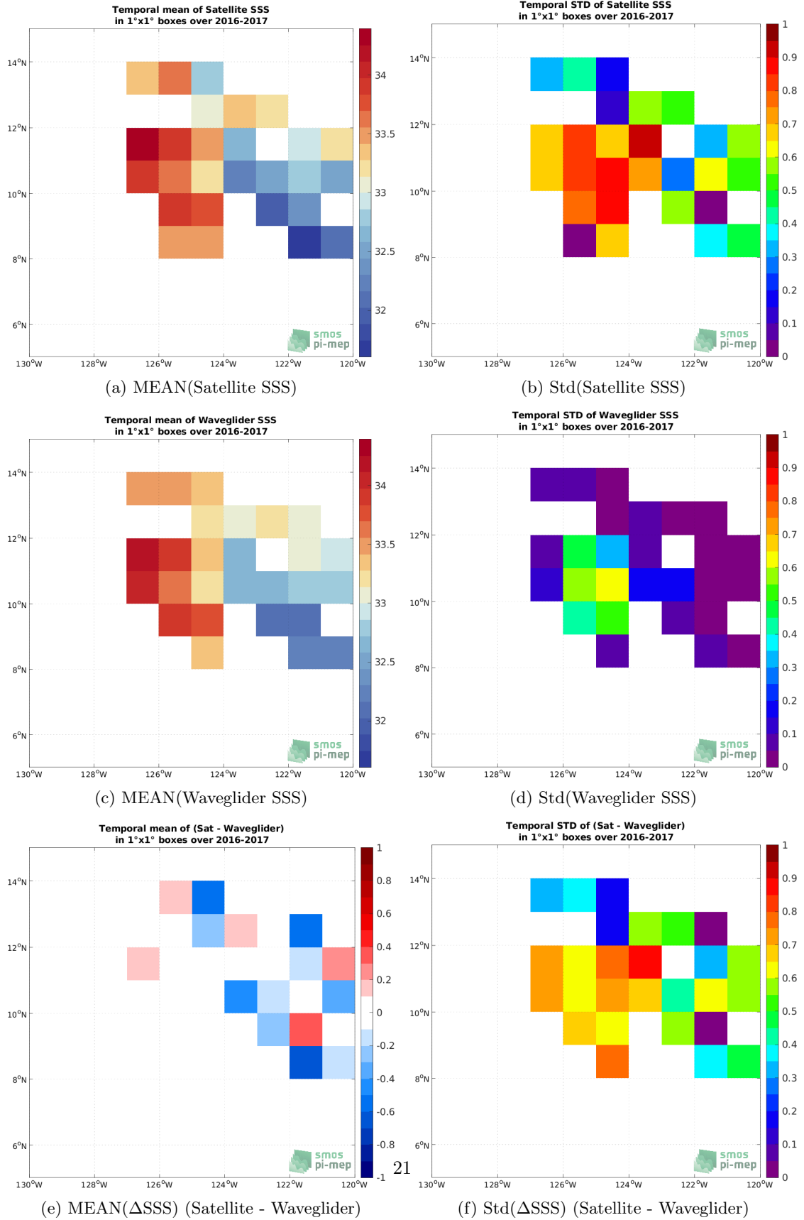
Figure 5: Temporal mean (left) and Std (right) of SSS from SMAP SSS L2 v5 - 40 km (RSS) (top), Waveglider (middle), and of \Delta SSS (Satellite - Waveglider). Only match-up pairs are used to generate these maps.
