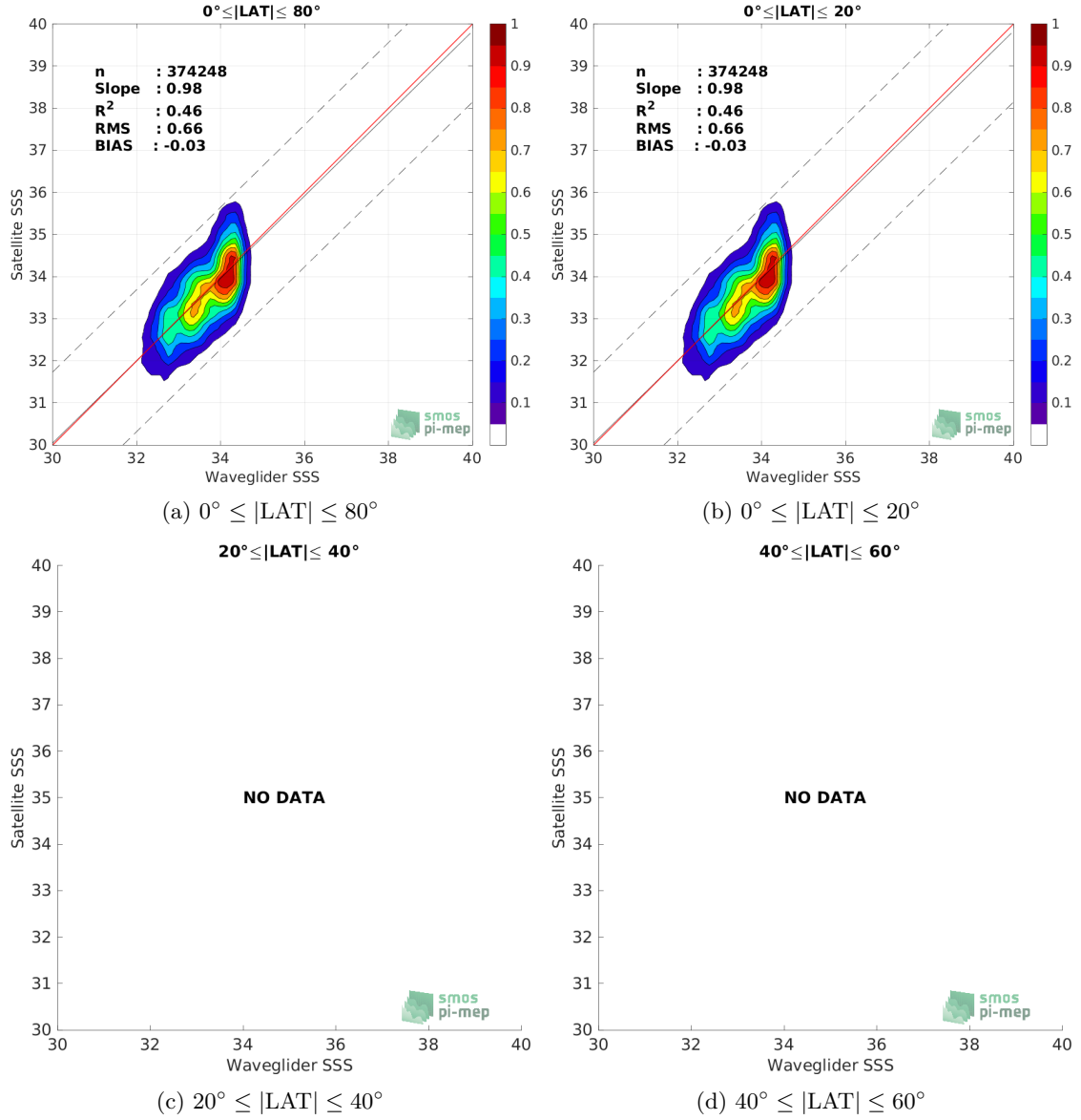
Figure 8: Contour maps of the concentration of SMAP SSS L2 v5 - 40 km (RSS) SSS (y-axis) versus Waveglider SSS (x-axis) at match-up pairs for different latitude bands. For each plot, the red line shows x=y . The black thin and dashed lines indicate a linear fit through the data cloud and the \pm 95\% confidence levels, respectively. The number match-up pairs n , the slope and R^2 coefficient of the linear fit, the root mean square (RMS) and the mean bias between satellite and in situ data are indicated for each latitude band in each plots.
