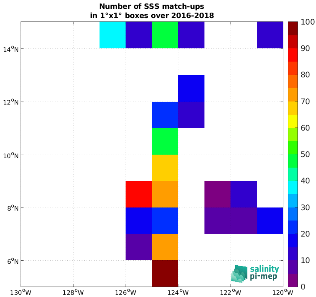
Figure 4: Number of SSS match-ups between TSG (SAMOS) SSS and the SMAP SSS L2 v5 - 40 km (RSS) SSS product for the SPURS 2 Pi-MEP region over 1°x1° boxes and for the full satellite product period.
