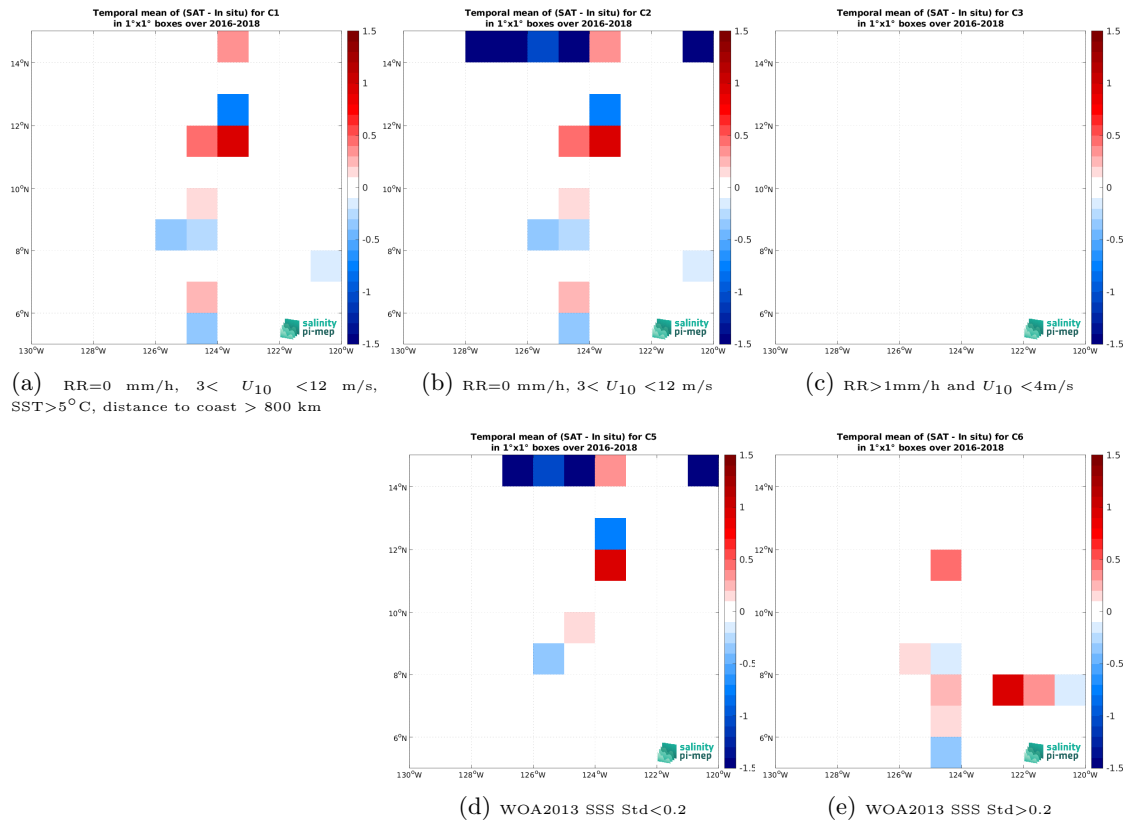
Figure 12: Temporal mean gridded over spatial boxes of size 1^\circ \times 1^\circ of \Delta SSS (SMAP SSS L2 v5 - 40 km (RSS) - TSG (SAMOS)) for 5 different subdatasets corresponding to:RR=0 mm/h, 3 < U_{10} < 12 m/s, SST > 5^\circ\text{C} , distance to coast > 800 km (a), RR=0 mm/h, 3 < U_{10} < 12 m/s (b), RR > 1 mm/h and U_{10} < 4 m/s (c), WOA2013 SSS Std < 0.2 (d), WOA2013 SSS Std > 0.2 (e).
