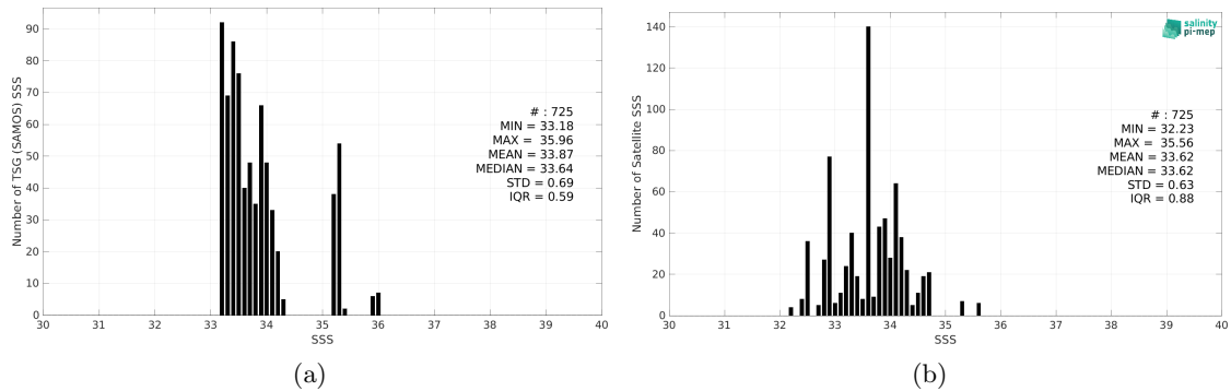
Figure 2: Histograms of SSS from TSG (SAMOS) (a) and SMAP SSS L2 v5 - 40 km (RSS) (b) considering all match-up pairs per bins of 0.1 over the SPURS 2 Pi-MEP region and for the full satellite product period.
