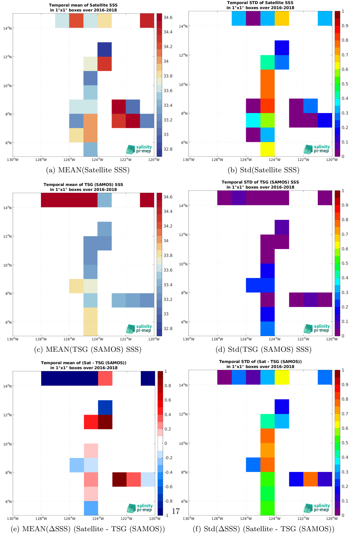
Figure 6: Temporal mean (left) and Std (right) of SSS from SMAP SSS L2 v5 - 40 km (RSS) (top), TSG (SAMOS) (middle), and of \Delta SSS (Satellite - TSG (SAMOS)). Only match-up pairs are used to generate these maps.
