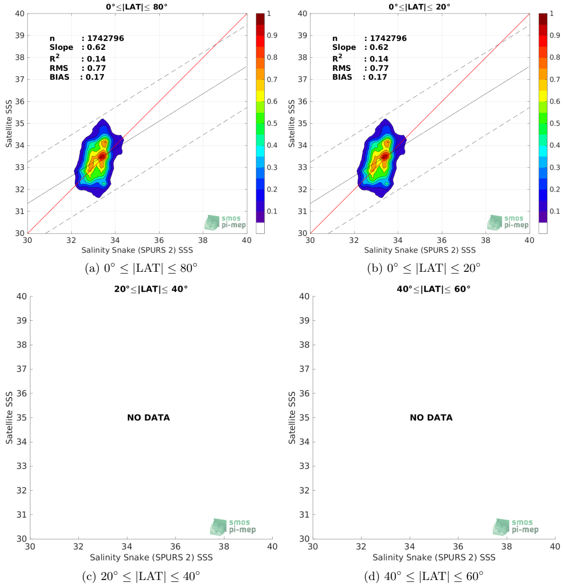
Figure 9: Contour maps of the concentration of SMAP SSS L2 v5 - 40 km (RSS) SSS (y-axis) versus Salinity Snake (SPURS 2) SSS (x-axis) at match-up pairs for different latitude bands. For each plot, the red line shows x=y . The black thin and dashed lines indicate a linear fit through the data cloud and the \pm 95\% confidence levels, respectively. The number match-up pairs n , the slope and R^2 coefficient of the linear fit, the root mean square (RMS) and the mean bias between satellite and in situ data are indicated for each latitude band in each plots.
