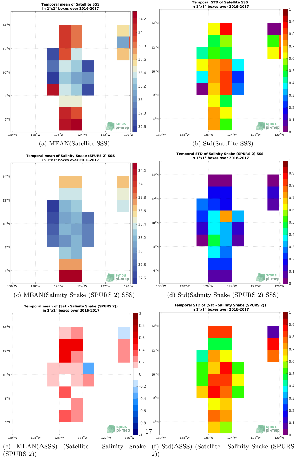
Figure 6: Temporal mean (left) and Std (right) of SSS from SMAP SSS L2 v5 - 40 km (RSS) (top), Salinity Snake (SPURS 2) (middle), and of \Delta SSS (Satellite - Salinity Snake (SPURS 2)). Only match-up pairs are used to generate these maps.
