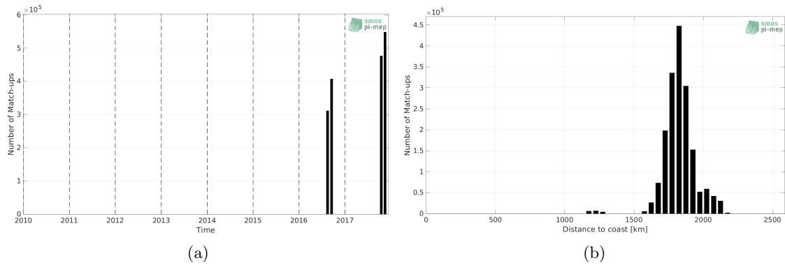
Figure 1: Number of match-ups between Salinity Snake (SPURS 2) and SMAP SSS L2 v5 - 40 km (RSS) SSS as a function of time (a) and as function of the distance to coast (b) over the SPURS 2 Pi-MEP region and for the full satellite product period.
