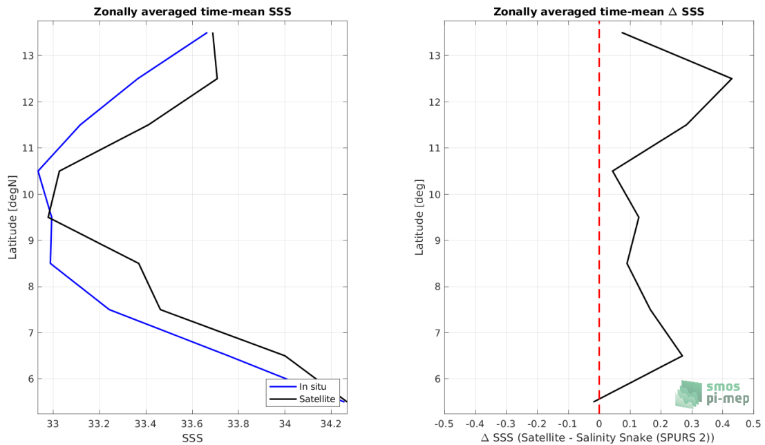
Figure 8: Left panel: Zonal mean SSS from SMAP SSS L2 v5 - 40 km (RSS) satellite product (black) and from Salinity Snake (SPURS 2) (blue). Right panel: Zonal mean of \Delta SSS (Satellite - Salinity Snake (SPURS 2)) for all the collected Pi-MEP match-up pairs estimated over the full satellite product period.
