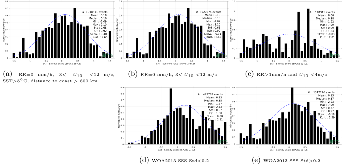
Figure 13: Normalized histogram of \Delta SSS (SMAP SSS L2 v5 - 40 km (RSS) - Salinity Snake (SPURS 2)) for 5 different subdatasets corresponding to: RR=0 mm/h, 3 < U_{10} < 12 m/s, SST > 5°C, distance to coast > 800 km (a), RR=0 mm/h, 3 < U_{10} < 12 m/s (b), RR > 1mm/h and U_{10} < 4 m/s (c), WOA2013 SSS Std < 0.2 (d), WOA2013 SSS Std > 0.2 (e).
