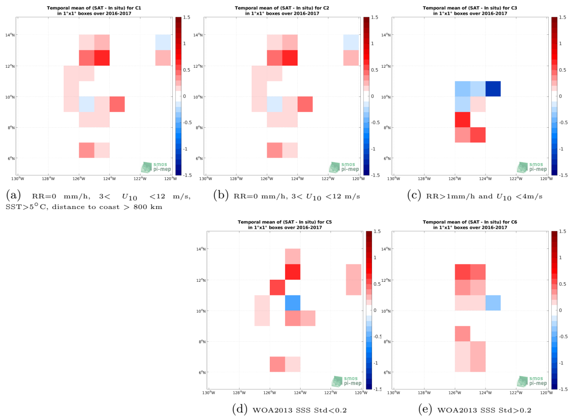
Figure 12: Temporal mean gridded over spatial boxes of size 1^\circ \times 1^\circ of \Delta SSS (SMAP SSS L2 v5 - 40 km (RSS) - Salinity Snake (SPURS 2)) for 5 different subdatasets corresponding to: RR=0 mm/h, 3 < U_{10} < 12 m/s, SST > 5°C, distance to coast > 800 km (a), RR=0 mm/h, 3 < U_{10} < 12 m/s (b), RR > 1mm/h and U_{10} < 4 m/s (c), WOA2013 SSS Std < 0.2 (d), WOA2013 SSS Std > 0.2 (e).
