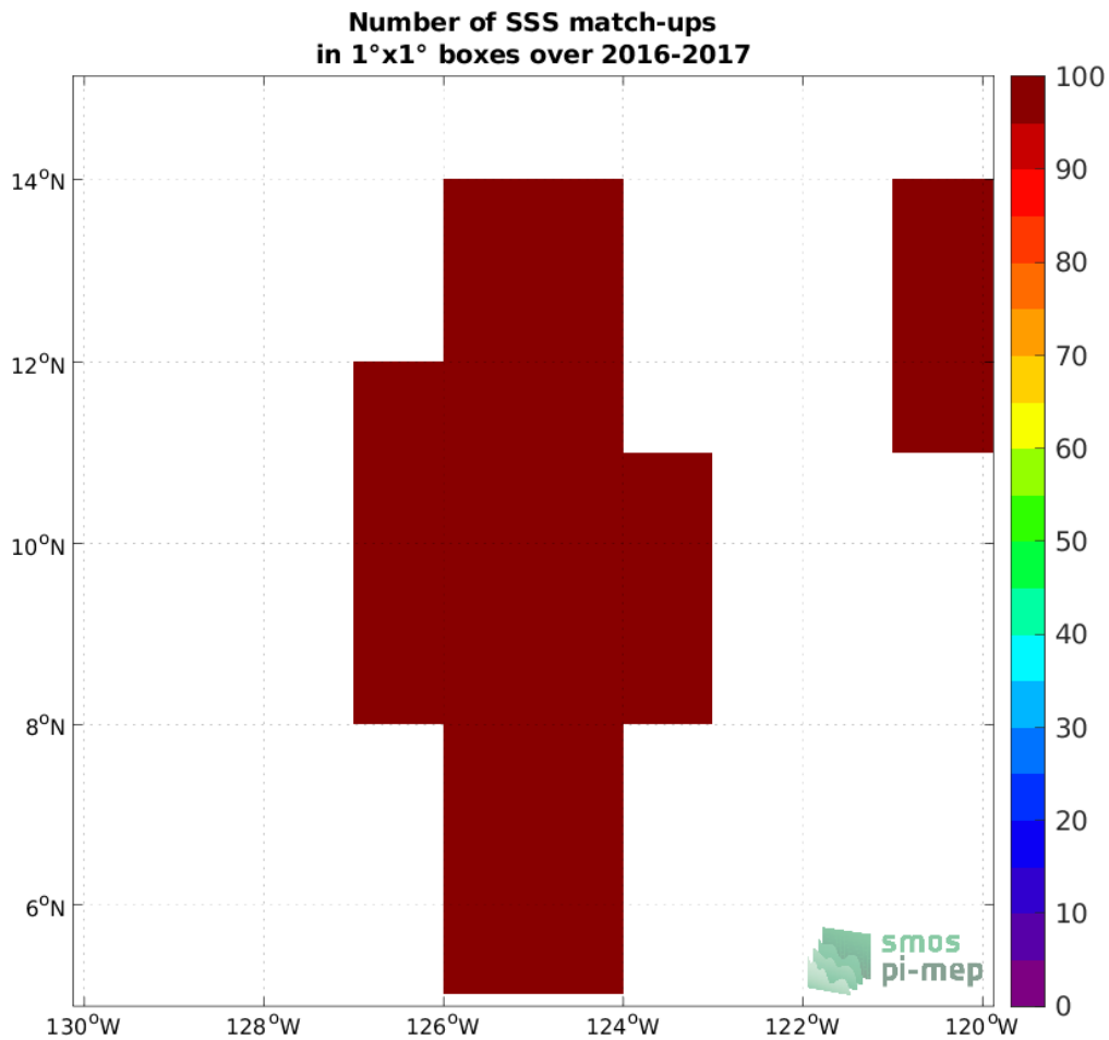
Figure 4: Number of SSS match-ups between Salinity Snake (SPURS 2) SSS and the SMAP SSS L2 v5 - 40 km (RSS) SSS product for the SPURS 2 Pi-MEP region over 1°x1° boxes and for the full satellite product period.
