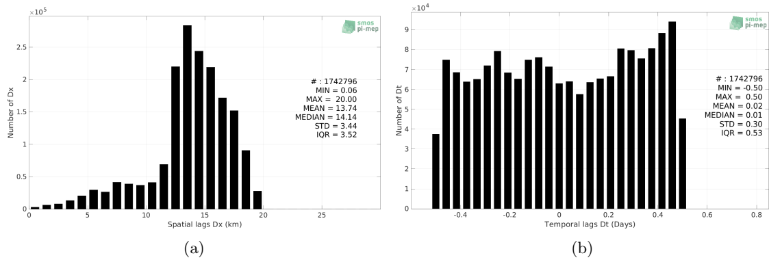
Figure 5: Histograms of the spatial (a) and temporal (b) lags between the location/time of the Salinity Snake (SPURS 2) measurement and the date of the corresponding SMAP SSS L2 v5 - 40 km (RSS) SSS pixel.
