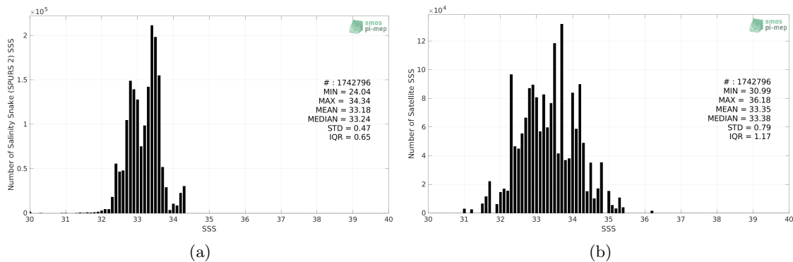
Figure 2: Histograms of SSS from Salinity Snake (SPURS 2) (a) and SMAP SSS L2 v5 - 40 km (RSS) (b) considering all match-up pairs per bins of 0.1 over the SPURS 2 Pi-MEP region and for the full satellite product period.
