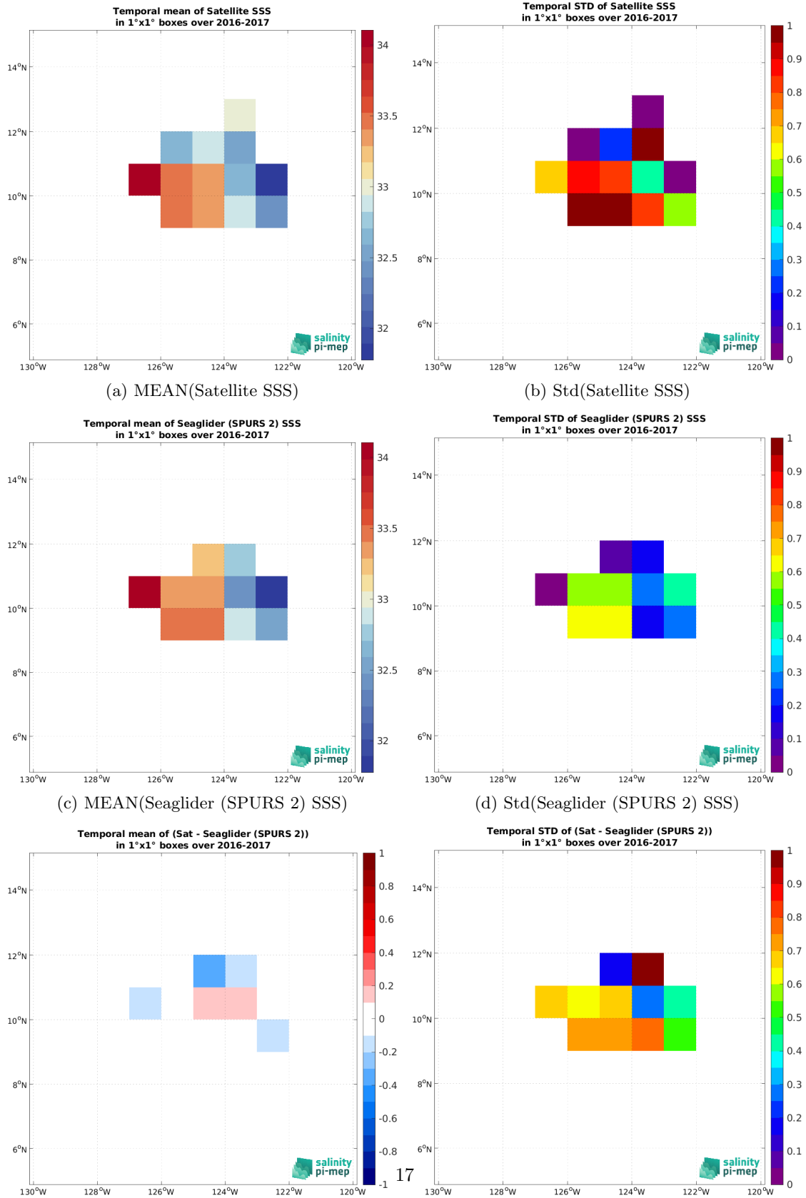
Figure 6: Temporal mean (left) and Std (right) of SSS from SMAP SSS L2 v5 - 40 km (RSS) (top), Seaglider (SPURS 2) (middle), and of \Delta SSS (Satellite - Seaglider (SPURS 2)). Only match-up pairs are used to generate these maps.
