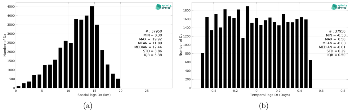
Figure 5: Histograms of the spatial (a) and temporal (b) lags between the location/time of the Seaglider (SPURS 2) measurement and the date of the corresponding SMAP SSS L2 v5 - 40 km (RSS) SSS pixel.
