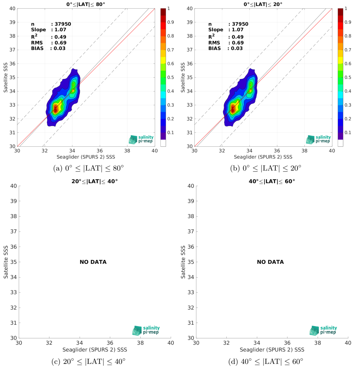
Figure 9: Contour maps of the concentration of SMAP SSS L2 v5 - 40 km (RSS) SSS (y-axis) versus Seaglider (SPURS 2) SSS (x-axis) at match-up pairs for different latitude bands. For each plot, the red line shows x=y . The black thin and dashed lines indicate a linear fit through the data cloud and the \pm 95\% confidence levels, respectively. The number match-up pairs n , the slope and R^2 coefficient of the linear fit, the root mean square (RMS) and the mean bias between satellite and in situ data are indicated for each latitude band in each plots.
