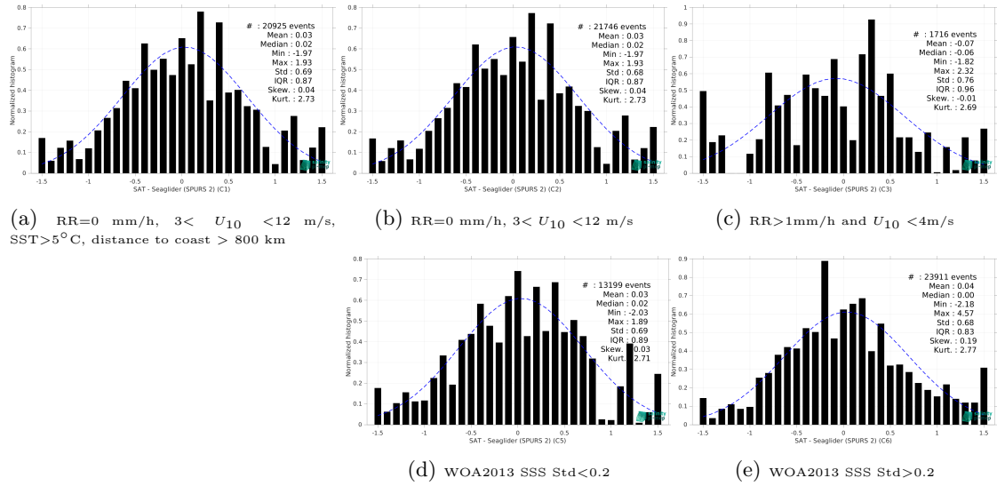
Figure 13: Normalized histogram of \Delta SSS (SMAP SSS L2 v5 - 40 km (RSS) - Seaglider (SPURS 2)) for 5 different subdatasets corresponding to: RR=0 mm/h, 3 < U_{10} < 12 m/s, SST>5°C, distance to coast > 800 km (a), RR=0 mm/h, 3 < U_{10} < 12 m/s (b), RR>1mm/h and U_{10} < 4 m/s (c), WOA2013 SSS Std<0.2 (d), WOA2013 SSS Std>0.2 (e).
