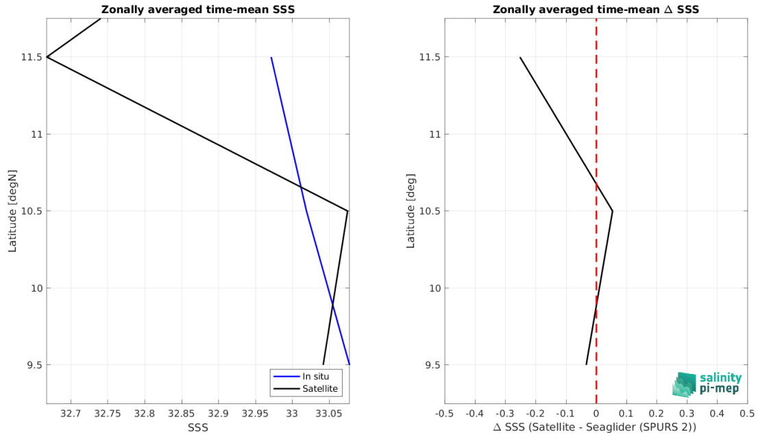
Figure 8: Left panel: Zonal mean SSS from SMAP SSS L2 v5 - 40 km (RSS) satellite product (black) and from Seaglider (SPURS 2) (blue). Right panel: Zonal mean of \Delta SSS (Satellite - Seaglider (SPURS 2)) for all the collected Pi-MEP match-up pairs estimated over the full satellite product period.
