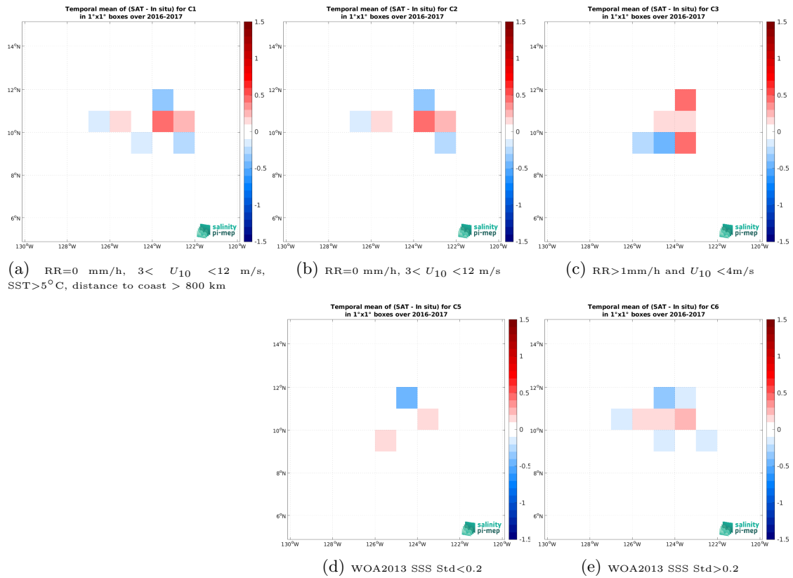
Figure 12: Temporal mean gridded over spatial boxes of size 1^\circ \times 1^\circ of \Delta SSS (SMAP SSS L2 v5 - 40 km (RSS) - Seaglider (SPURS 2)) for 5 different subdatasets corresponding to:RR=0 mm/h, 3 < U_{10} < 12 m/s, SST >5^\circ\text{C} , distance to coast > 800 km (a), RR=0 mm/h, 3 < U_{10} < 12 m/s (b), RR >1 mm/h and U_{10} < 4 m/s (c), WOA2013 SSS Std <0.2 (d), WOA2013 SSS Std >0.2 (e).
