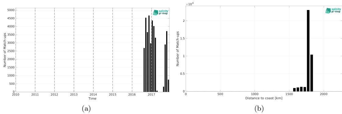
Figure 1: Number of match-ups between Seaglider (SPURS 2) and SMAP SSS L2 v5 - 40 km (RSS) SSS as a function of time (a) and as function of the distance to coast (b) over the SPURS 2 Pi-MEP region and for the full satellite product period.
