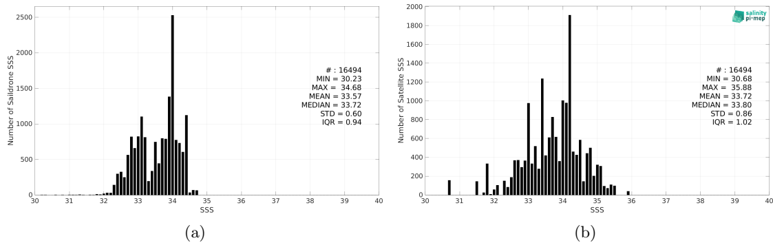
Figure 2: Histograms of SSS from Sairdrone (a) and SMAP SSS L2 v5 - 40 km (RSS) (b) considering all match-up pairs per bins of 0.1 over the SPURS 2 Pi-MEP region and for the full satellite product period.
