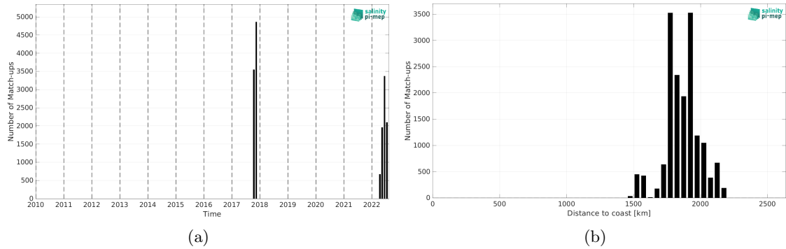
Figure 1: Number of match-ups between Sairdrone and SMAP SSS L2 v5 - 40 km (RSS) SSS as a function of time (a) and as function of the distance to coast (b) over the SPURS 2 Pi-MEP region and for the full satellite product period.
