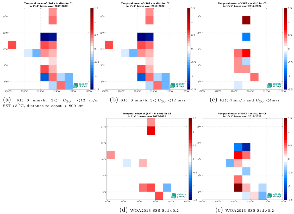
Figure 12: Temporal mean gridded over spatial boxes of size 1^\circ \times 1^\circ of \Delta SSS (SMAP SSS L2 v5 - 40 km (RSS) - Sairdrone) for 5 different subdatasets corresponding to:RR=0 mm/h, 3 < U_{10} < 12 m/s, SST >5^\circ\text{C} , distance to coast > 800 km (a), RR=0 mm/h, 3 < U_{10} < 12 m/s (b), RR >1 mm/h and U_{10} < 4 m/s (c), WOA2013 SSS Std <0.2 (d), WOA2013 SSS Std >0.2 (e).
