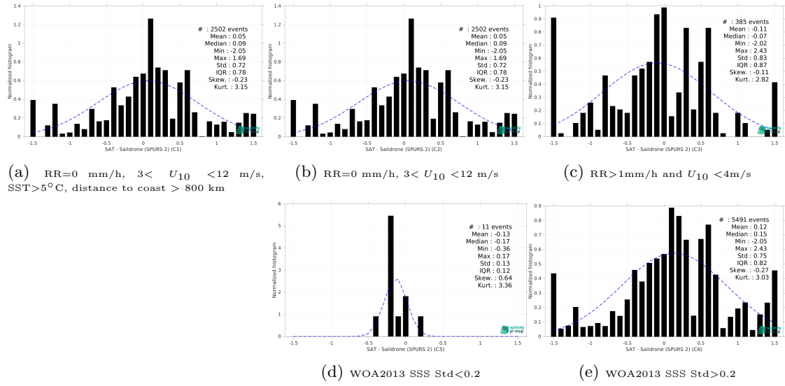
Figure 13: Normalized histogram of \Delta SSS (SMAP SSS L2 v5 - 40 km (RSS) - Saildrone (SPURS 2)) for 5 different subdatasets corresponding to: RR=0 mm/h, 3 < U_{10} < 12 m/s, SST > 5°C, distance to coast > 800 km (a), RR=0 mm/h, 3 < U_{10} < 12 m/s (b), RR > 1mm/h and U_{10} < 4 m/s (c), WOA2013 SSS Std < 0.2 (d), WOA2013 SSS Std > 0.2 (e).
