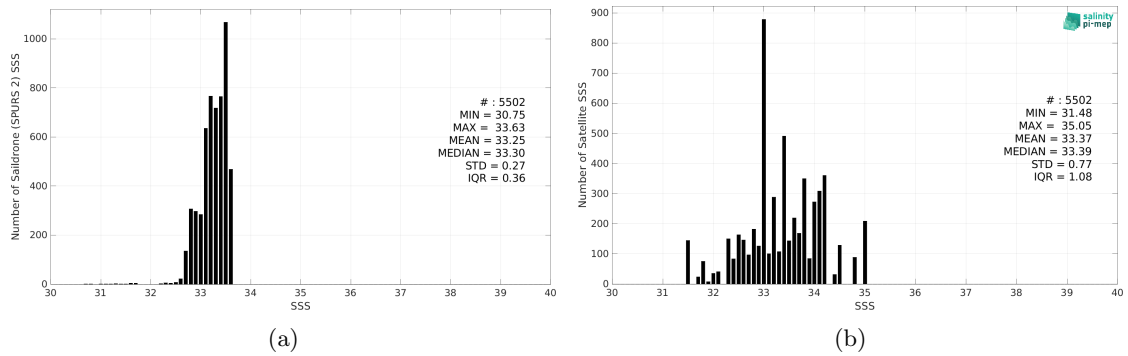
Figure 2: Histograms of SSS from Saildrone (SPURS 2) (a) and SMAP SSS L2 v5 - 40 km (RSS) (b) considering all match-up pairs per bins of 0.1 over the SPURS 2 Pi-MEP region and for the full satellite product period.
