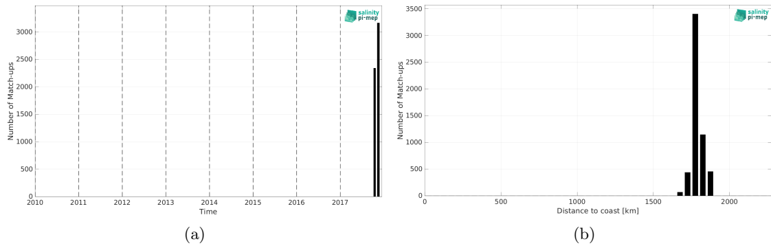
Figure 1: Number of match-ups between Saildrone (SPURS 2) and SMAP SSS L2 v5 - 40 km (RSS) SSS as a function of time (a) and as function of the distance to coast (b) over the SPURS 2 Pi-MEP region and for the full satellite product period.
