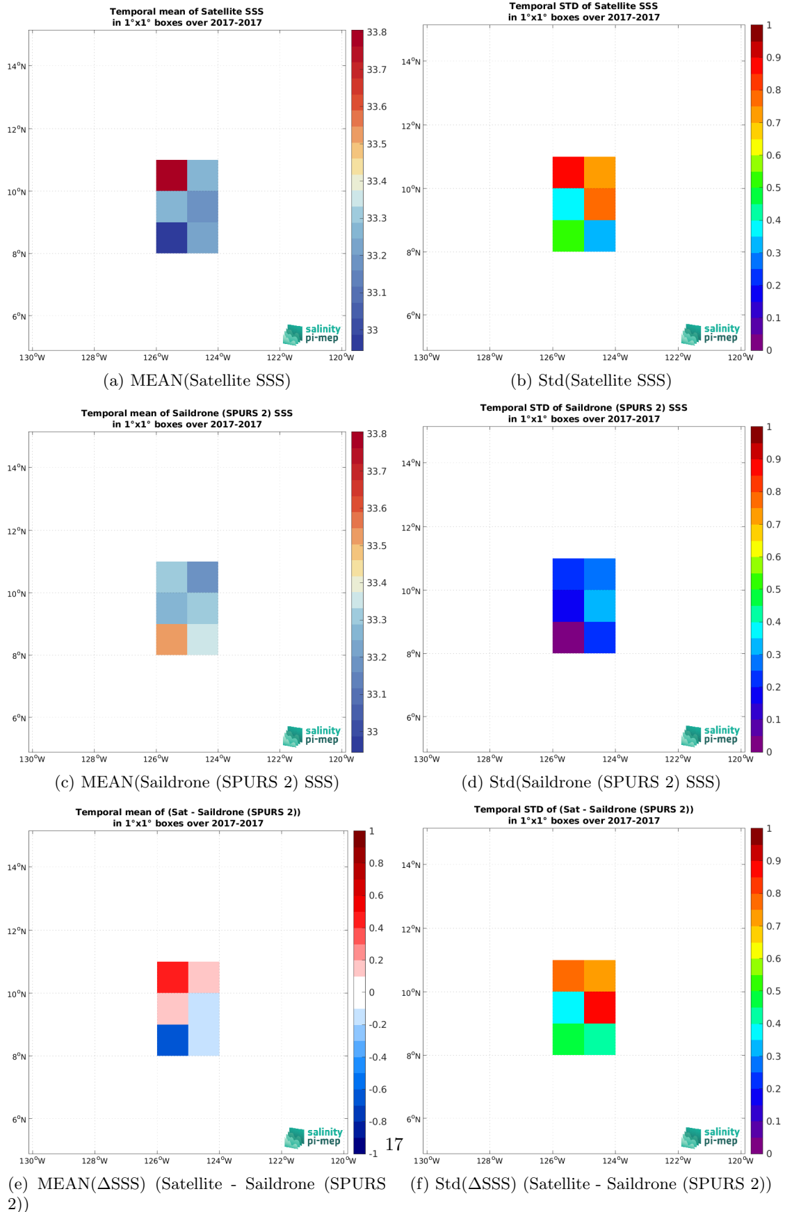
Figure 6: Temporal mean (left) and Std (right) of SSS from SMAP SSS L2 v5 - 40 km (RSS) (top), Saildrone (SPURS 2) (middle), and of \Delta SSS (Satellite - Saildrone (SPURS 2)). Only match-up pairs are used to generate these maps.
