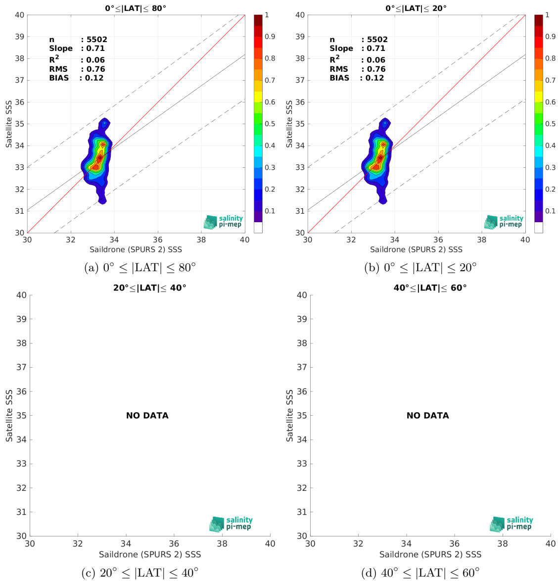
Figure 9: Contour maps of the concentration of SMAP SSS L2 v5 - 40 km (RSS) SSS (y-axis) versus Saildrone (SPURS 2) SSS (x-axis) at match-up pairs for different latitude bands. For each plot, the red line shows x=y . The black thin and dashed lines indicate a linear fit through the data cloud and the \pm 95\% confidence levels, respectively. The number match-up pairs n , the slope and R^2 coefficient of the linear fit, the root mean square (RMS) and the mean bias between satellite and in situ data are indicated for each latitude band in each plots.
