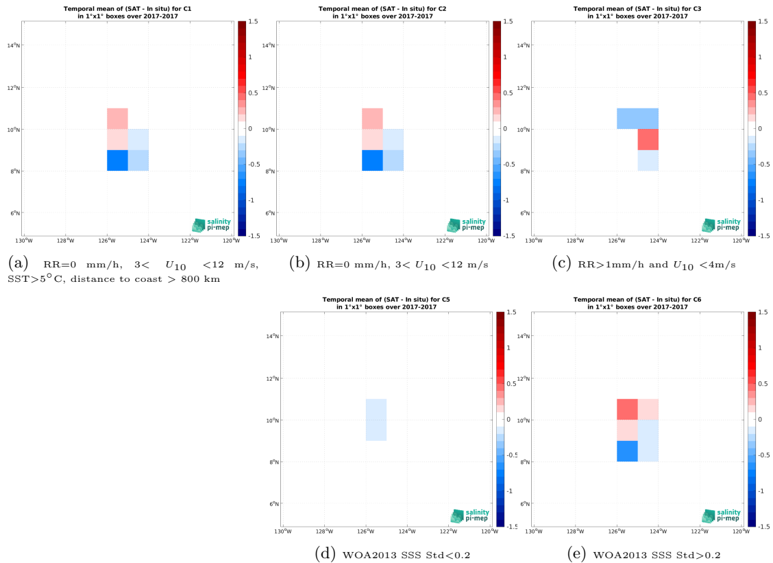
Figure 12: Temporal mean gridded over spatial boxes of size 1^\circ \times 1^\circ of \Delta SSS (SMAP SSS L2 v5 - 40 km (RSS) - Saildrone (SPURS 2)) for 5 different subdatasets corresponding to:RR=0 mm/h, 3 < U_{10} < 12 m/s, SST >5^\circ\text{C} , distance to coast > 800 km (a), RR=0 mm/h, 3 < U_{10} < 12 m/s (b), RR >1 mm/h and U_{10} < 4 m/s (c), WOA2013 SSS Std <0.2 (d), WOA2013 SSS Std >0.2 (e).
