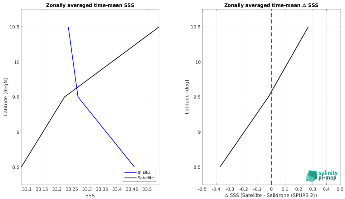
Figure 8: Left panel: Zonal mean SSS from SMAP SSS L2 v5 - 40 km (RSS) satellite product (black) and from Sairdrone (SPURS 2) (blue). Right panel: Zonal mean of \Delta SSS (Satellite - Sairdrone (SPURS 2)) for all the collected Pi-MEP match-up pairs estimated over the full satellite product period.
