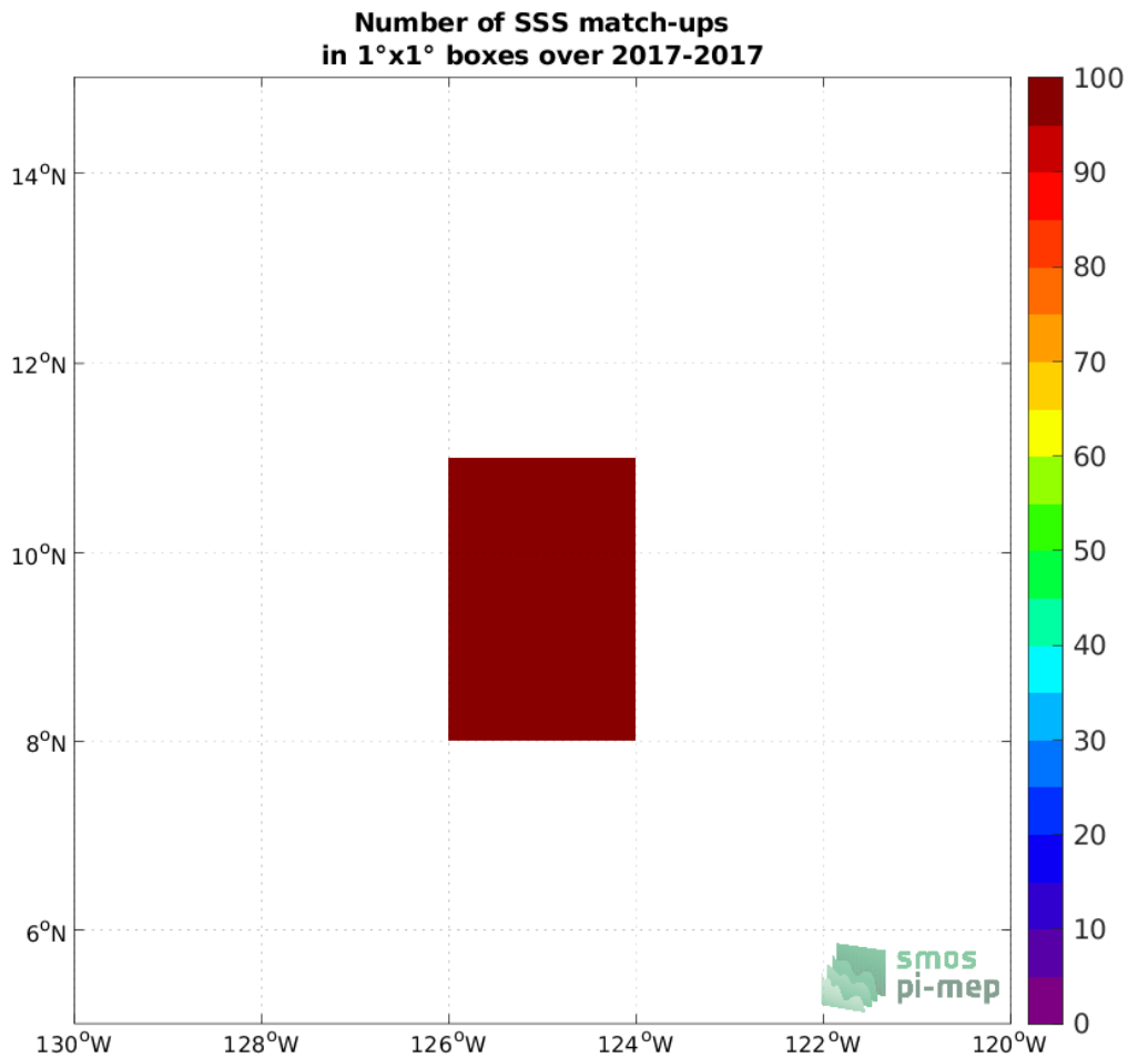
Figure 3: Number of SSS match-ups between Saildrone SSS and the SMAP SSS L2 v5 - 40 km (RSS) SSS product for the SPURS 2 Pi-MEP region over 1°x1° boxes and for the full satellite product period.
