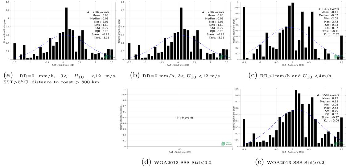
Figure 12: Normalized histogram of \Delta SSS (SMAP SSS L2 v5 - 40 km (RSS) - Saildrone) for 5 different subdatasets corresponding to: RR=0 mm/h, 3 < U_{10} < 12 m/s, SST>5°C, distance to coast > 800 km (a), RR=0 mm/h, 3 < U_{10} < 12 m/s (b), RR>1mm/h and U_{10} < 4 m/s (c), WOA2013 SSS Std<0.2 (d), WOA2013 SSS Std>0.2 (e).
