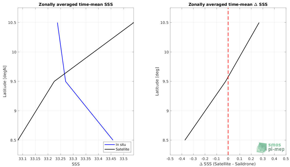
Figure 7: Left panel: Zonal mean SSS from SMAP SSS L2 v5 - 40 km (RSS) satellite product (black) and from Sairdrone (blue). Right panel: Zonal mean of \Delta SSS (Satellite - Sairdrone) for all the collected Pi-MEP match-up pairs estimated over the full satellite product period.
