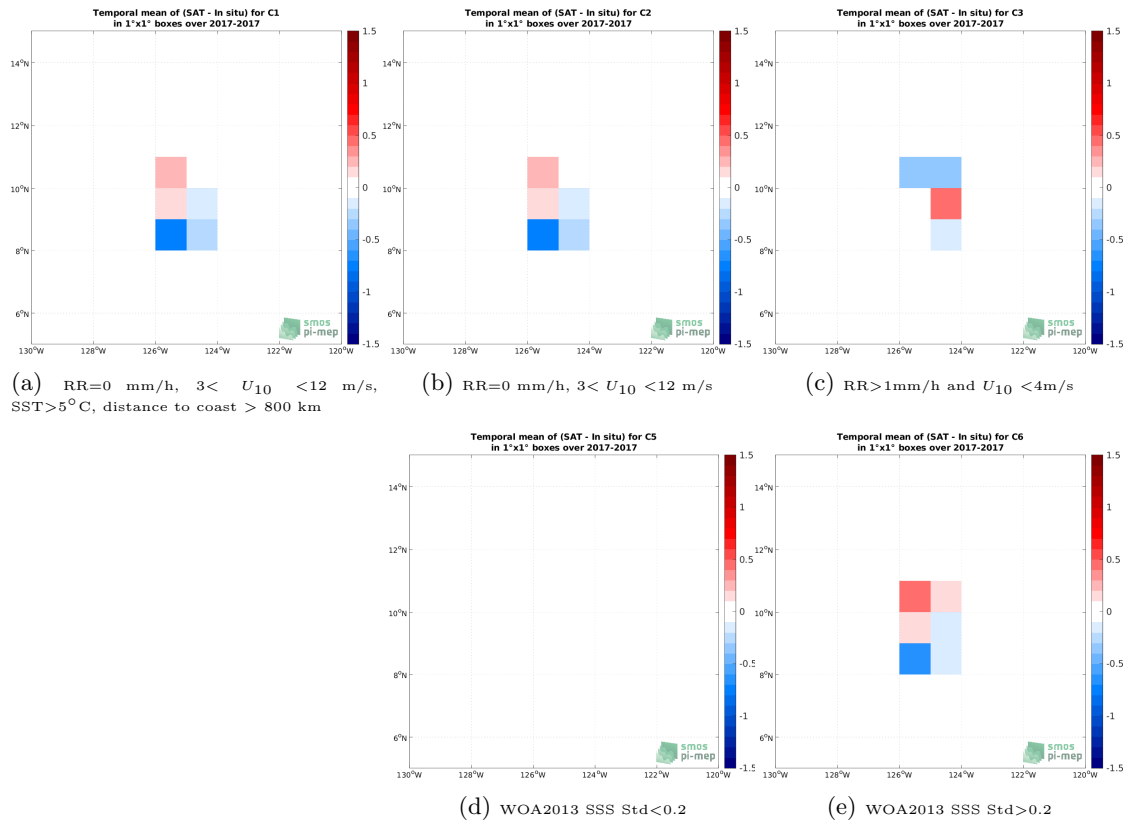
Figure 11: Temporal mean gridded over spatial boxes of size 1^\circ \times 1^\circ of \Delta SSS (SMAP SSS L2 v5 - 40 km (RSS) - Sairdrone) for 5 different subdatasets corresponding to:RR=0 mm/h, 3 < U_{10} < 12 m/s, SST >5^\circ\text{C} , distance to coast > 800 km (a), RR=0 mm/h, 3 < U_{10} < 12 m/s (b), RR >1 mm/h and U_{10} < 4 m/s (c), WOA2013 SSS Std <0.2 (d), WOA2013 SSS Std >0.2 (e).
