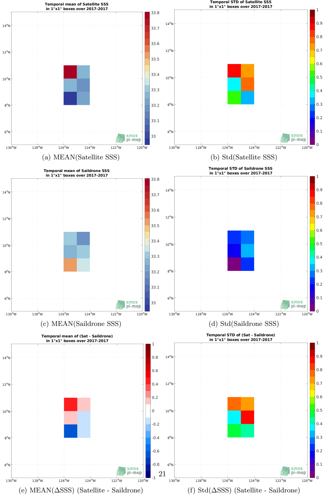
Figure 5: Temporal mean (left) and Std (right) of SSS from SMAP SSS L2 v5 - 40 km (RSS) (top), Saildrone (middle), and of \Delta SSS (Satellite - Saildrone). Only match-up pairs are used to generate these maps.
