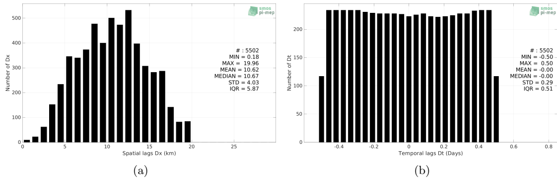
Figure 4: Histograms of the spatial (a) and temporal (b) lags between the location/time of the Saildrone measurement and the date of the corresponding SMAP SSS L2 v5 - 40 km (RSS) SSS pixel.
