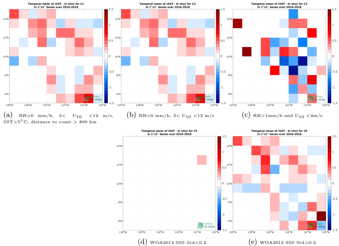
Figure 11: Temporal mean gridded over spatial boxes of size 1^\circ \times 1^\circ of \Delta SSS (SMAP SSS L2 v5 - 40 km (RSS) - Surface drifters) for 5 different subdatasets corresponding to:RR=0 mm/h, 3 < U_{10} < 12 m/s, SST > 5°C, distance to coast > 800 km (a), RR=0 mm/h, 3 < U_{10} < 12 m/s (b), RR > 1mm/h and U_{10} < 4 m/s (c), WOA2013 SSS Std < 0.2 (d), WOA2013 SSS Std > 0.2 (e).
