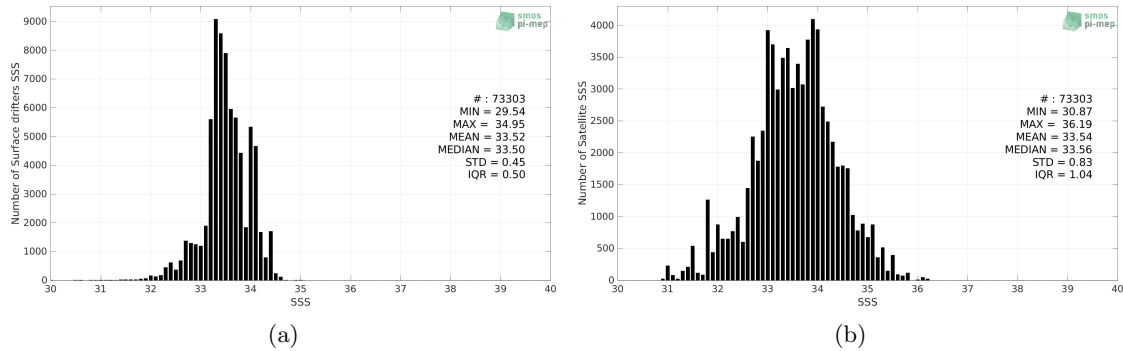
Figure 2: Histograms of SSS from Surface drifters (a) and SMAP SSS L2 v5 - 40 km (RSS) (b) considering all match-up pairs per bins of 0.1 over the SPURS 2 Pi-MEP region and for the full satellite product period.
