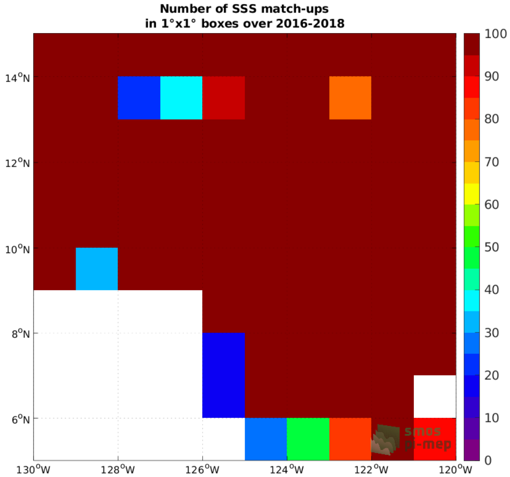
Figure 3: Number of SSS match-ups between Surface drifters SSS and the SMAP SSS L2 v5 - 40 km (RSS) SSS product for the SPURS 2 Pi-MEP region over 1°x1° boxes and for the full satellite product period.
