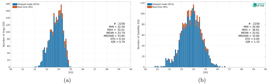
Figure 2: Histograms of SSS from Argo (a) and SMAP SSS L2 v5 - 40 km (RSS) (b) considering all match-up pairs per bins of 0.1 over the SPURS 2 Pi-MEP region and for the full satellite product period.
