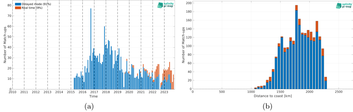
Figure 1: Number of match-ups between Argo and SMAP SSS L2 v5 - 40 km (RSS) SSS as a function of time (a) and as function of the distance to coast (b) over the SPURS 2 Pi-MEP region and for the full satellite product period.
