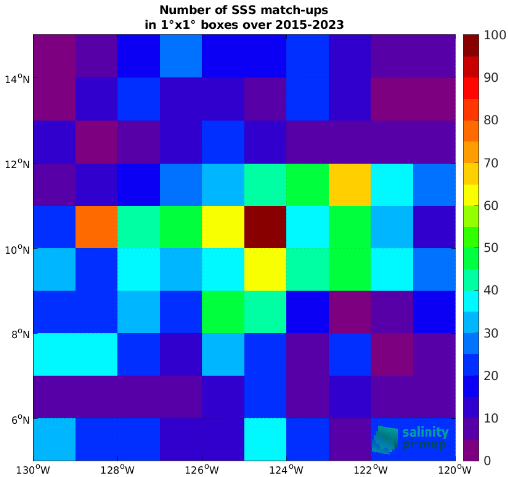
Figure 4: Number of SSS match-ups between Argo SSS and the SMAP SSS L2 v5 - 40 km (RSS) SSS product for the SPURS 2 Pi-MEP region over 1°x1° boxes and for the full satellite product period.
