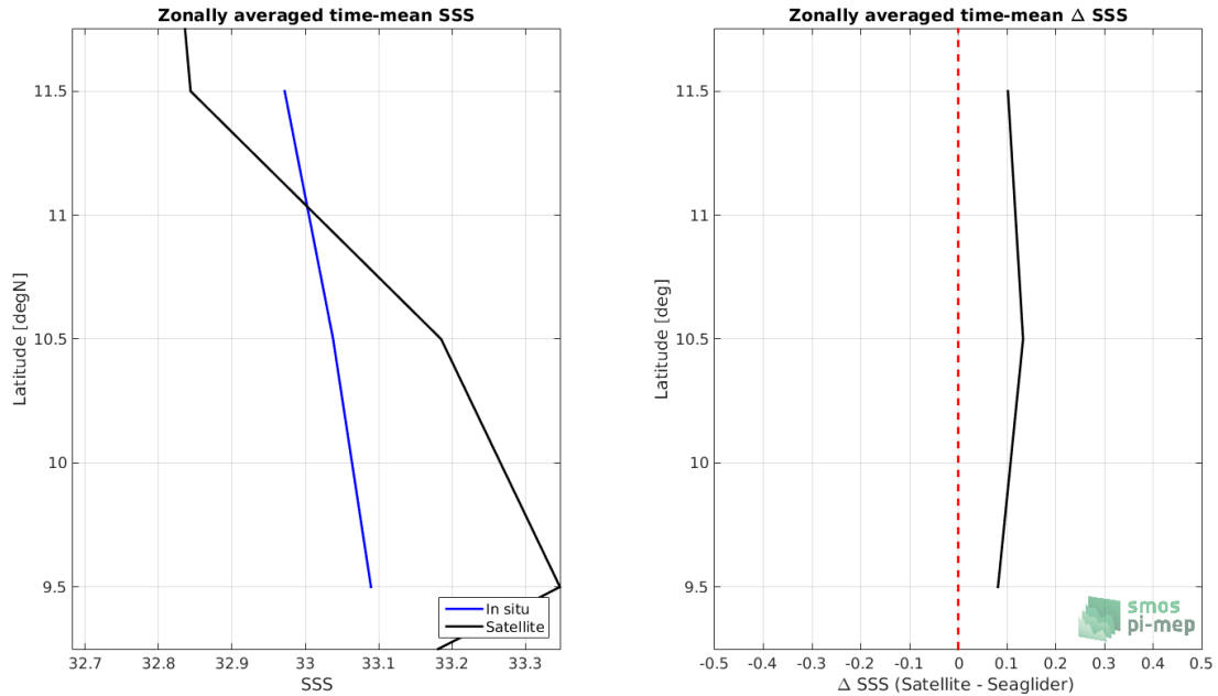
Figure 8: Left panel: Zonal mean SSS from SMAP SSS L2 v4 (RSS) satellite product (black) and from Seaglider (blue). Right panel: Zonal mean of \Delta SSS (Satellite - Seaglider) for all the collected Pi-MEP match-up pairs estimated over the full satellite product period.
