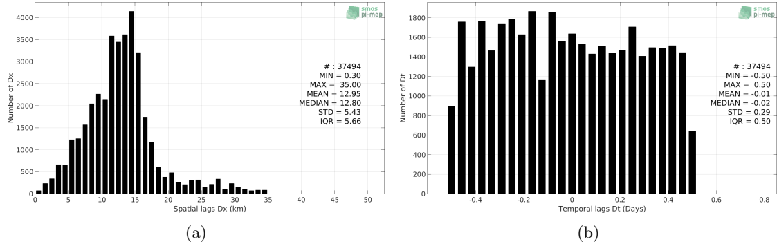
Figure 5: Histograms of the spatial (a) and temporal (b) lags between the time of the Seaglider measurements and the date of the corresponding SMAP SSS L2 v4 (RSS) SSS product.
