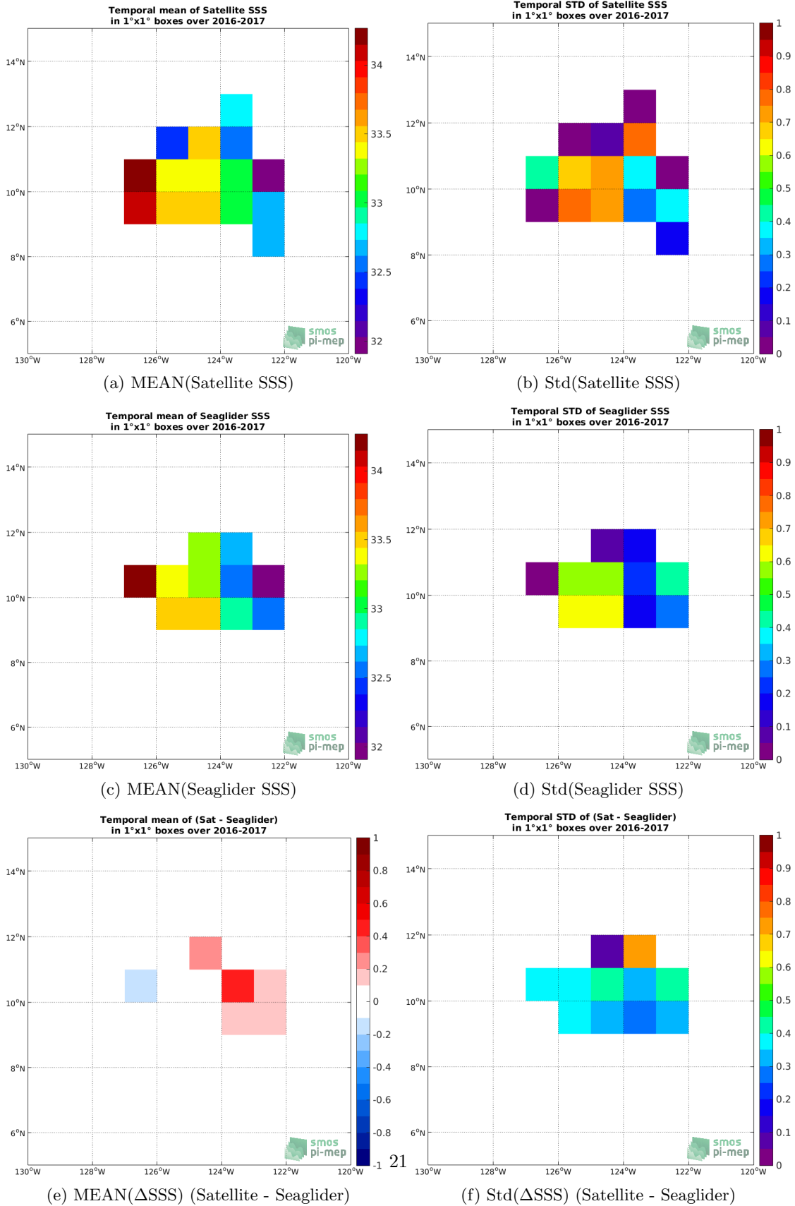
Figure 6: Temporal mean (left) and Std (right) of SSS from SMAP SSS L2 v4 (RSS) (top), Seaglider (middle), and of \Delta SSS (Satellite - Seaglider). Only match-up pairs are used to generate these maps.
