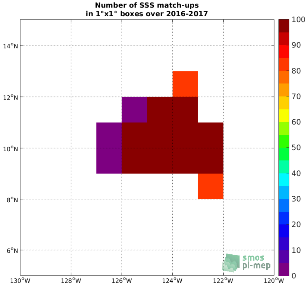
Figure 4: Number of SSS match-ups between Seaglider SSS and the SMAP SSS L2 v4 (RSS) SSS product for the SPURS 2 Pi-MEP region over 1°x1° boxes and for the full satellite product period.
