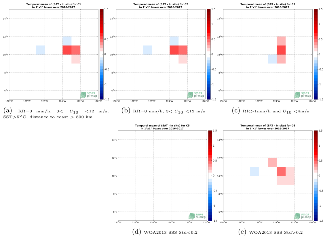
Figure 12: Temporal mean gridded over spatial boxes of size 1^\circ \times 1^\circ of \Delta SSS (SMAP SSS L2 v4 (RSS) - Seaglider) for 5 different subdatasets corresponding to:RR=0 mm/h, 3 < U_{10} < 12 m/s, SST >5^\circ\text{C} , distance to coast > 800 km (a), RR=0 mm/h, 3 < U_{10} < 12 m/s (b), RR >1 mm/h and U_{10} < 4 m/s (c), WOA2013 SSS Std <0.2 (d), WOA2013 SSS Std >0.2 (e).
