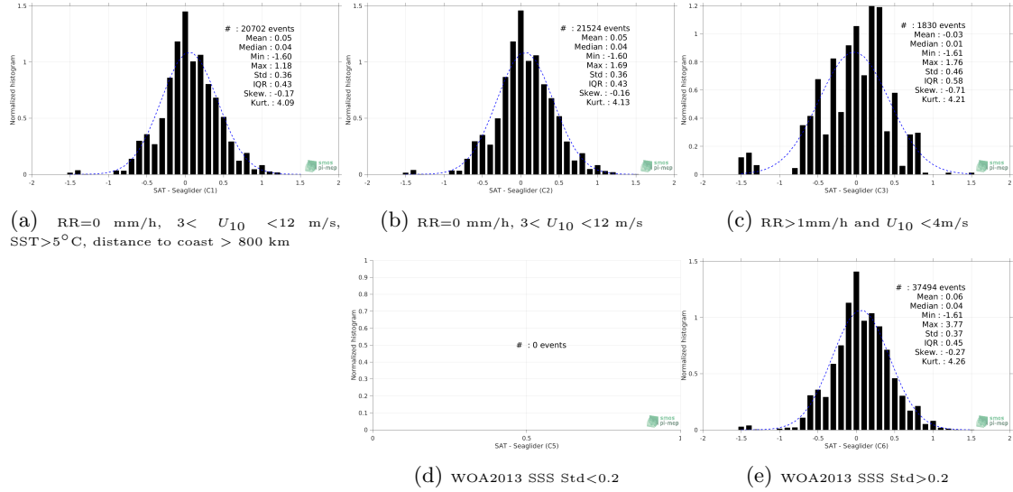
Figure 13: Normalized histogram of \Delta SSS (SMAP SSS L2 v4 (RSS) - Seaglider) for 5 different subdatasets corresponding to: RR=0 mm/h, 3 < U_{10} < 12 m/s, SST > 5°C, distance to coast > 800 km (a), RR=0 mm/h, 3 < U_{10} < 12 m/s (b), RR > 1mm/h and U_{10} < 4 m/s (c), WOA2013 SSS Std < 0.2 (d), WOA2013 SSS Std > 0.2 (e).
