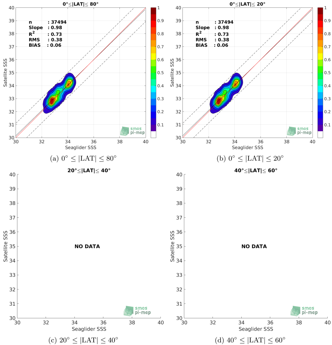
Figure 9: Contour maps of the concentration of SMAP SSS L2 v4 (RSS) SSS (y-axis) versus Seaglider SSS (x-axis) at match-up pairs for different latitude bands. For each plot, the red line shows x=y . The black thin and dashed lines indicate a linear fit through the data cloud and the \pm 95\% confidence levels, respectively. The number match-up pairs n , the slope and R^2 coefficient of the linear fit, the root mean square (RMS) and the mean bias between satellite and in situ data are indicated for each latitude band in each plots.
