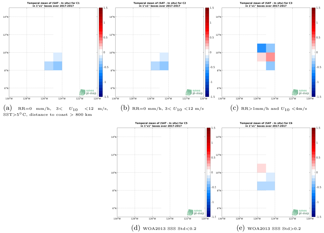
Figure 11: Temporal mean gridded over spatial boxes of size 1^\circ \times 1^\circ of \Delta SSS (SMAP SSS L2 v4 (RSS) - Saildrone) for 5 different subdatasets corresponding to: RR=0 mm/h, 3 < U_{10} < 12 m/s, SST>5°C, distance to coast > 800 km (a), RR=0 mm/h, 3 < U_{10} < 12 m/s (b), RR>1mm/h and U_{10} < 4 m/s (c), WOA2013 SSS Std<0.2 (d), WOA2013 SSS Std>0.2 (e).
