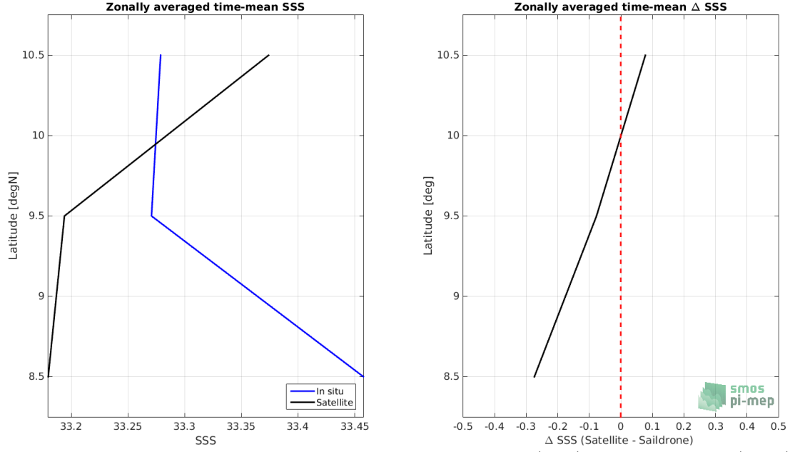
Figure 7: Left panel: Zonal mean SSS from SMAP SSS L2 v4 (RSS) satellite product (black) and from Saildrone (blue). Right panel: Zonal mean of \Delta SSS (Satellite - Saildrone) for all the collected Pi-MEP match-up pairs estimated over the full satellite product period.
