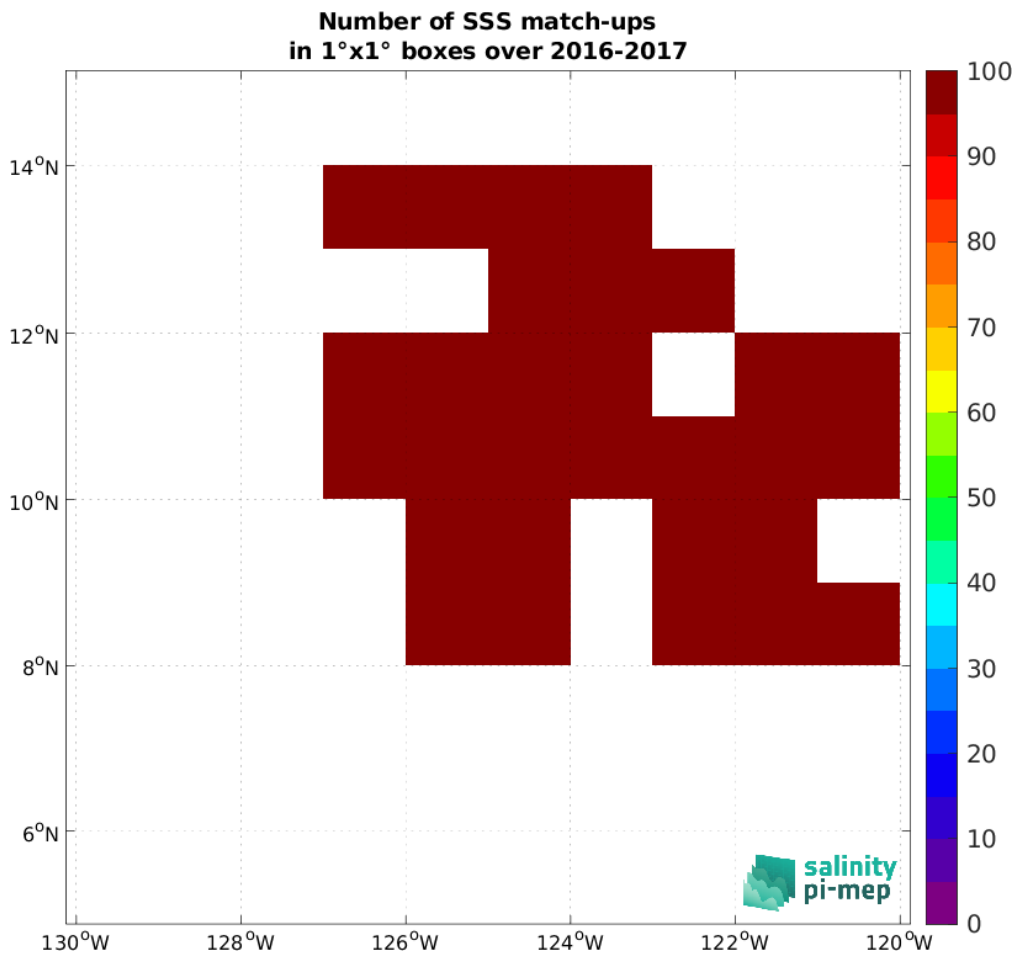
Figure 5: Number of SSS match-ups between Waveglider (SPURS 2) SSS and the SMAP SSS L2 v5.0 (JPL) SSS product for the SPURS 2 Pi-MEP region over 1^\circ \times 1^\circ boxes and for the full satellite product period.
