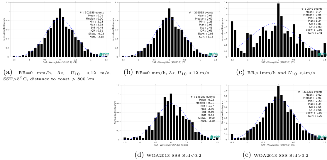
Figure 15: Normalized histogram of \Delta\text{SSS} (SMAP SSS L2 v5.0 (JPL) - Waveglider (SPURS 2)) for 5 different subdatasets corresponding to: RR=0 mm/h, 3 < U_{10} < 12 m/s, SST>5°C, distance to coast > 800 km (a), RR=0 mm/h, 3 < U_{10} < 12 m/s (b), RR>1mm/h and U_{10} < 4 m/s (c), WOA2013 SSS Std<0.2 (d), WOA2013 SSS Std>0.2 (e).
