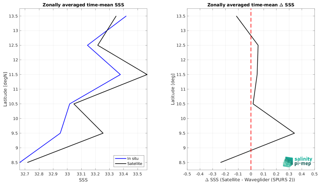
Figure 9: Left panel: Zonal mean SSS from SMAP SSS L2 v5.0 (JPL) satellite product (black) and from Waveglider (SPURS 2) (blue). Right panel: Zonal mean of \Delta SSS (Satellite - Waveglider (SPURS 2)) for all the collected Pi-MEP match-up pairs estimated over the full satellite product period.
