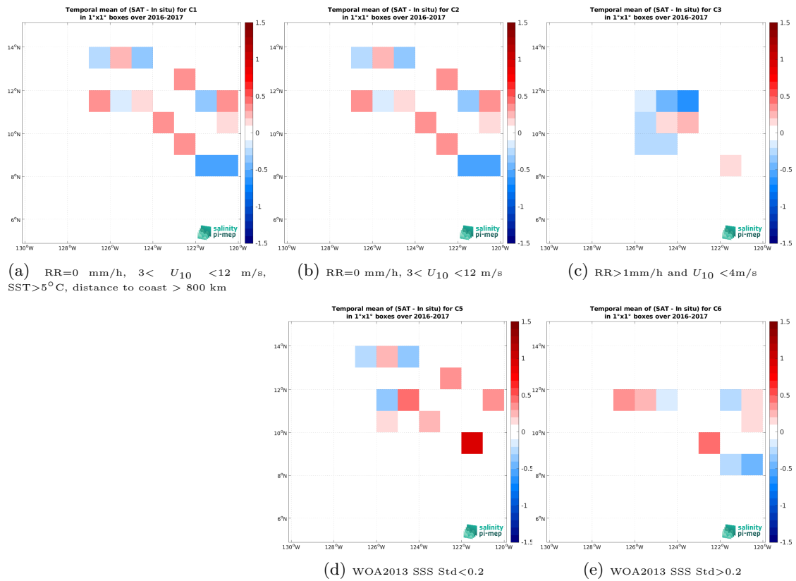
Figure 14: Temporal mean gridded over spatial boxes of size 1^\circ \times 1^\circ of \Delta SSS (SMAP SSS L2 v5.0 (JPL) - Waveglider (SPURS 2)) for 5 different subdatasets corresponding to:RR=0 mm/h, 3 < U_{10} < 12 m/s, SST>5°C, distance to coast > 800 km (a), RR=0 mm/h, 3 < U_{10} < 12 m/s (b), RR>1mm/h and U_{10} < 4 m/s (c), WOA2013 SSS Std<0.2 (d), WOA2013 SSS Std>0.2 (e).
