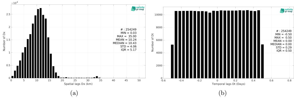
Figure 6: Histograms of the spatial (a) and temporal (b) lags between the location/time of the Waveglider (SPURS 2) measurement and the date of the corresponding SMAP SSS L2 v5.0 (JPL) SSS pixel.
