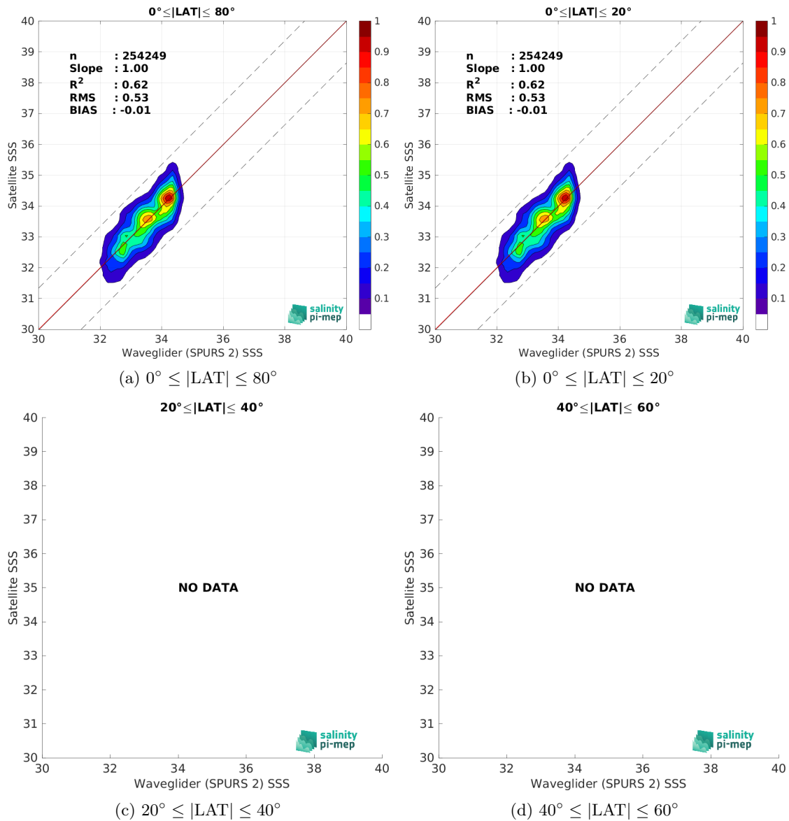
Figure 10: Contour maps of the concentration of SMAP SSS L2 v5.0 (JPL) SSS (y-axis) versus Waveglider (SPURS 2) SSS (x-axis) at match-up pairs for different latitude bands. For each plot, the red line shows x=y . The black thin and dashed lines indicate a linear fit through the data cloud and the \pm 95\% confidence levels, respectively. The number match-up pairs n , the slope and R^2 coefficient of the linear fit, the root mean square (RMS) and the mean bias between satellite and in situ data are indicated for each latitude band in each plots.
