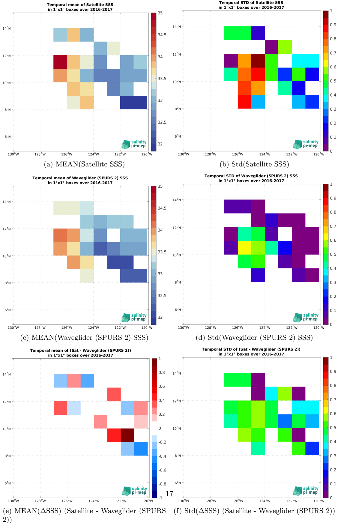
Figure 7: Temporal mean (left) and Std (right) of SSS from SMAP SSS L2 v5.0 (JPL) (top), Waveglider (SPURS 2) (middle), and of \Delta SSS (Satellite - Waveglider (SPURS 2)). Only match-up pairs are used to generate these maps.
