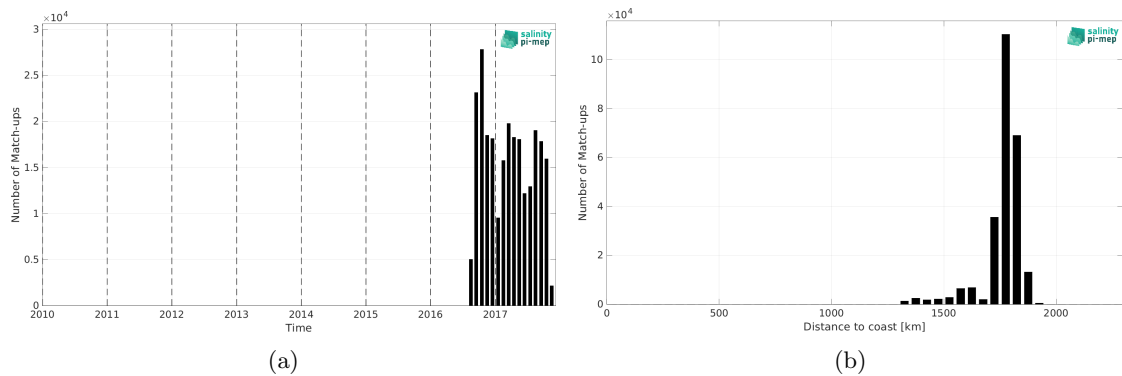
Figure 2: Number of match-ups between Waveglider (SPURS 2) and SMAP SSS L2 v5.0 (JPL) SSS as a function of time (a) and as function of the distance to coast (b) over the SPURS 2 Pi-MEP region and for the full satellite product period.
