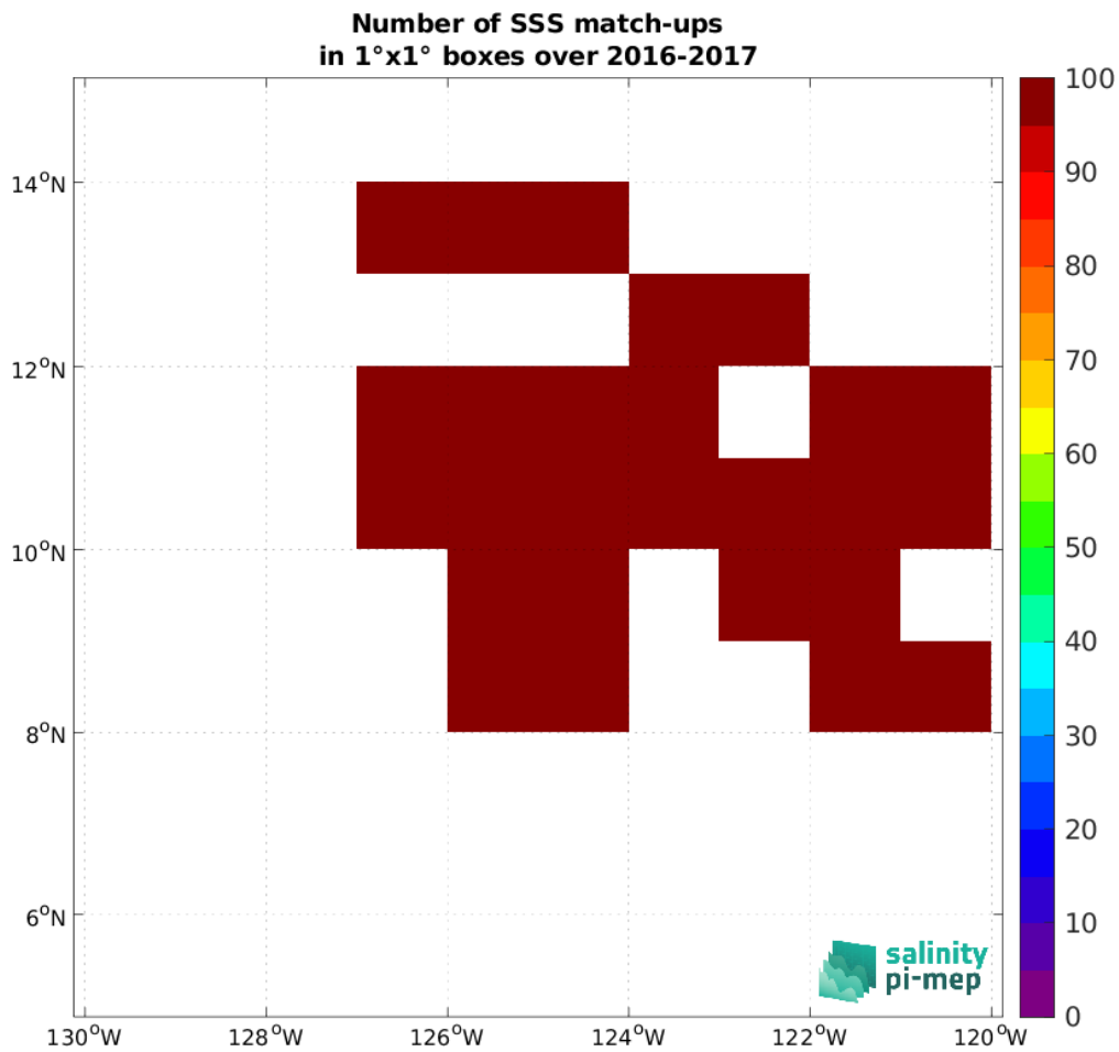
Figure 5: Number of SSS match-ups between Waveglider (SPURS 2) SSS and the SMAP SSS L2 v5.0 (JPL) SSS product for the SPURS 2 Pi-MEP region over 1°x1° boxes and for the full satellite product period.
