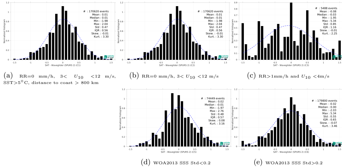
Figure 15: Normalized histogram of \Delta SSS (SMAP SSS L2 v5.0 (JPL) - Waveglider (SPURS 2)) for 5 different subdatasets corresponding to: RR=0 mm/h, 3 < U_{10} < 12 m/s, SST>5°C, distance to coast > 800 km (a), RR=0 mm/h, 3 < U_{10} < 12 m/s (b), RR>1mm/h and U_{10} < 4 m/s (c), WOA2013 SSS Std<0.2 (d), WOA2013 SSS Std>0.2 (e).
