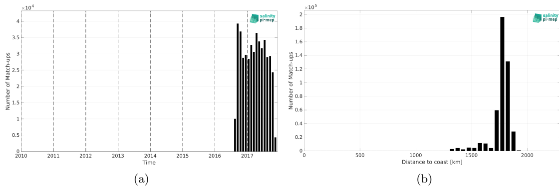
Figure 1: Number of match-ups between Waveglider (SPURS 2) and SMAP SSS L2 v5.0 (JPL) SSS as a function of time (a) and as function of the distance to coast (b) over the SPURS 2 Pi-MEP region and for the full satellite product period.
