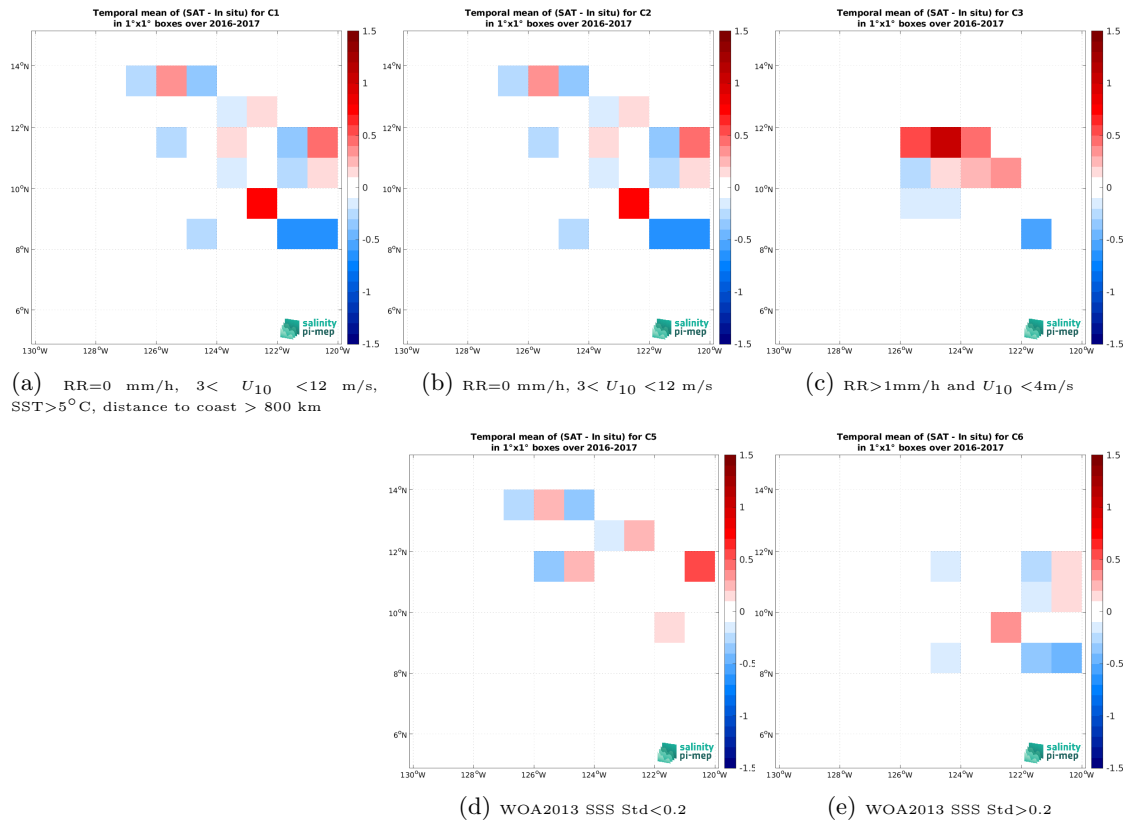
Figure 12: Temporal mean gridded over spatial boxes of size 1^\circ \times 1^\circ of \Delta SSS (SMAP SSS L2 v5.0 (JPL) - Waveglider (SPURS 2)) for 5 different subdatasets corresponding to:RR=0 mm/h, 3 < U_{10} < 12 m/s, SST >5^\circ\text{C} , distance to coast > 800 km (a), RR=0 mm/h, 3 < U_{10} < 12 m/s (b), RR >1 mm/h and U_{10} < 4 m/s (c), WOA2013 SSS Std <0.2 (d), WOA2013 SSS Std >0.2 (e).
