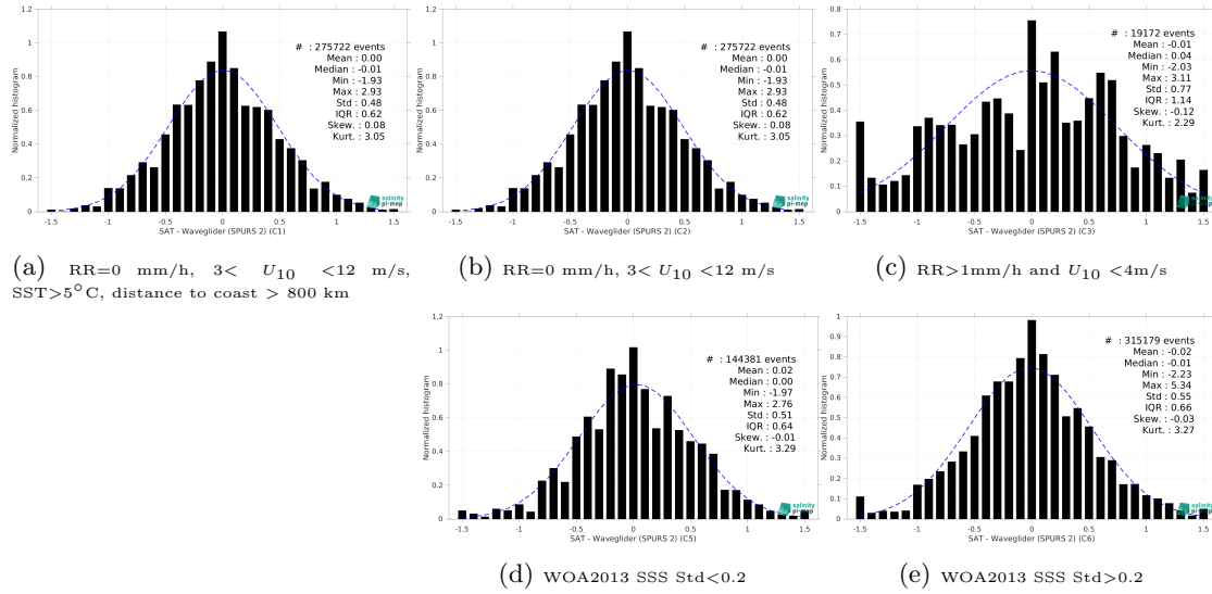
Figure 13: Normalized histogram of \Delta SSS (SMAP SSS L2 v5.0 (JPL) - Waveglider (SPURS 2)) for 5 different subdatasets corresponding to: RR=0 mm/h, 3 < U_{10} < 12 m/s, SST > 5°C, distance to coast > 800 km (a), RR=0 mm/h, 3 < U_{10} < 12 m/s (b), RR > 1mm/h and U_{10} < 4 m/s (c), WOA2013 SSS Std < 0.2 (d), WOA2013 SSS Std > 0.2 (e).
