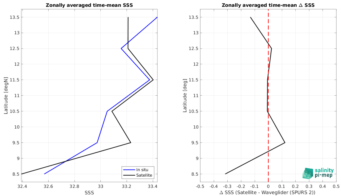
Figure 8: Left panel: Zonal mean SSS from SMAP SSS L2 v5.0 (JPL) satellite product (black) and from Waveglider (SPURS 2) (blue). Right panel: Zonal mean of \Delta SSS (Satellite - Waveglider (SPURS 2)) for all the collected Pi-MEP match-up pairs estimated over the full satellite product period.
