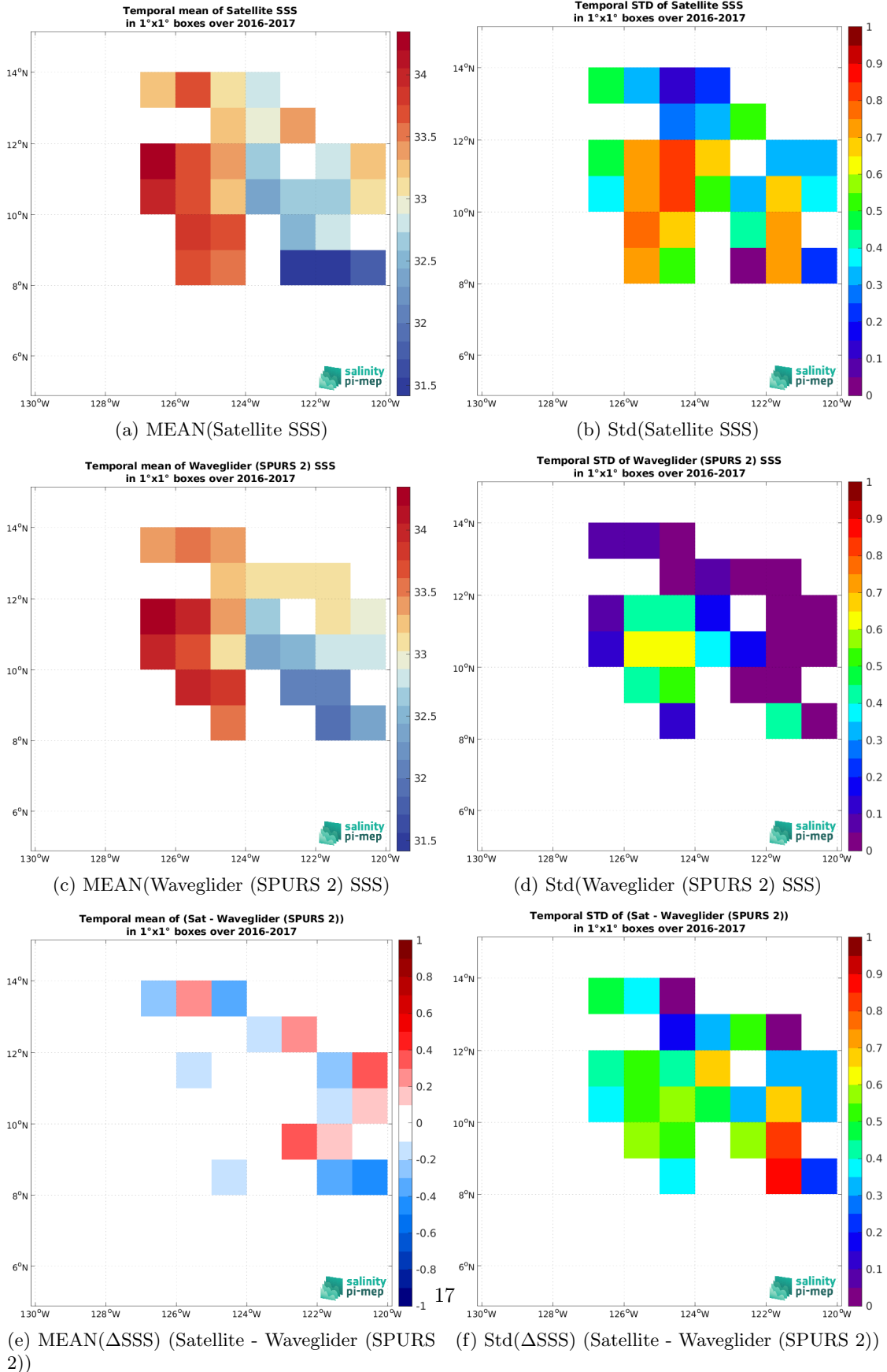
Figure 6: Temporal mean (left) and Std (right) of SSS from SMAP SSS L2 v5.0 (JPL) (top), Waveglider (SPURS 2) (middle), and of \Delta SSS (Satellite - Waveglider (SPURS 2)). Only match-up pairs are used to generate these maps.
