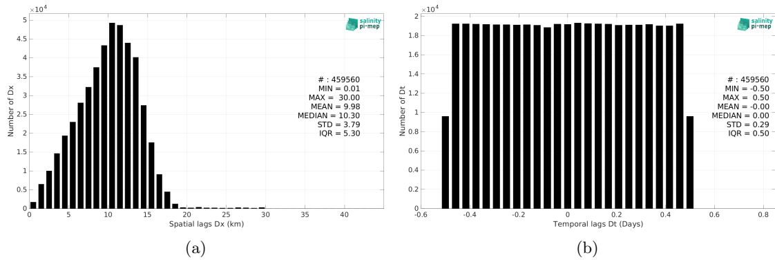
Figure 5: Histograms of the spatial (a) and temporal (b) lags between the location/time of the Waveglider (SPURS 2) measurement and the date of the corresponding SMAP SSS L2 v5.0 (JPL) SSS pixel.
