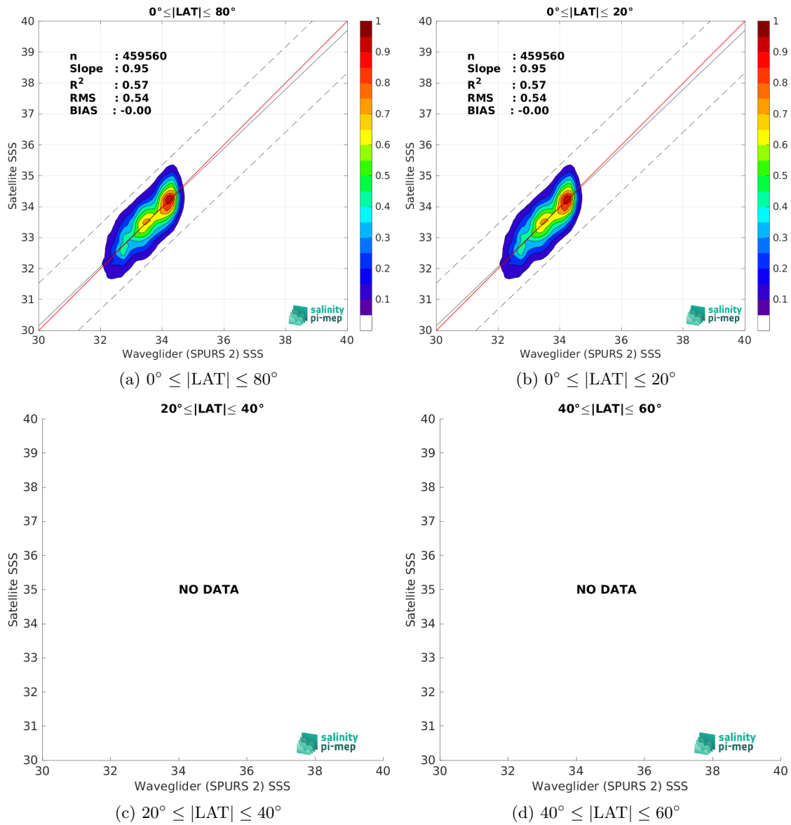
Figure 9: Contour maps of the concentration of SMAP SSS L2 v5.0 (JPL) SSS (y-axis) versus Waveglider (SPURS 2) SSS (x-axis) at match-up pairs for different latitude bands. For each plot, the red line shows x=y . The black thin and dashed lines indicate a linear fit through the data cloud and the \pm 95\% confidence levels, respectively. The number match-up pairs n , the slope and R^2 coefficient of the linear fit, the root mean square (RMS) and the mean bias between satellite and in situ data are indicated for each latitude band in each plots.
