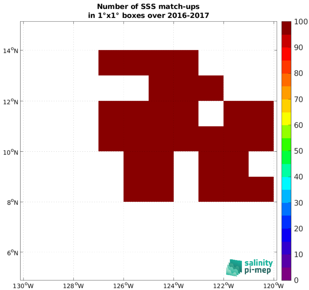
Figure 4: Number of SSS match-ups between Waveglider (SPURS 2) SSS and the SMAP SSS L2 v5.0 (JPL) SSS product for the SPURS 2 Pi-MEP region over 1°x1° boxes and for the full satellite product period.
