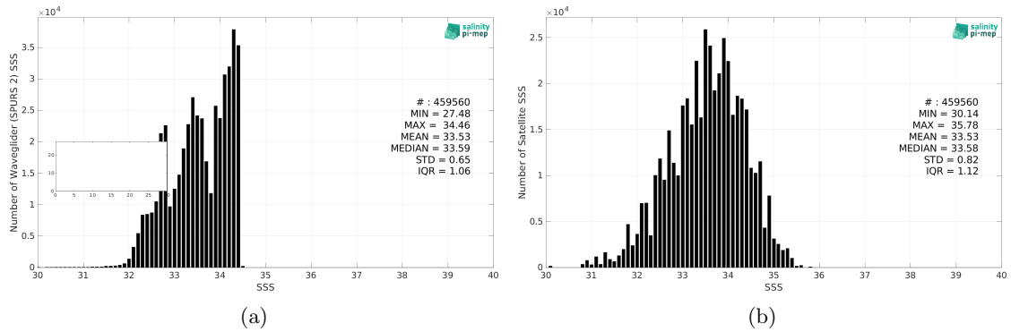
Figure 2: Histograms of SSS from Waveglider (SPURS 2) (a) and SMAP SSS L2 v5.0 (JPL) (b) considering all match-up pairs per bins of 0.1 over the SPURS 2 Pi-MEP region and for the full satellite product period.
