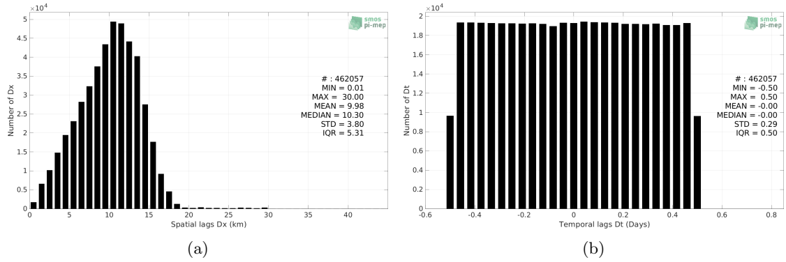
Figure 5: Histograms of the spatial (a) and temporal (b) lags between the location/time of the Waveglider measurement and the date of the corresponding SMAP SSS L2 v5.0 (JPL) SSS pixel.
