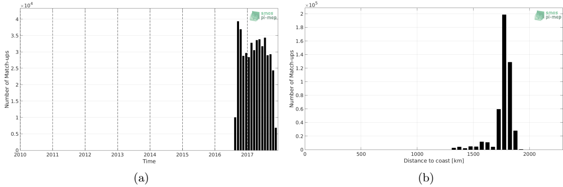
Figure 1: Number of match-ups between Waveglider and SMAP SSS L2 v5.0 (JPL) SSS as a function of time (a) and as function of the distance to coast (b) over the SPURS 2 Pi-MEP region and for the full satellite product period.
