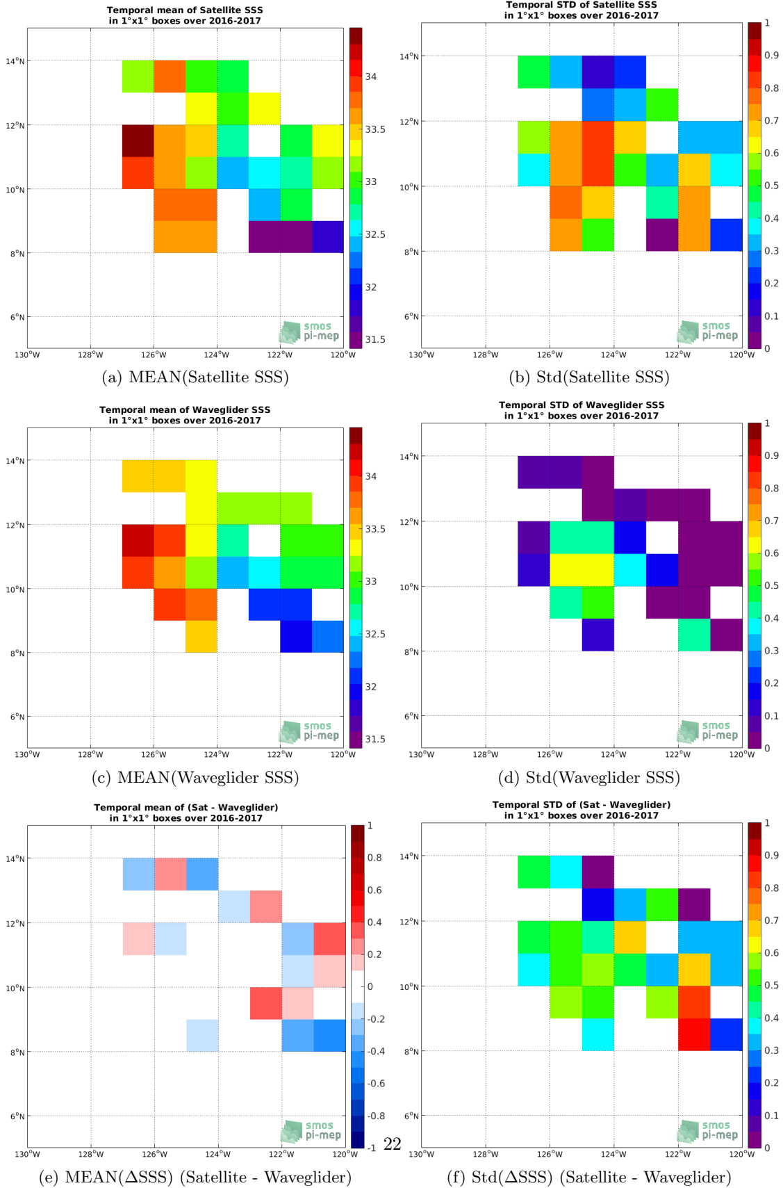
Figure 6: Temporal mean (left) and Std (right) of SSS from SMAP SSS L2 v5.0 (JPL) (top), Waveglider (middle), and of \Delta SSS (Satellite - Waveglider). Only match-up pairs are used to generate these maps.
