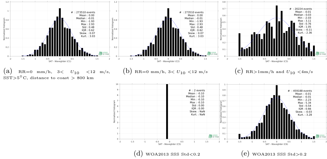
Figure 13: Normalized histogram of \Delta SSS (SMAP SSS L2 v5.0 (JPL) - Waveglider) for 5 different subdatasets corresponding to: RR=0 mm/h, 3 < U_{10} < 12 m/s, SST > 5°C, distance to coast > 800 km (a), RR=0 mm/h, 3 < U_{10} < 12 m/s (b), RR > 1mm/h and U_{10} < 4 m/s (c), WOA2013 SSS Std < 0.2 (d), WOA2013 SSS Std > 0.2 (e).
