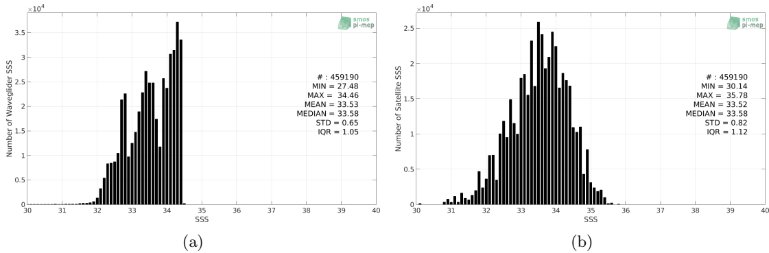
Figure 2: Histograms of SSS from Waveglider (a) and SMAP SSS L2 v5.0 (JPL) (b) considering all match-up pairs per bins of 0.1 over the SPURS 2 Pi-MEP region and for the full satellite product period.
