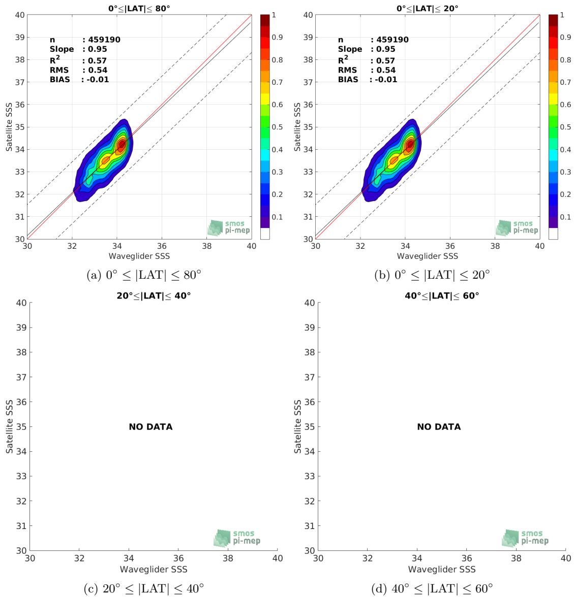
Figure 9: Contour maps of the concentration of SMAP SSS L2 v5.0 (JPL) SSS (y-axis) versus Waveglider SSS (x-axis) at match-up pairs for different latitude bands. For each plot, the red line shows x=y . The black thin and dashed lines indicate a linear fit through the data cloud and the \pm 95\% confidence levels, respectively. The number match-up pairs n , the slope and R^2 coefficient of the linear fit, the root mean square (RMS) and the mean bias between satellite and in situ data are indicated for each latitude band in each plots.
