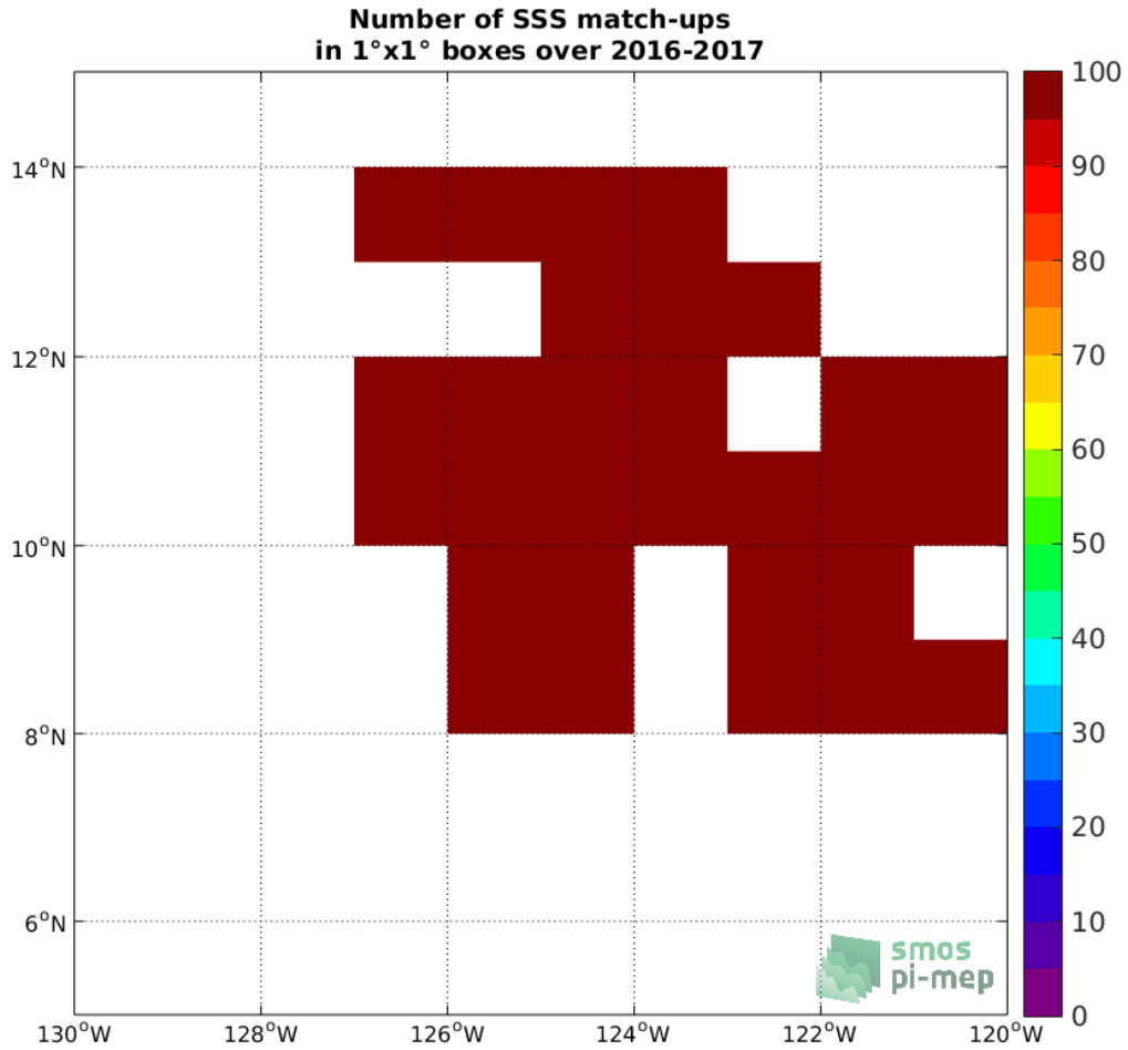
Figure 4: Number of SSS match-ups between Waveglider SSS and the SMAP SSS L2 v5.0 (JPL) SSS product for the SPURS 2 Pi-MEP region over 1°x1° boxes and for the full satellite product period.
