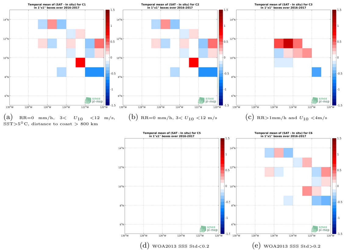
Figure 12: Temporal mean gridded over spatial boxes of size 1^\circ \times 1^\circ of \Delta SSS (SMAP SSS L2 v5.0 (JPL) - Waveglider) for 5 different subdatasets corresponding to:RR=0 mm/h, 3 < U_{10} < 12 m/s, SST >5^\circ\text{C} , distance to coast > 800 km (a), RR=0 mm/h, 3 < U_{10} < 12 m/s (b), RR >1 mm/h and U_{10} < 4 m/s (c), WOA2013 SSS Std <0.2 (d), WOA2013 SSS Std >0.2 (e).
