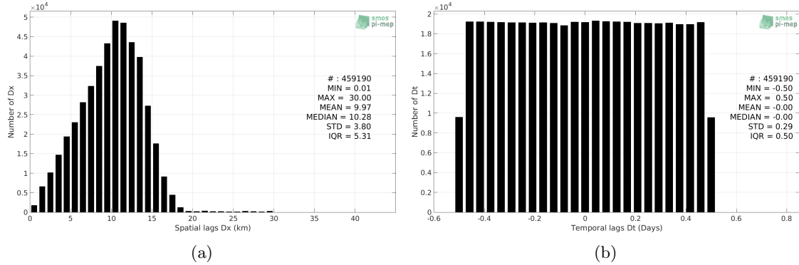
Figure 5: Histograms of the spatial (a) and temporal (b) lags between the time of the Waveglider measurements and the date of the corresponding SMAP SSS L2 v5.0 (JPL) SSS product.
