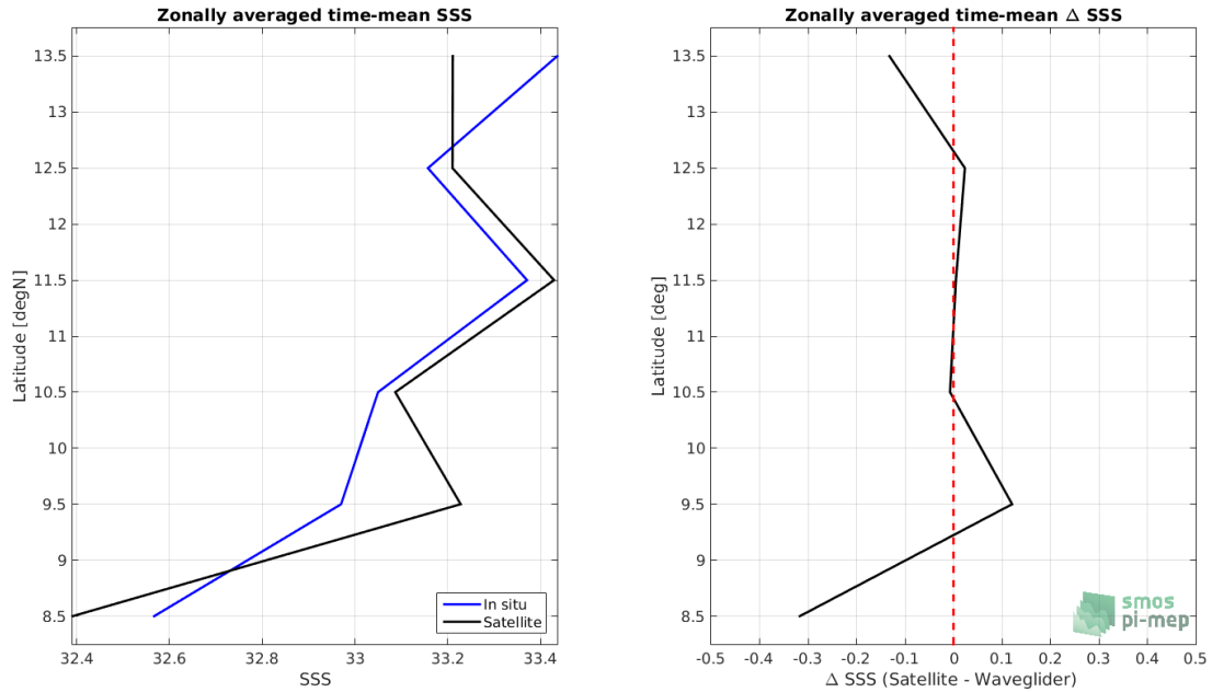
Figure 8: Left panel: Zonal mean SSS from SMAP SSS L2 v5.0 (JPL) satellite product (black) and from Waveglider (blue). Right panel: Zonal mean of \Delta SSS (Satellite - Waveglider) for all the collected Pi-MEP match-up pairs estimated over the full satellite product period.
