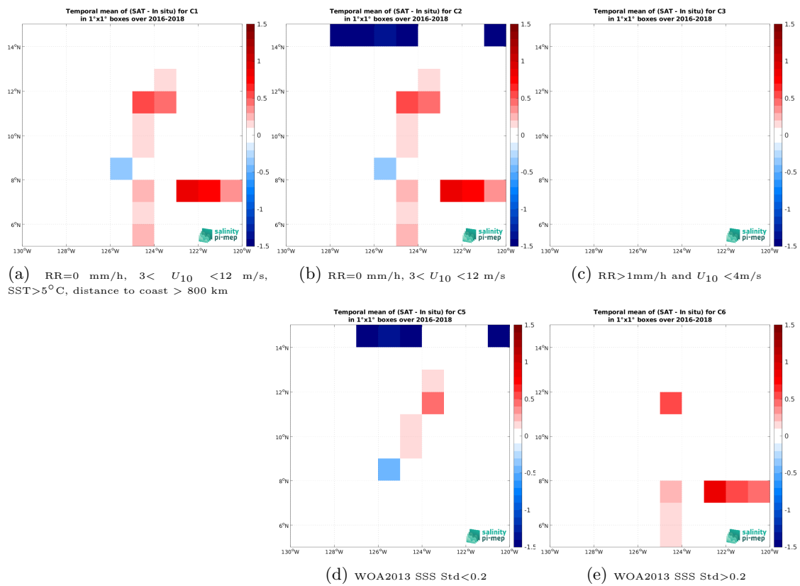
Figure 14: Temporal mean gridded over spatial boxes of size 1^\circ \times 1^\circ of \Delta SSS (SMAP SSS L2 v5.0 (JPL) - TSG (SAMOS)) for 5 different subdatasets corresponding to:RR=0 mm/h, 3 < U_{10} < 12 m/s, SST > 5°C, distance to coast > 800 km (a), RR=0 mm/h, 3 < U_{10} < 12 m/s (b), RR > 1mm/h and U_{10} < 4 m/s (c), WOA2013 SSS Std < 0.2 (d), WOA2013 SSS Std > 0.2 (e).
