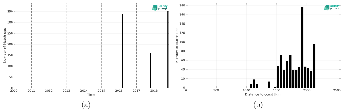
Figure 2: Number of match-ups between TSG (SAMOS) and SMAP SSS L2 v5.0 (JPL) SSS as a function of time (a) and as function of the distance to coast (b) over the SPURS 2 Pi-MEP region and for the full satellite product period.
