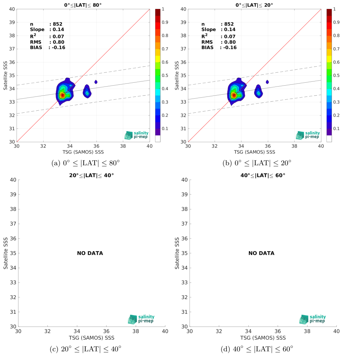
Figure 10: Contour maps of the concentration of SMAP SSS L2 v5.0 (JPL) SSS (y-axis) versus TSG (SAMOS) SSS (x-axis) at match-up pairs for different latitude bands. For each plot, the red line shows x=y . The black thin and dashed lines indicate a linear fit through the data cloud and the \pm 95\% confidence levels, respectively. The number match-up pairs n , the slope and R^2 coefficient of the linear fit, the root mean square (RMS) and the mean bias between satellite and in situ data are indicated for each latitude band in each plots.
