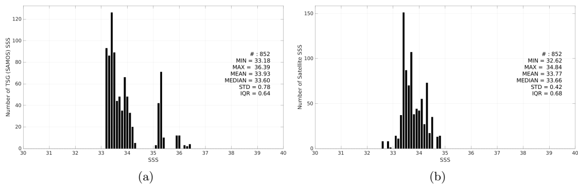
Figure 3: Histograms of SSS from TSG (SAMOS) (a) and SMAP SSS L2 v5.0 (JPL) (b) considering all match-up pairs per bins of 0.1 over the SPURS 2 Pi-MEP region and for the full satellite product period.
