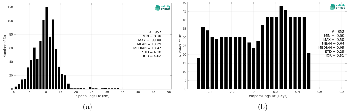
Figure 6: Histograms of the spatial (a) and temporal (b) lags between the location/time of the TSG (SAMOS) measurement and the date of the corresponding SMAP SSS L2 v5.0 (JPL) SSS pixel.
