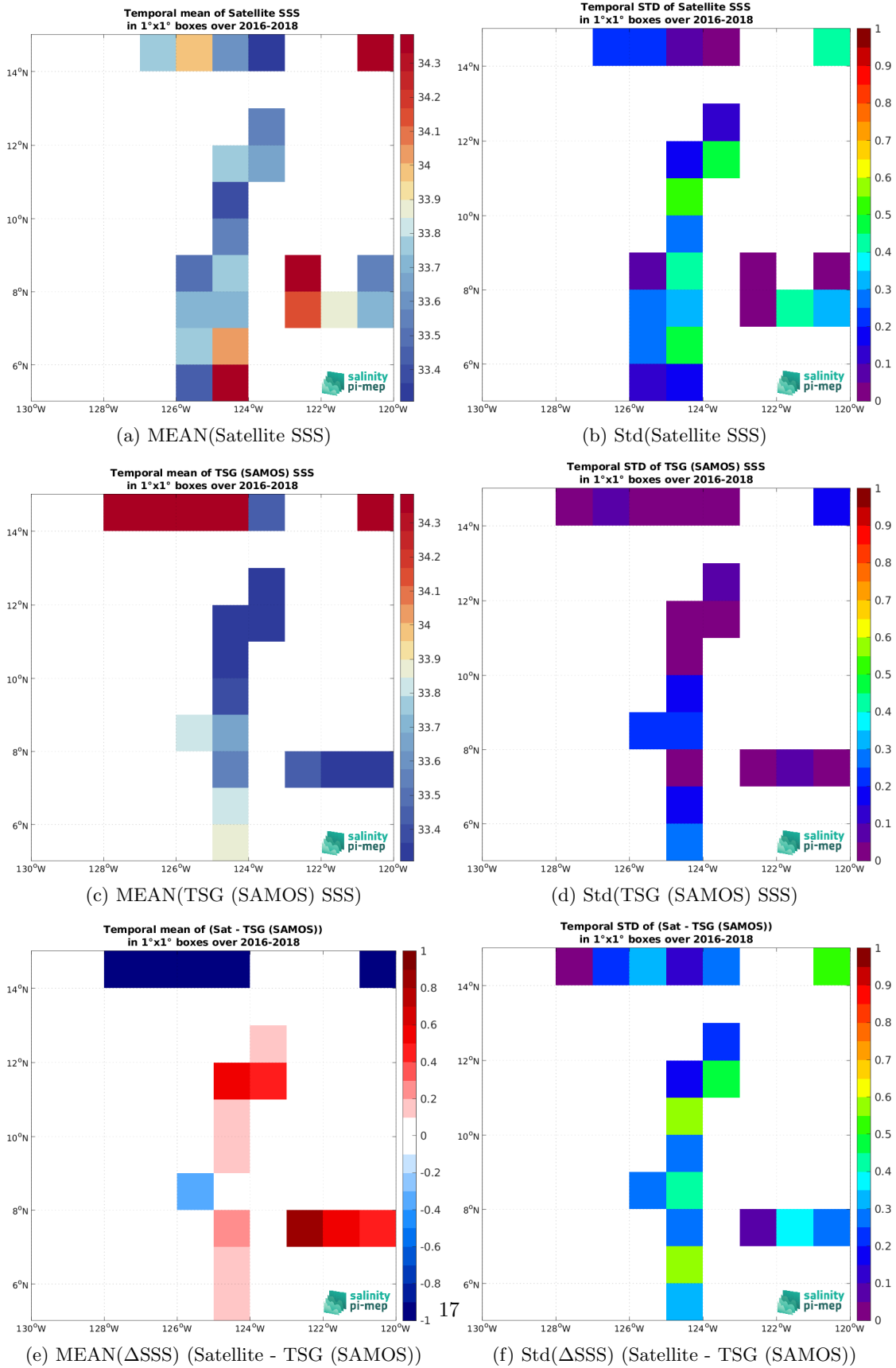
Figure 7: Temporal mean (left) and Std (right) of SSS from SMAP SSS L2 v5.0 (JPL) (top), TSG (SAMOS) (middle), and of \Delta SSS (Satellite - TSG (SAMOS)). Only match-up pairs are used to generate these maps.
