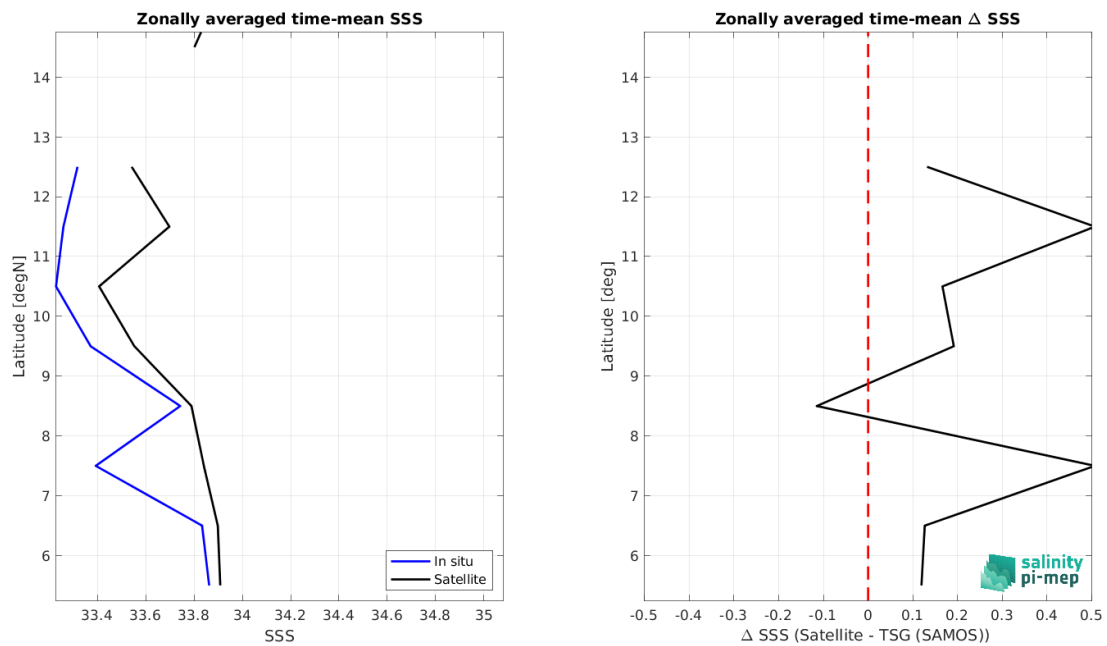
Figure 9: Left panel: Zonal mean SSS from SMAP SSS L2 v5.0 (JPL) satellite product (black) and from TSG (SAMOS) (blue). Right panel: Zonal mean of \Delta SSS (Satellite - TSG (SAMOS)) for all the collected Pi-MEP match-up pairs estimated over the full satellite product period.
