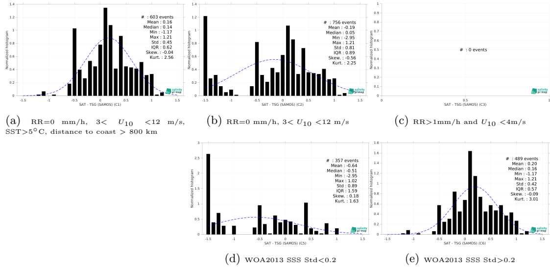
Figure 15: Normalized histogram of \Delta SSS (SMAP SSS L2 v5.0 (JPL) - TSG (SAMOS)) for 5 different subdatasets corresponding to: RR=0 mm/h, 3 < U_{10} < 12 m/s, SST > 5°C, distance to coast > 800 km (a), RR=0 mm/h, 3 < U_{10} < 12 m/s (b), RR > 1mm/h and U_{10} < 4 m/s (c), WOA2013 SSS Std < 0.2 (d), WOA2013 SSS Std > 0.2 (e).
