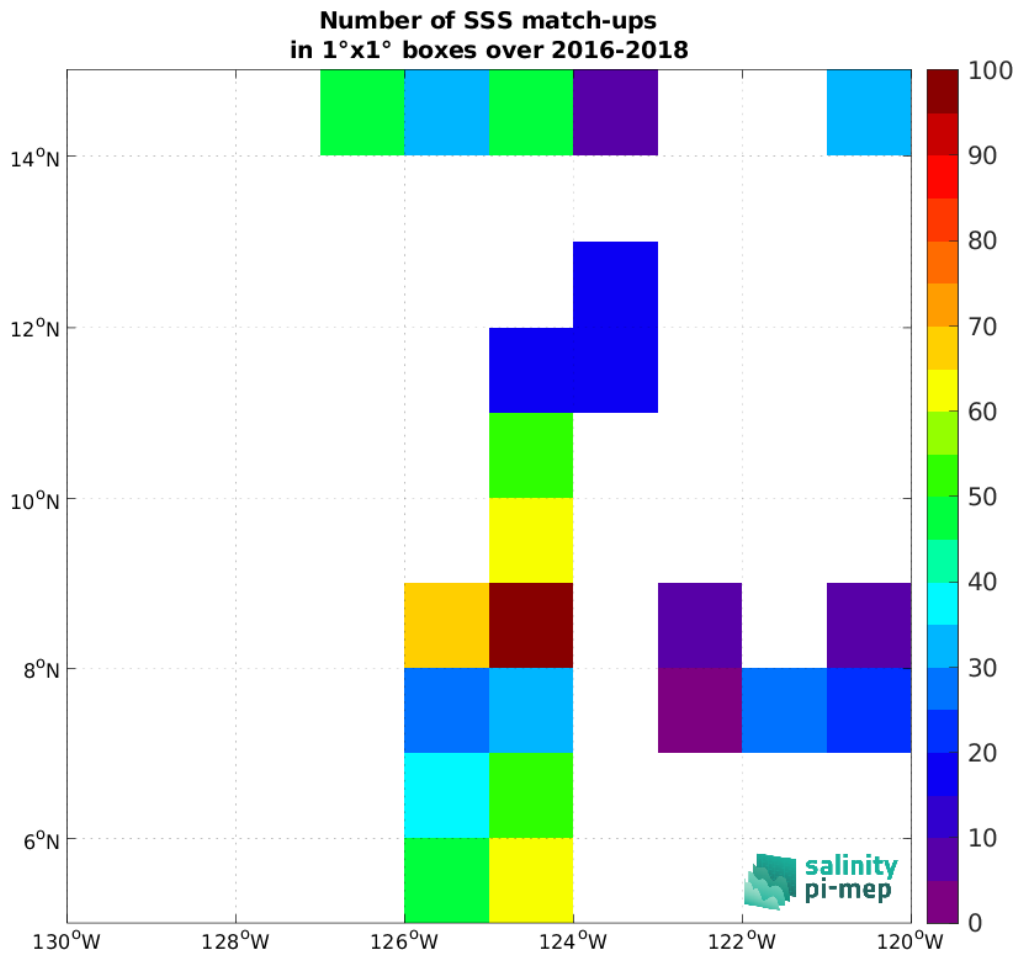
Figure 5: Number of SSS match-ups between TSG (SAMOS) SSS and the SMAP SSS L2 v5.0 (JPL) SSS product for the SPURS 2 Pi-MEP region over 1°x1° boxes and for the full satellite product period.
