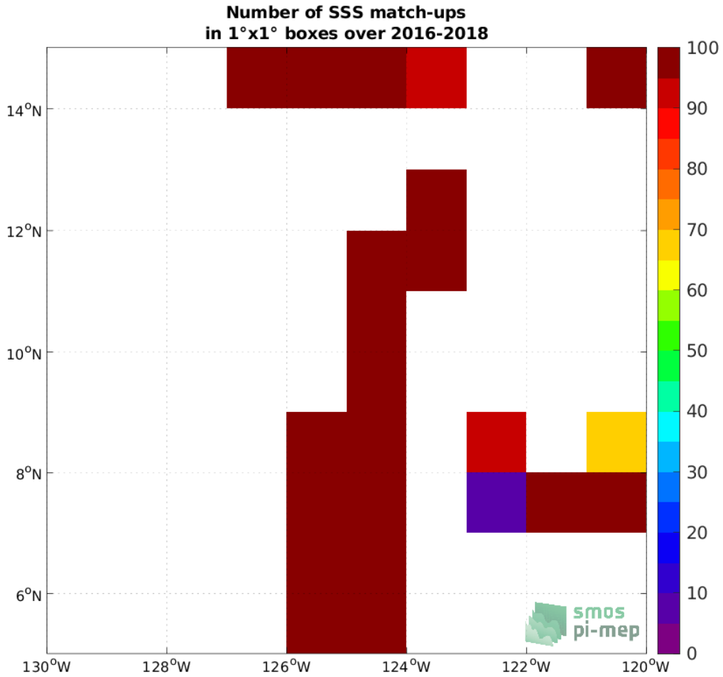
Figure 4: Number of SSS match-ups between TSG (SAMOS) SSS and the SMAP SSS L2 v5.0 (JPL) SSS product for the SPURS 2 Pi-MEP region over 1°x1° boxes and for the full satellite product period.
