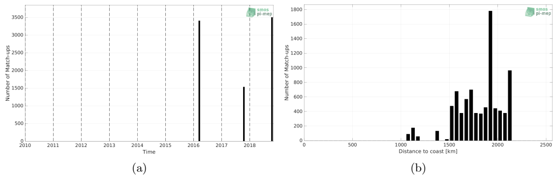
Figure 1: Number of match-ups between TSG (SAMOS) and SMAP SSS L2 v5.0 (JPL) SSS as a function of time (a) and as function of the distance to coast (b) over the SPURS 2 Pi-MEP region and for the full satellite product period.
