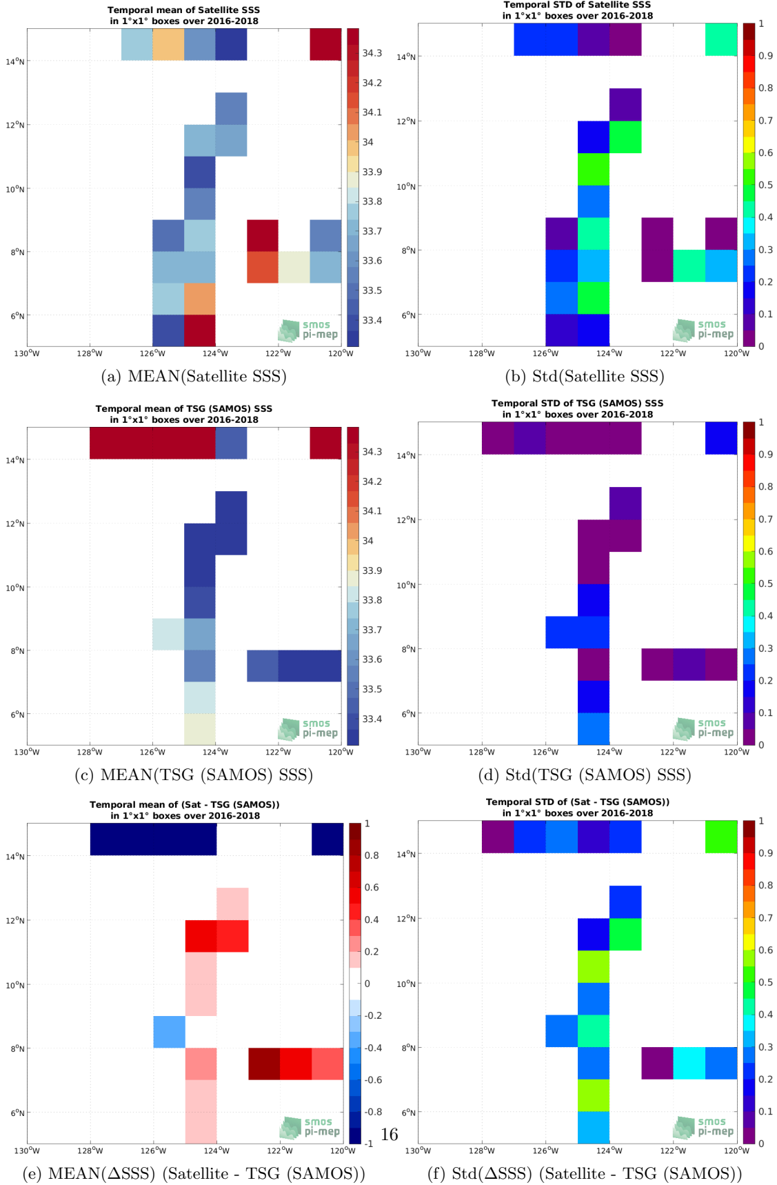
Figure 6: Temporal mean (left) and Std (right) of SSS from SMAP SSS L2 v5.0 (JPL) (top), TSG (SAMOS) (middle), and of \Delta SSS (Satellite - TSG (SAMOS)). Only match-up pairs are used to generate these maps.
