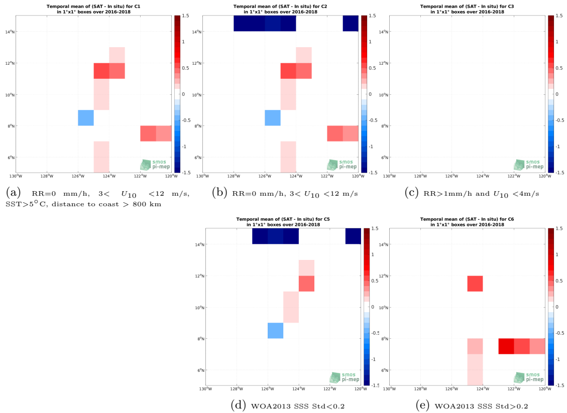
Figure 12: Temporal mean gridded over spatial boxes of size 1^\circ \times 1^\circ of \Delta SSS (SMAP SSS L2 v5.0 (JPL) - TSG (SAMOS)) for 5 different subdatasets corresponding to:RR=0 mm/h, 3 < U_{10} < 12 m/s, SST >5^\circ C, distance to coast > 800 km (a), RR=0 mm/h, 3 < U_{10} < 12 m/s (b), RR >1 mm/h and U_{10} < 4 m/s (c), WOA2013 SSS Std <0.2 (d), WOA2013 SSS Std >0.2 (e).
