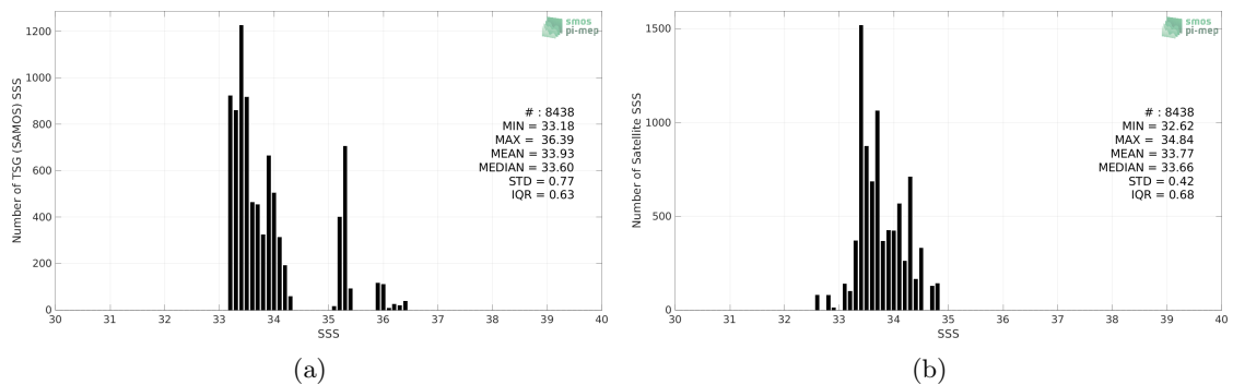
Figure 2: Histograms of SSS from TSG (SAMOS) (a) and SMAP SSS L2 v5.0 (JPL) (b) considering all match-up pairs per bins of 0.1 over the SPURS 2 Pi-MEP region and for the full satellite product period.
